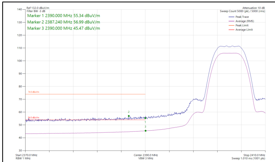
Figure 41 - Bluetooth HDR8, SISO, Core 0 - 2404 MHz Band Edge Frequency 2390 MHz
