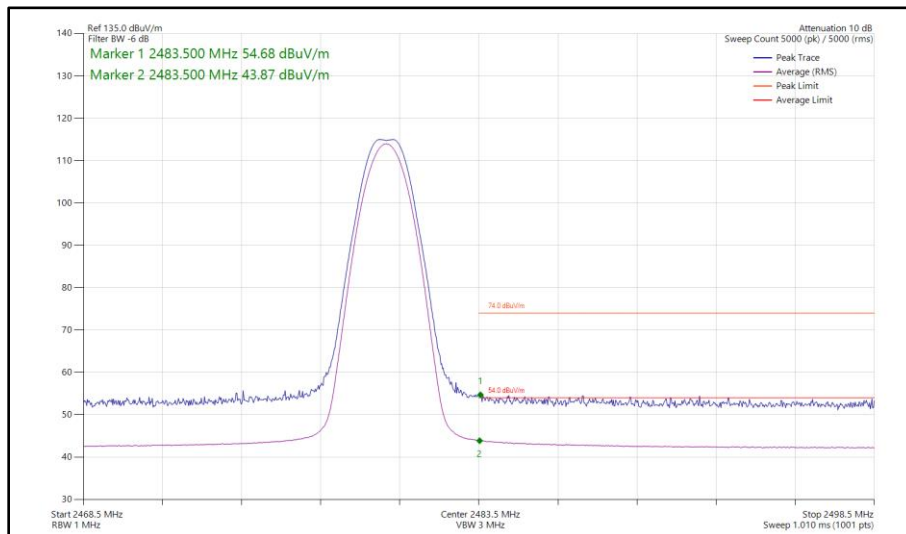
Figure 66 - Bluetooth LE1M, MIMO, Core 0 - Core 1 - 2480 MHz Band Edge Frequency 2483.5 MHz
