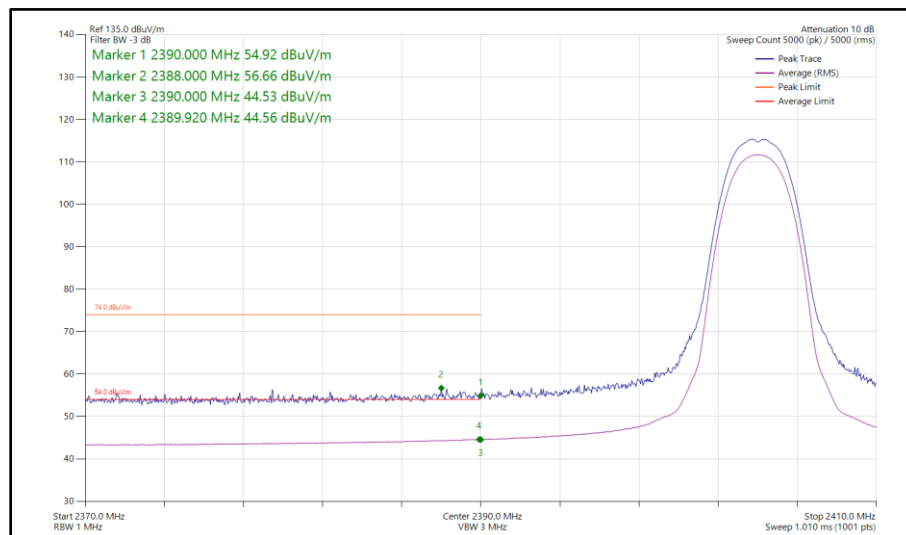
Figure 50 - Bluetooth HDR4, SISO, Core 1 - 2404 MHz Band Edge Frequency 2390 MHz
