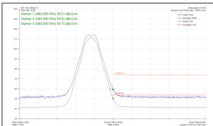
Figure 68 - Bluetooth LE2M, MIMO, Core 0 - Core 1 - 2480 MHz Band Edge Frequency 2483.5 MHz
