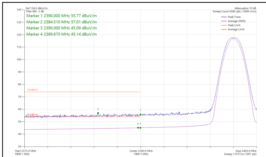
Figure 52 - Bluetooth LE1M, SISO, Core 1 - 2402 MHz Band Edge Frequency 2390 MHz
