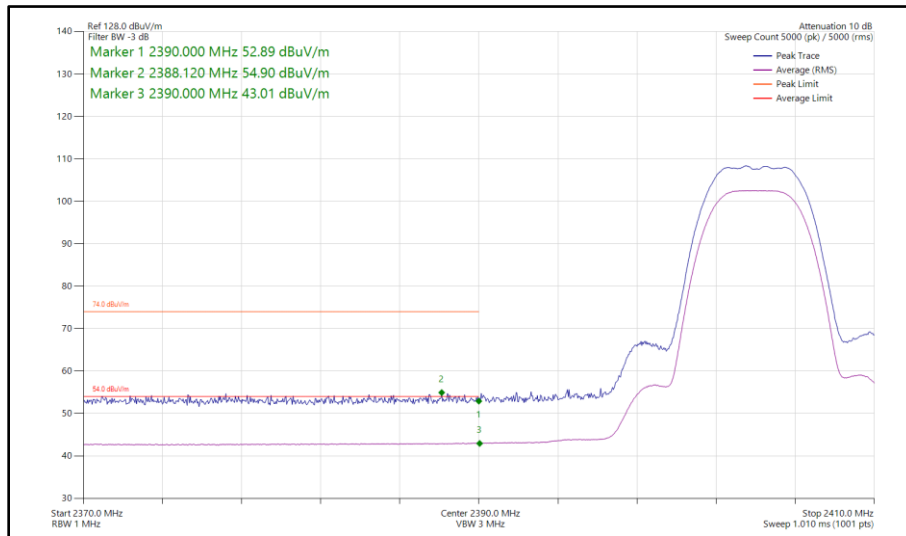
Figure 31 - Bluetooth HDR8, MIMO, Core 0 - Core 1 - 2404 MHz Band Edge Frequency 2390 MHz
