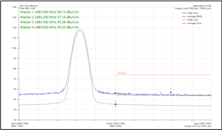
Figure 46 - Bluetooth LE1M, SISO, Core 0 - 2478 MHz Band Edge Frequency 2483.5 MHz
