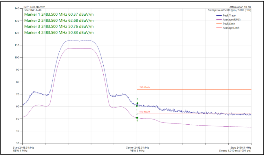
Figure 45 - Bluetooth HDR8, SISO, Core 0 - 2476 MHz Band Edge Frequency 2483.5 MHz
