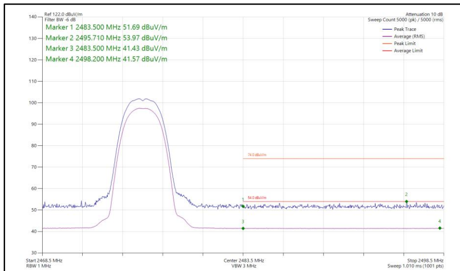
Figure 34 - Bluetooth HDR4, MIMO, Core 0 - Core 1 - 2476 MHz Band Edge Frequency 2483.5 MHz
