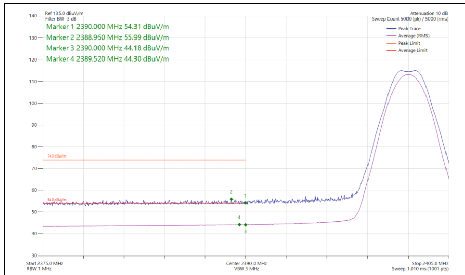
Figure 43 - Bluetooth LE2M, SISO, Core 0 - 2402 MHz Band Edge Frequency 2390 MHz
