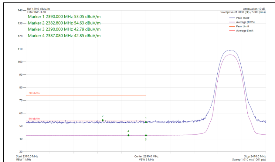
Figure 30 - Bluetooth HDR4, MIMO, Core 0 - Core 1 - 2404 MHz Band Edge Frequency 2390 MHz
