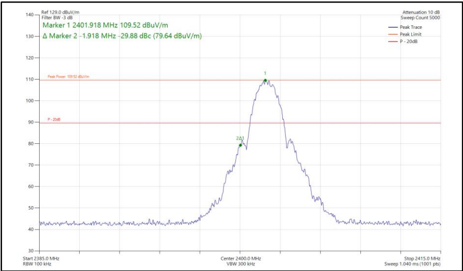
Figure 244 - Bluetooth LE2M, SISO, Core 1 - 2402 MHz Band Edge Frequency 2400 MHz
