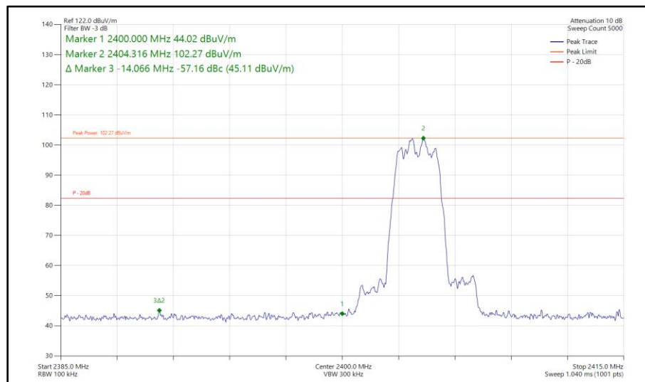
Figure 241 - Bluetooth HDR4, SISO, Core 1 - 2404 MHz Band Edge Frequency 2400 MHz
