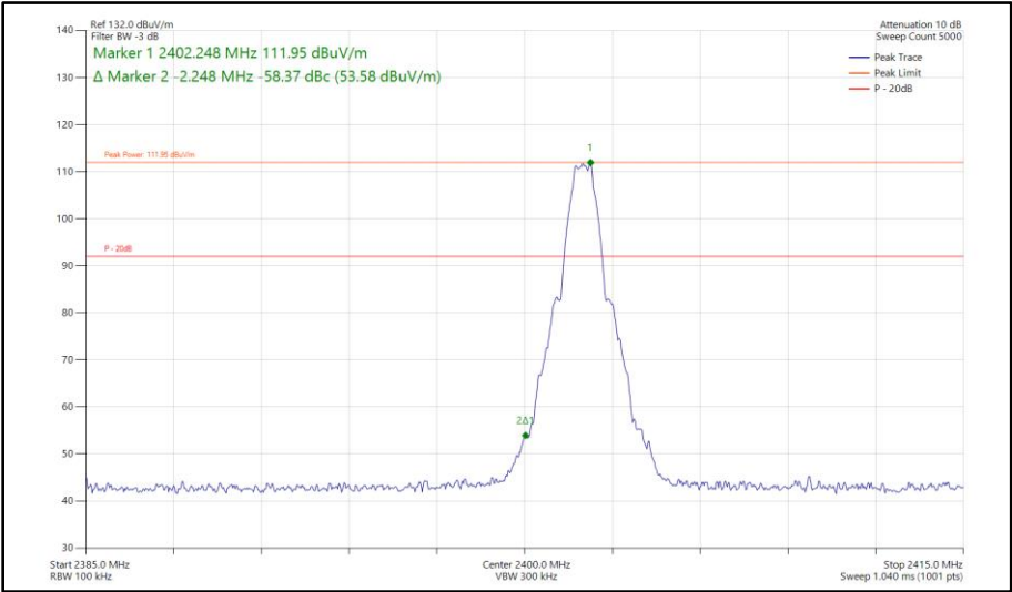
Figure 243 - Bluetooth LE1M, SISO, Core 1 - 2402 MHz Band Edge Frequency 2400 MHz
