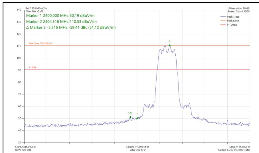
Figure 257 - Bluetooth HDR4, SISO, Core 1 - 2404 MHz Band Edge Frequency 2400 MHz
