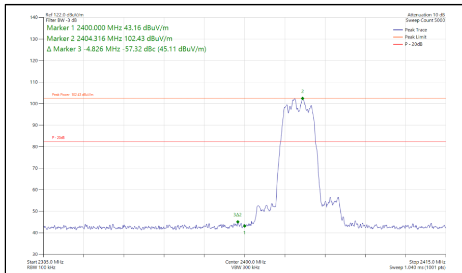
Figure 249 - Bluetooth HDR4, MIMO, Core 0 - Core 1 - 2404 MHz Band Edge Frequency 2400 MHz
