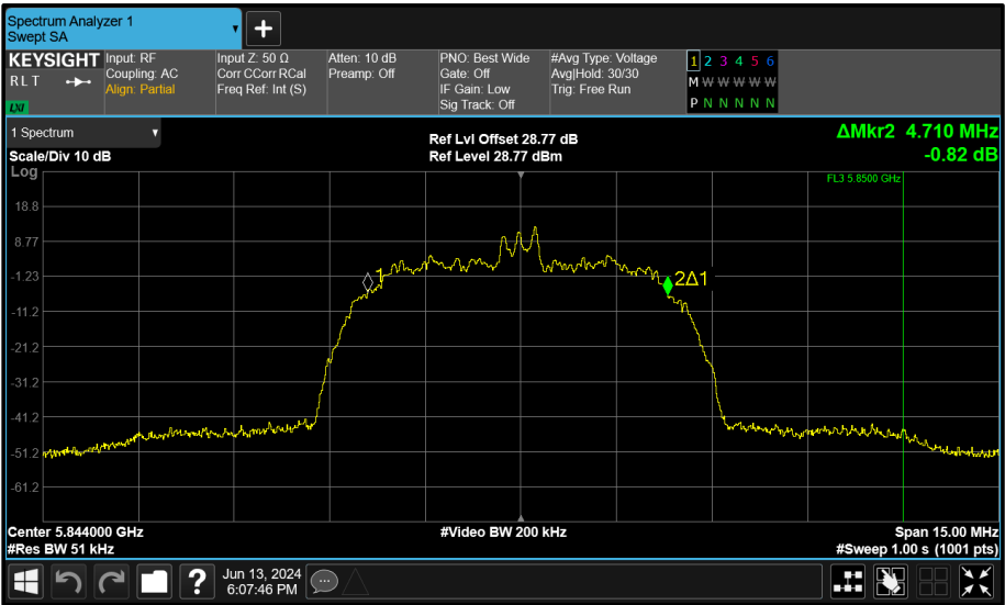
Figure 74 - Core 0 (A) 5844 MHz (CH119) 99% Bandwidth
