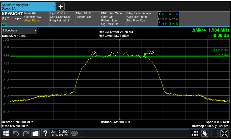
Figure 67 - Core 0 (A) 5789 MHz (CH64) 6 dB Bandwidth
