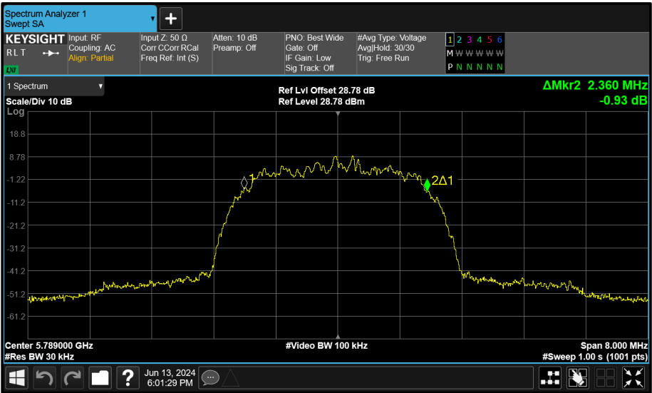
Figure 66 - Core 0 (A) 5789 MHz (CH64) 99% Bandwidth
