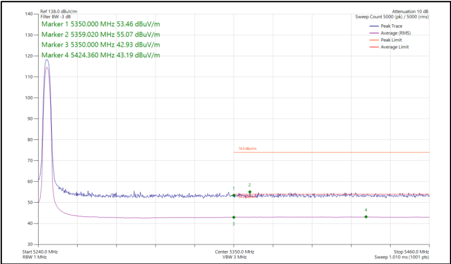
Figure 25 - Bluetooth HDR4, SISO, Core 1 - 5245 MHz Band Edge Frequency 5350 MHz
