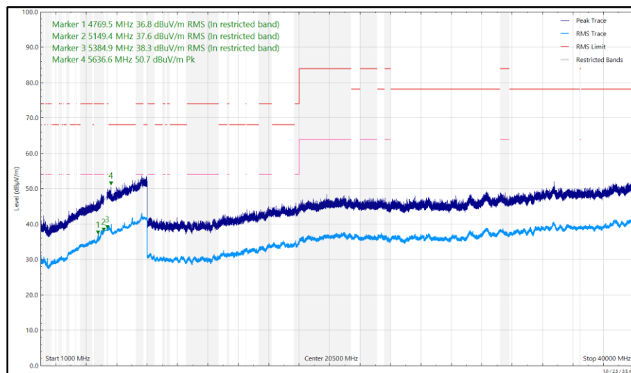
Figure 245 - 5203 MHz, HDR4, ePA, Core 0 + Core 1, 1 GHz to 40 GHz, Horizontal
