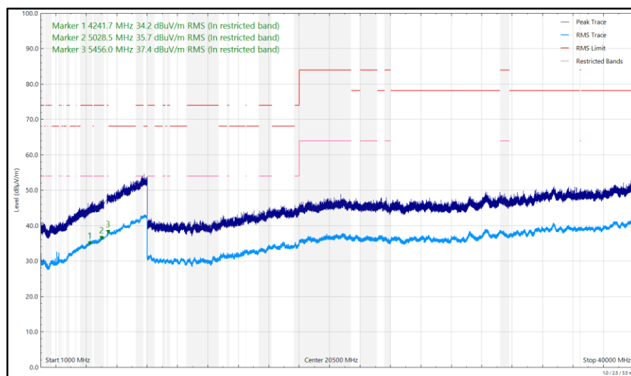
Figure 232 - 5245 MHz, DH5, iPA, Core 0 + Core 1, 1 GHz to 40 GHz, Horizontal
