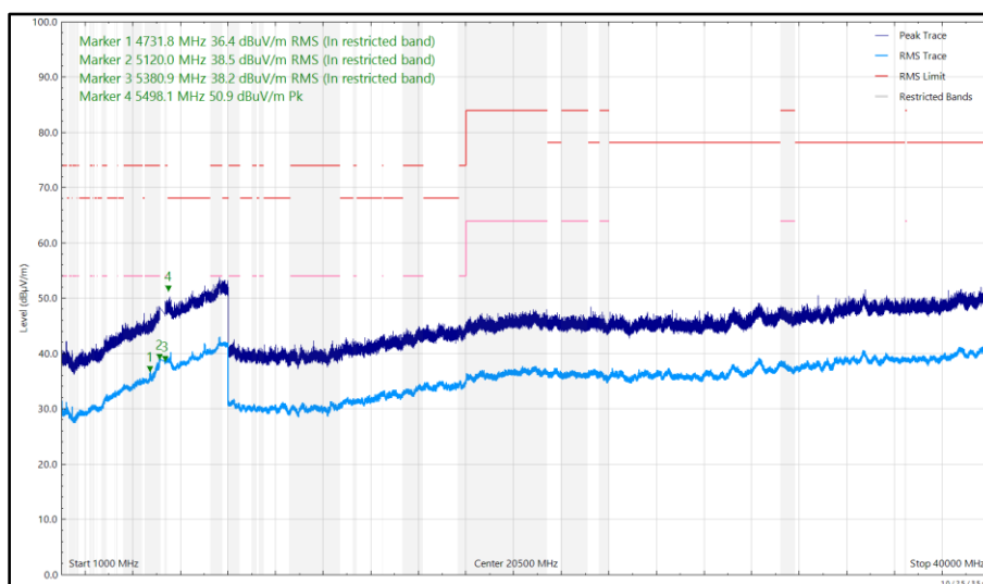
Figure 242 - 5162 MHz, HDR4, ePA, Core 0 + Core 1, 1 GHz to 40 GHz, Horizontal
