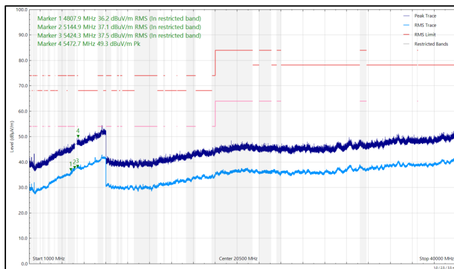
Figure 249 - 5245 MHz, HDR4, ePA, Core 0 + Core 1, 1 GHz to 40 GHz, Vertical
