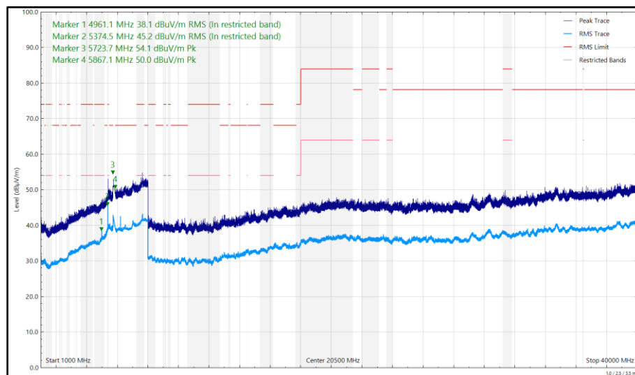
Figure 253 - 5788 MHz, HDR4, ePA, Core 0 + Core 1, 1 GHz to 40 GHz, Horizontal
