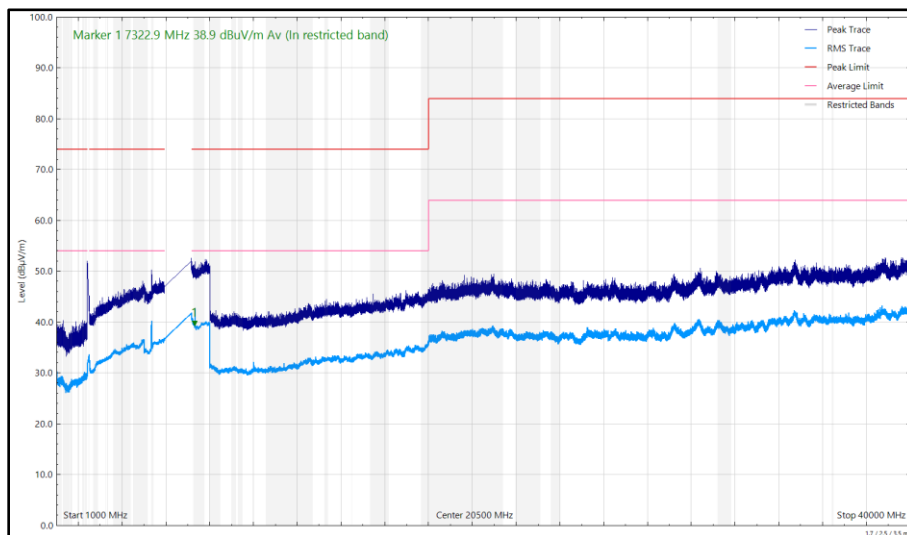
Figure 33 - U-NII-8 - 6995 MHz (CH209), HE20, SU, CDD, Core 0 + Core 1 and 2441 MHz
