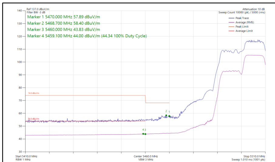
Figure 22 - 802.11ax HE20, RU 106-54, SISO, Core 0 - 5500 MHz Band Edge Frequency 5460 MHz
