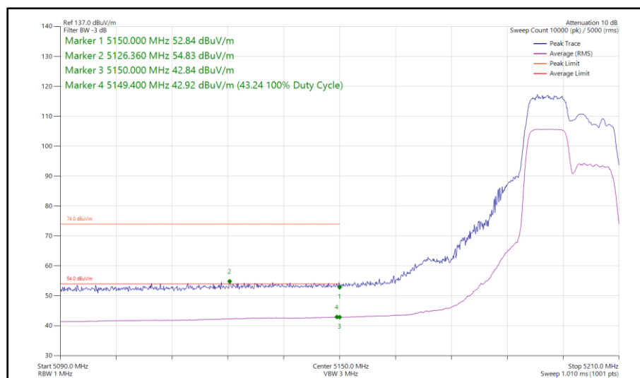
Figure 32 - 802.11ax HE20, RU 106-53, SISO, Core 1 - 5200 MHz Band Edge Frequency 5150 MHz
