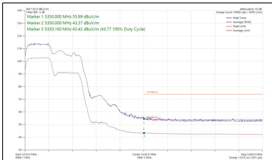
Figure 40 - 802.11ax HE20, RU 106-53, SISO, Core 1 - 5320 MHz Band Edge Frequency 5350 MHz
