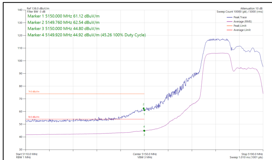
Figure 52 - 802.11ax HE20, RU 106-53, CDD, Core 0 - Core 1 - 5180 MHz Band Edge Frequency 5150 MHz
