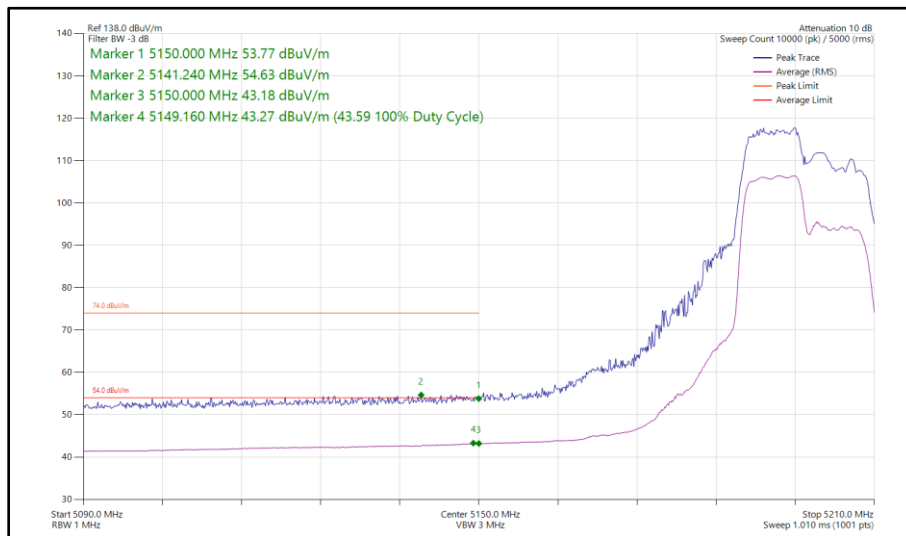
Figure 54 - 802.11ax HE20, RU 106-53, CDD, Core 0 - Core 1 - 5200 MHz Band Edge Frequency 5150 MHz
