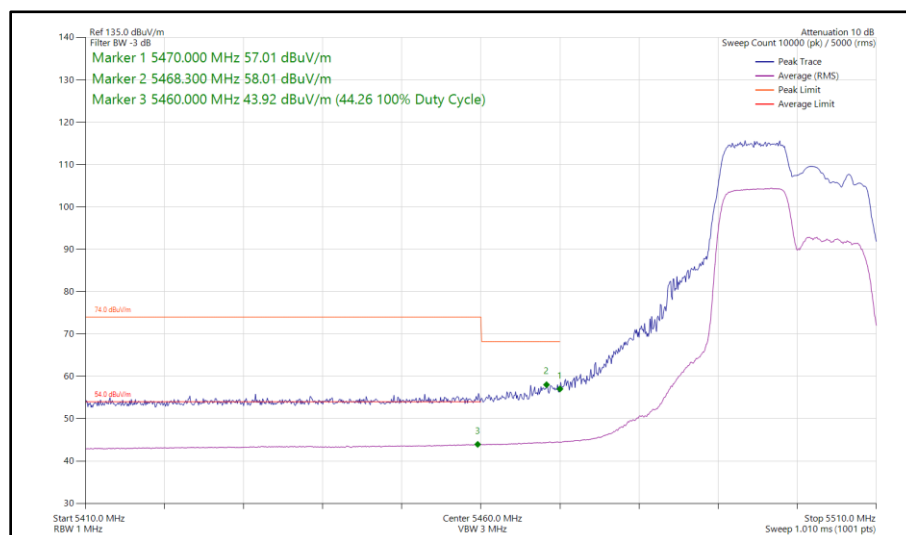
Figure 46 - 802.11ax HE20, RU 106-53, SISO, Core 1 - 5500 MHz Band Edge Frequency 5460 MHz
