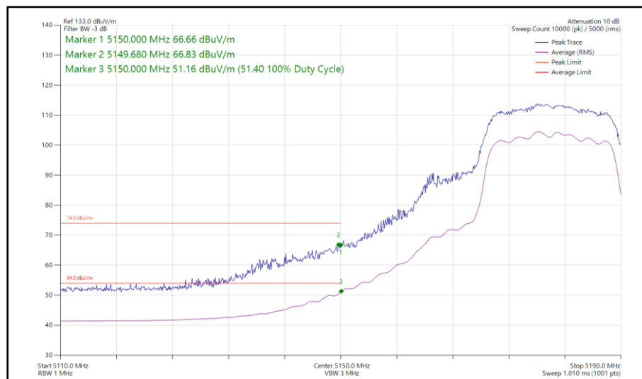
Figure 49 - 802.11n HT20, CDD, Core 0 - Core 1 - 5180 MHz Band Edge Frequency 5150 MHz
