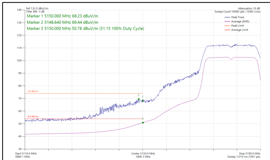
Figure 27 - 802.11n HT20, SISO, Core 1 - 5180 MHz Band Edge Frequency 5150 MHz
