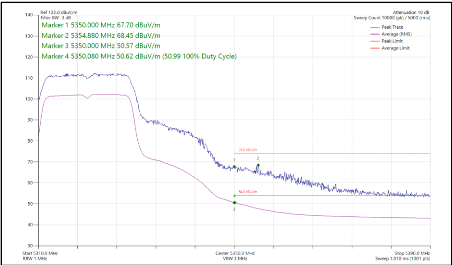
Figure 36 - 802.11n HT20, SISO, Core 1 - 5320 MHz Band Edge Frequency 5350 MHz
