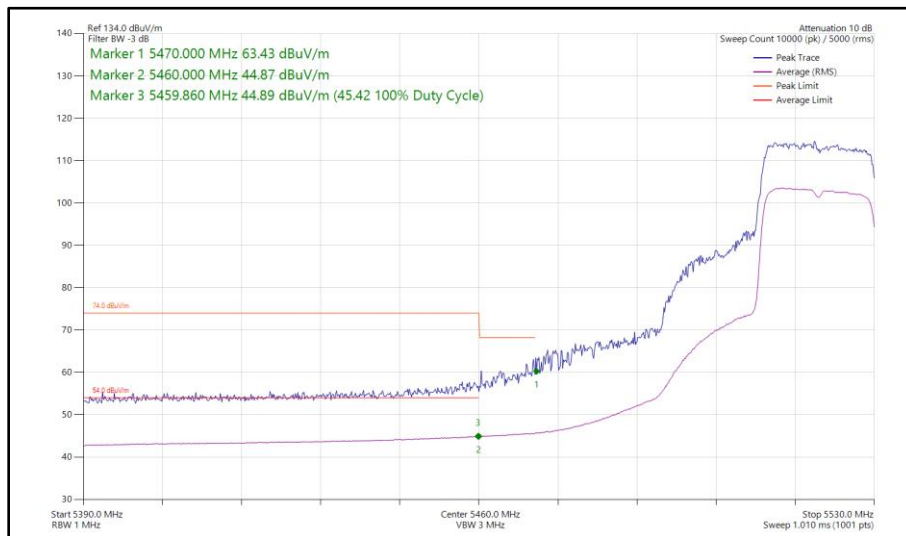
Figure 23 - 802.11ax HE20, SU, SISO, Core 0 - 5520 MHz Band Edge Frequency 5460 MHz
