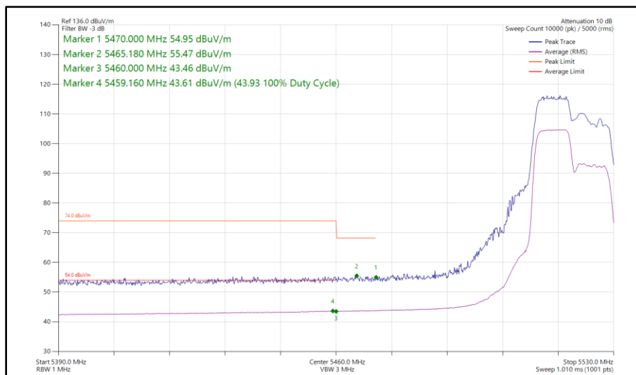
Figure 24 - 802.11ax HE20, RU 106-53, SISO, Core 0 - 5520 MHz Band Edge Frequency 5460 MHz
