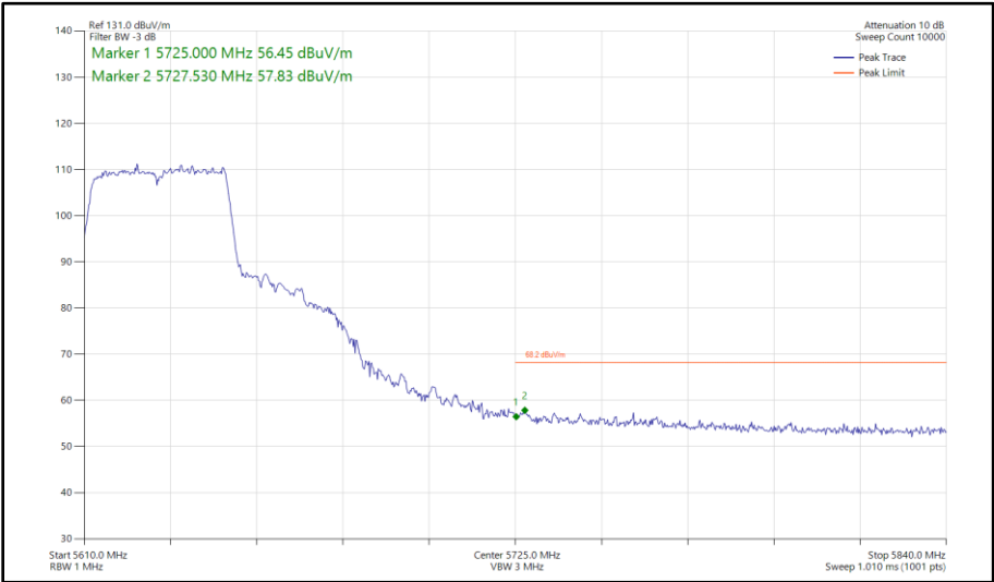
Figure 587 - 802.11n HT40, SDM, Core 0 - Core 1 - 5630 MHz Band Edge Frequency 5725 MHz
