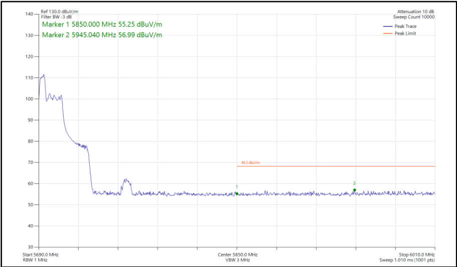
Figure 575 - 802.11ax HE40, RU 52-37, CDD, Core 0 - Core 1 - 5710 MHz Band Edge Frequency 5850 MHz
