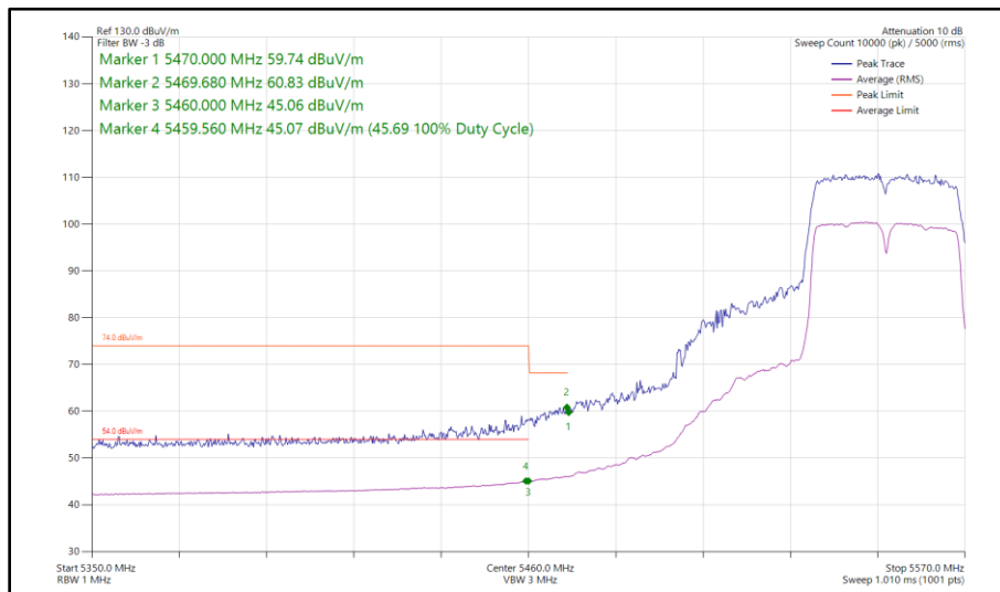
Figure 517 - 802.11n HT40, SISO, Core 0 - 5550 MHz Band Edge Frequency 5470 MHz
