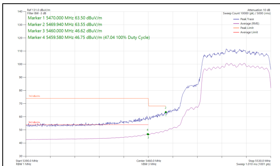
Figure 560 - 802.11ax HE40, SU, CDD, Core 0 - Core 1 - 5510 MHz Band Edge Frequency 5470 MHz
