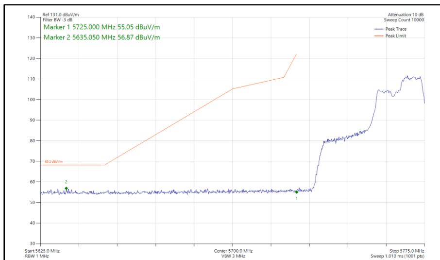
Figure 586 - 802.11ax HE40, RU 106-56, SDM, Core 0 - Core 1 - 5755 MHz Band Edge Frequency 5725 MHz
