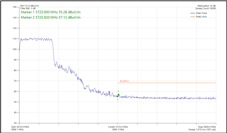
Figure 569 - 802.11ax HE40, SU, CDD, Core 0 - Core 1 - 5630 MHz Band Edge Frequency 5725 MHz
