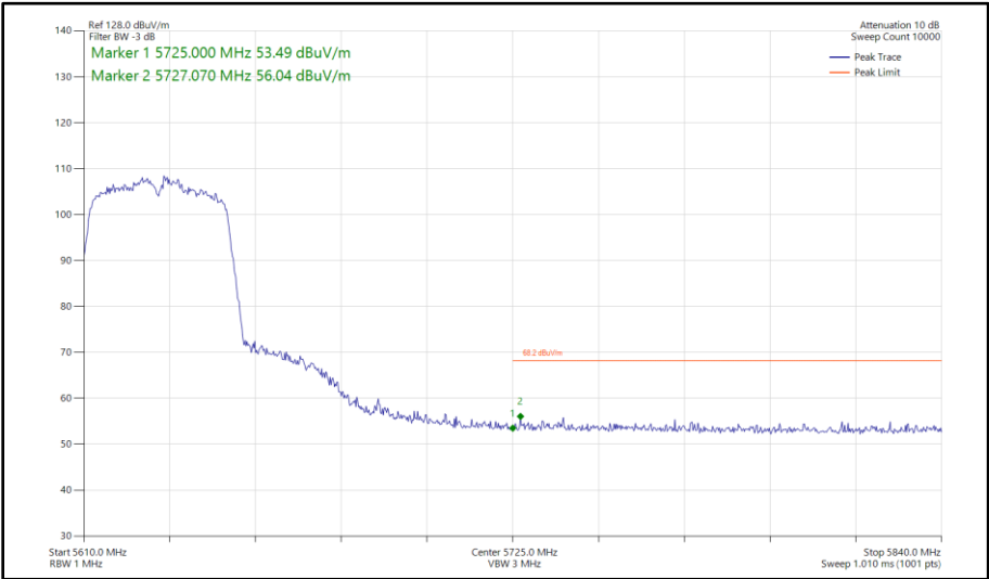
Figure 525 - 802.11n HT40, SISO, Core 0 - 5630 MHz Band Edge Frequency 5725 MHz
