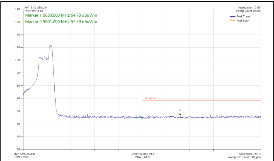
Figure 555 - 802.11ax HE40, RU 52-44, SISO, Core 1 - 5710 MHz Band Edge Frequency 5850 MHz
