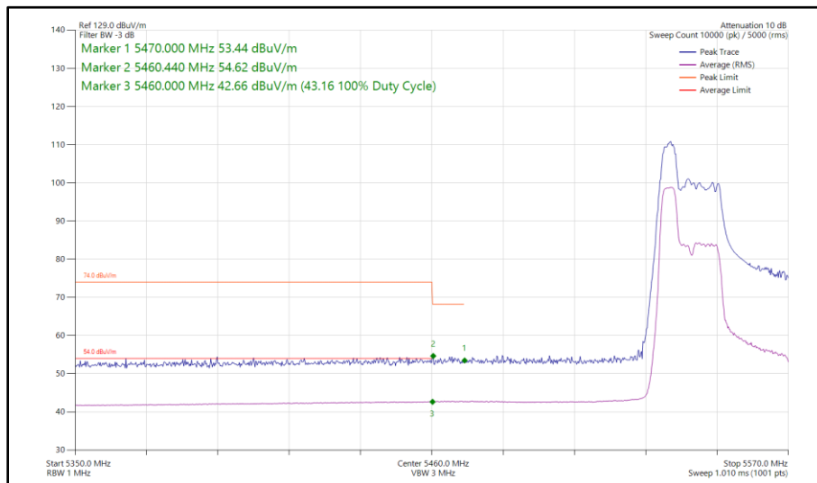
Figure 542 - 802.11ax HE40, RU 52-37, SISO, Core 1 - 5550 MHz Band Edge Frequency 5470 MHz
