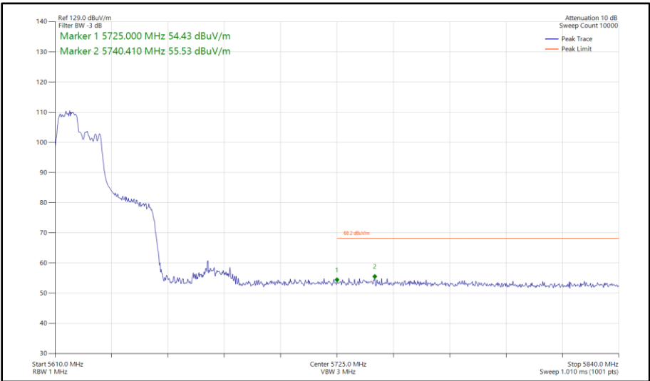
Figure 590 - 802.11ax HE40, RU 106-53, SDM, Core 0 - Core 1 - 5630 MHz Band Edge Frequency 5725 MHz
