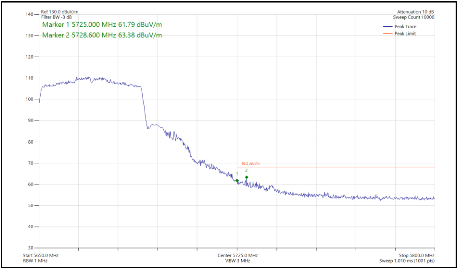
Figure 529 - 802.11ax HE40, SU, SISO, Core 0 - 5670 MHz Band Edge Frequency 5725 MHz
