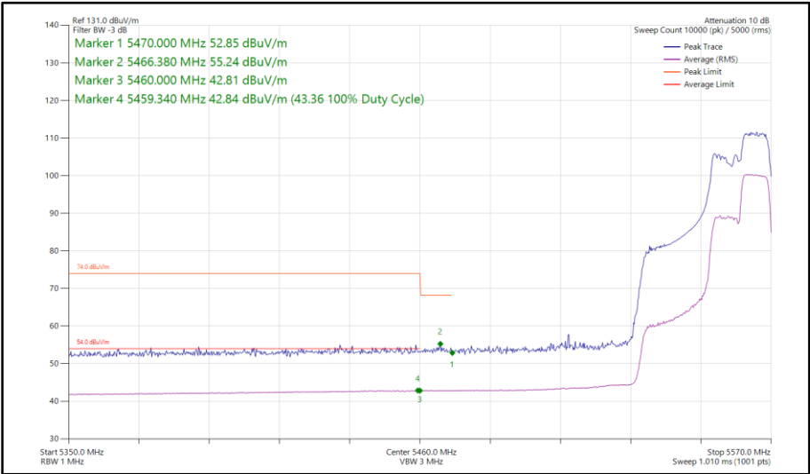
Figure 521 - 802.11ax HE40, RU 106-56, SISO, Core 0 - 5550 MHz Band Edge Frequency 5470 MHz
