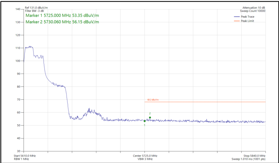
Figure 549 - 802.11ax HE40, RU 106-53, SISO, Core 1 - 5630 MHz Band Edge Frequency 5725 MHz
