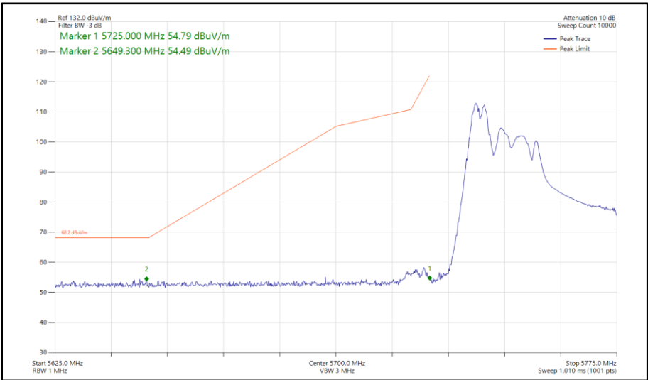
Figure 566 - 802.11ax HE40, RU 52-37, CDD, Core 0 - Core 1 - 5755 MHz Band Edge Frequency 5725 MHz
