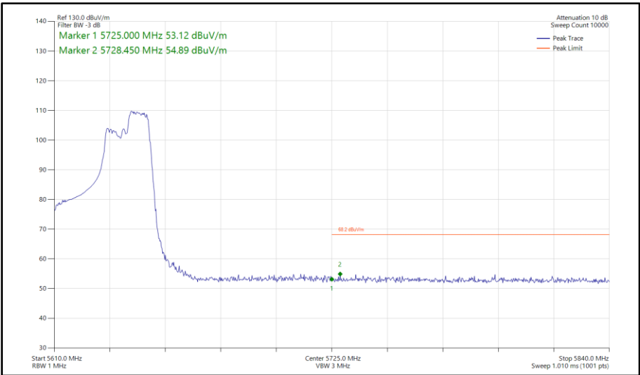
Figure 528 - 802.11ax HE40, RU 106-56, SISO, Core 0 - 5630 MHz Band Edge Frequency 5725 MHz
