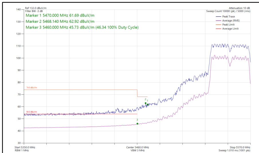
Figure 559 - 802.11n HT40, CDD, Core 0 - Core 1 - 5550 MHz Band Edge Frequency 5470 MHz
