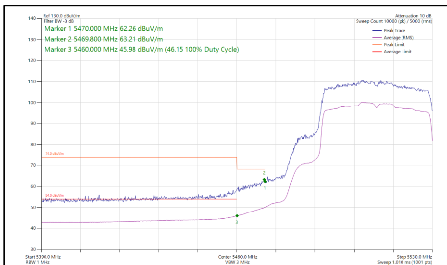
Figure 539 - 802.11ax HE40, SU, SISO, Core 1 - 5510 MHz Band Edge Frequency 5470 MHz
