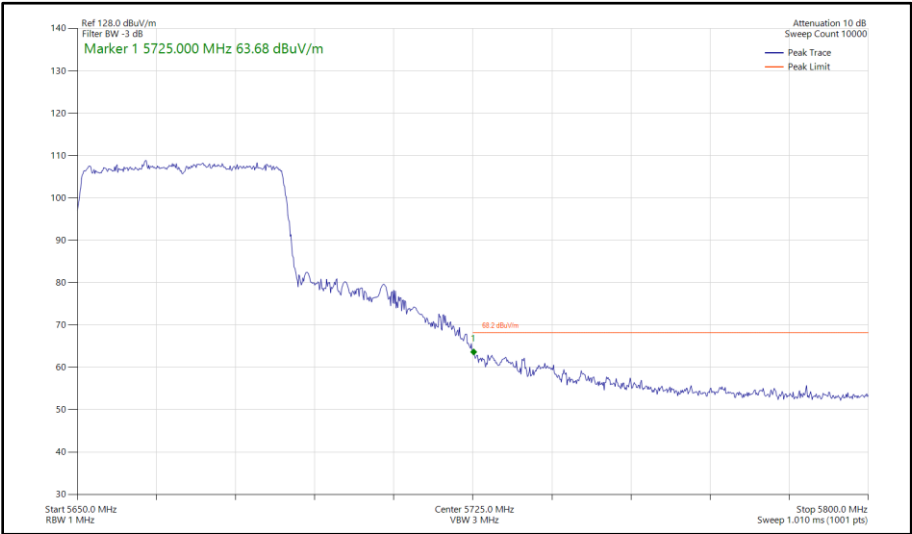
Figure 550 - 802.11ax HE40, SU, SISO, Core 1 - 5670 MHz Band Edge Frequency 5725 MHz
