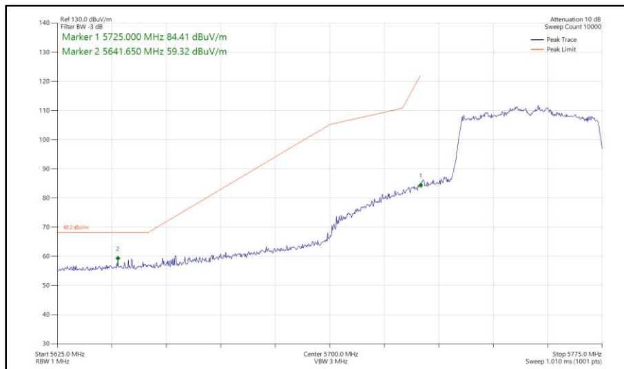
Figure 585 - 802.11ax HE40, SU, SDM, Core 0 - Core 1 - 5755 MHz Band Edge Frequency 5725 MHz
