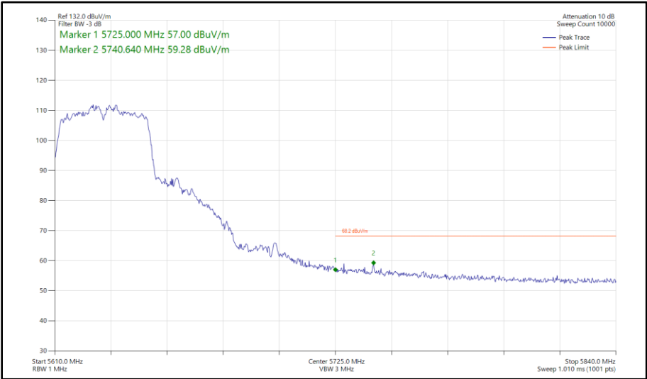
Figure 567 - 802.11n HT40, CDD, Core 0 - Core 1 - 5630 MHz Band Edge Frequency 5725 MHz
