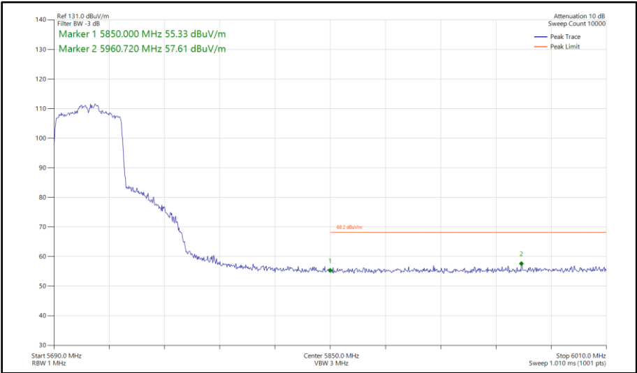
Figure 533 - 802.11ax HE40, SU, SISO, Core 0 - 5710 MHz Band Edge Frequency 5850 MHz
