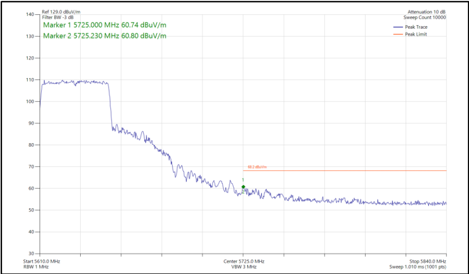
Figure 548 - 802.11ax HE40, SU, SISO, Core 1 - 5630 MHz Band Edge Frequency 5725 MHz
