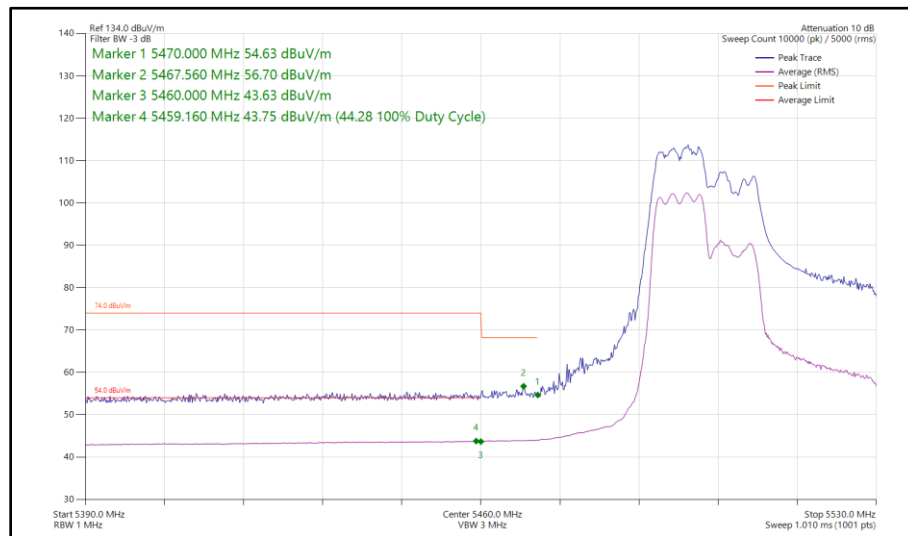
Figure 561 - 802.11ax HE40, RU 106-53, CDD, Core 0 - Core 1 - 5510 MHz Band Edge Frequency 5470 MHz
