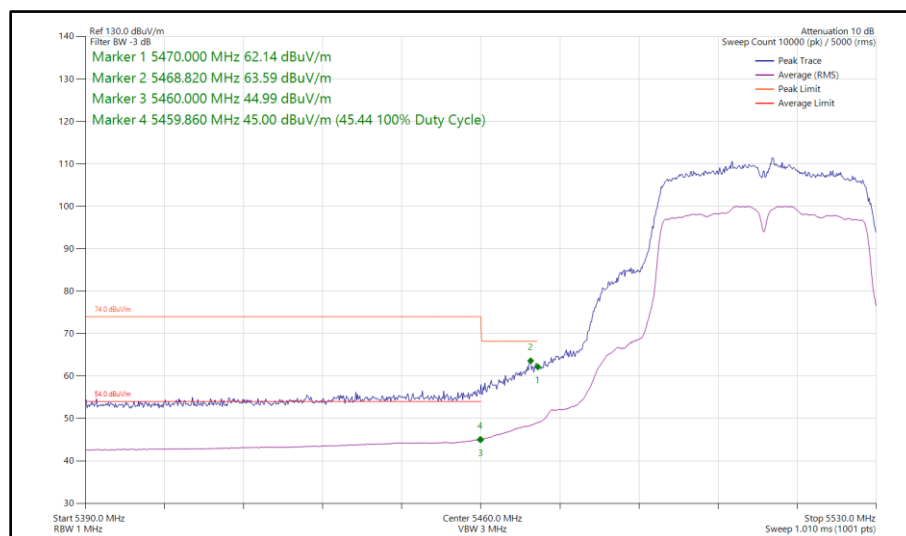
Figure 516 - 802.11n HT40, SISO, Core 0 - 5510 MHz Band Edge Frequency 5470 MHz
