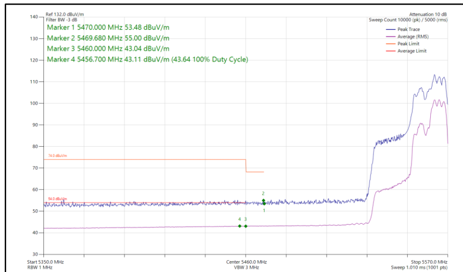
Figure 563 - 802.11ax HE40, RU 106-56, CDD, Core 0 - Core 1 - 5550 MHz Band Edge Frequency 5470 MHz
