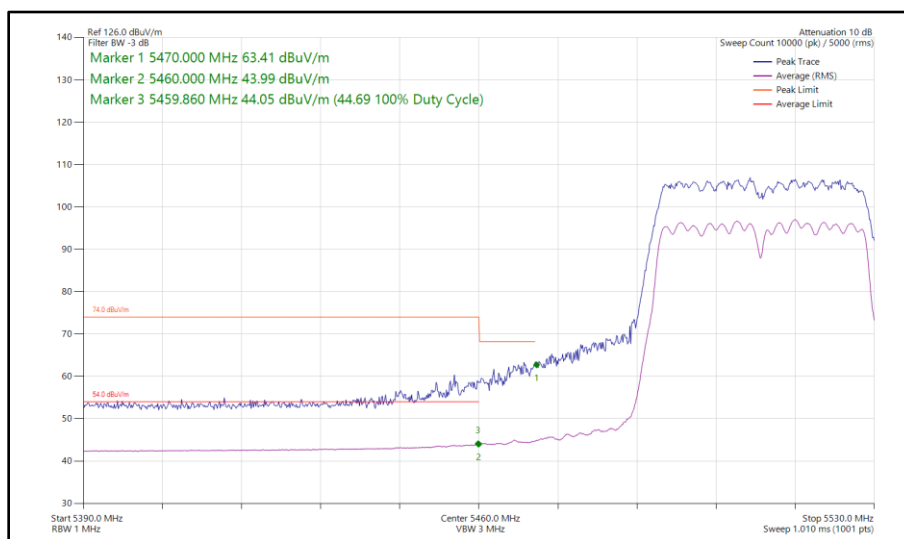
Figure 558 - 802.11n HT40, CDD, Core 0 - Core 1 - 5510 MHz Band Edge Frequency 5470 MHz
