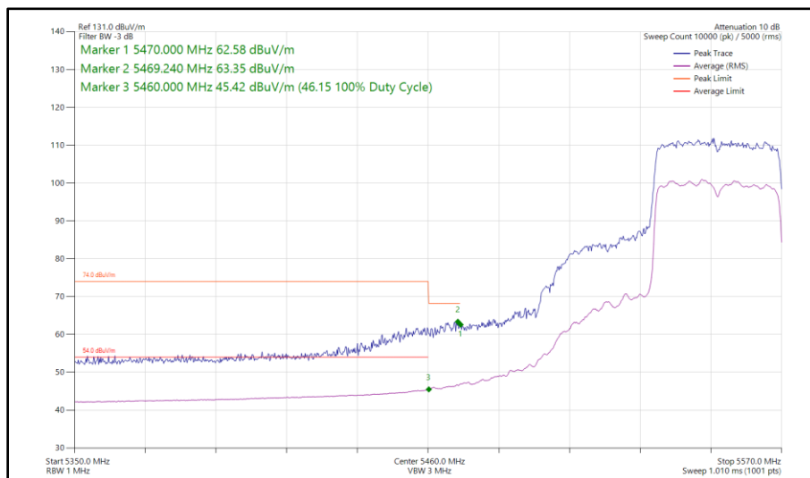
Figure 582 - 802.11ax HE40, SU, SDM, Core 0 - Core 1 - 5550 MHz Band Edge Frequency 5470 MHz
