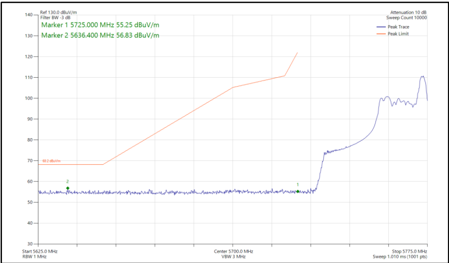
Figure 545 - 802.11ax HE40, RU 26-17, SISO, Core 1 - 5755 MHz Band Edge Frequency 5725 MHz
