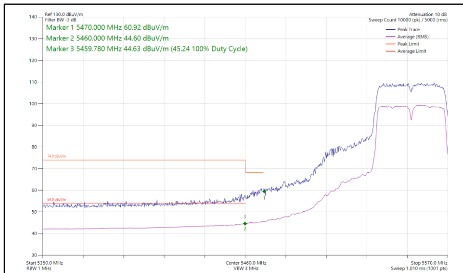
Figure 538 - 802.11n HT40, SISO, Core 1 - 5550 MHz Band Edge Frequency 5470 MHz
