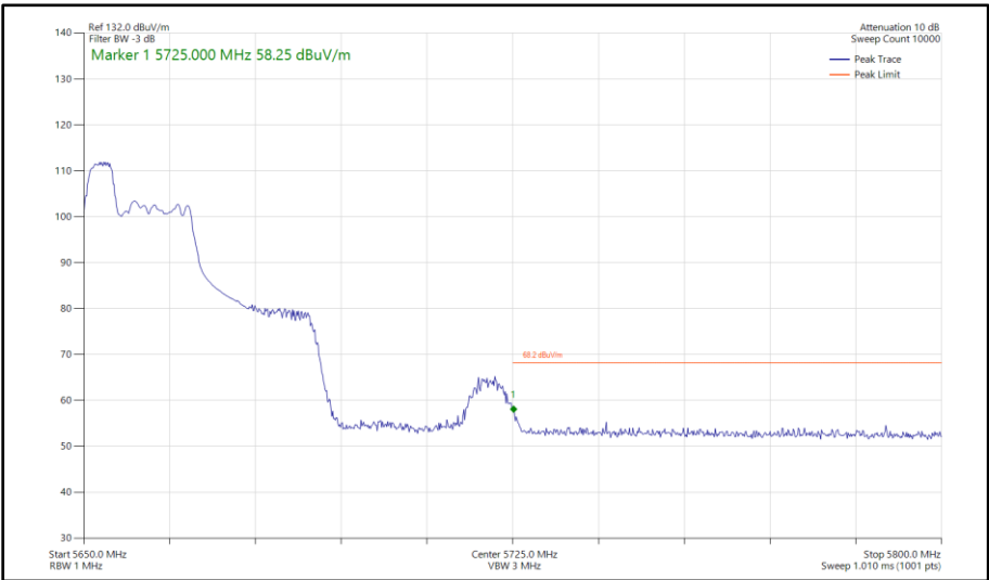
Figure 551 - 802.11ax HE40, RU 52-37, SISO, Core 1 - 5670 MHz Band Edge Frequency 5725 MHz
