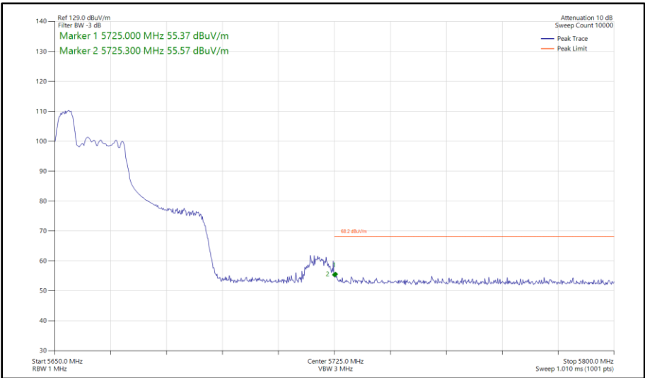
Figure 530 - 802.11ax HE40, RU 52-37, SISO, Core 0 - 5670 MHz Band Edge Frequency 5725 MHz
