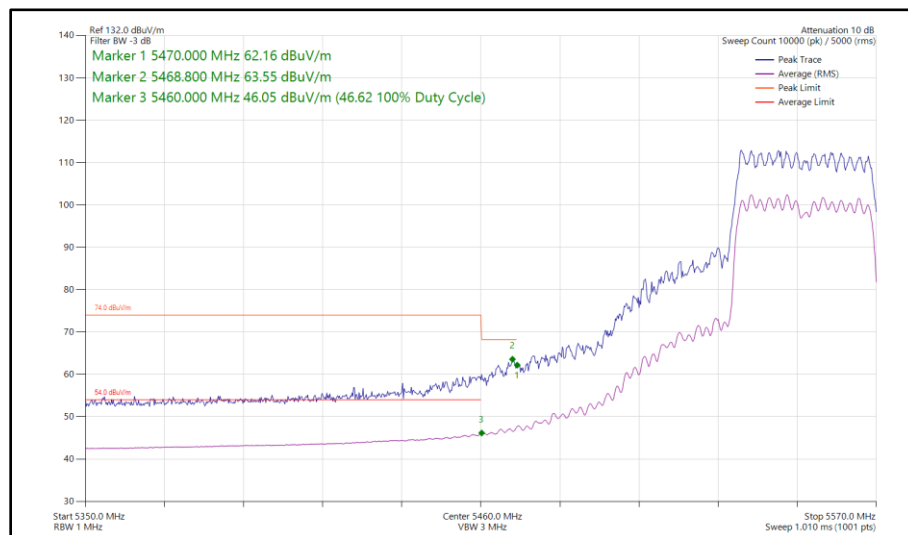
Figure 562 - 802.11ax HE40, SU, CDD, Core 0 - Core 1 - 5550 MHz Band Edge Frequency 5470 MHz
