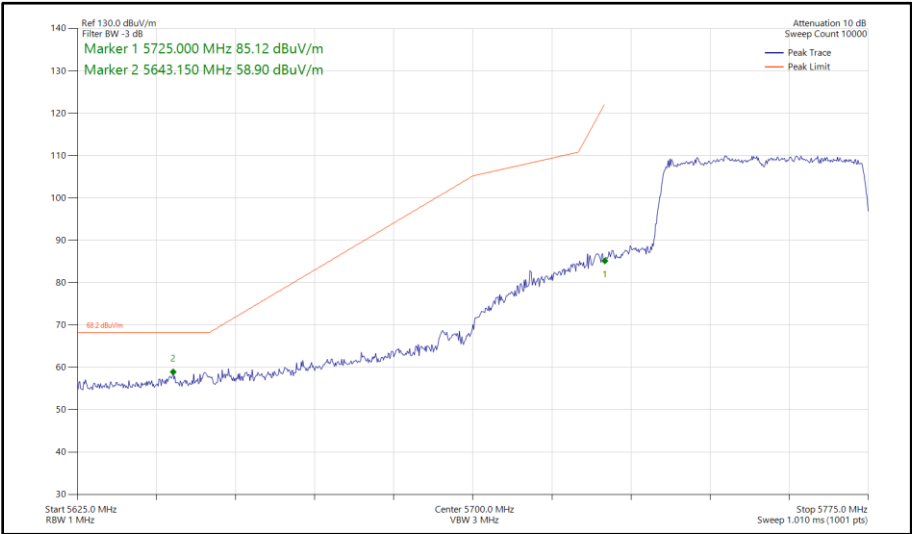
Figure 523 - 802.11ax HE40, SU, SISO, Core 0 - 5755 MHz Band Edge Frequency 5725 MHz
