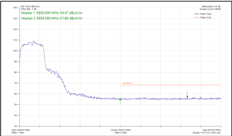
Figure 572 - 802.11n HT40, CDD, Core 0 - Core 1 - 5710 MHz Band Edge Frequency 5850 MHz
