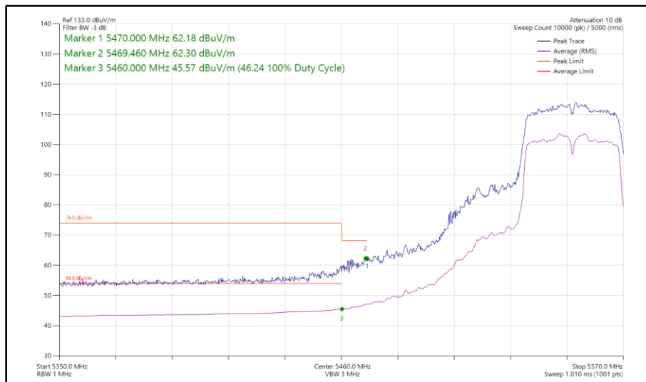
Figure 579 - 802.11n HT40, SDM, Core 0 - Core 1 - 5550 MHz Band Edge Frequency 5470 MHz
