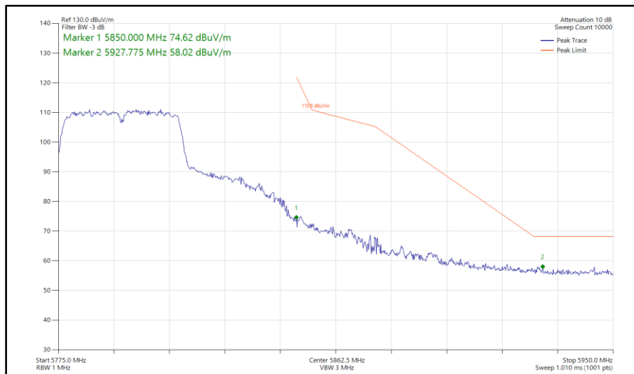
Figure 573 - 802.11n HT40, CDD, Core 0 - Core 1 - 5795 MHz Band Edge Frequency 5850 MHz
