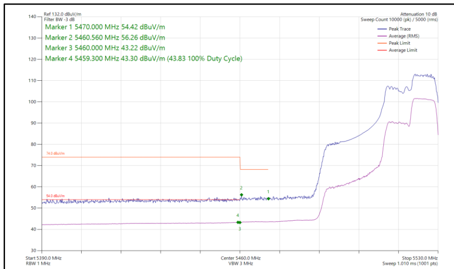
Figure 519 - 802.11ax HE40, RU 106-56, SISO, Core 0 - 5510 MHz Band Edge Frequency 5470 MHz
