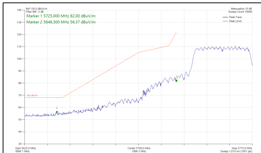
Figure 564 - 802.11n HT40, CDD, Core 0 - Core 1 - 5755 MHz Band Edge Frequency 5725 MHz
