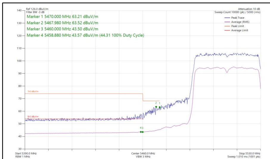
Figure 580 - 802.11ax HE40, SU, SDM, Core 0 - Core 1 - 5510 MHz Band Edge Frequency 5470 MHz
