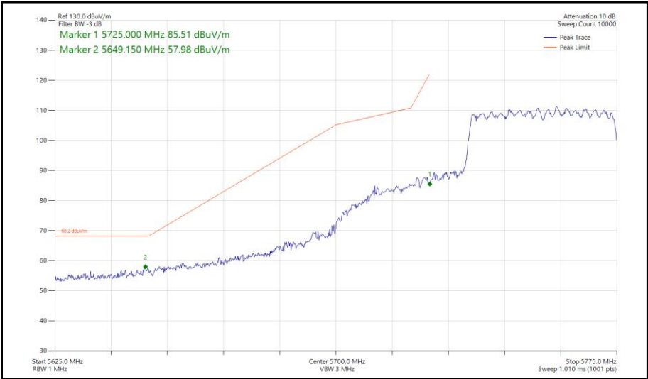
Figure 565 - 802.11ax HE40, SU, CDD, Core 0 - Core 1 - 5755 MHz Band Edge Frequency 5725 MHz
