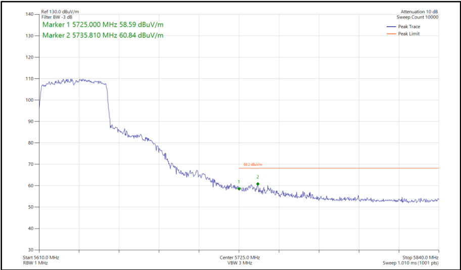
Figure 589 - 802.11ax HE40, SU, SDM, Core 0 - Core 1 - 5630 MHz Band Edge Frequency 5725 MHz
