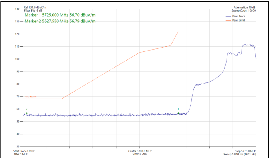
Figure 524 - 802.11ax HE40, RU 106-56, SISO, Core 0 - 5755 MHz Band Edge Frequency 5725 MHz
