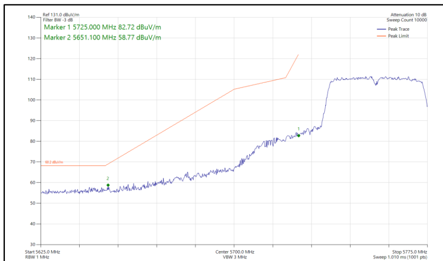
Figure 543 - 802.11n HT40, SISO, Core 1 - 5755 MHz Band Edge Frequency 5725 MHz
