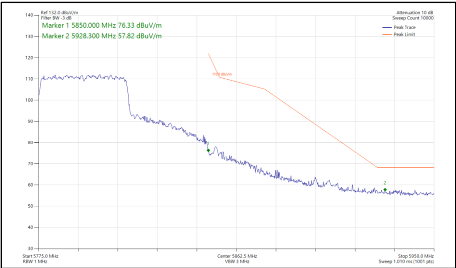
Figure 576 - 802.11ax HE40, SU, CDD, Core 0 - Core 1 - 5795 MHz Band Edge Frequency 5850 MHz
