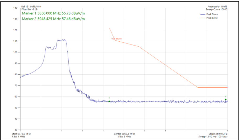
Figure 536 - 802.11ax HE40, RU 106-56, SISO, Core 0 - 5795 MHz Band Edge Frequency 5850 MHz
