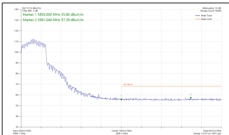
Figure 574 - 802.11ax HE40, SU, CDD, Core 0 - Core 1 - 5710 MHz Band Edge Frequency 5850 MHz
