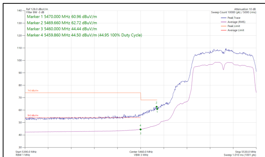
Figure 537 - 802.11n HT40, SISO, Core 1 - 5510 MHz Band Edge Frequency 5470 MHz
