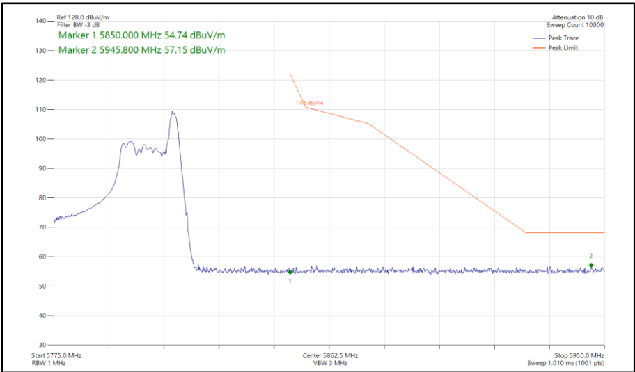
Figure 557 - 802.11ax HE40, RU 26-17, SISO, Core 1 - 5795 MHz Band Edge Frequency 5850 MHz
