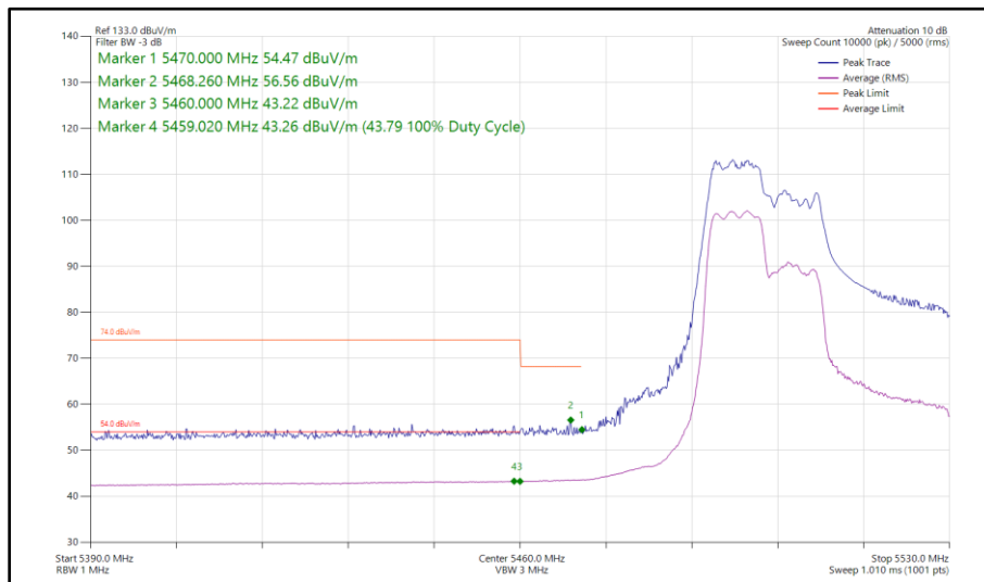
Figure 581 - 802.11ax HE40, RU 106-53, SDM, Core 0 - Core 1 - 5510 MHz Band Edge Frequency 5470 MHz
