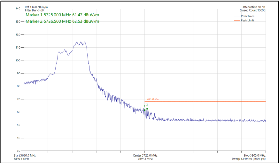
Figure 571 - 802.11ax HE40, RU 106-56, CDD, Core 0 - Core 1 - 5670 MHz Band Edge Frequency 5725 MHz
