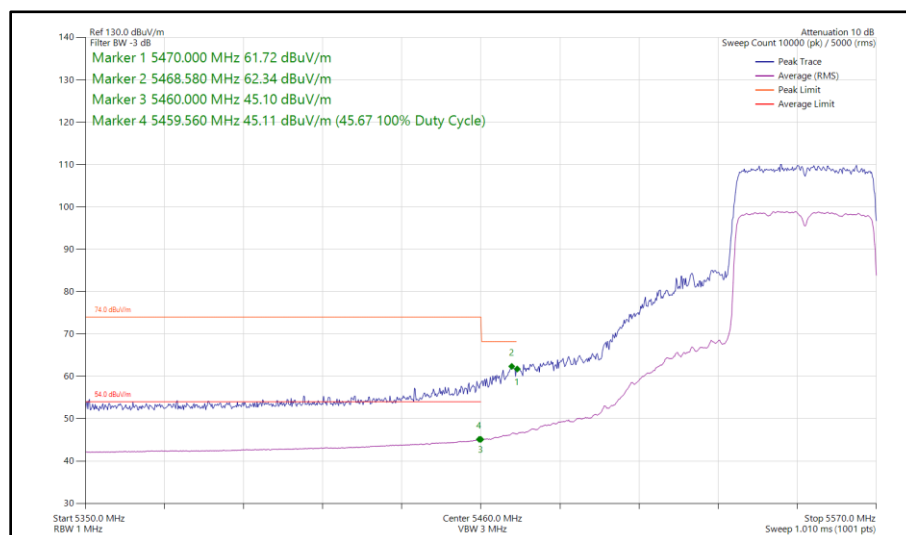
Figure 541 - 802.11ax HE40, SU, SISO, Core 1 - 5550 MHz Band Edge Frequency 5470 MHz
