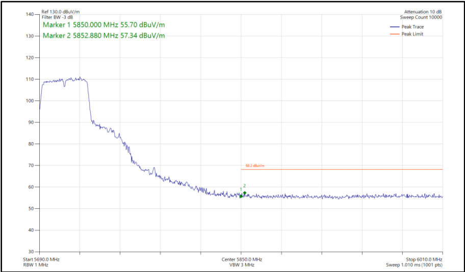
Figure 552 - 802.11n HT40, SISO, Core 1 - 5710 MHz Band Edge Frequency 5850 MHz
