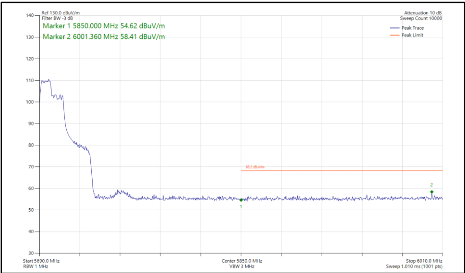
Figure 534 - 802.11ax HE40, RU 106-53, SISO, Core 0 - 5710 MHz Band Edge Frequency 5850 MHz
