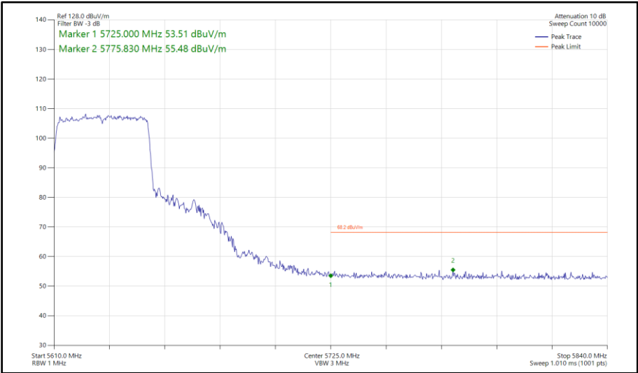
Figure 527 - 802.11ax HE40, SU, SISO, Core 0 - 5630 MHz Band Edge Frequency 5725 MHz
