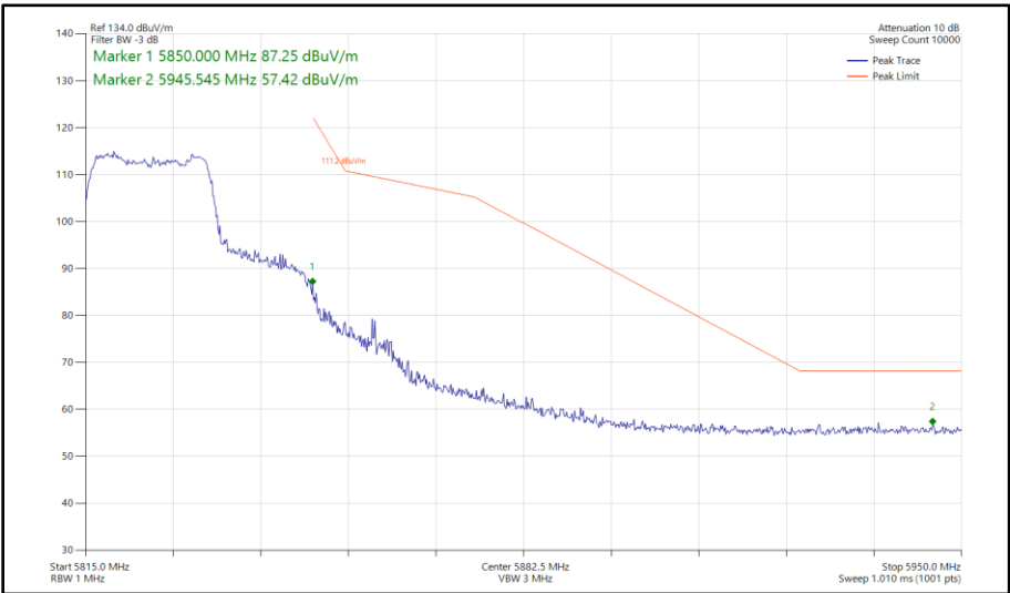
Figure 515 - 802.11ac VHT20, TxBF, Core 0 - Core 1 - 5825 MHz Band Edge Frequency 5850 MHz
