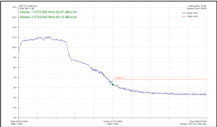
Figure 568 - 802.11n HT40, CDD, Core 0 - Core 1 - 5670 MHz Band Edge Frequency 5725 MHz
