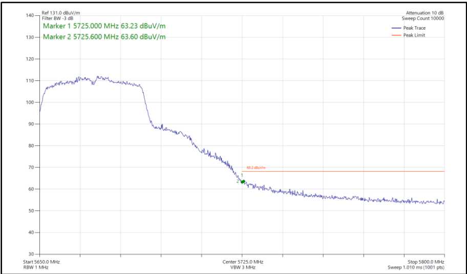
Figure 547 - 802.11n HT40, SISO, Core 1 - 5670 MHz Band Edge Frequency 5725 MHz
