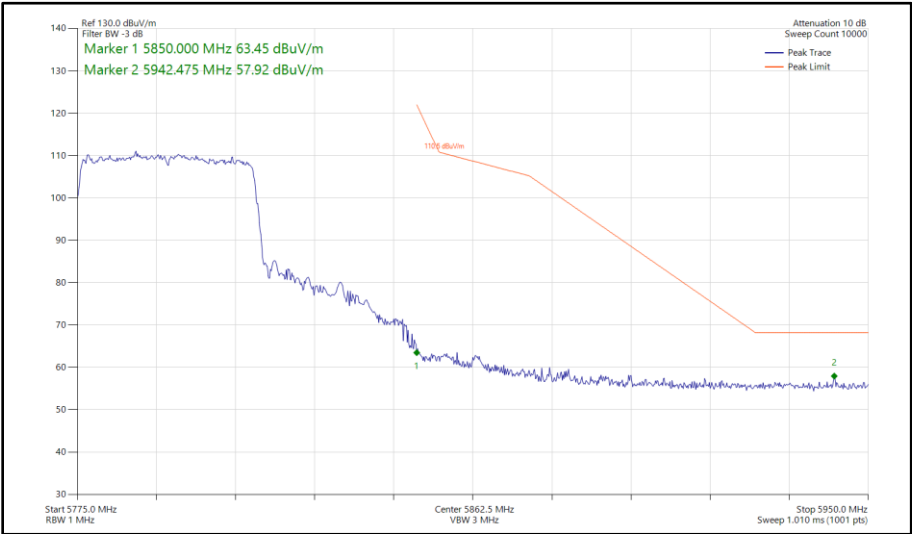
Figure 556 - 802.11ax HE40, SU, SISO, Core 1 - 5795 MHz Band Edge Frequency 5850 MHz
