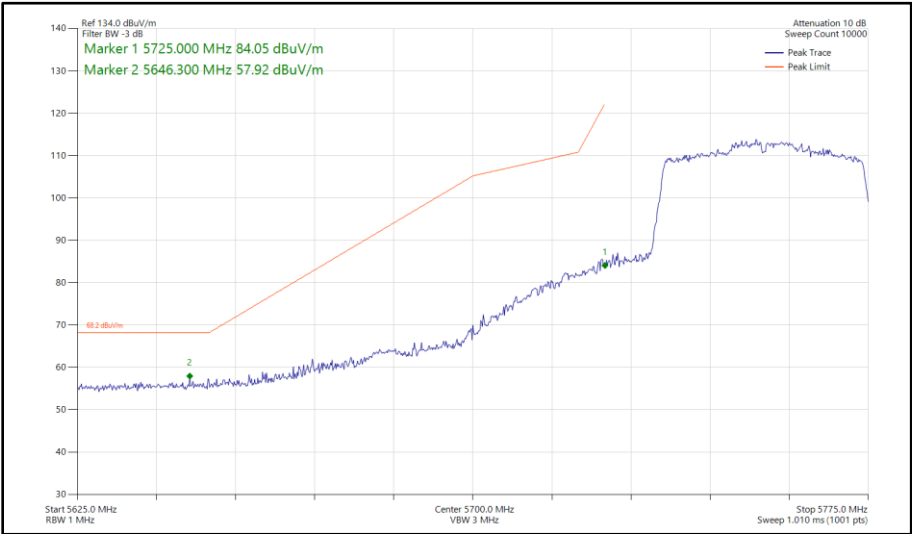
Figure 544 - 802.11ax HE40, SU, SISO, Core 1 - 5755 MHz Band Edge Frequency 5725 MHz
