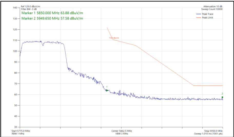
Figure 553 - 802.11n HT40, SISO, Core 1 - 5795 MHz Band Edge Frequency 5850 MHz
