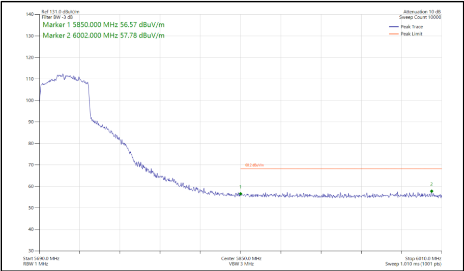
Figure 554 - 802.11ax HE40, SU, SISO, Core 1 - 5710 MHz Band Edge Frequency 5850 MHz
