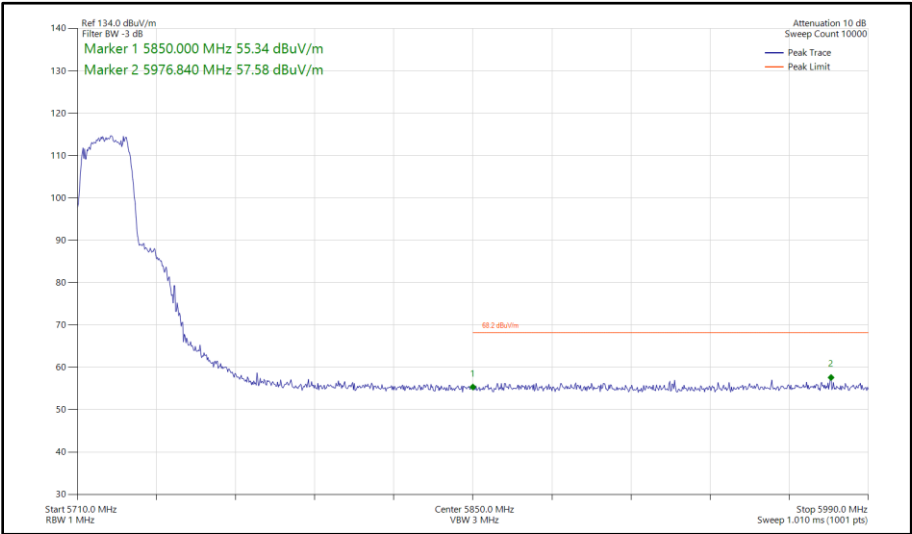
Figure 514 - 802.11ac VHT20, TxBF, Core 0 - Core 1 - 5720 MHz Band Edge Frequency 5850 MHz
