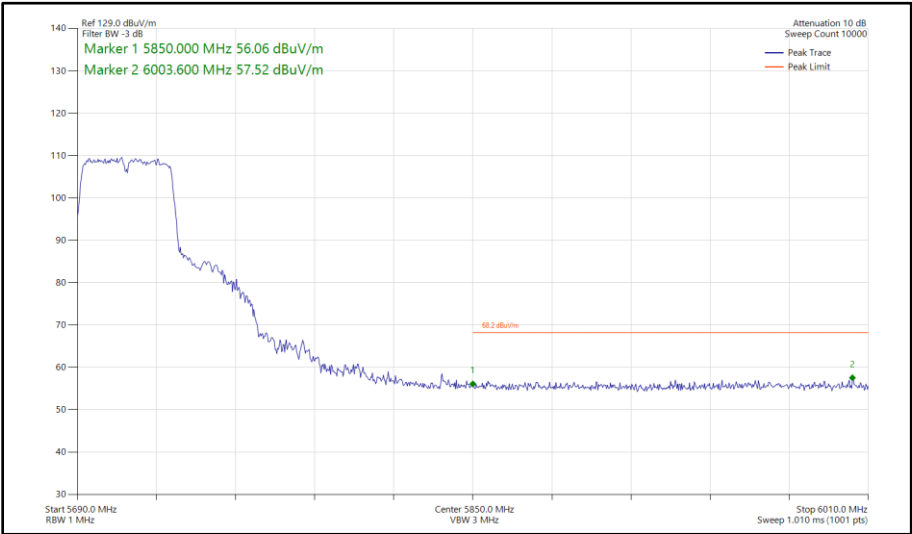
Figure 531 - 802.11n HT40, SISO, Core 0 - 5710 MHz Band Edge Frequency 5850 MHz
