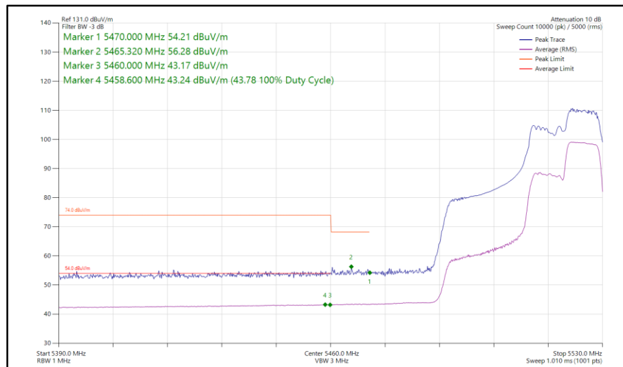
Figure 540 - 802.11ax HE40, RU 106-56, SISO, Core 1 - 5510 MHz Band Edge Frequency 5470 MHz
