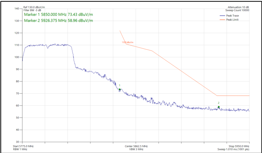
Figure 532 - 802.11n HT40, SISO, Core 0 - 5795 MHz Band Edge Frequency 5850 MHz
