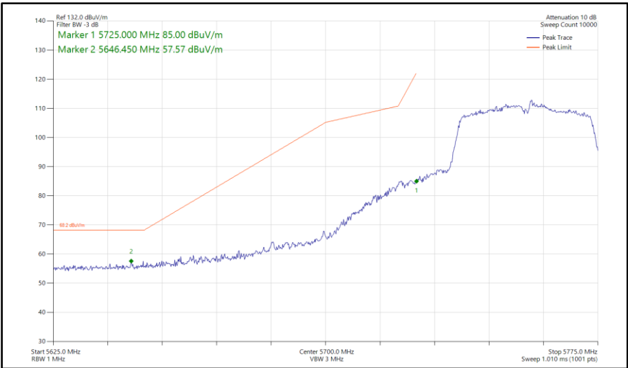
Figure 522 - 802.11n HT40, SISO, Core 0 - 5755 MHz Band Edge Frequency 5725 MHz
