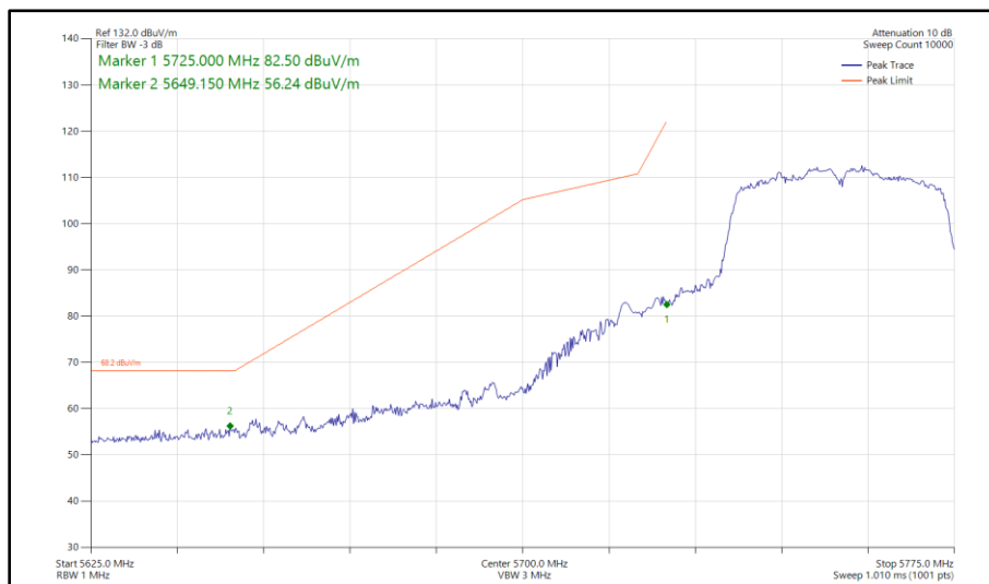
Figure 584 - 802.11n HT40, SDM, Core 0 - Core 1 - 5755 MHz Band Edge Frequency 5725 MHz
