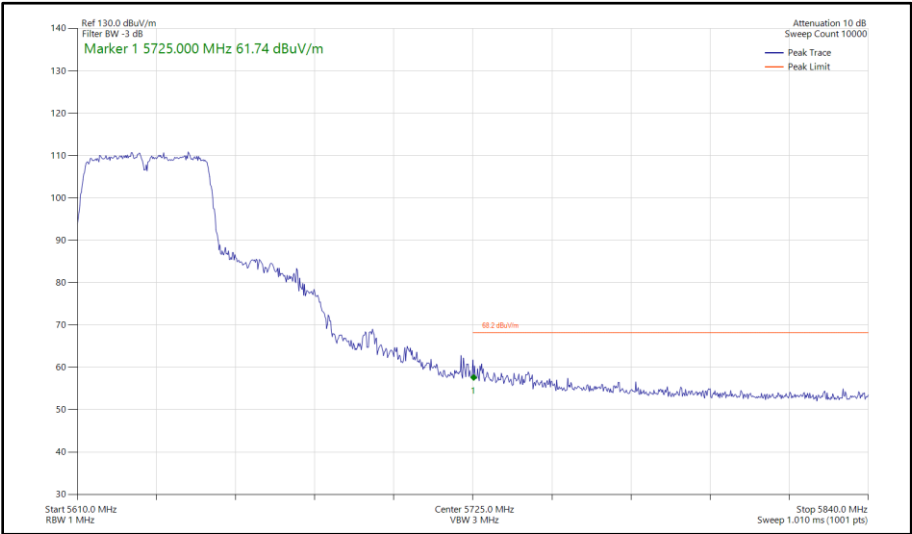
Figure 546 - 802.11n HT40, SISO, Core 1 - 5630 MHz Band Edge Frequency 5725 MHz
