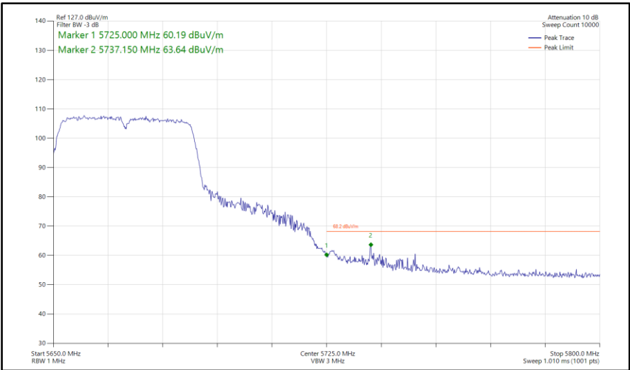
Figure 526 - 802.11n HT40, SISO, Core 0 - 5670 MHz Band Edge Frequency 5725 MHz
