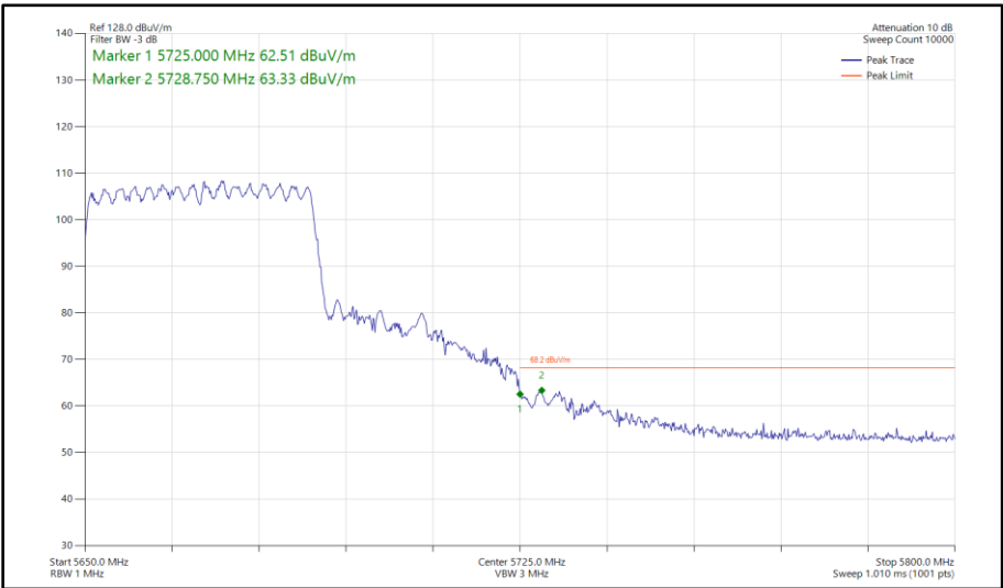
Figure 570 - 802.11ax HE40, SU, CDD, Core 0 - Core 1 - 5670 MHz Band Edge Frequency 5725 MHz
