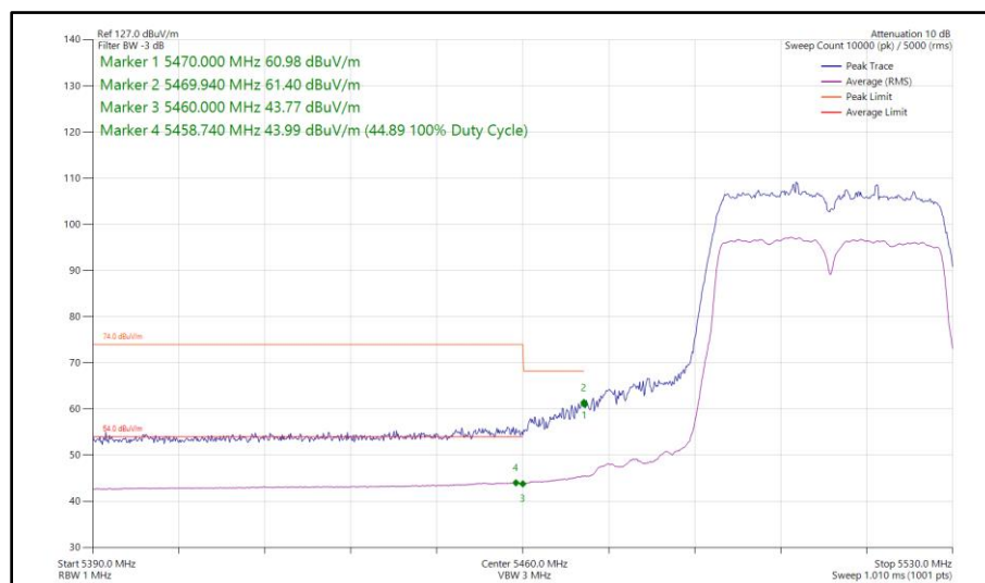
Figure 578 - 802.11n HT40, SDM, Core 0 - Core 1 - 5510 MHz Band Edge Frequency 5470 MHz
