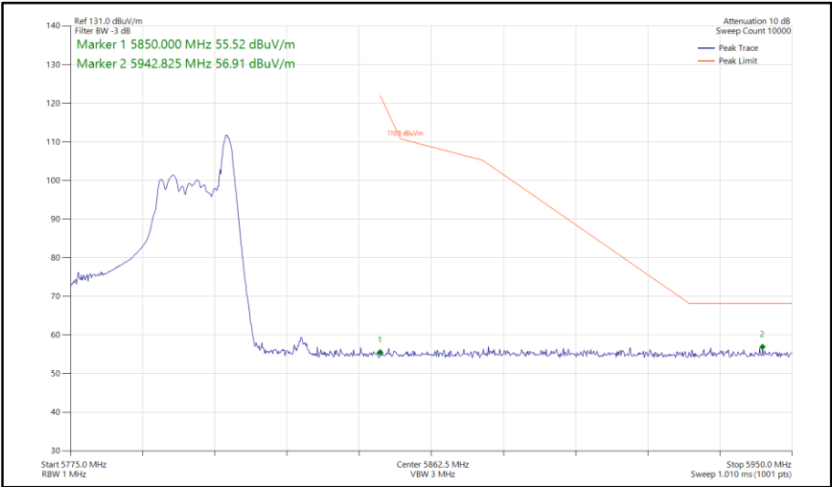
Figure 577 - 802.11ax HE40, RU 26-17, CDD, Core 0 - Core 1 - 5795 MHz Band Edge Frequency 5850 MHz
