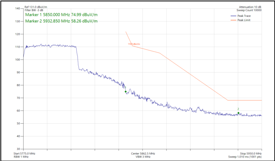
Figure 535 - 802.11ax HE40, SU, SISO, Core 0 - 5795 MHz Band Edge Frequency 5850 MHz
