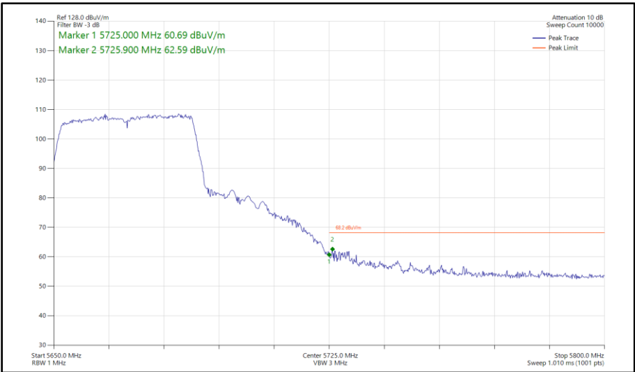
Figure 588 - 802.11n HT40, SDM, Core 0 - Core 1 - 5670 MHz Band Edge Frequency 5725 MHz
