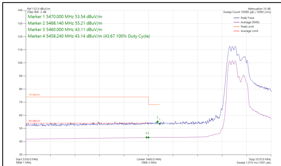
Figure 583 - 802.11ax HE40, RU 106-53, SDM, Core 0 - Core 1 - 5550 MHz Band Edge Frequency 5470 MHz
