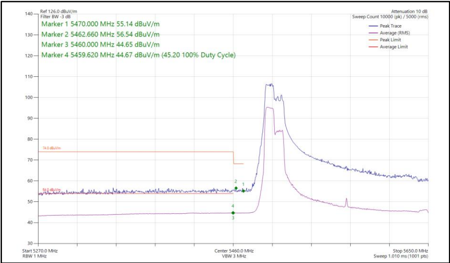
Figure 673 - 802.11ax HE160, RU 106-53P, SISO, Core 0 - 5570 MHz Band Edge Frequency 5470 MHz
