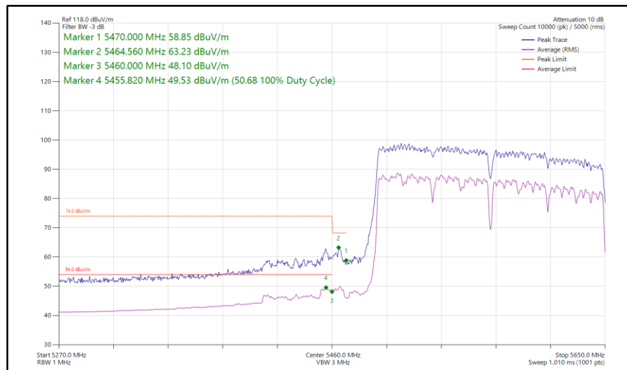
Figure 683 - 802.11ac VHT160, CDD, Core 0 - Core 1 - 5570 MHz Band Edge Frequency 5470 MHz
