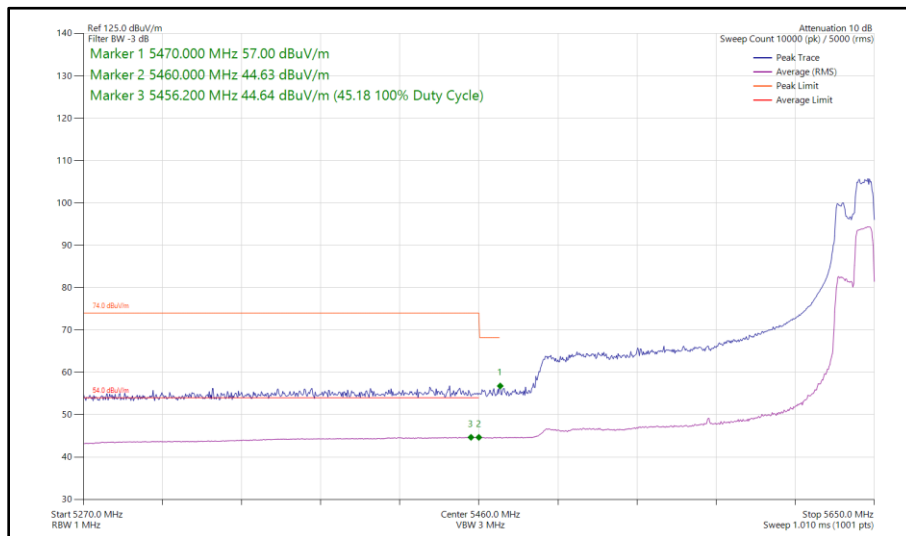
Figure 679 - 802.11ax HE160, RU 106-60S, SISO, Core 1 - 5570 MHz Band Edge Frequency 5470 MHz
