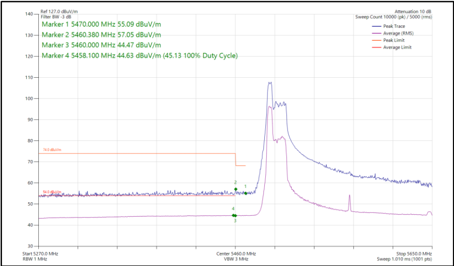
Figure 691 - 802.11ax HE160, RU 52-37P, SDM, Core 0 - Core 1 - 5570 MHz Band Edge Frequency 5470 MHz
