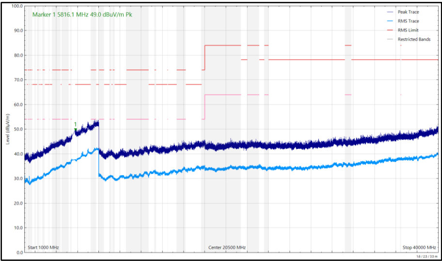
Figure 720 - U-NII-2C - 5700 MHz (CH140), 802.11a, Core 1, 1 GHz to 40 GHz, Horizontal
