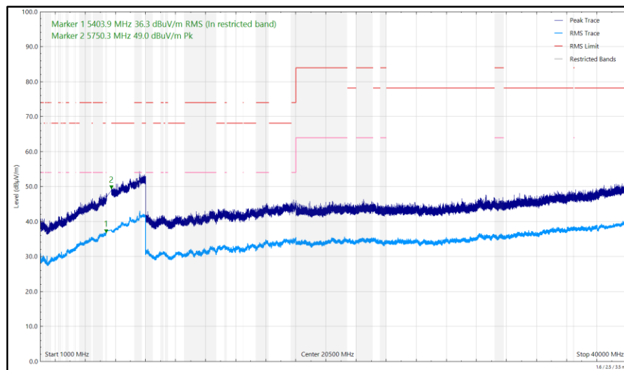
Figure 718 - U-NII-2C - 5500 MHz (CH100), 802.11a, Core 1, 1 GHz to 40 GHz, Horizontal
