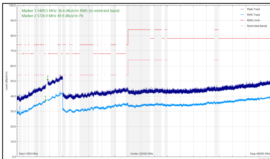
Figure 735 - U-NII-2C - 5500 MHz (CH100), HT20, CDD, Core 0 + Core 1, 1 GHz to 40 GHz, Vertical
