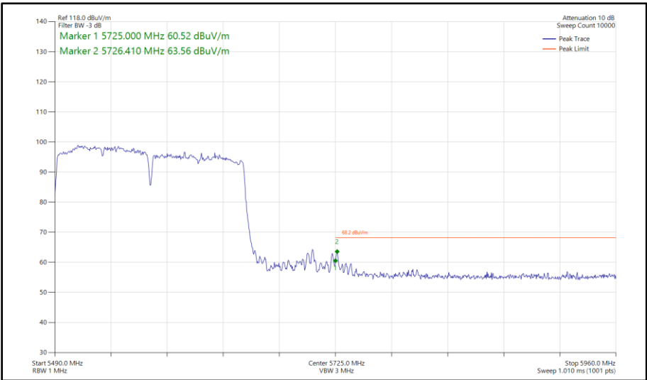
Figure 692 - 802.11ac VHT160, SDM, Core 0 - Core 1 - 5570 MHz Band Edge Frequency 5725 MHz
