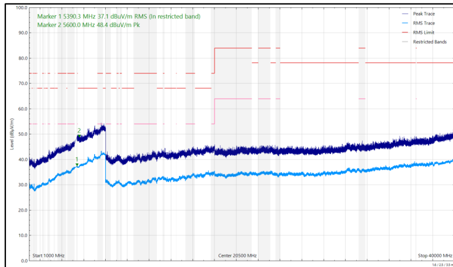
Figure 700 - U-NII-2A - 5320 MHz (CH64), 802.11a, Core 0, 1 GHz to 40 GHz, Horizontal
