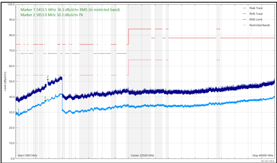
Figure 722 - U-NII-3 - 5745 MHz (CH149), 802.11a, Core 1, 1 GHz to 40 GHz, Horizontal
