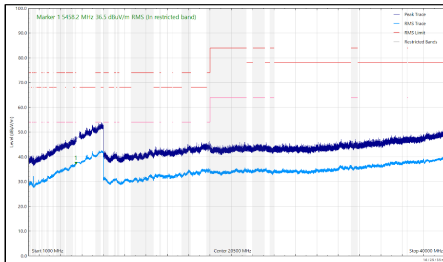
Figure 736 - U-NII-2C - 5700 MHz (CH140), HT20, CDD, Core 0 + Core 1, 1 GHz to 40 GHz, Horizontal
