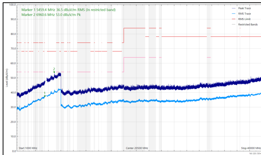
Figure 704 - U-NII-2C - 5700 MHz (CH140), 802.11a, Core 0, 1 GHz to 40 GHz, Horizontal
