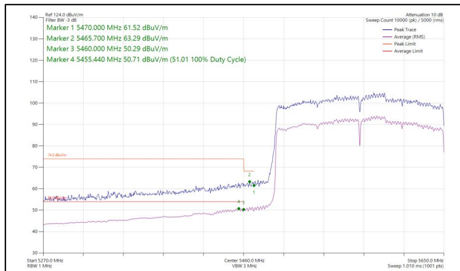
Figure 684 - 802.11ax HE160, SU, CDD, Core 0 - Core 1 - 5570 MHz Band Edge Frequency 5470 MHz
