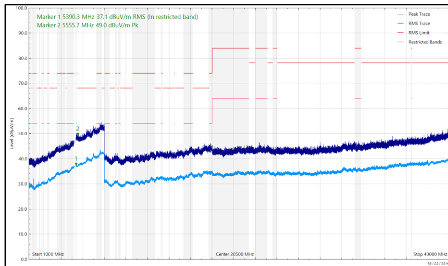
Figure 748 - U-NII-2A - 5320 MHz (CH64), HE20, RU52-37, CDD, Core 0 + Core 1, 1 GHz to 40 GHz, Horizontal
