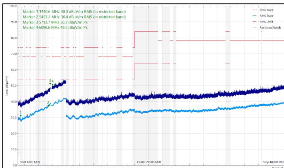
Figure 759 - U-NII-3 - 5825 MHz (CH165), HE20, RU26-0, CDD, Core 0 + Core 1, 1 GHz to 40 GHz, Vertical
