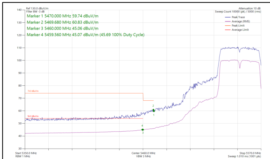
Figure 102 - 802.11n HT40, SISO, Core 0 - 5550 MHz Band Edge Frequency 5460 MHz
