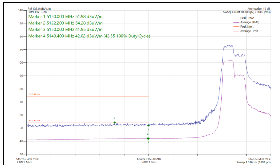
Figure 112 - 802.11ax HE40, RU 106-53, SISO, Core 1 - 5230 MHz Band Edge Frequency 5150 MHz
