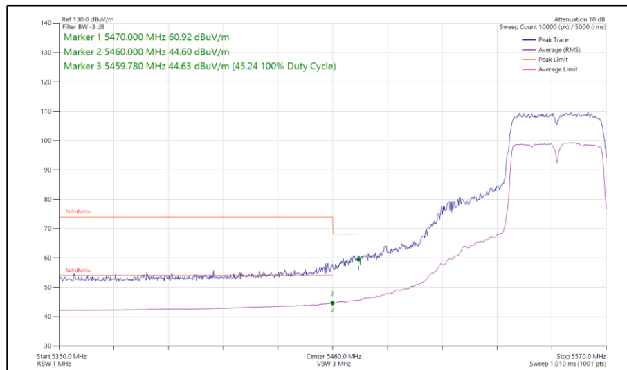
Figure 120 - 802.11n HT40, SISO, Core 1 - 5550 MHz Band Edge Frequency 5460 MHz
