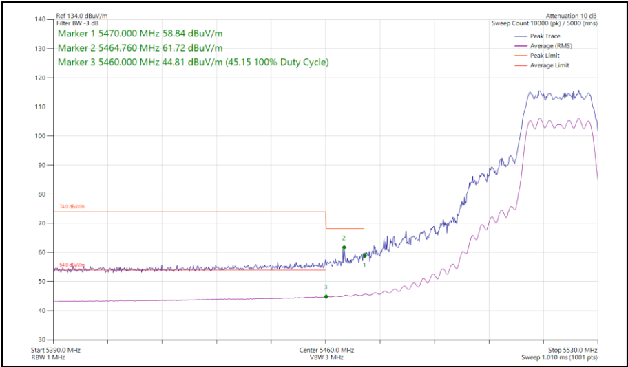
Figure 62 - 802.11n HT20, CDD, Core 0 - Core 1 - 5520 MHz Band Edge Frequency 5460 MHz
