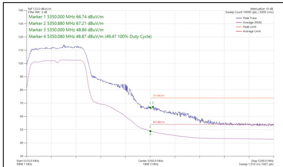
Figure 72 - 802.11n HT20, SDM, Core 0 - Core 1 - 5320 MHz Band Edge Frequency 5350 MHz
