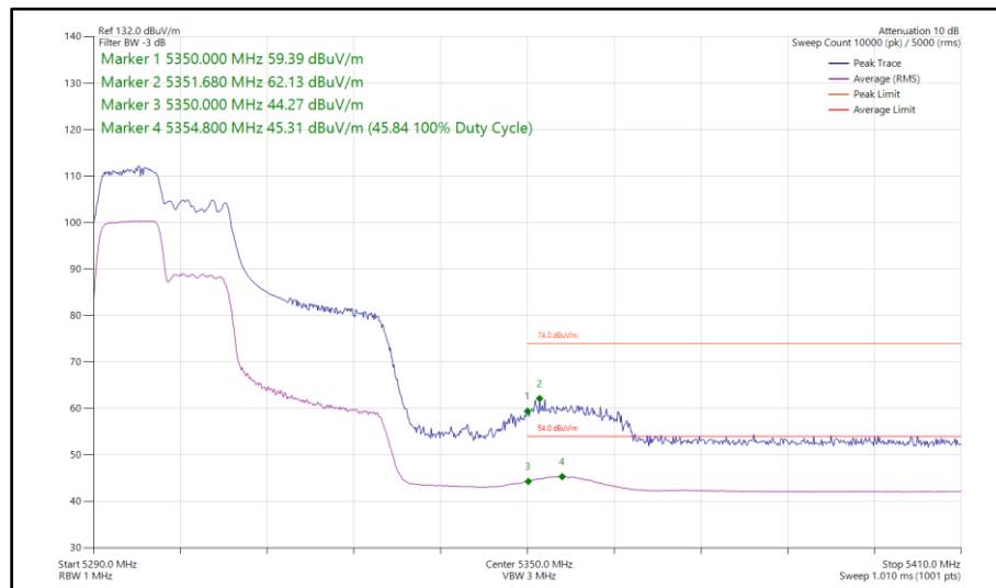
Figure 118 - 802.11ax HE40, RU 106-53, SISO, Core 1 - 5310 MHz Band Edge Frequency 5350 MHz
