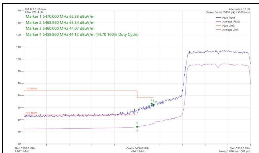
Figure 103 - 802.11ax HE40, SU, SISO, Core 0 - 5510 MHz Band Edge Frequency 5460 MHz
