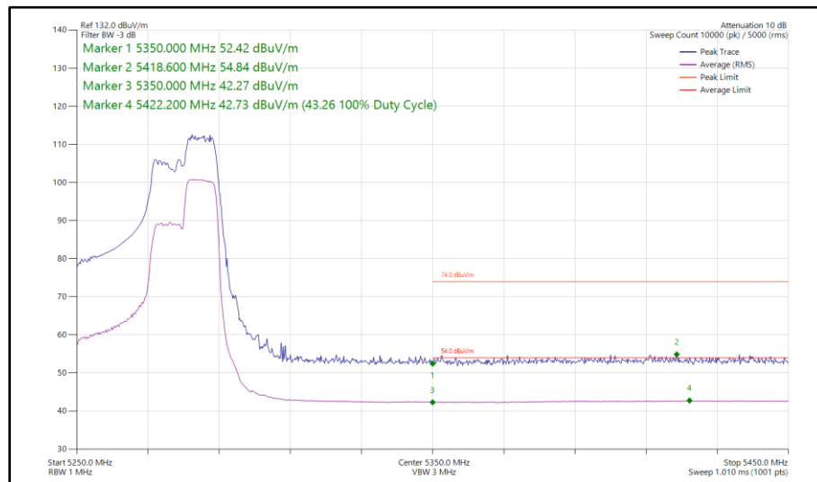
Figure 116 - 802.11ax HE40, RU 106-56, SISO, Core 1 - 5270 MHz Band Edge Frequency 5350 MHz
