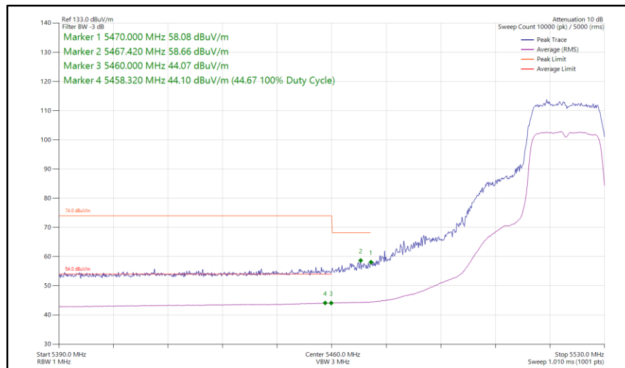
Figure 78 - 802.11n HT20, SDM, Core 0 - Core 1 - 5520 MHz Band Edge Frequency 5460 MHz
