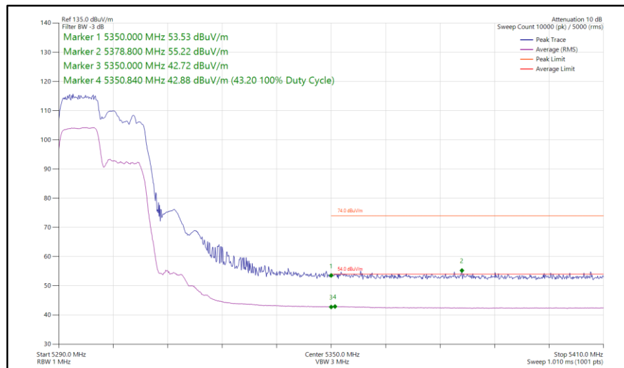
Figure 74 - 802.11ax HE20, RU 106-53, SDM, Core 0 - Core 1 - 5300 MHz Band Edge Frequency 5350 MHz
