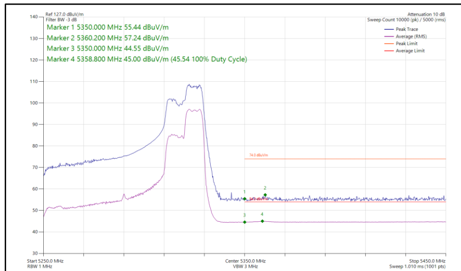
Figure 199 - 802.11ax HE80, RU 106-60, SDM, Core 0 - Core 1 - 5290 MHz Band Edge Frequency 5350 MHz
