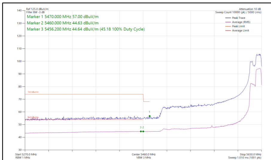
Figure 223 - 802.11ax HE160, RU 106-60S, SISO, Core 1 - 5570 MHz Band Edge Frequency 5460 MHz
