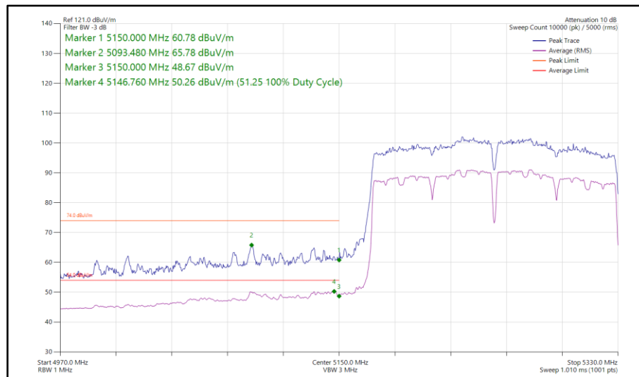
Figure 206 - 802.11ac VHT160, SISO, Core 0 - 5250 MHz Band Edge Frequency 5150 MHz
