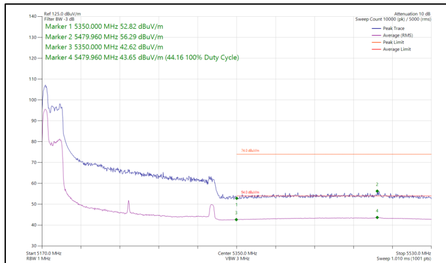
Figure 229 - 802.11ax HE160, RU 52-37P, CDD, Core 0 - Core 1 - 5250 MHz Band Edge Frequency 5350 MHz
