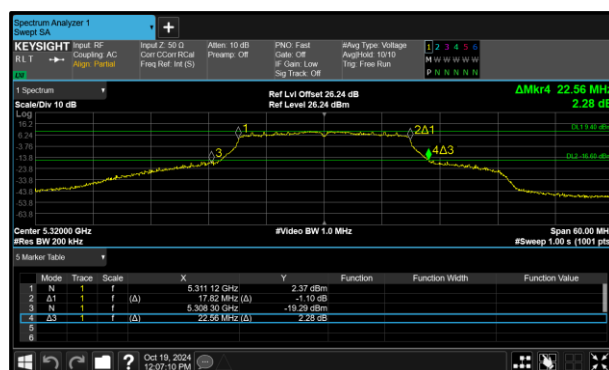
Figure 245 - 802.11n HT20 Maximum 26 dB EBW
