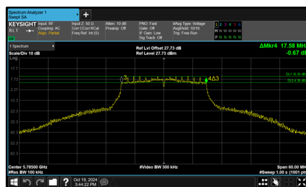
Figure 353 - 802.11n HT20 Maximum 6 dB EBW
