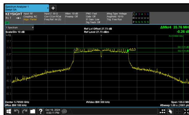
Figure 355 - 802.11n HT40 Maximum 6 dB EBW
