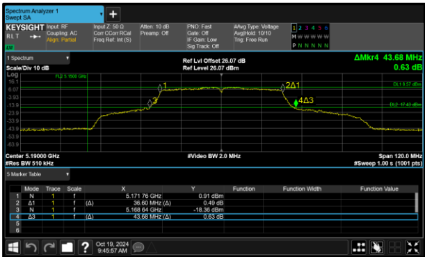
Figure 339 - 802.11n HT40 Maximum 26 dB EBW
