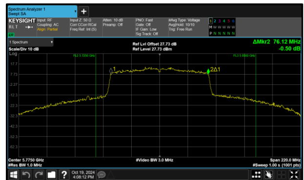
Figure 369 - 802.11ac VHT80 Maximum 99% OBW
