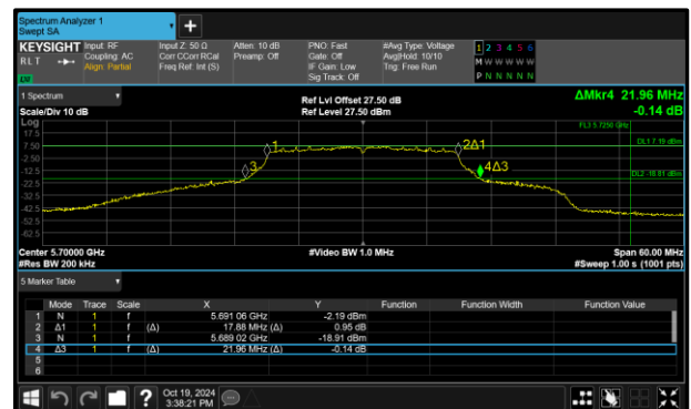
Figure 365 - 802.11n HT20 Maximum 99% OBW
