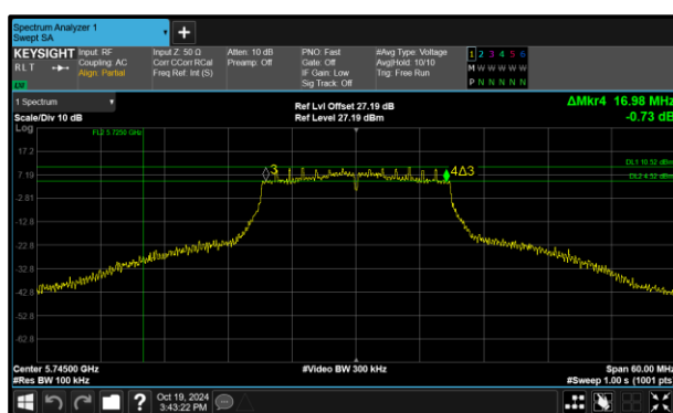
Figure 352 - 802.11n HT20 Minimum 6 dB EBW
