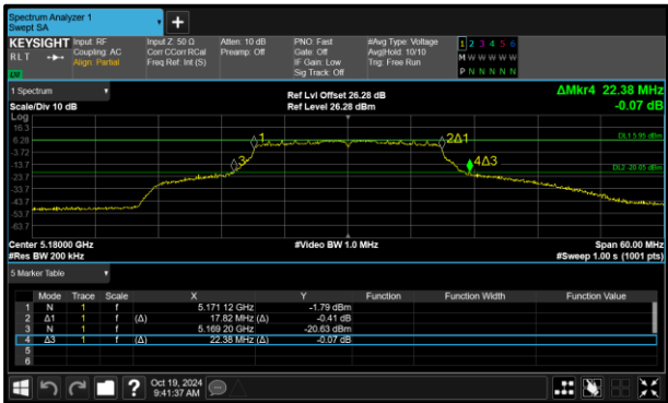
Figure 337 - 802.11n HT20 Maximum 26 dB EBW
