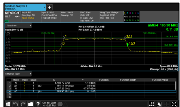
Figure 371 - 802.11ac VHT160 Maximum 99% OBW
