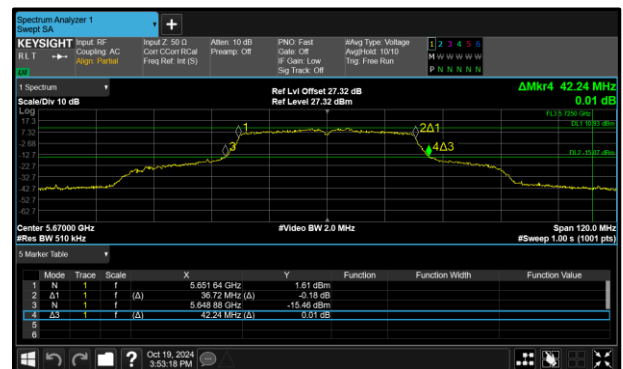
Figure 367 - 802.11n HT40 Maximum 99% OBW
