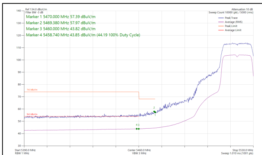
Figure 395 - 802.11n HT20, SISO, Core 0 - 5520 MHz Band Edge Frequency 5470 MHz
