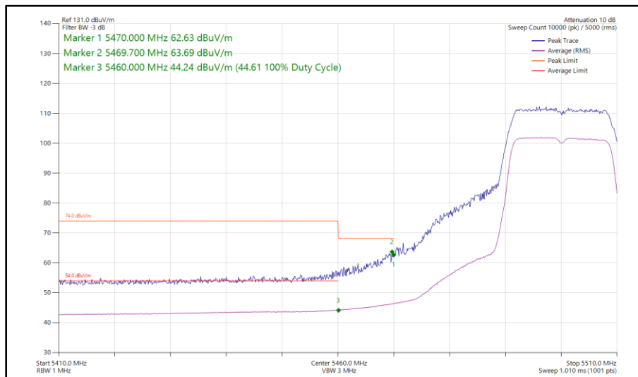
Figure 394 - 802.11n HT20, SISO, Core 0 - 5500 MHz Band Edge Frequency 5470 MHz
