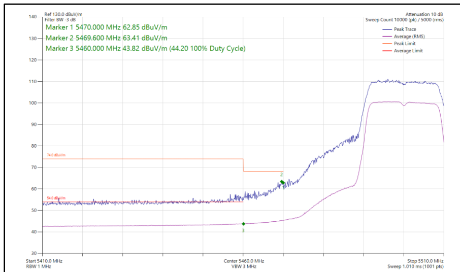
Figure 428 - 802.11n HT20, SISO, Core 1 - 5500 MHz Band Edge Frequency 5470 MHz
