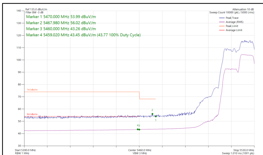
Figure 399 - 802.11ax HE20, RU 106-54, SISO, Core 0 - 5520 MHz Band Edge Frequency 5470 MHz
