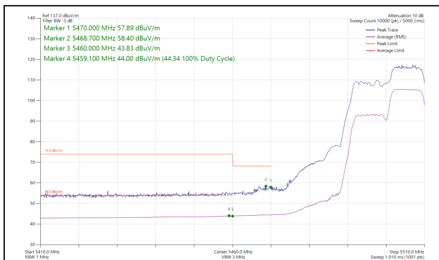
Figure 397 - 802.11ax HE20, RU 106-54, SISO, Core 0 - 5500 MHz Band Edge Frequency 5470 MHz
