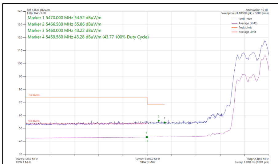
Figure 465 - 802.11ax HE20, RU 52-40, CDD, Core 0 - Core 1 - 5520 MHz Band Edge Frequency 5470 MHz
