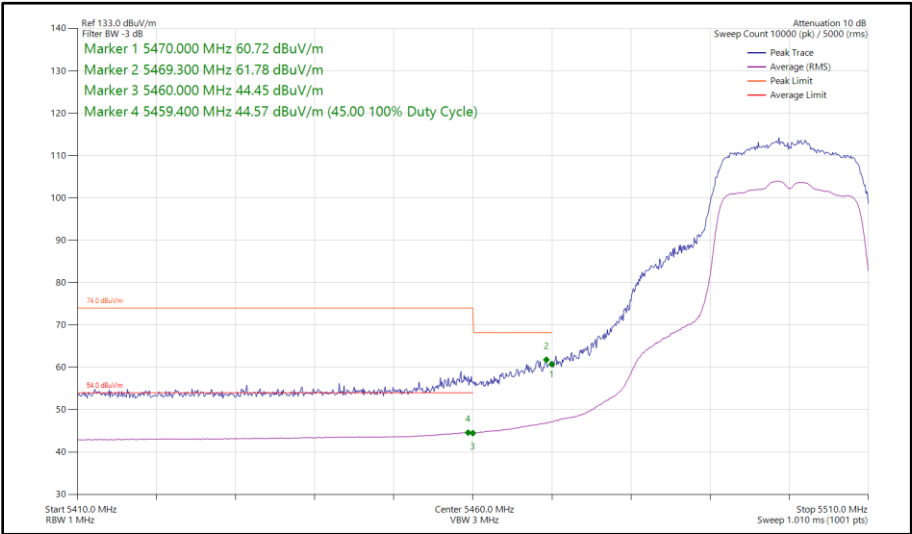
Figure 485 - 802.11n HT20, SDM, Core 0 - Core 1 - 5500 MHz Band Edge Frequency 5470 MHz
