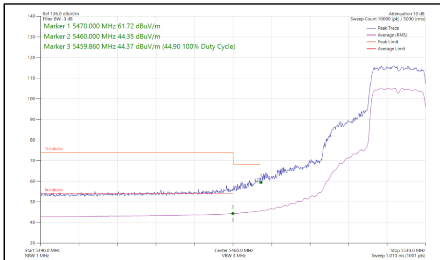
Figure 464 - 802.11ax HE20, SU, CDD, Core 0 - Core 1 - 5520 MHz Band Edge Frequency 5470 MHz
