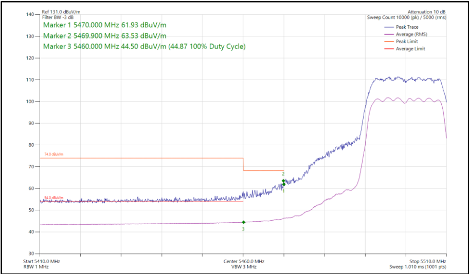
Figure 460 - 802.11n HT20, CDD, Core 0 - Core 1 - 5500 MHz Band Edge Frequency 5470 MHz
