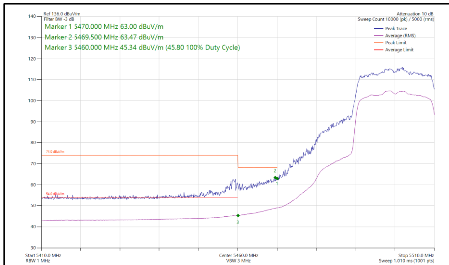
Figure 487 - 802.11ax HE20, SU, SDM, Core 0 - Core 1 - 5500 MHz Band Edge Frequency 5470 MHz
