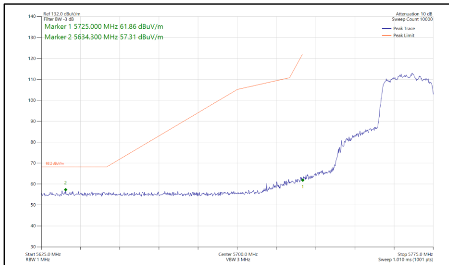
Figure 470 - 802.11ax HE20, SU, CDD, Core 0 - Core 1 - 5765 MHz Band Edge Frequency 5725 MHz
