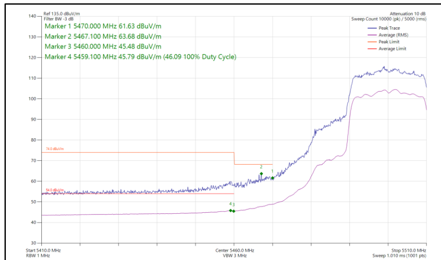
Figure 462 - 802.11ax HE20, SU, CDD, Core 0 - Core 1 - 5500 MHz Band Edge Frequency 5470 MHz
