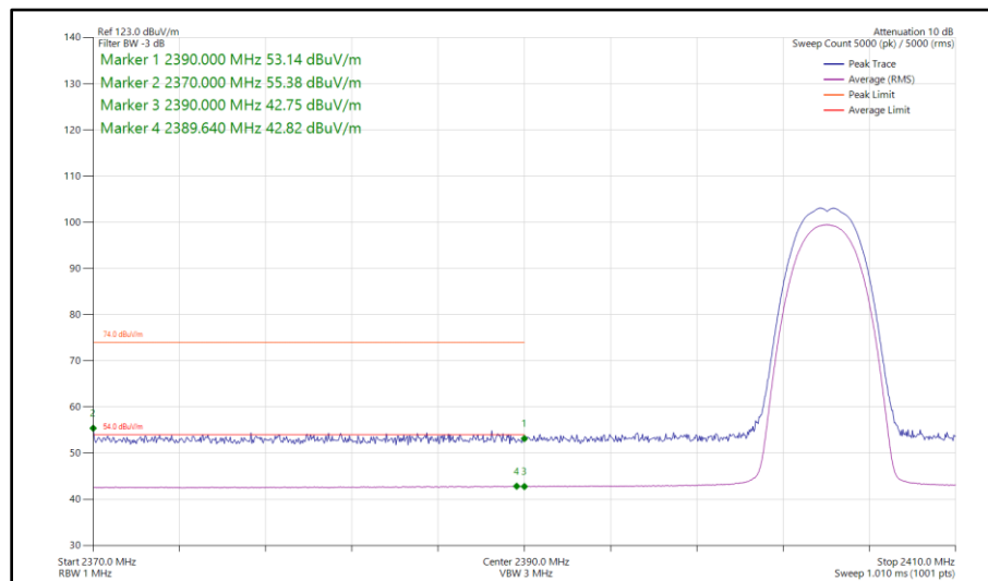
Figure 31 - Bluetooth HDR4, MIMO, Core 0 - Core 1 - 2404 MHz Band Edge Frequency 2390 MHz
