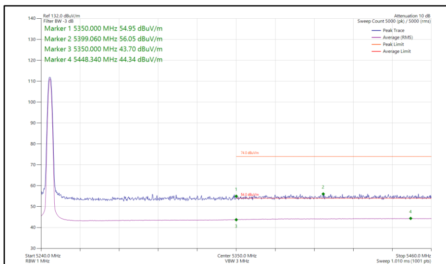
Figure 34 - Bluetooth DH5, MIMO, Core 0 - Core 1 - 5245 MHz Band Edge Frequency 5350 MHz
