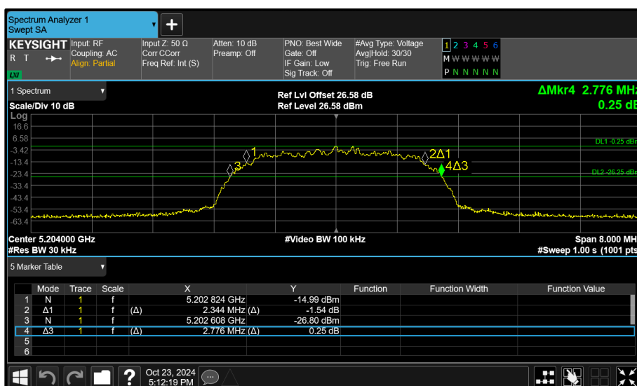
Figure 41 - Core 1 (B) 5204 MHz (CH54) 26 dB and 99% Bandwidth
