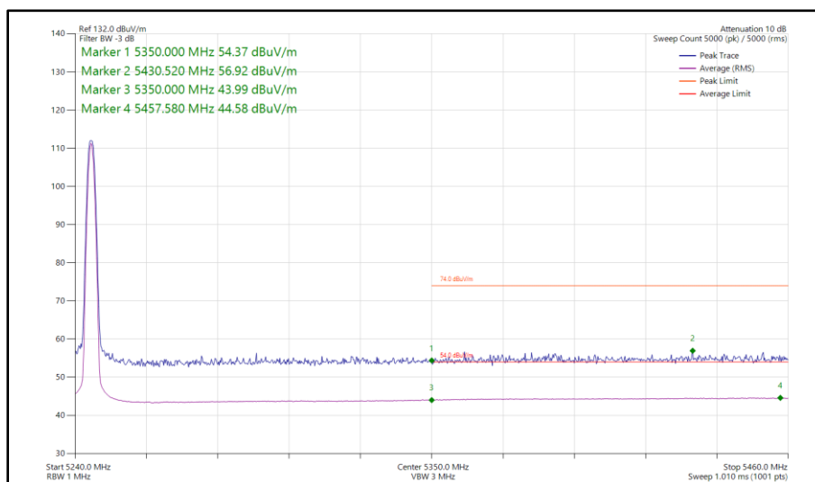
Figure 28 - Bluetooth DH5, SISO, Core 1 - 5245 MHz Band Edge Frequency 5350 MHz
