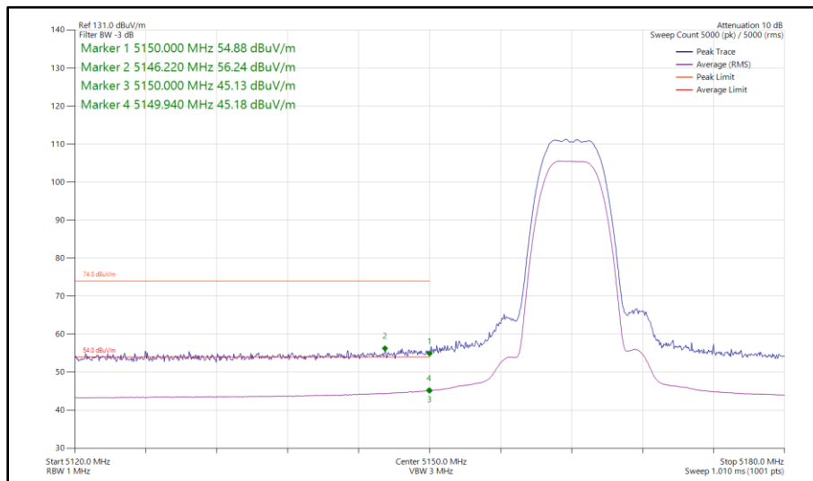
Figure 21 - Bluetooth HDR8, SISO, Core 0 - 5162 MHz Band Edge Frequency 5150 MHz
