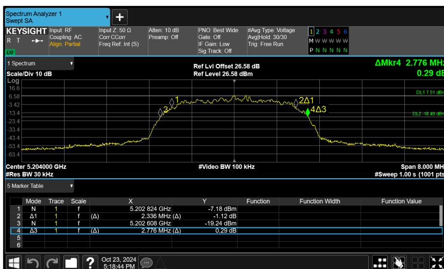
Figure 65 - Core 1 (B) 5204 MHz (CH54) 26 dB and 99% Bandwidth
