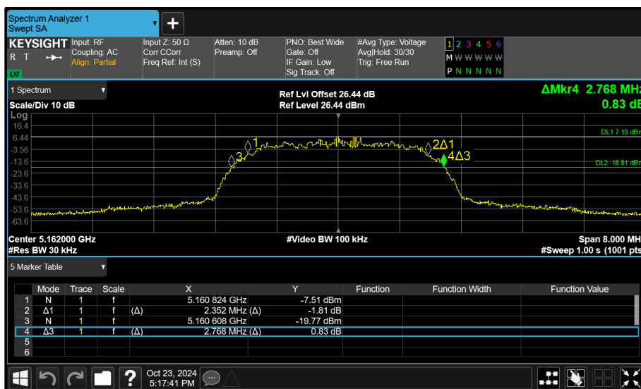
Figure 64 - Core 1 (B) 5162 MHz (CH12) 26 dB and 99% Bandwidth
