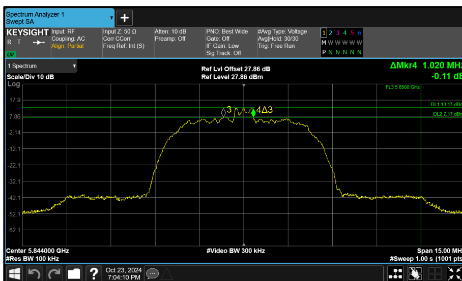
Figure 171 - Core 1 (B) 5844 MHz (CH119) 6 dB Bandwidth
