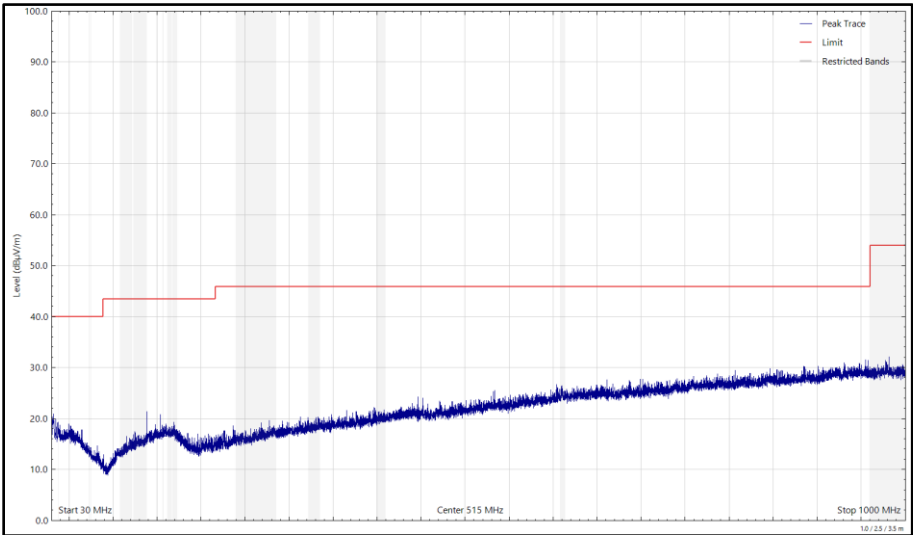
Figure 57 - 2440 MHz (CH18), Thread, ePA, Core 1, 30 MHz to 1 GHz, Horizontal (Peak)
