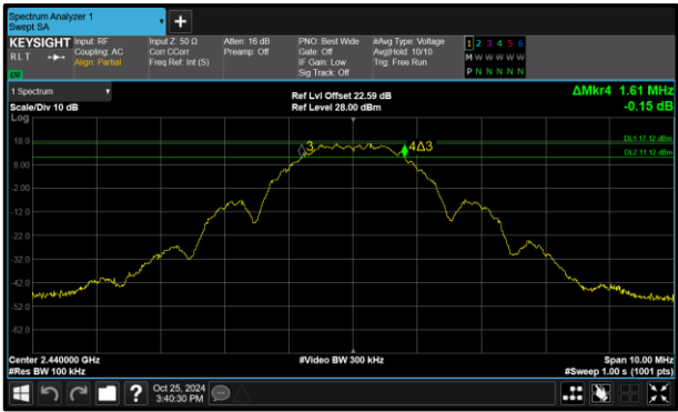
Figure 32 - Core 1 (B) 2440 MHz (CH18) 6 dB Bandwidth
