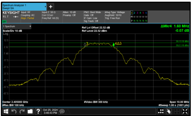
Figure 36 - Core 2 (C) 2405 MHz (CH11) 6 dB Bandwidth
