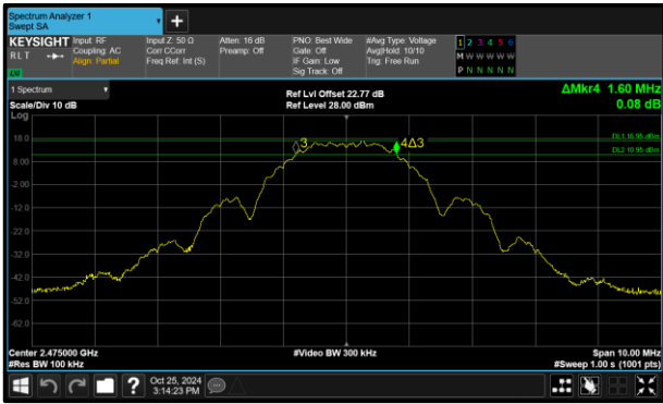
Figure 22 - Core 0 (A) 2475 MHz (CH25) 6 dB Bandwidth
