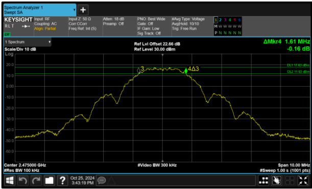
Figure 34 - Core 1 (B) 2475 MHz (CH25) 6 dB Bandwidth
