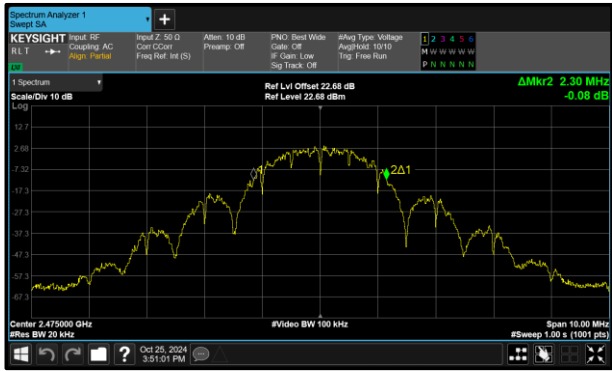
Figure 39 - Core 2 (C) 2475 MHz (CH25) 99% Bandwidth
