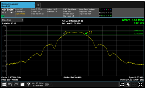
Figure 24 - Core 1 (B) 2405 MHz (CH11) 6 dB Bandwidth
