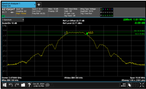
Figure 16 - Core 0 (A) 2475 MHz (CH25) 6 dB Bandwidth
