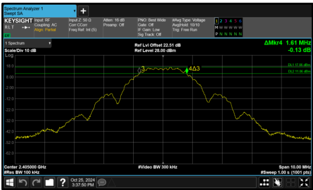
Figure 30 - Core 1 (B) 2405 MHz (CH11) 6 dB Bandwidth
