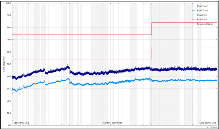
Figure 47 - 2405 MHz (CH11), Thread, ePA, Core 0, 1 GHz to 26 GHz, Horizontal
