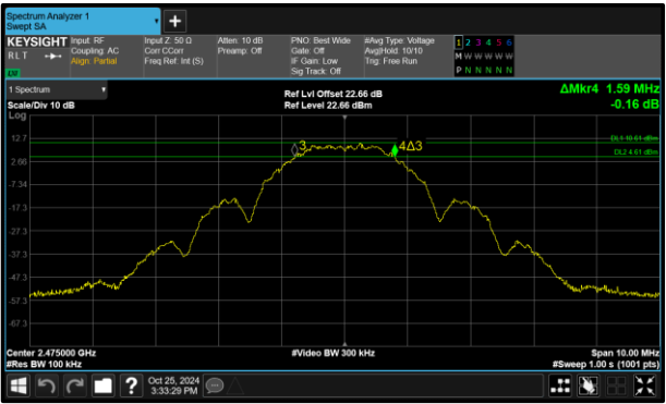
Figure 28 - Core 1 (B) 2475 MHz (CH25) 6 dB Bandwidth
