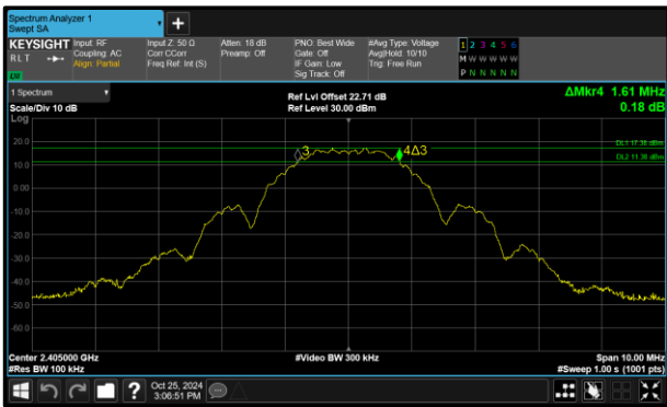
Figure 18 - Core 0 (A) 2405 MHz (CH11) 6 dB Bandwidth
