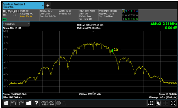
Figure 37 - Core 2 (C) 2440 MHz (CH18) 99% Bandwidth
