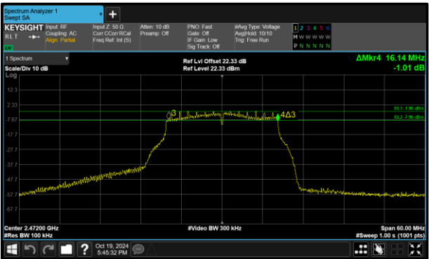
Figure 107 - 802.11g Maximum 6 dB EBW
