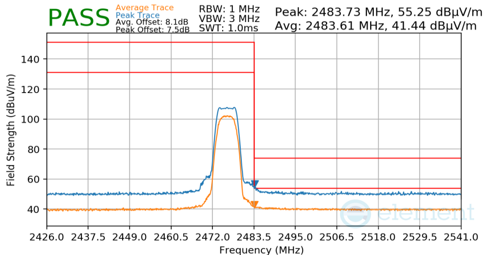
Plot 7-50. Radiated Restricted Upper Band Edge Measurement
