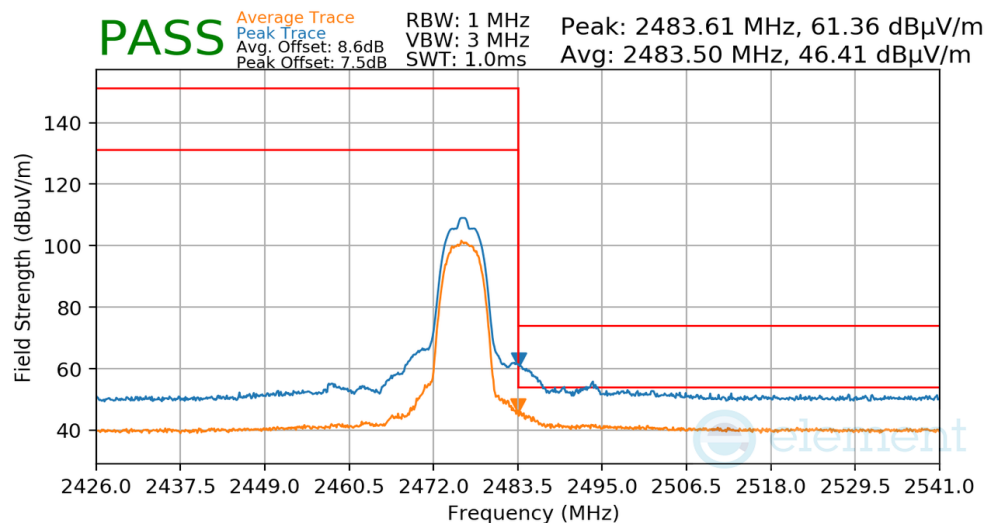
Plot 7-48. Radiated Restricted Upper Band Edge Measurement
