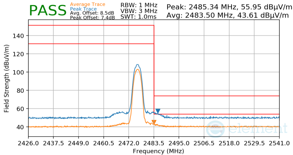
Plot 7-47. Radiated Restricted Upper Band Edge Measurement
