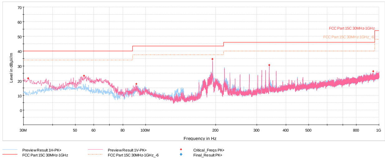
Plot 7-51. Radiated Spurious Emissions Below 1GHz (4Mbps, – Ch.73 with AC/DC Adapter and USB-C cable)
