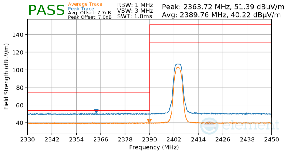
Plot 7-45. Radiated Restricted Lower Band Edge Measurement
