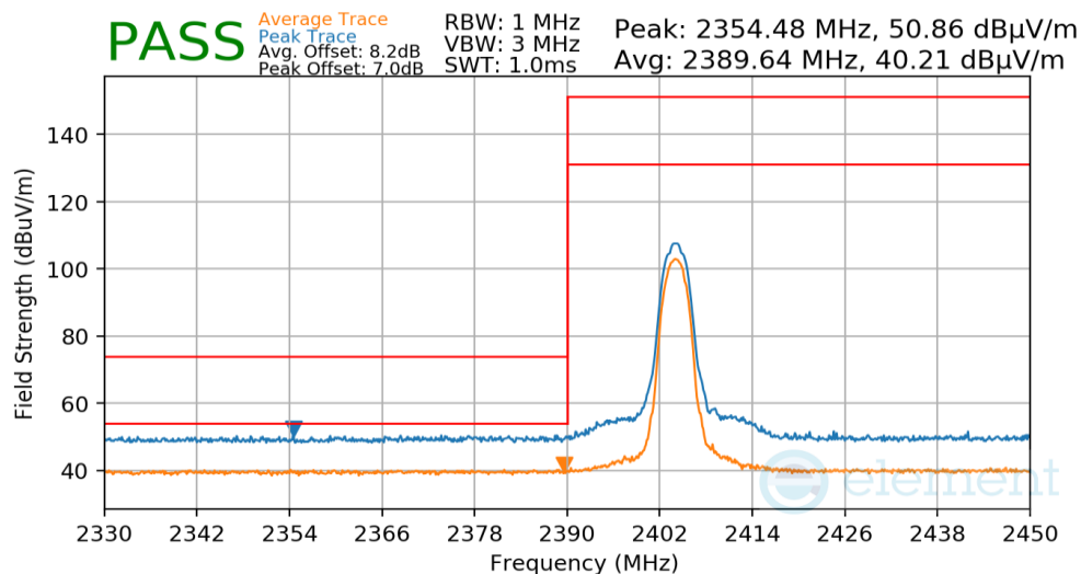
Plot 7-43. Radiated Restricted Lower Band Edge Measurement
