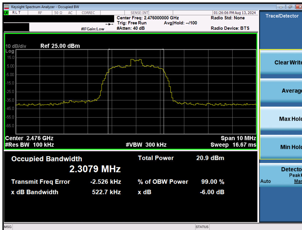
Plot 7-3. 6dB BW & 99% OBW Plot (Bluetooth (HDR4), 4Mbps, – Ch. 73)
