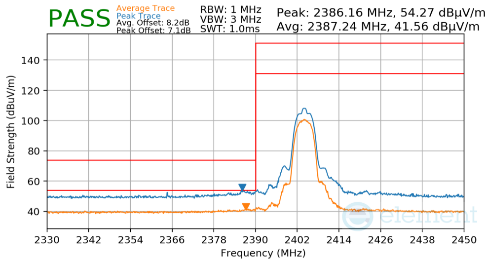
Plot 7-44. Radiated Restricted Lower Band Edge Measurement
