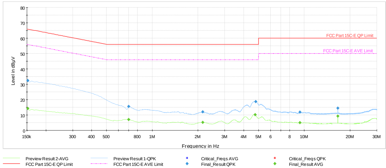
Plot 7-52. AC Line Conducted Plot with Bluetooth HDR (L1, 4Mbps - Ch.73 with host PC and USB-C cable)
