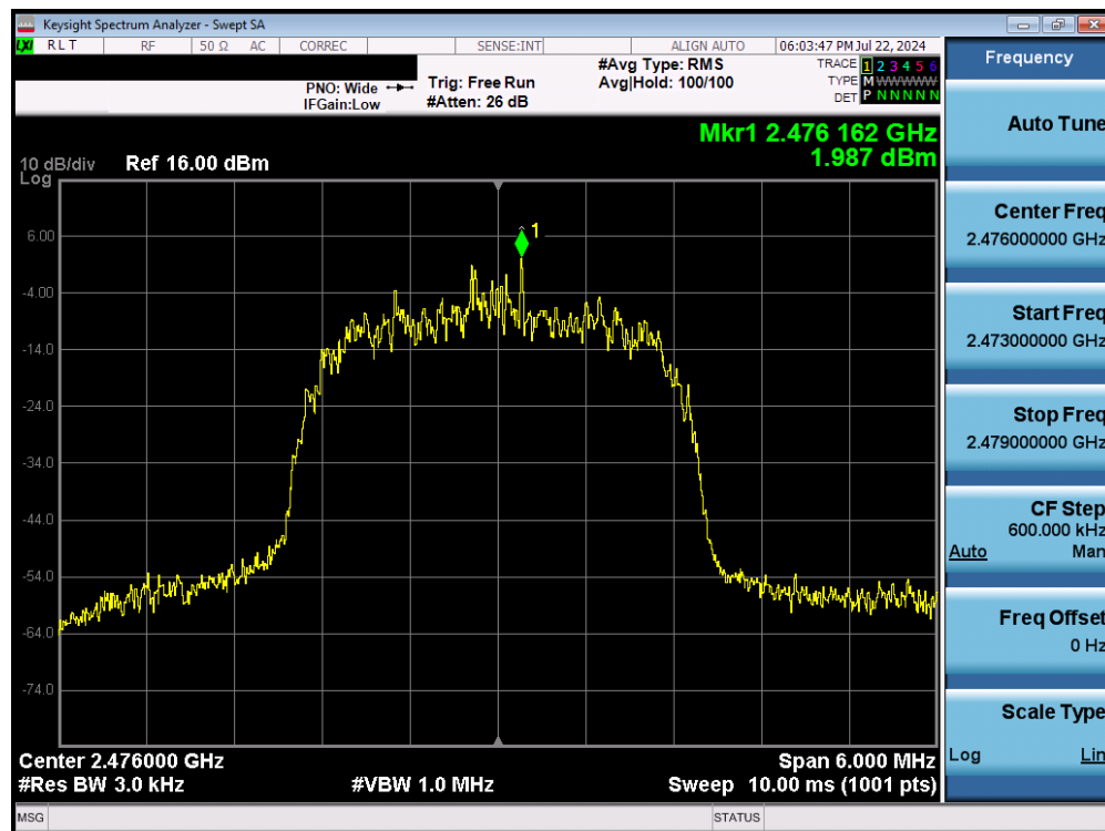
Plot 7-15. Power Spectral Density Plot (Bluetooth (HDR4), 4Mbps, – Ch. 73)
