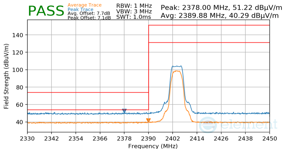
Plot 7-46. Radiated Restricted Lower Band Edge Measurement
