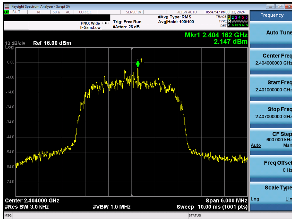
Plot 7-13. Power Spectral Density Plot (Bluetooth (HDR4), 4Mbps, – Ch. 1)
