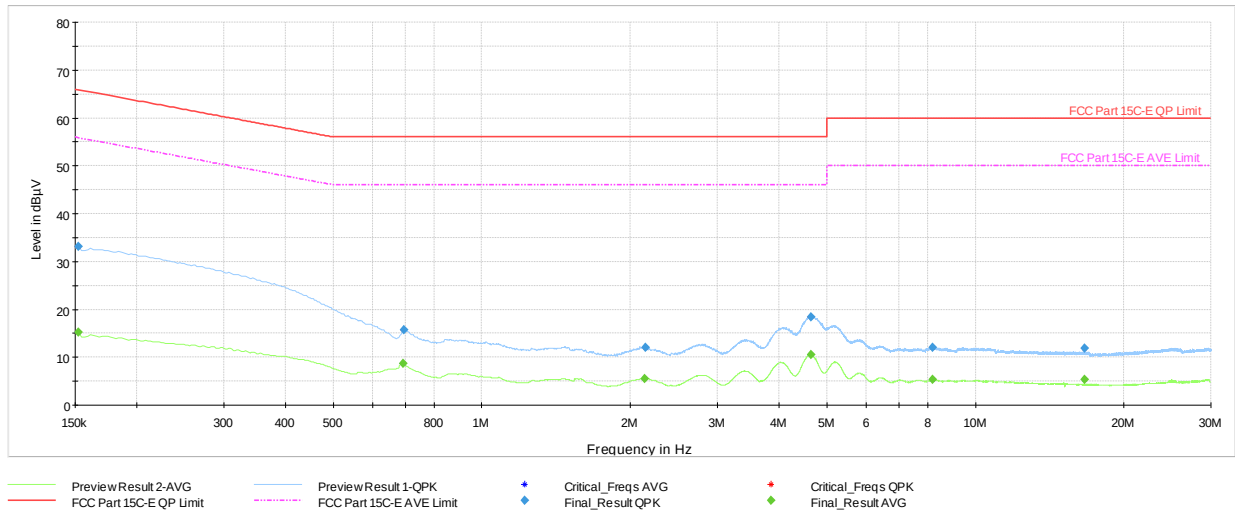
Plot 7-53. AC Line Conducted Plot with Bluetooth HDR (N, 4Mbps - Ch.73 with host PC and USB-C cable)
