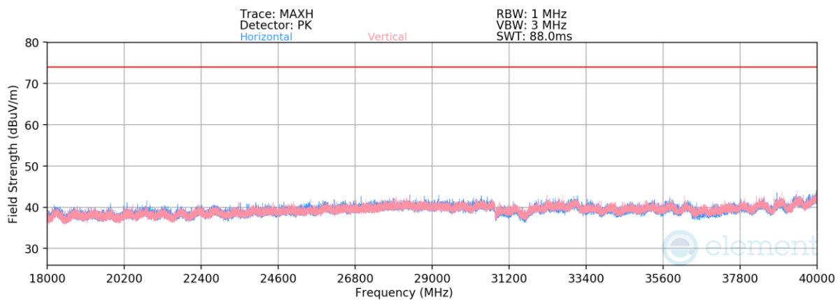
Plot 7-42. Radiated Spurious Emissions Above 18GHz (4Mbps, HDR4, – Ch. 38)
