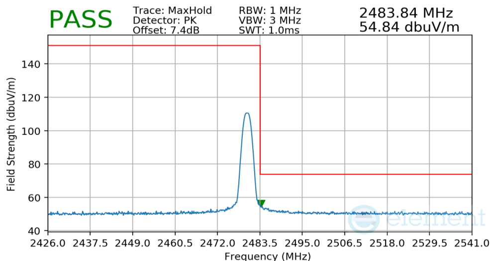
Plot 7-35. Radiated Restricted Upper Band Edge Measurement
