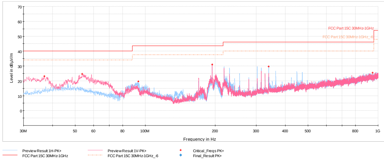
Plot 7-37. Radiated Spurious Emissions Below 1GHz (GFSK – Ch.78, with AC/DC Adapter & USB-C Cable)
