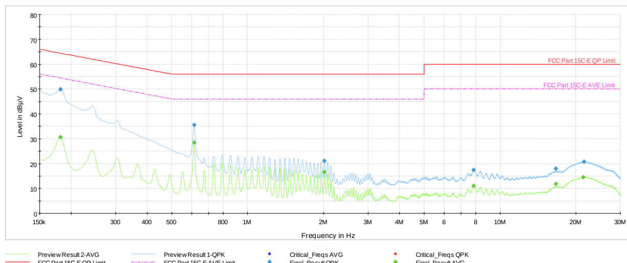
Plot 7-39. AC Line-Conducted Test Plot (N GFSK – Ch.78, with host PC & USB-C cable)
