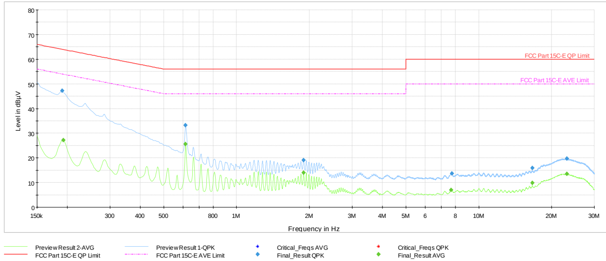
Plot 7-38. AC Line-Conducted Test Plot (L1, GFSK – Ch.78, with host PC & USB-C cable)
