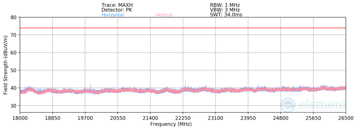
Plot 7-32. Radiated Spurious Emissions above 18GHz (GFSK – Ch.78)
