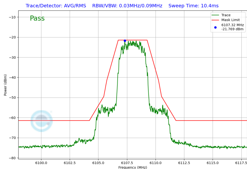
Plot 7-43. VLP In-Band Emission Plot (NB UNII HDR4 – 6108MHz)
