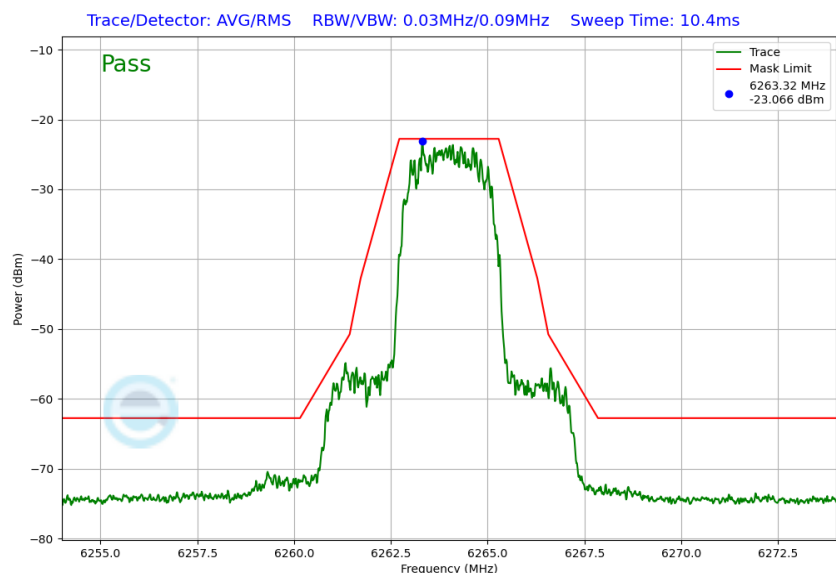
Plot 7-44. VLP In-Band Emission Plot (NB UNII HDR4 – 6264MHz)
