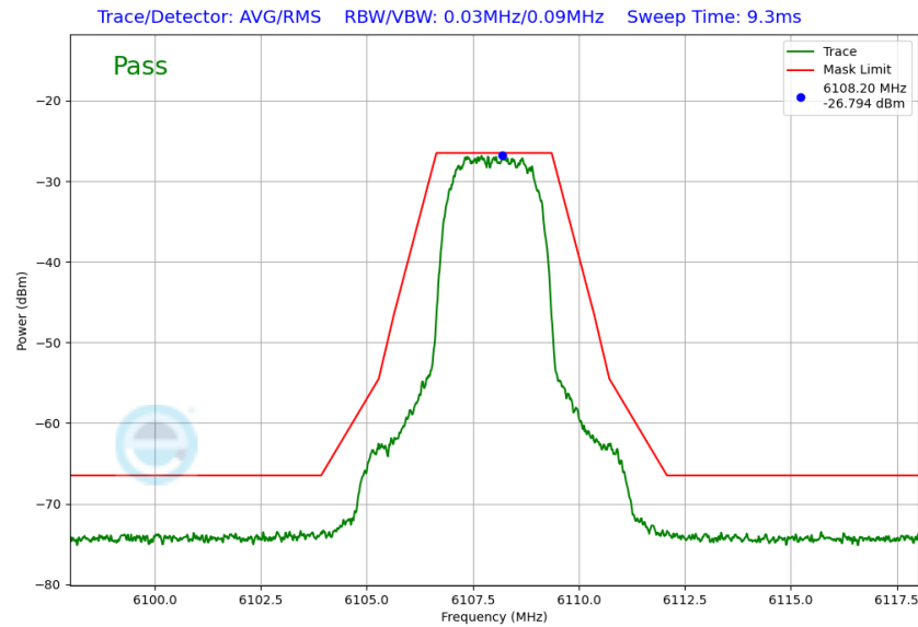
Plot 7-49. VLP In-Band Emission Plot (NB UNII HDRp4 – 6108MHz)
