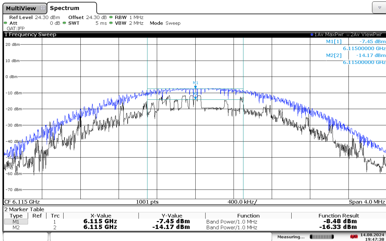
Plot 7-59. Power Spectral Density Plot (NB UNII BDR, 6115MHz)
