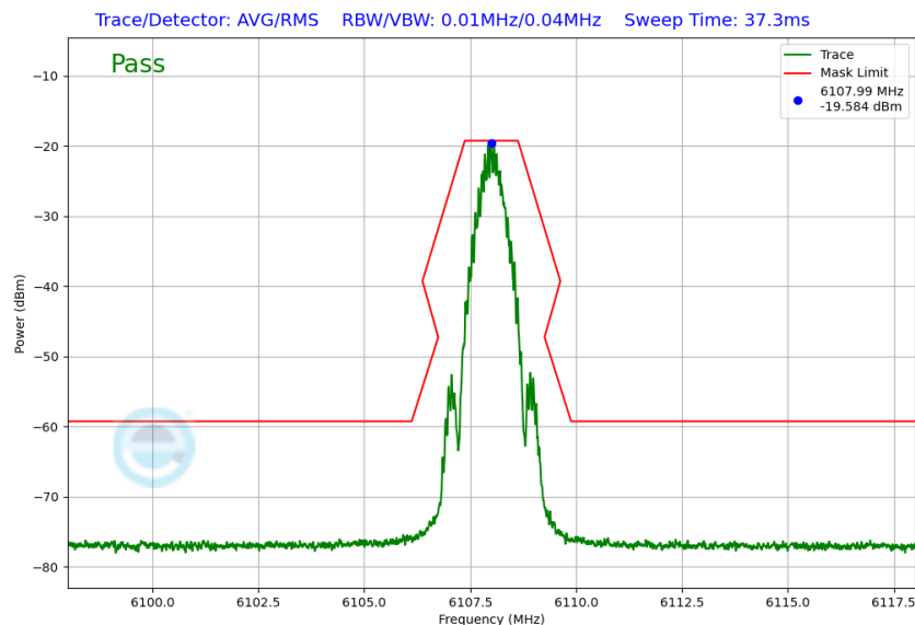
Plot 7-37. VLP In-Band Emission Plot (NB UNII BDR – 6108MHz)
