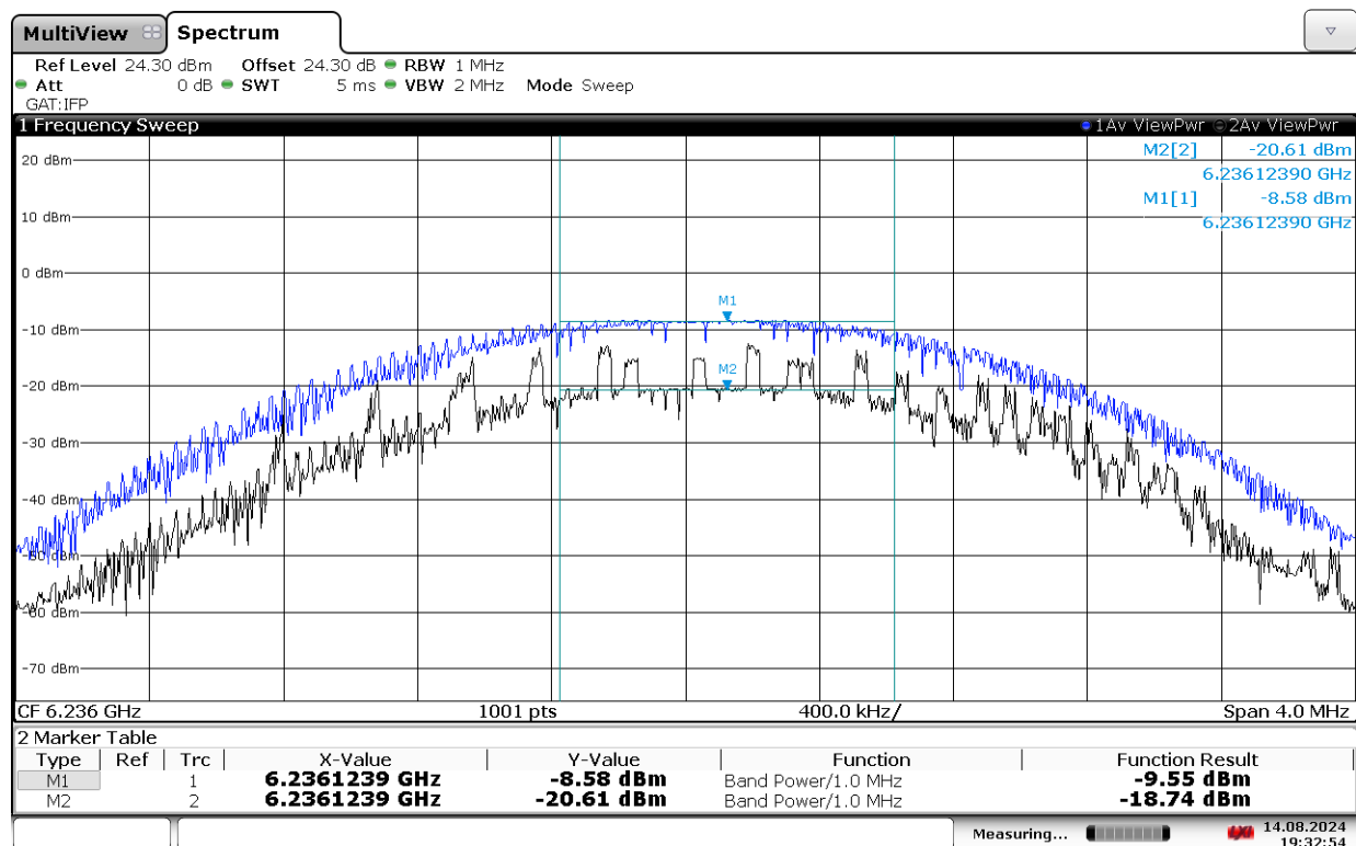
Plot 7-60. Power Spectral Density Plot (NB U11 BDR, 6236MHz)
