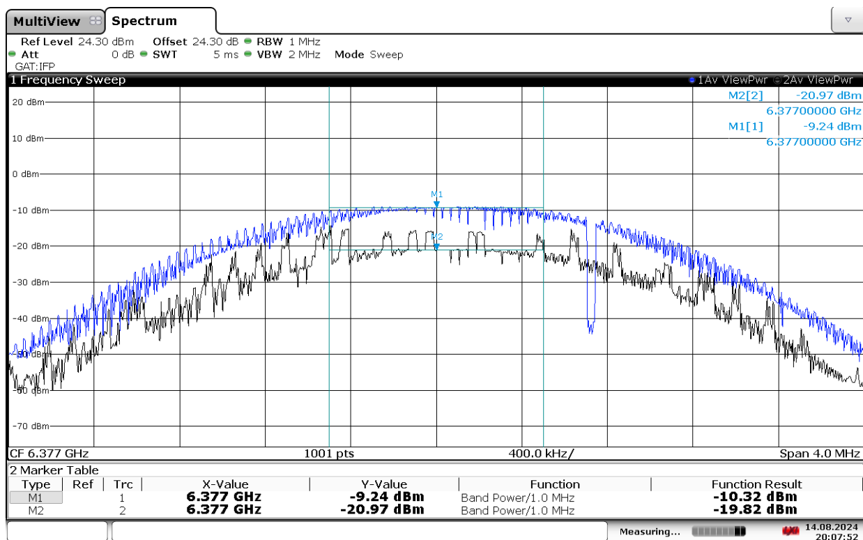
Plot 7-61. Power Spectral Density Plot (NB U11 BDR, 6377MHz)
