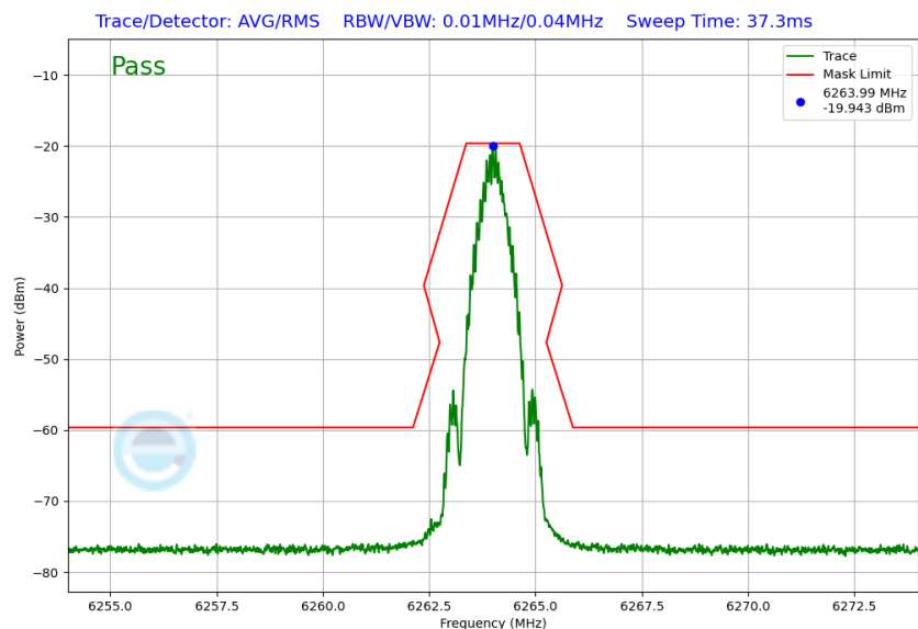
Plot 7-38. VLP In-Band Emission Plot (NB UNII BDR – 6264MHz)
