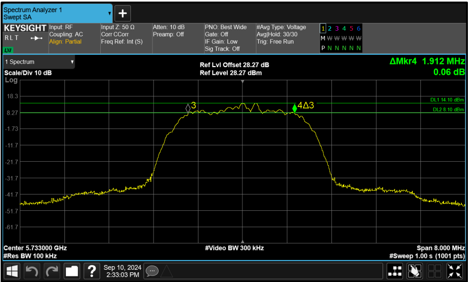
Figure 89 - Core 0 (A) 5733 MHz (CH8) 6 dB Bandwidth
