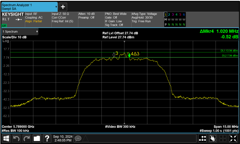
Figure 107 - Core 1 (B) 5789 MHz (CH64) 6 dB Bandwidth
