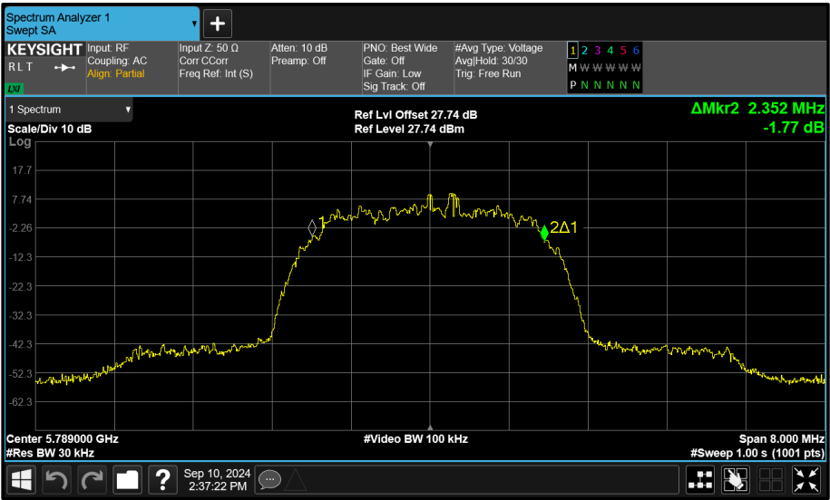
Figure 94 - Core 1 (B) 5789 MHz (CH64) 99% Bandwidth
