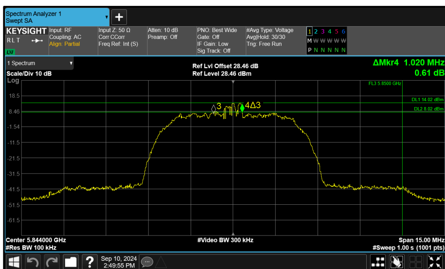
Figure 109 - Core 0 (A) 5844 MHz (CH119) 6 dB Bandwidth
