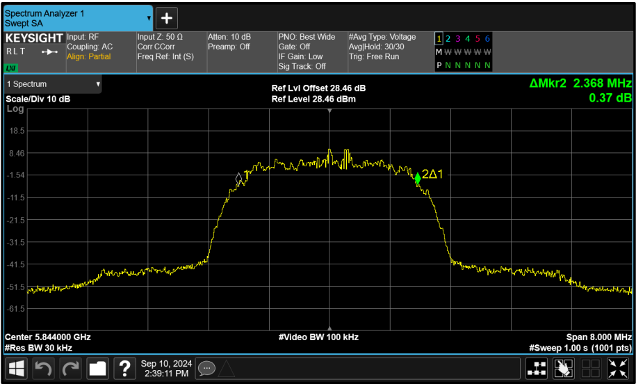
Figure 96 - Core 0 (A) 5844 MHz (CH119) 99% Bandwidth
