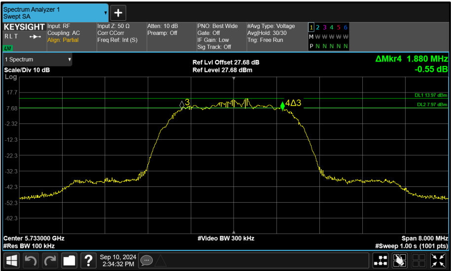
Figure 91 - Core 1 (B) 5733 MHz (CH8) 6 dB Bandwidth
