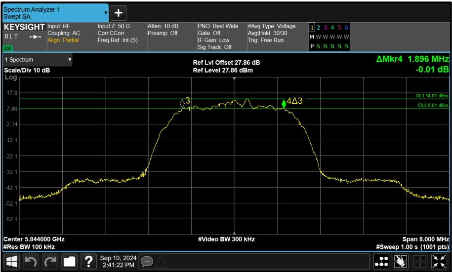
Figure 99 - Core 1 (B) 5844 MHz (CH119) 6 dB Bandwidth
