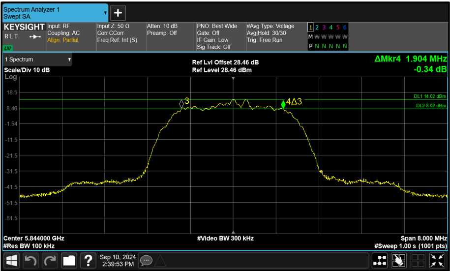
Figure 97 - Core 0 (A) 5844 MHz (CH119) 6 dB Bandwidth
