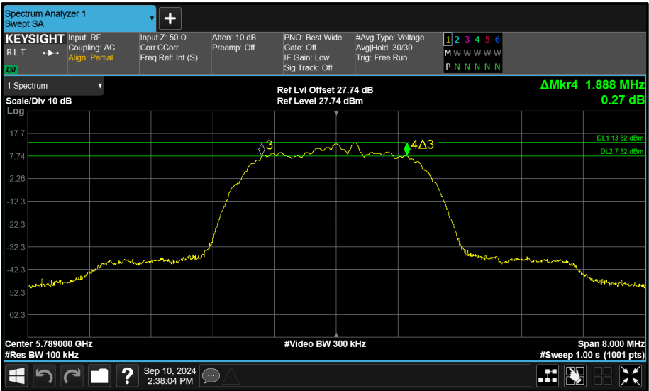
Figure 95 - Core 1 (B) 5789 MHz (CH64) 6 dB Bandwidth
