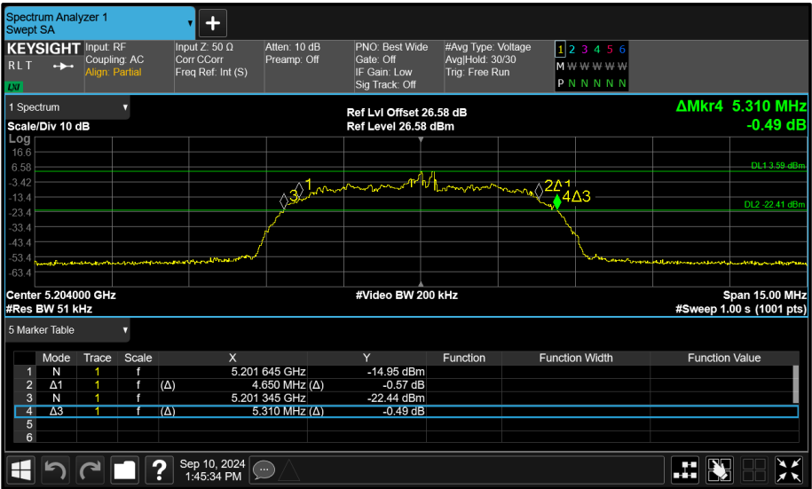
Figure 127 - Core 1 (B) 5204 MHz (CH54) 26 dB and 99% Bandwidth
