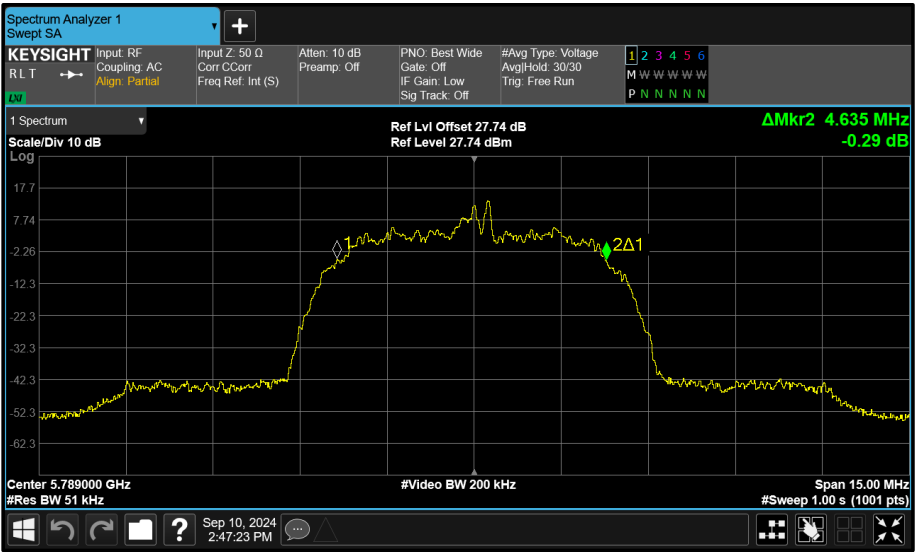
Figure 106 - Core 1 (B) 5789 MHz (CH64) 99% Bandwidth
