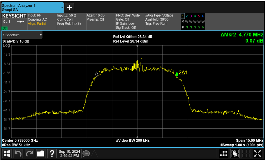
Figure 104 - Core 0 (A) 5789 MHz (CH64) 99% Bandwidth
