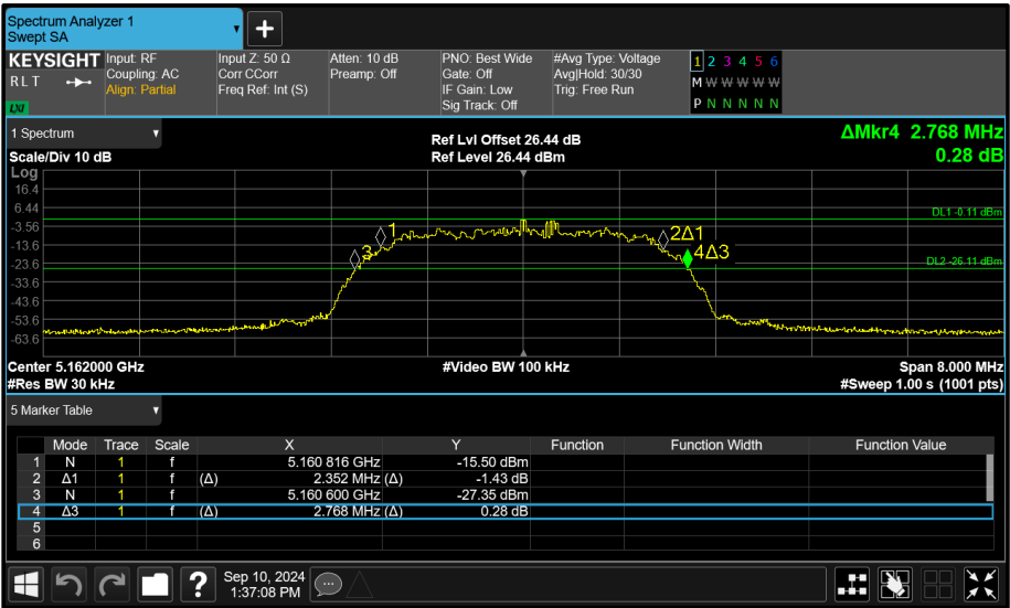
Figure 119 - Core 1 (B) 5162 MHz (CH12) 26 dB and 99% Bandwidth
