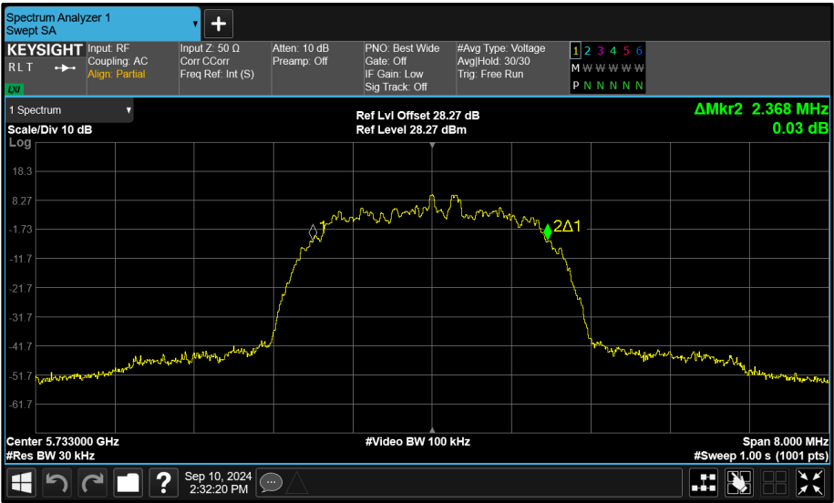
Figure 88 - Core 0 (A) 5733 MHz (CH8) 99% Bandwidth
