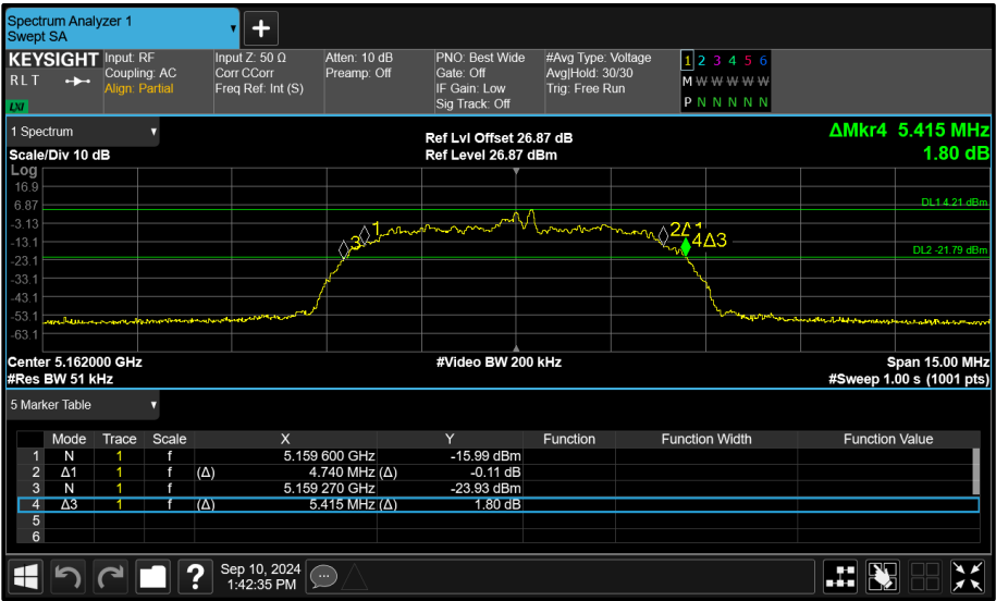
Figure 124 - Core 0 (A) 5162 MHz (CH12) 26 dB and 99% Bandwidth
