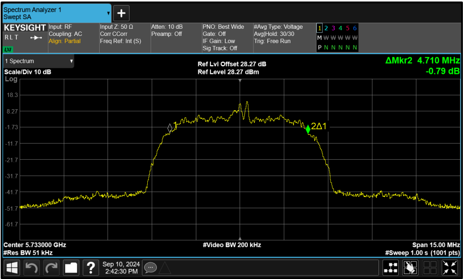
Figure 100 - Core 0 (A) 5733 MHz (CH8) 99% Bandwidth
