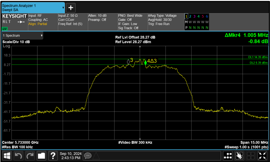
Figure 101 - Core 0 (A) 5733 MHz (CH8) 6 dB Bandwidth
