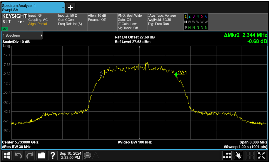
Figure 90 - Core 1 (B) 5733 MHz (CH8) 99% Bandwidth
