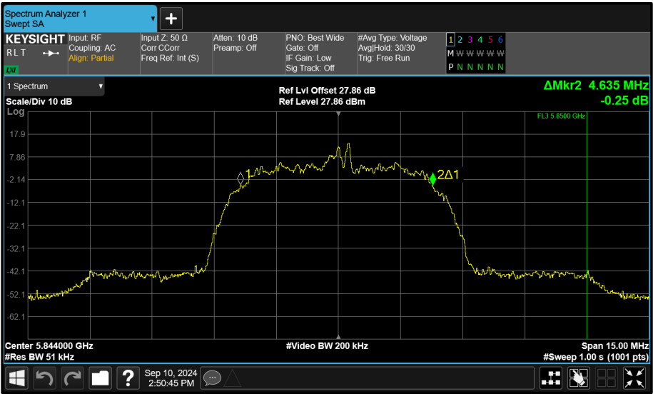
Figure 110 - Core 1 (B) 5844 MHz (CH119) 99% Bandwidth
