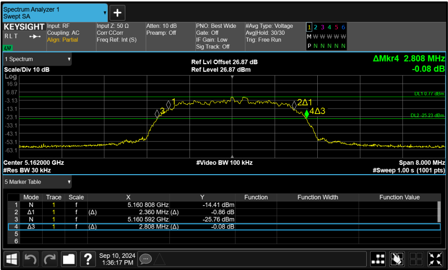
Figure 118 - Core 0 (A) 5162 MHz (CH12) 26 dB and 99% Bandwidth
