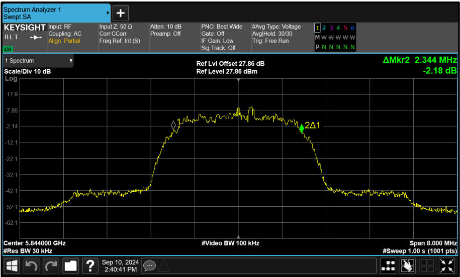
Figure 98 - Core 1 (B) 5844 MHz (CH119) 99% Bandwidth
