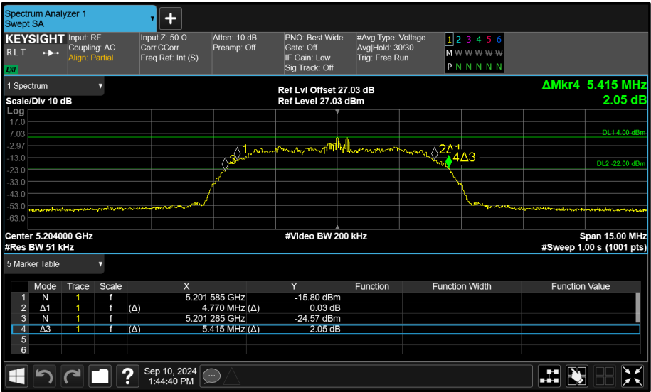
Figure 126 - Core 0 (A) 5204 MHz (CH54) 26 dB and 99% Bandwidth
