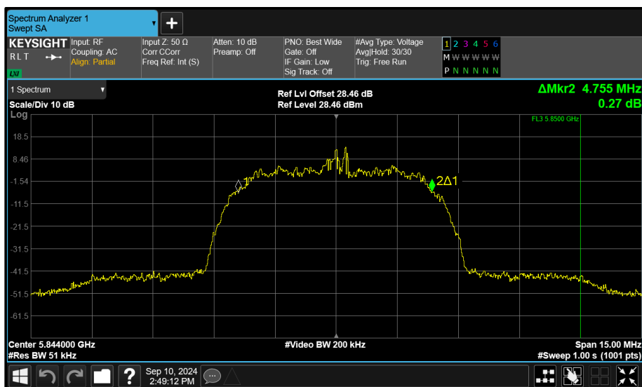
Figure 108 - Core 0 (A) 5844 MHz (CH119) 99% Bandwidth
