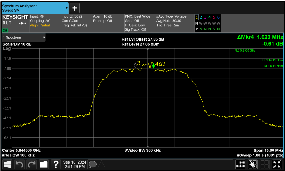
Figure 111 - Core 1 (B) 5844 MHz (CH119) 6 dB Bandwidth
