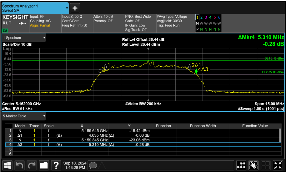
Figure 125 - Core 1 (B) 5162 MHz (CH12) 26 dB and 99% Bandwidth
