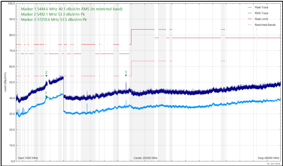
Figure 705 - U-NII-3 - 5745 MHz (CH149), HE20, RU26-0, CDD, Core 0 + Core 1, 1 GHz to 40 GHz, Horizontal
