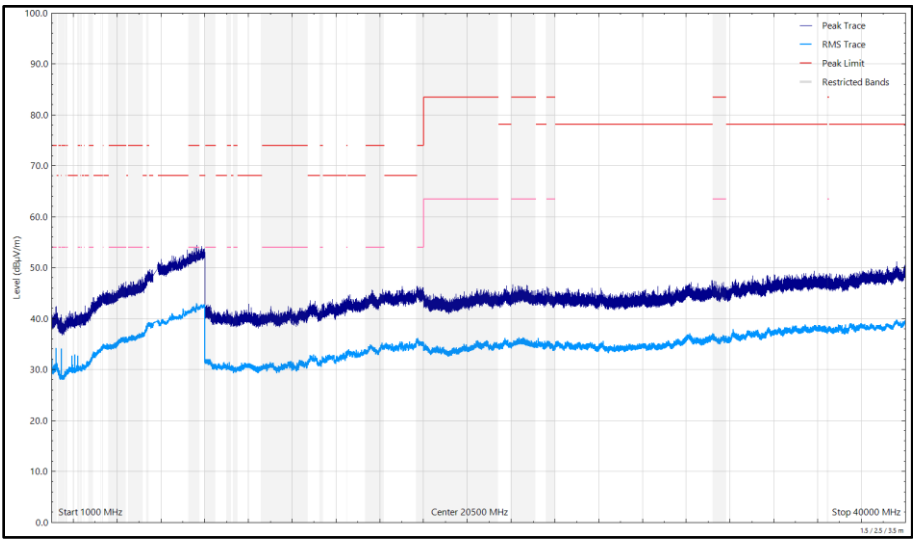
Figure 673 - U-NII-3 - 5745 MHz (CH149), 802.11a, Core 1, 1 GHz to 40 GHz, Horizontal
