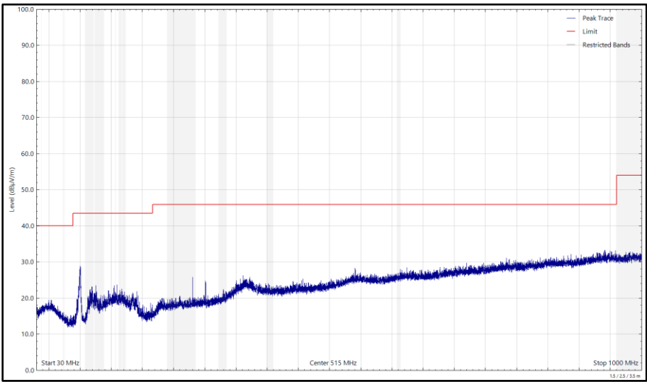
Figure 675 - U-NII-3 - 5825 MHz (CH165), 802.11a, Core 1, 30 MHz to 1 GHz, Horizontal (Peak)
