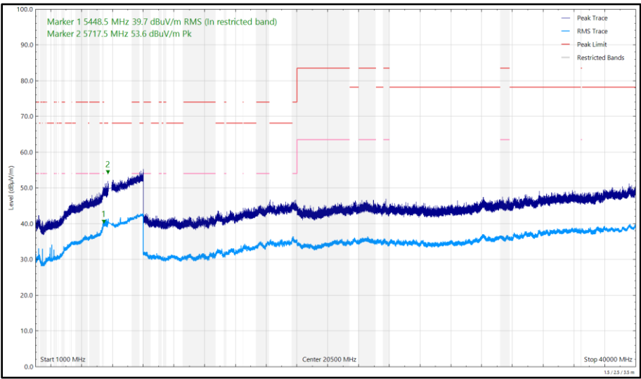
Figure 692 - U-NII-3 - 5825 MHz (CH165), HT20, CDD, Core 0 + Core 1, 1 GHz to 40 GHz, Horizontal
