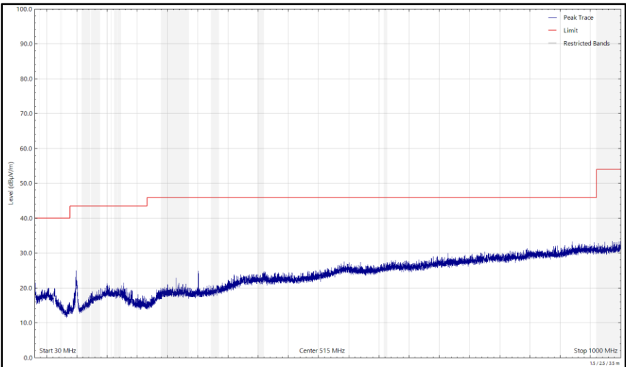
Figure 709 - U-NII-3 - 5825 MHz (CH165), HE20, RU26-0, CDD, Core 0 + Core 1, 30 MHz to 1 GHz, Vertical (Peak)
