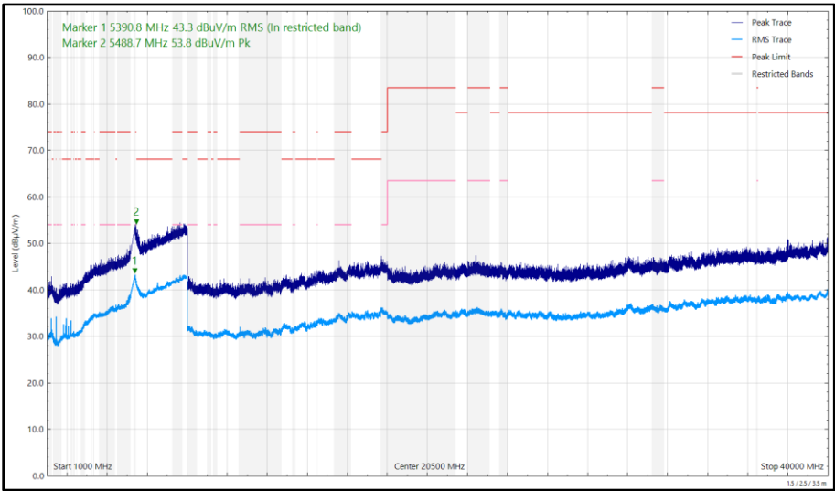
Figure 683 - U-NII-2A - 5320 MHz (CH64), HT20, CDD, Core 0 + Core 1, 1 GHz to 40 GHz, Horizontal
