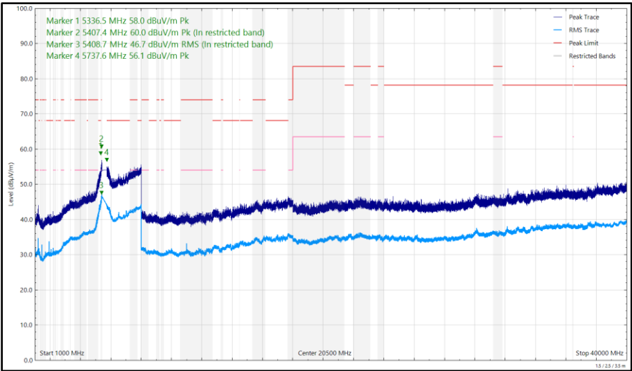
Figure 702 - U-NII-2C - 5500 MHz (CH100), HE20, RU52-37, CDD, Core 0 + Core 1, 1 GHz to 40 GHz, Vertical
