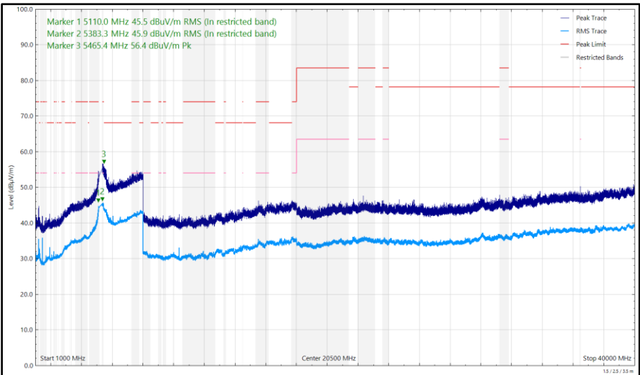
Figure 698 - U-NII-1 - 5180 MHz (CH36), HE20, RU26-0, CDD, Core 0 + Core 1, 1 GHz to 40 GHz, Vertical
