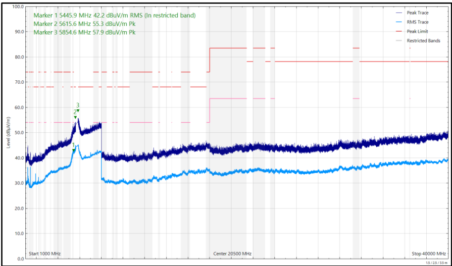
Figure 674 - U-NII-3 - 5745 MHz (CH149), 802.11a, Core 1, 1 GHz to 40 GHz, Vertical
