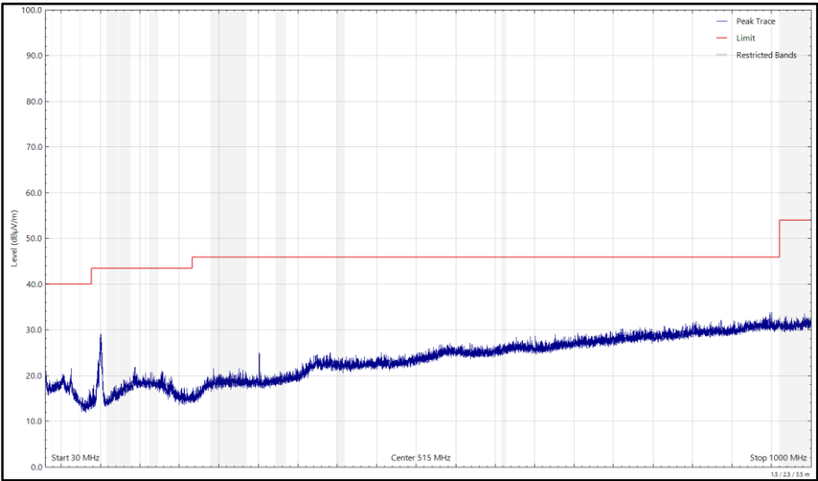
Figure 681 - U-NII-1 - 5180 MHz (CH36), HT20, CDD, Core 0 + Core 1, 30 MHz to 1 GHz, Vertical (Peak)
