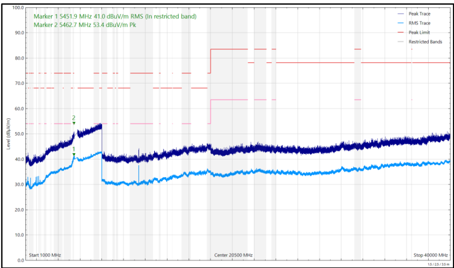
Figure 703 - U-NII-2C - 5700 MHz (CH140), HE20, RU52-37, CDD, Core 0 + Core 1, 1 GHz to 40 GHz, Horizontal
