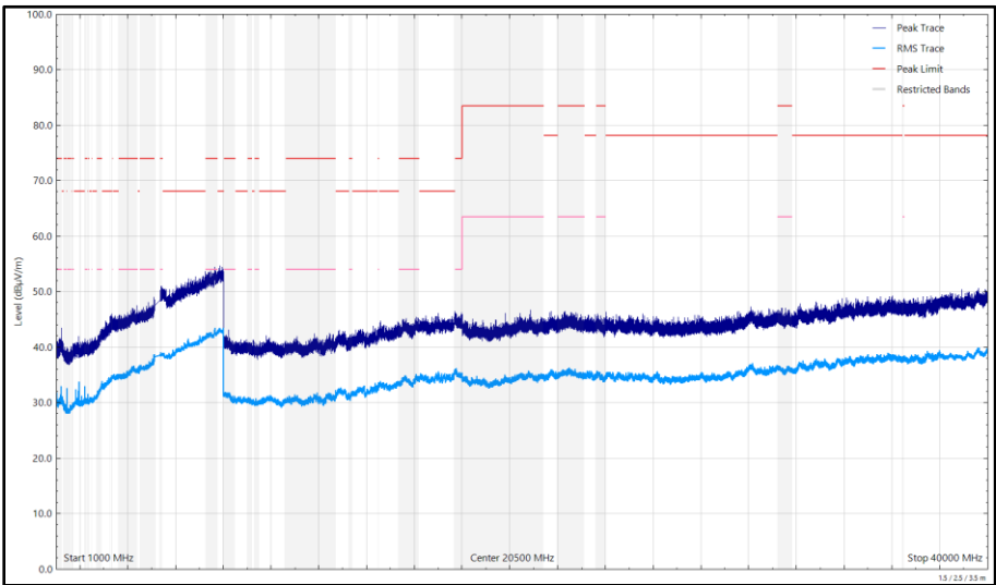
Figure 664 - U-NII-1 - 5180 MHz (CH36), 802.11a, Core 1, 1 GHz to 40 GHz, Horizontal
