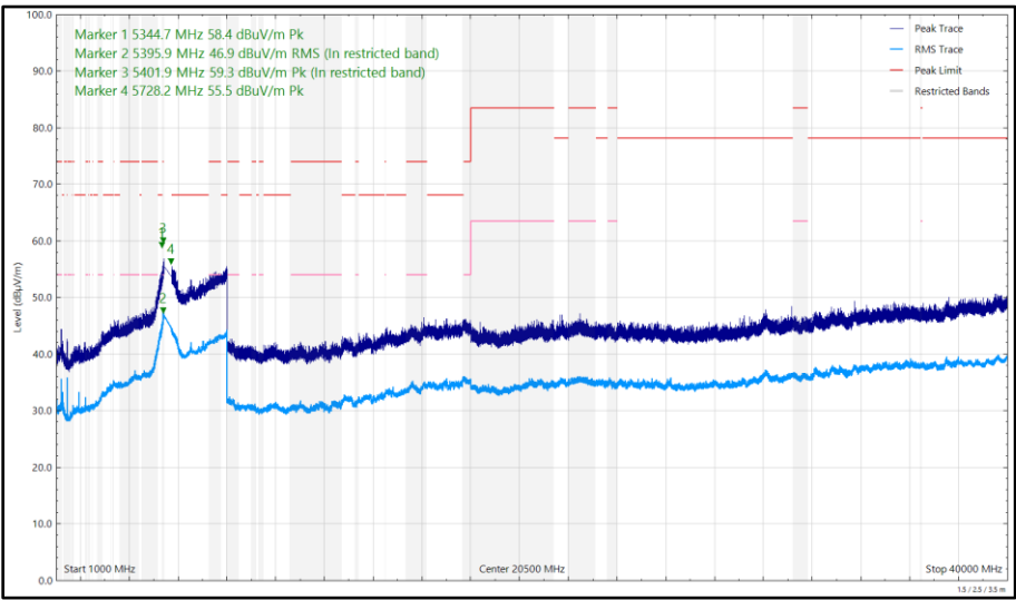
Figure 686 - U-NII-2C - 5500 MHz (CH100), HT20, CDD, Core 0 + Core 1, 1 GHz to 40 GHz, Vertical
