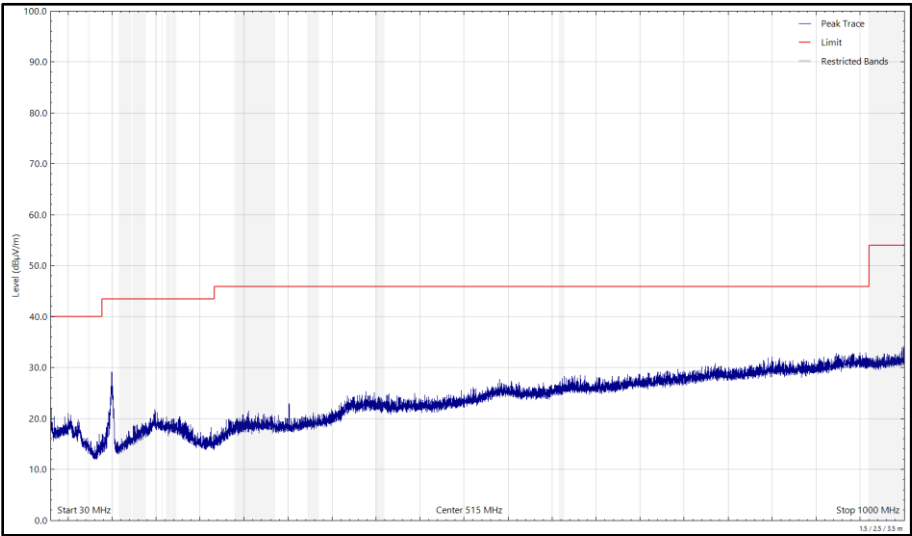
Figure 677 - U-NII-3 - 5825 MHz (CH165), 802.11a, Core 1, 30 MHz to 1 GHz, Vertical (Peak)
