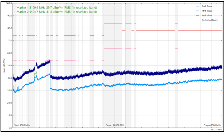
Figure 680 - U-NII-1 - 5180 MHz (CH36), HT20, CDD, Core 0 + Core 1, 1 GHz to 40 GHz, Horizontal
