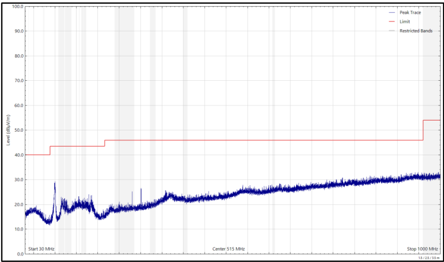
Figure 663 - U-NII-1 - 5180 MHz (CH36), 802.11a, Core 1, 30 MHz to 1 GHz, Horizontal (Peak)
