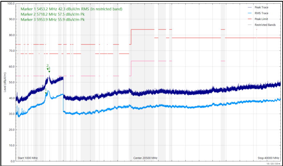
Figure 662 - U-NII-3 - 5825 MHz (CH165), 802.11a, Core 0, 1 GHz to 40 GHz, Vertical
