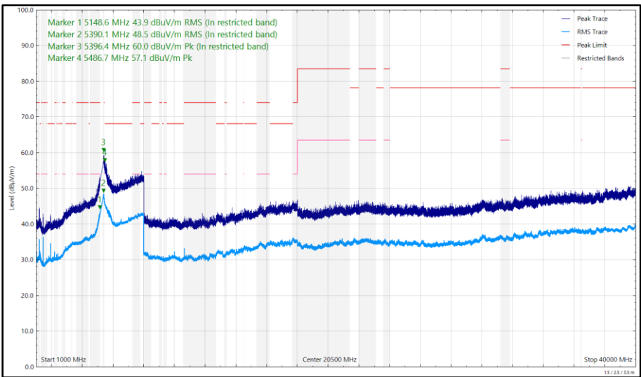
Figure 684 - U-NII-2A - 5320 MHz (CH64), HT20, CDD, Core 0 + Core 1, 1 GHz to 40 GHz, Vertical
