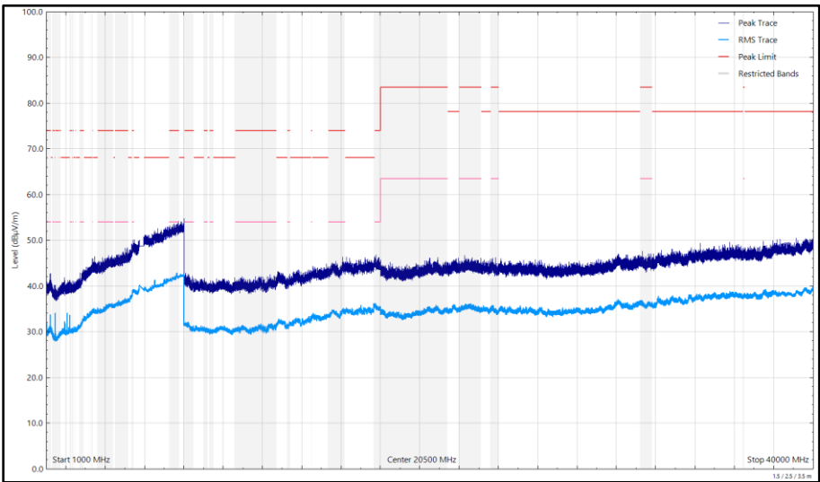
Figure 676 - U-NII-3 - 5825 MHz (CH165), 802.11a, Core 1, 1 GHz to 40 GHz, Horizontal
