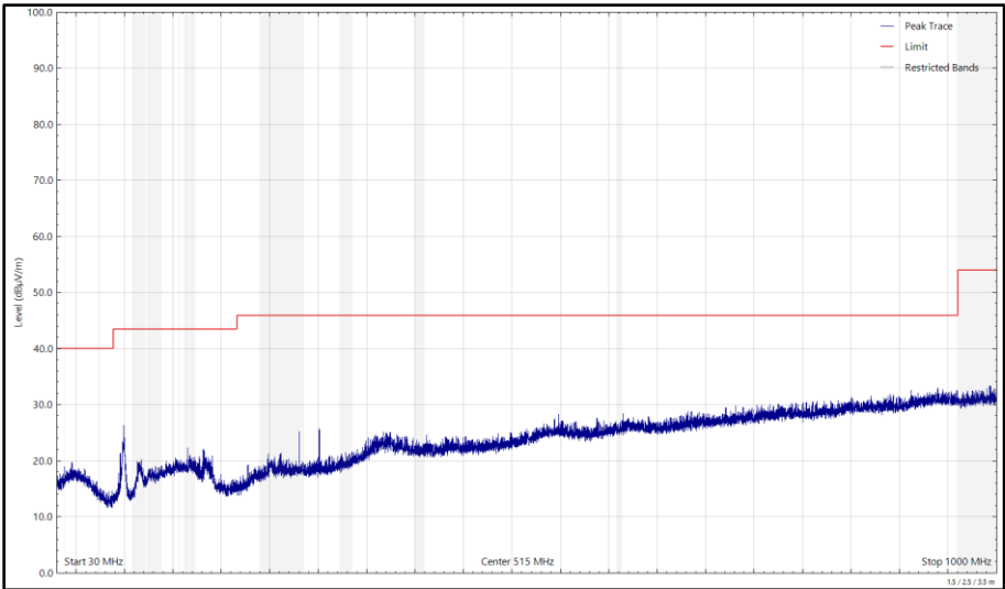
Figure 707 - U-NII-3 - 5825 MHz (CH165), HE20, RU26-0, CDD, Core 0 + Core 1, 30 MHz to 1 GHz, Horizontal (Peak)
