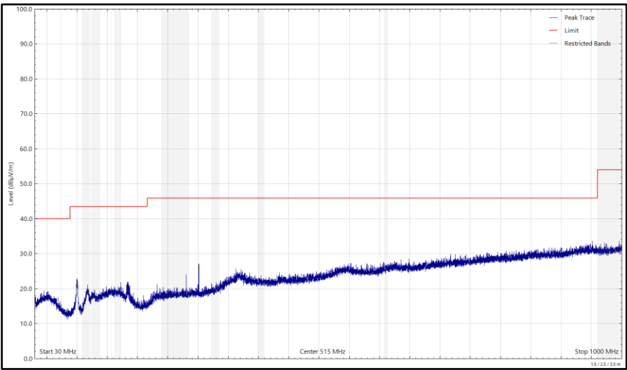
Figure 691 - U-NII-3 - 5825 MHz (CH165), HT20, CDD, Core 0 + Core 1, 30 MHz to 1 GHz, Horizontal (Peak)
