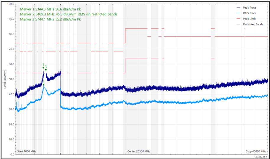
Figure 670 - U-NII-2C - 5500 MHz (CH100), 802.11a, Core 1, 1 GHz to 40 GHz, Vertical
