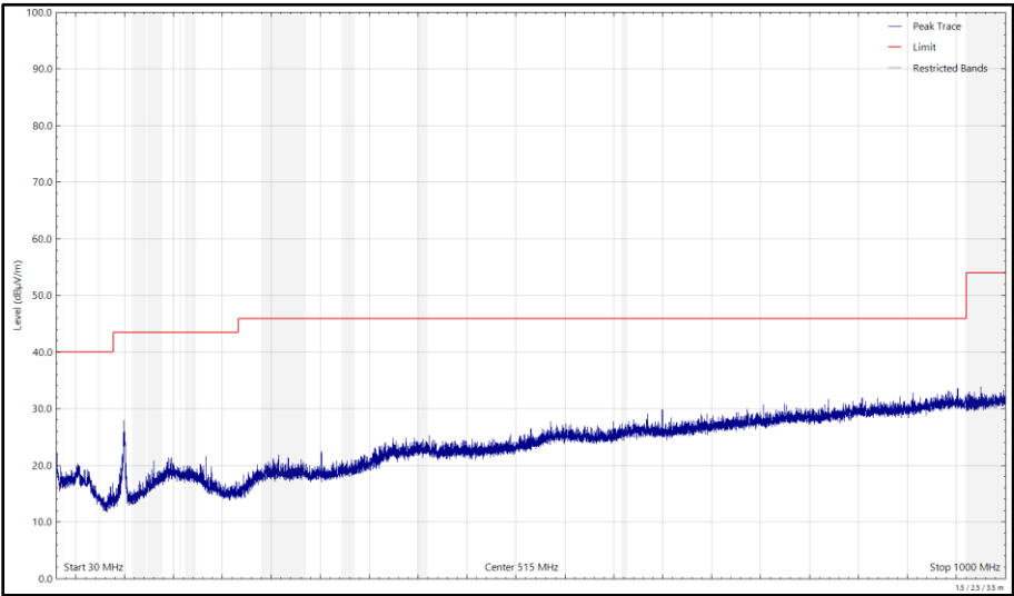
Figure 661 - U-NII-3 - 5825 MHz (CH165), 802.11a, Core 0, 30 MHz to 1 GHz, Vertical (Peak)
