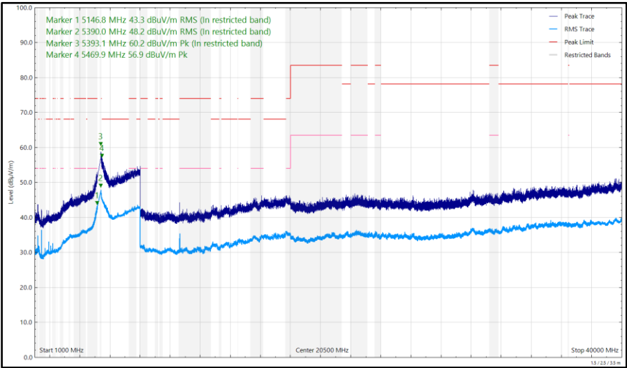
Figure 700 - U-NII-2A - 5320 MHz (CH64), HE20, RU52-37, CDD, Core 0 + Core 1, 1 GHz to 40 GHz, Vertical
