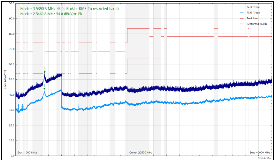
Figure 699 - U-NII-2A - 5320 MHz (CH64), HE20, RU52-37, CDD, Core 0 + Core 1, 1 GHz to 40 GHz, Horizontal
