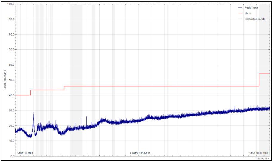
Figure 679 - U-NII-1 - 5180 MHz (CH36), HT20, CDD, Core 0 + Core 1, 30 MHz to 1 GHz, Horizontal (Peak)
