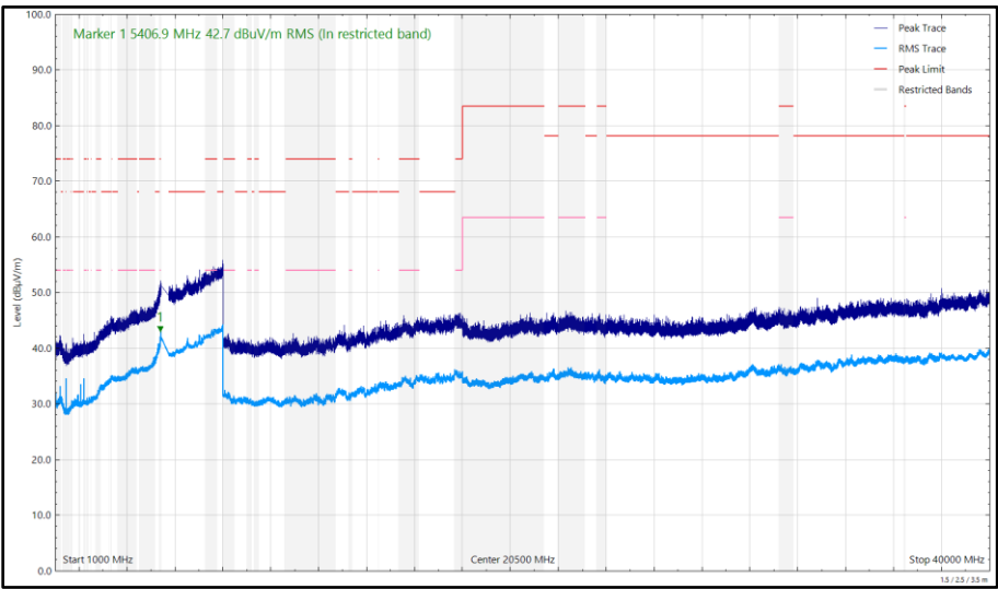
Figure 685 - U-NII-2C - 5500 MHz (CH100), HT20, CDD, Core 0 + Core 1, 1 GHz to 40 GHz, Horizontal
