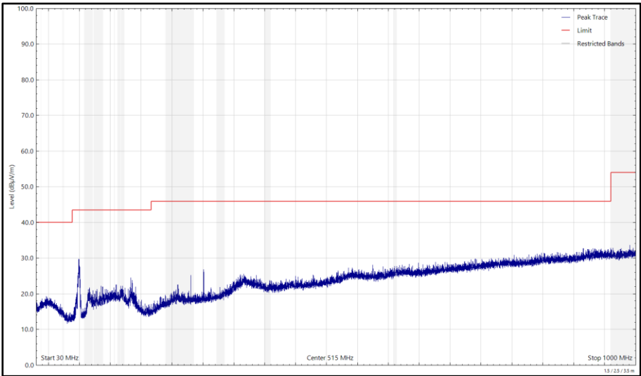
Figure 695 - U-NII-1 - 5180 MHz (CH36), HE20, RU26-0, CDD, Core 0 + Core 1, 30 MHz to 1 GHz, Horizontal (Peak)
