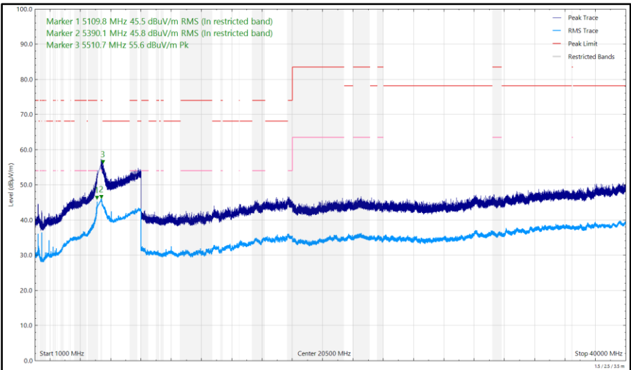
Figure 682 - U-NII-1 - 5180 MHz (CH36), HT20, CDD, Core 0 + Core 1, 1 GHz to 40 GHz, Vertical
