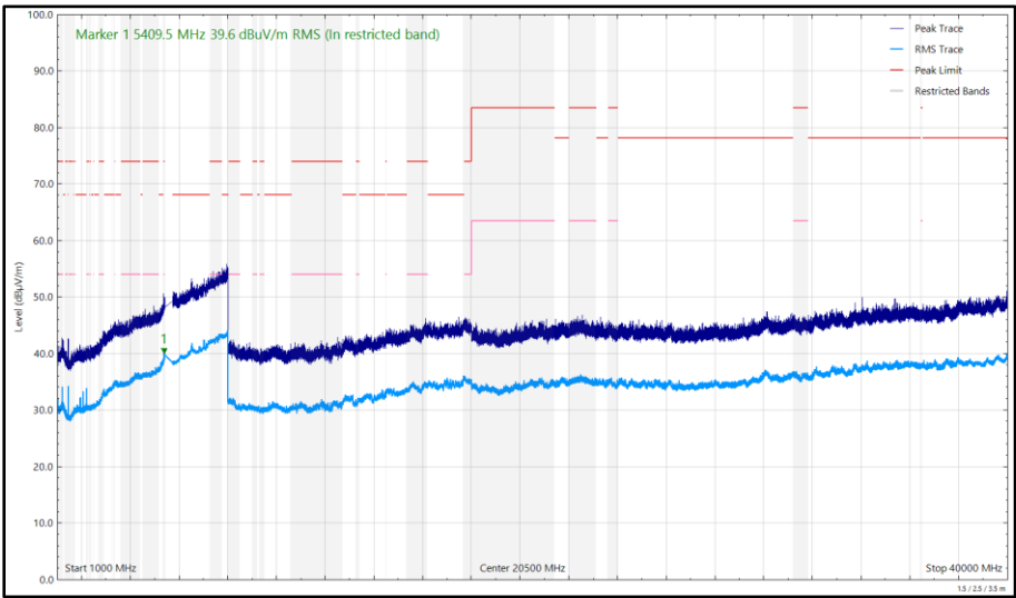
Figure 669 - U-NII-2C - 5500 MHz (CH100), 802.11a, Core 1, 1 GHz to 40 GHz, Horizontal
