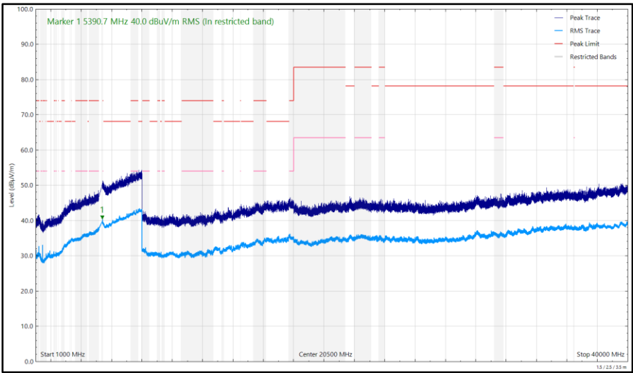
Figure 667 - U-NII-2A - 5320 MHz (CH64), 802.11a, Core 1, 1 GHz to 40 GHz, Horizontal
