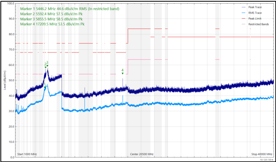
Figure 706 - U-NII-3 - 5745 MHz (CH149), HE20, RU26-0, CDD, Core 0 + Core 1, 1 GHz to 40 GHz, Vertical
