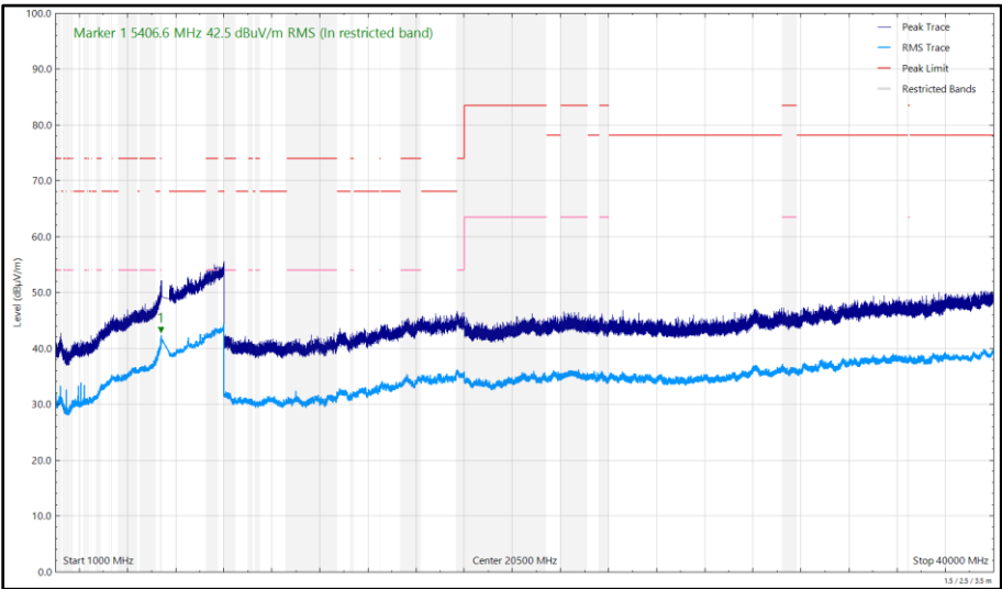
Figure 701 - U-NII-2C - 5500 MHz (CH100), HE20, RU52-37, CDD, Core 0 + Core 1, 1 GHz to 40 GHz, Horizontal
