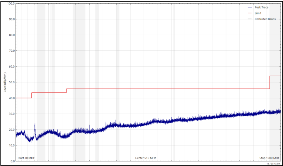
Figure 693 - U-NII-3 - 5825 MHz (CH165), HT20, CDD, Core 0 + Core 1, 30 MHz to 1 GHz, Vertical (Peak)
