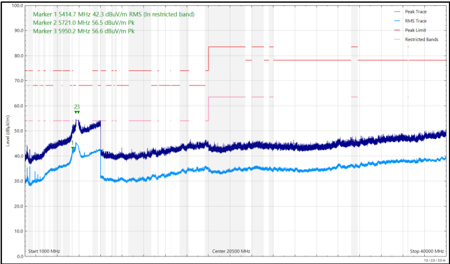
Figure 678 - U-NII-3 - 5825 MHz (CH165), 802.11a, Core 1, 1 GHz to 40 GHz, Vertical
