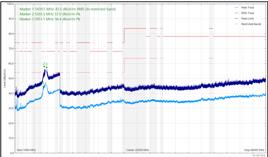
Figure 694 - U-NII-3 - 5825 MHz (CH165), HT20, CDD, Core 0 + Core 1, 1 GHz to 40 GHz, Vertical
