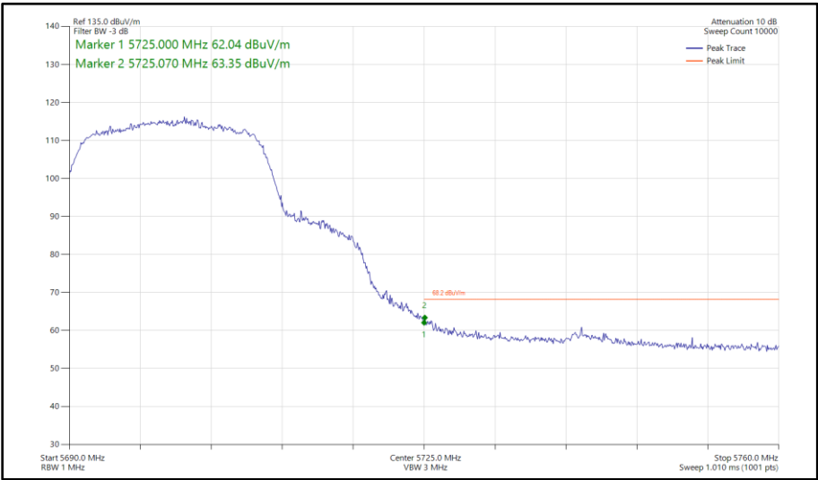
Figure 360 - 802.11n HT20, SISO, Core 0 - 5700 MHz Band Edge Frequency 5725 MHz
