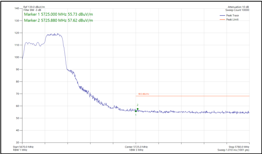
Figure 396 - 802.11ax HE20, RU 106-54, SISO, Core 1 - 5680 MHz Band Edge Frequency 5725 MHz
