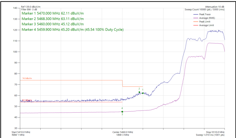
Figure 381 - 802.11ax HE20, RU 106-54, SISO, Core 1 - 5500 MHz Band Edge Frequency 5470 MHz
