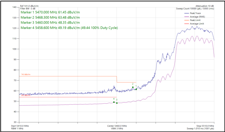
Figure 410 - 802.11n HT20, CDD, Core 0 - Core 1 - 5500 MHz Band Edge Frequency 5470 MHz
