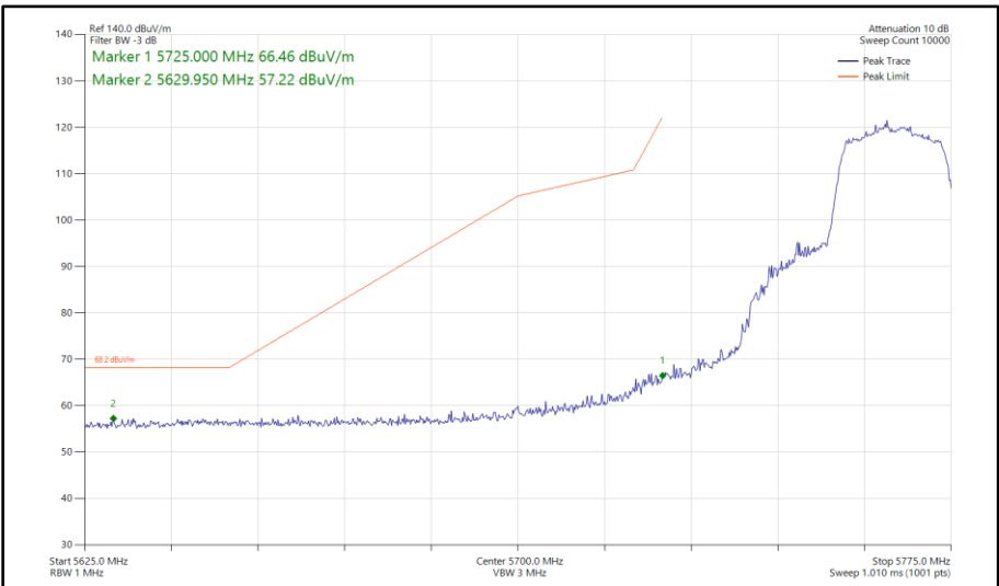
Figure 387 - 802.11n HT20, SISO, Core 1 - 5765 MHz Band Edge Frequency 5725 MHz
