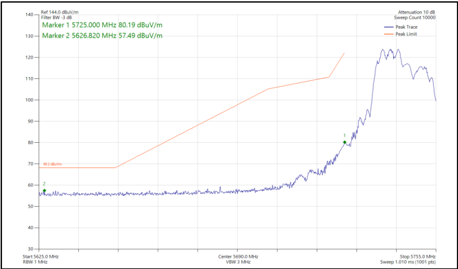
Figure 419 - 802.11ax HE20, RU 106-53, CDD, Core 0 - Core 1 - 5745 MHz Band Edge Frequency 5725 MHz
