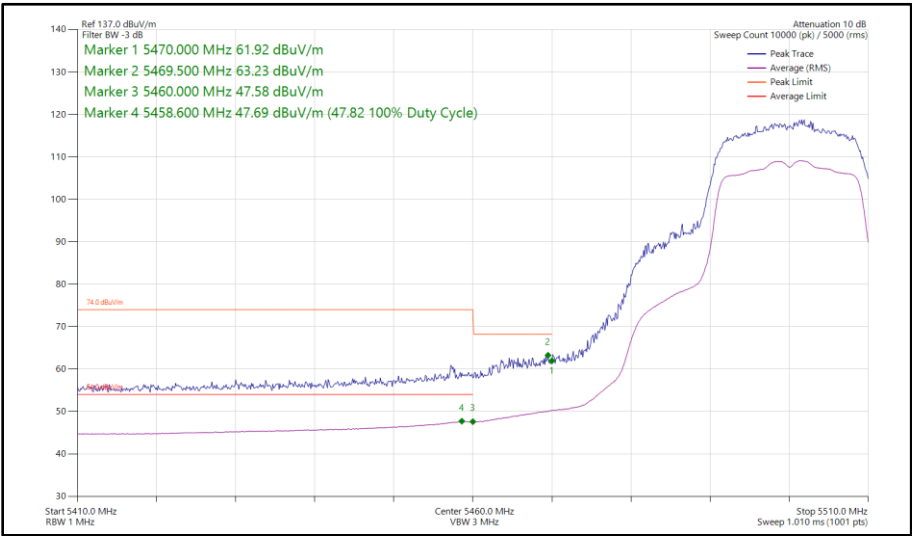
Figure 378 - 802.11n HT20, SISO, Core 1 - 5500 MHz Band Edge Frequency 5470 MHz
