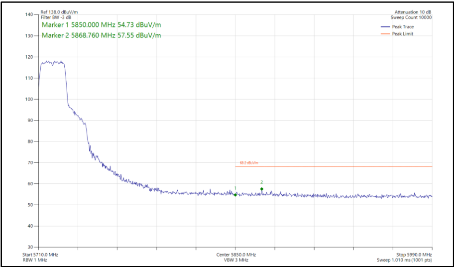
Figure 368 - 802.11n HT20, SISO, Core 0 - 5720 MHz Band Edge Frequency 5850 MHz
