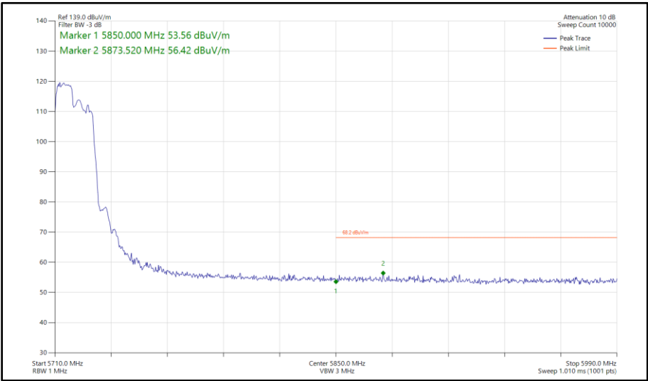
Figure 372 - 802.11ax HE20, RU 106-53, SISO, Core 0 - 5720 MHz Band Edge Frequency 5850 MHz
