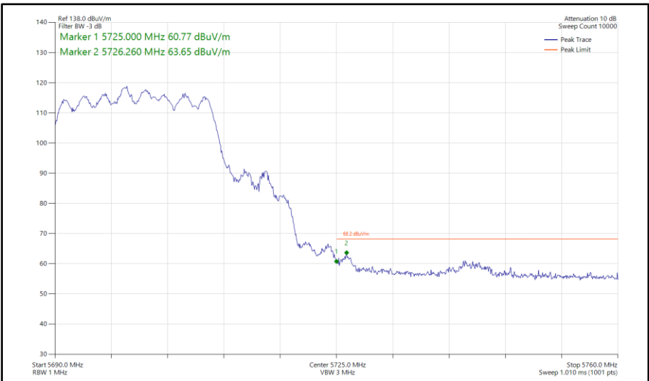
Figure 425 - 802.11ax HE20, SU, CDD, Core 0 - Core 1 - 5700 MHz Band Edge Frequency 5725 MHz
