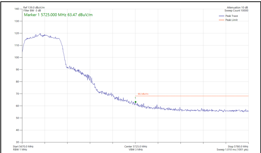
Figure 393 - 802.11n HT20, SISO, Core 1 - 5680 MHz Band Edge Frequency 5725 MHz
