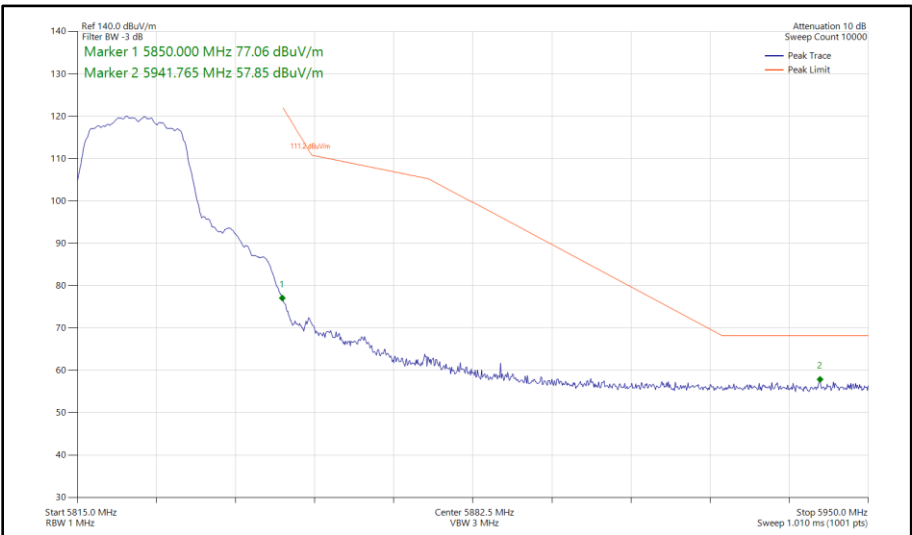
Figure 401 - 802.11a, SISO, Core 1 - 5825 MHz Band Edge Frequency 5850 MHz
