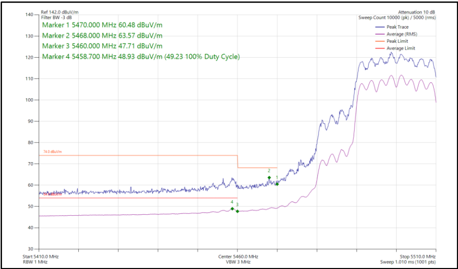
Figure 412 - 802.11ax HE20, SU, CDD, Core 0 - Core 1 - 5500 MHz Band Edge Frequency 5470 MHz
