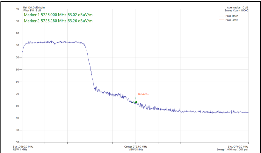
Figure 397 - 802.11ax HE20, SU, SISO, Core 1 - 5700 MHz Band Edge Frequency 5725 MHz
