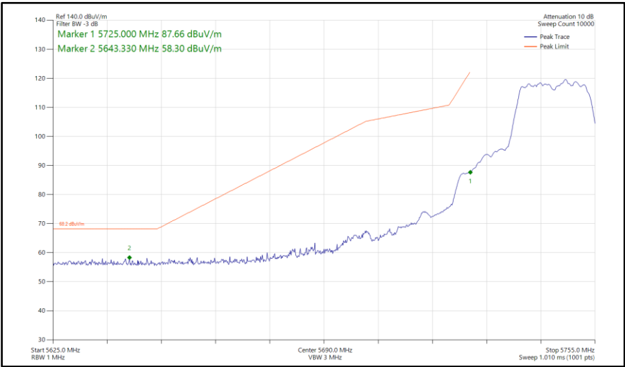
Figure 384 - 802.11a, SISO, Core 1 - 5745 MHz Band Edge Frequency 5725 MHz
