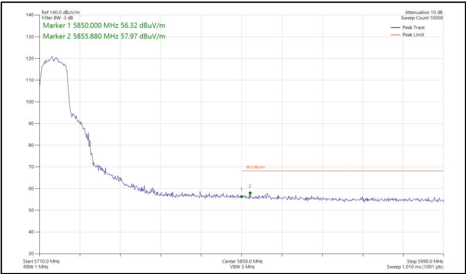
Figure 402 - 802.11n HT20, SISO, Core 1 - 5720 MHz Band Edge Frequency 5850 MHz
