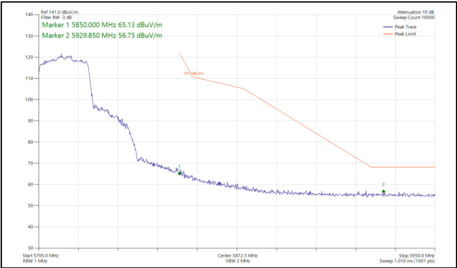
Figure 373 - 802.11ax HE20, SU, SISO, Core 0 - 5805 MHz Band Edge Frequency 5850 MHz
