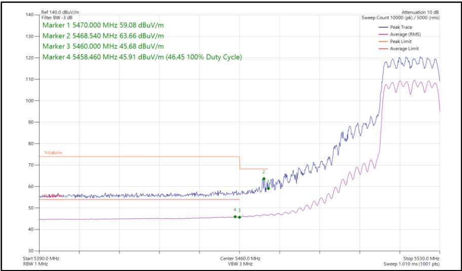
Figure 414 - 802.11ax HE20, SU, CDD, Core 0 - Core 1 - 5520 MHz Band Edge Frequency 5470 MHz
