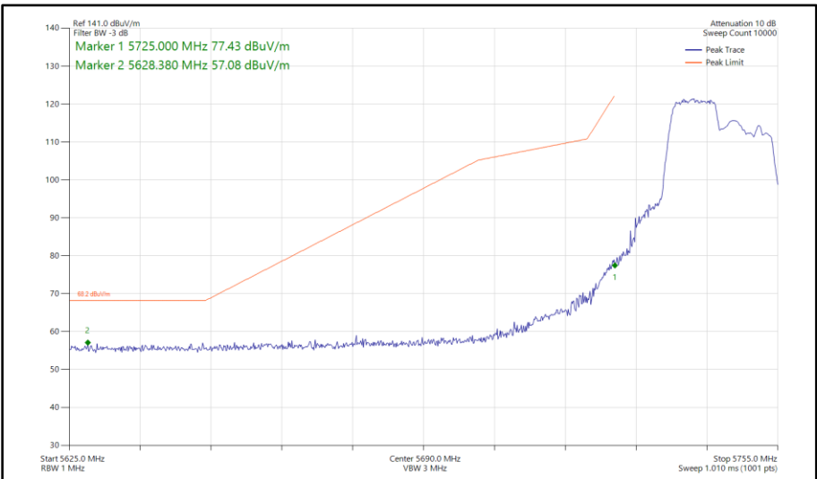
Figure 389 - 802.11ax HE20, RU 106-53, SISO, Core 1 - 5745 MHz Band Edge Frequency 5725 MHz
