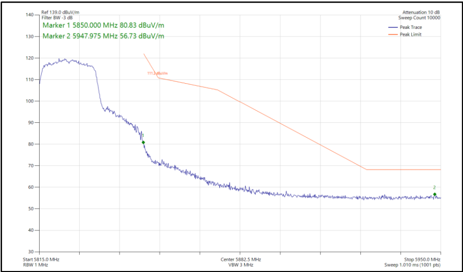
Figure 370 - 802.11n HT20, SISO, Core 0 - 5825 MHz Band Edge Frequency 5850 MHz
