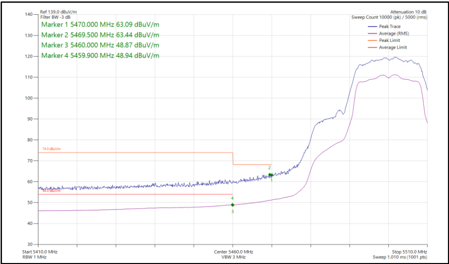
Figure 376 - 802.11a, SISO, Core 1 - 5500 MHz Band Edge Frequency 5470 MHz
