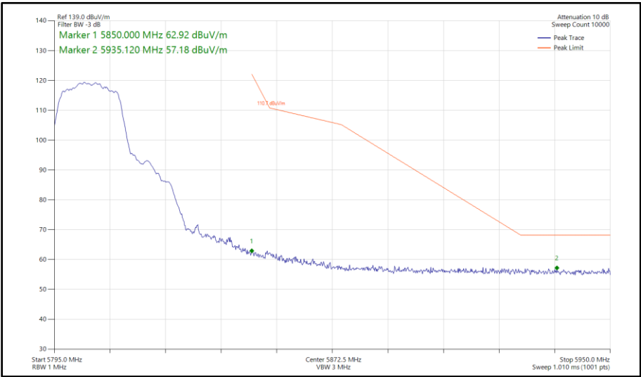
Figure 400 - 802.11a, SISO, Core 1 - 5805 MHz Band Edge Frequency 5850 MHz
