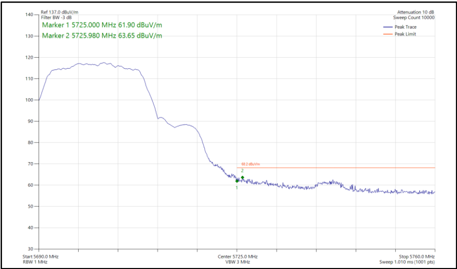
Figure 392 - 802.11a, SISO, Core 1 - 5700 MHz Band Edge Frequency 5725 MHz
