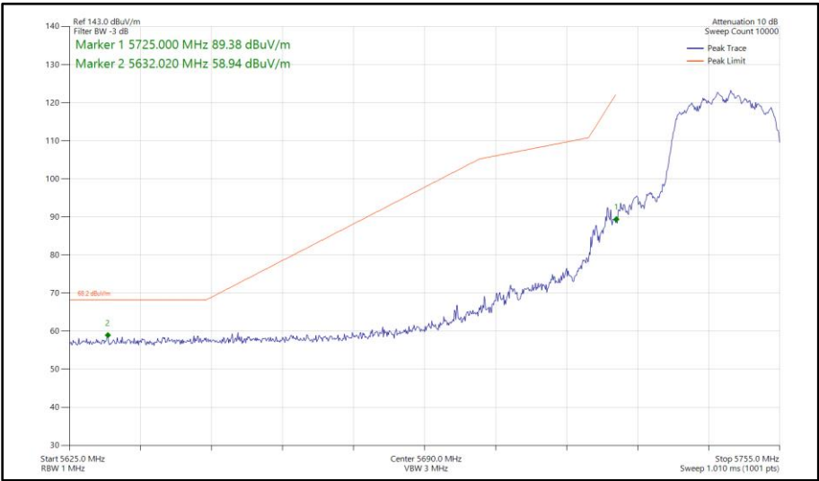
Figure 416 - 802.11n HT20, CDD, Core 0 - Core 1 - 5745 MHz Band Edge Frequency 5725 MHz
