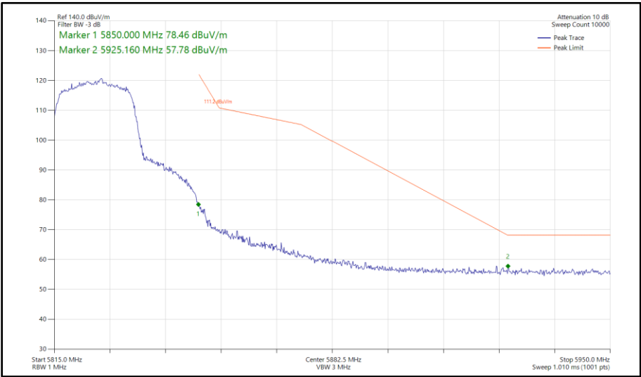
Figure 404 - 802.11n HT20, SISO, Core 1 - 5825 MHz Band Edge Frequency 5850 MHz
