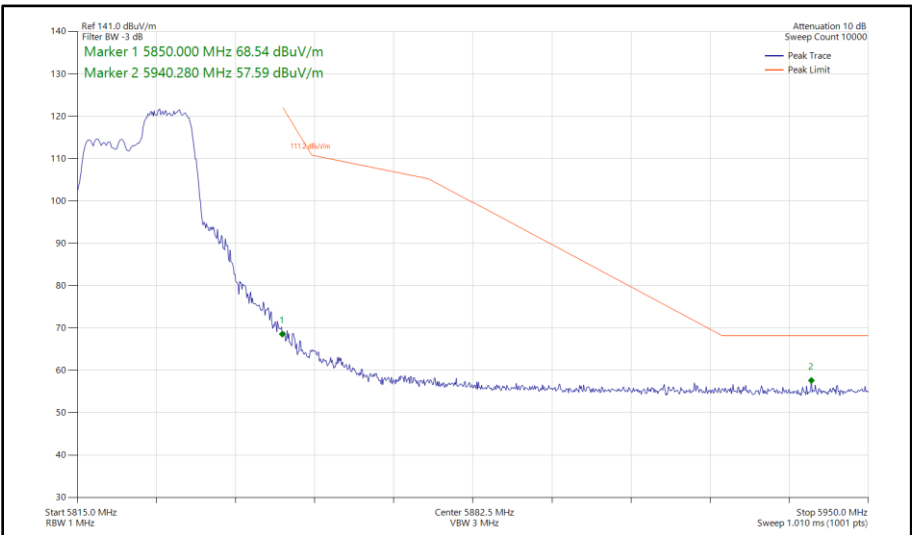
Figure 409 - 802.11ax HE20, RU 106-54, SISO, Core 1 - 5825 MHz Band Edge Frequency 5850 MHz
