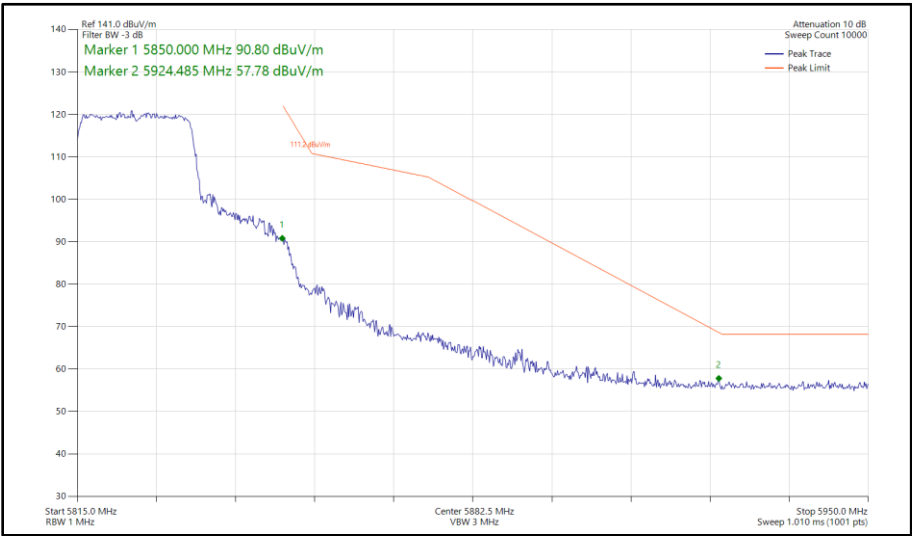
Figure 408 - 802.11ax HE20, SU, SISO, Core 1 - 5825 MHz Band Edge Frequency 5850 MHz
