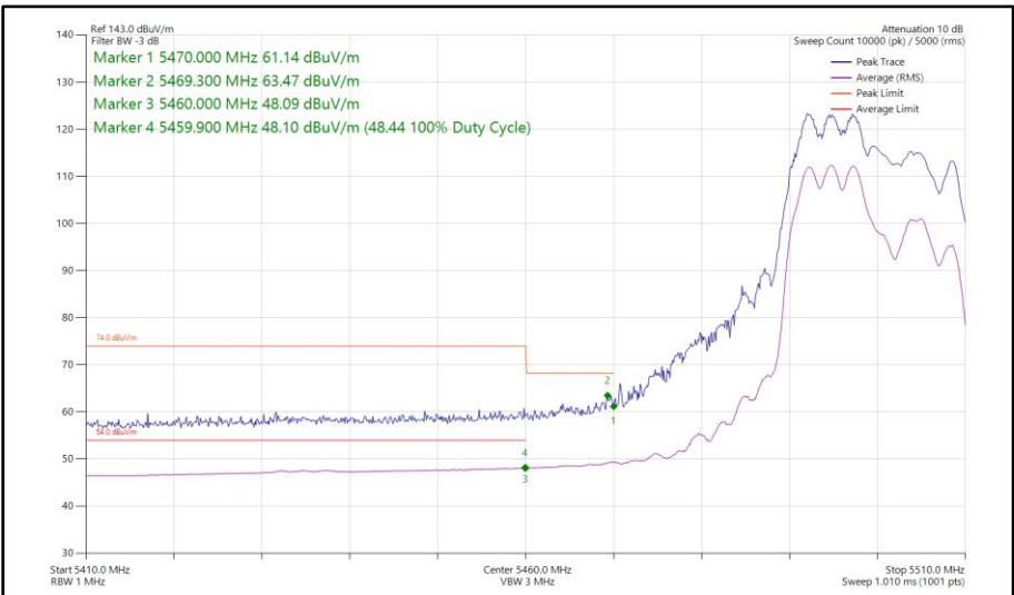
Figure 413 - 802.11ax HE20, RU 106-53, CDD, Core 0 - Core 1 - 5500 MHz Band Edge Frequency 5470 MHz
