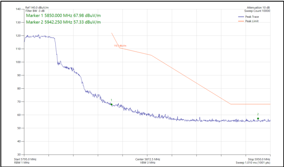
Figure 407 - 802.11ax HE20, SU, SISO, Core 1 - 5805 MHz Band Edge Frequency 5850 MHz
