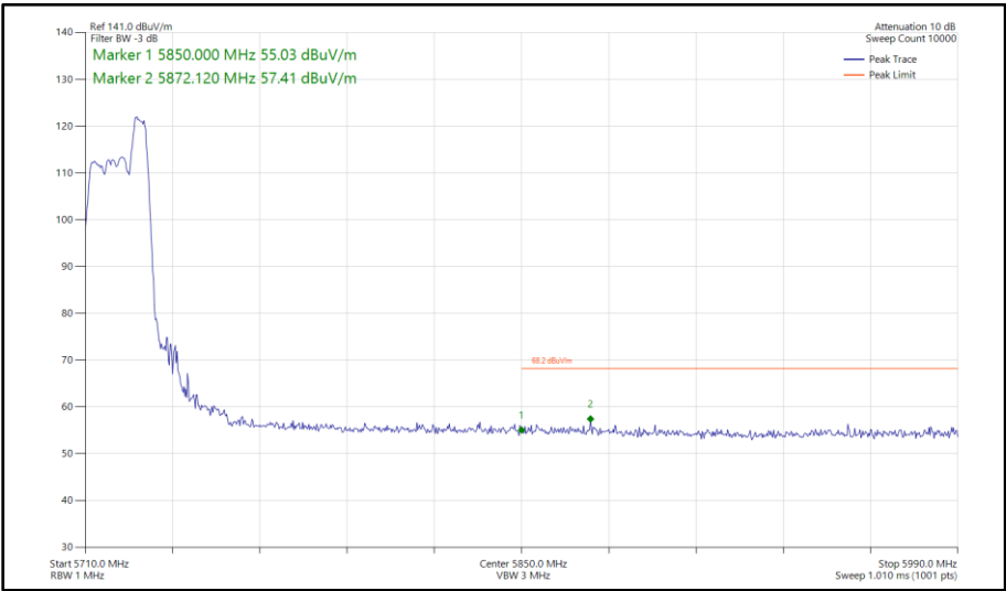
Figure 406 - 802.11ax HE20, RU 52-40, SISO, Core 1 - 5720 MHz Band Edge Frequency 5850 MHz
