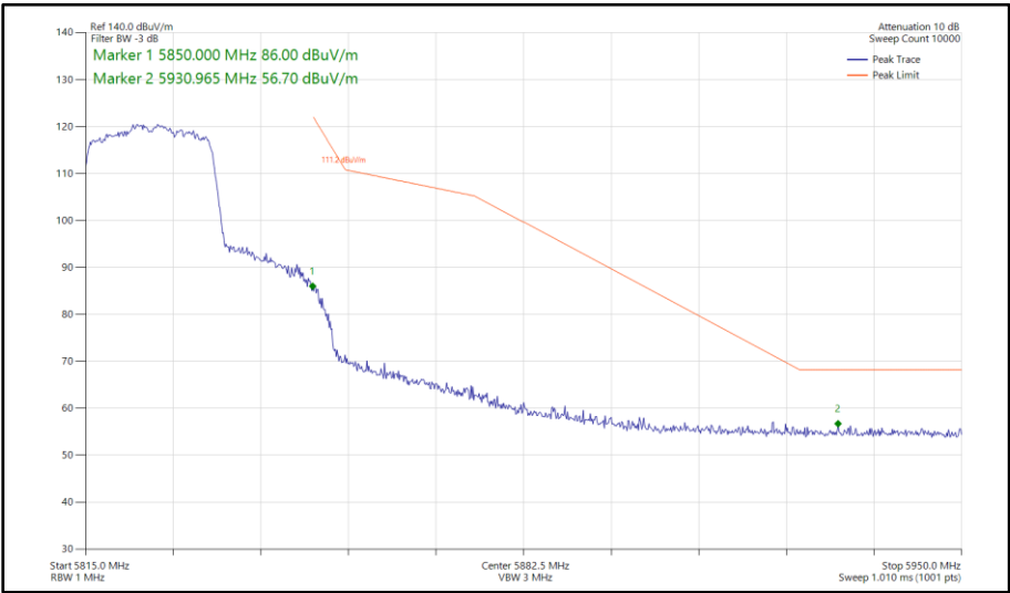
Figure 374 - 802.11ax HE20, SU, SISO, Core 0 - 5825 MHz Band Edge Frequency 5850 MHz
