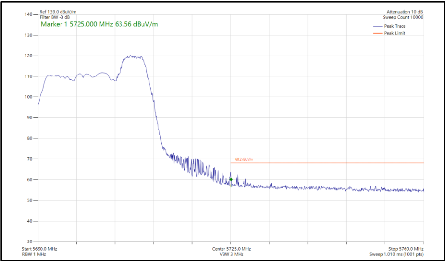
Figure 398 - 802.11ax HE20, RU 52-40, SISO, Core 1 - 5700 MHz Band Edge Frequency 5725 MHz
