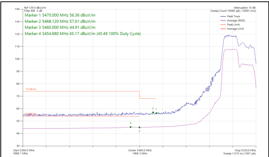
Figure 383 - 802.11ax HE20, RU 106-53, SISO, Core 1 - 5520 MHz Band Edge Frequency 5470 MHz
