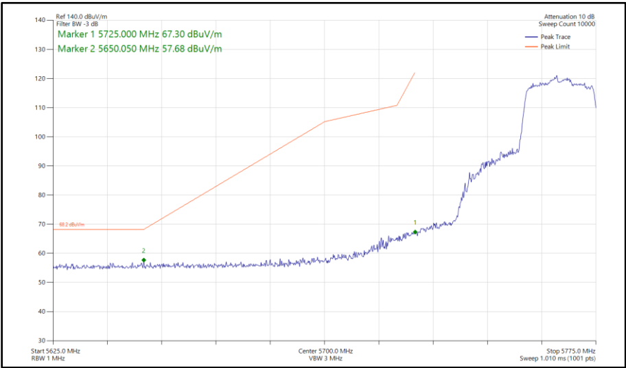
Figure 390 - 802.11ax HE20, SU, SISO, Core 1 - 5765 MHz Band Edge Frequency 5725 MHz
