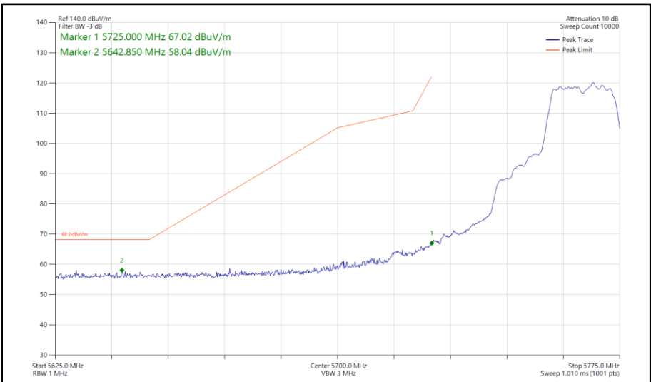
Figure 385 - 802.11a, SISO, Core 1 - 5765 MHz Band Edge Frequency 5725 MHz
