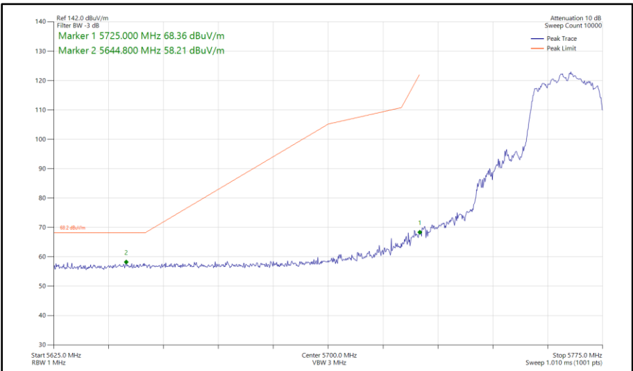
Figure 417 - 802.11n HT20, CDD, Core 0 - Core 1 - 5765 MHz Band Edge Frequency 5725 MHz
