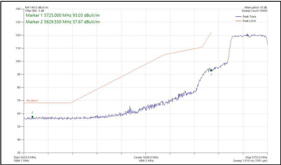
Figure 388 - 802.11ax HE20, SU, SISO, Core 1 - 5745 MHz Band Edge Frequency 5725 MHz
