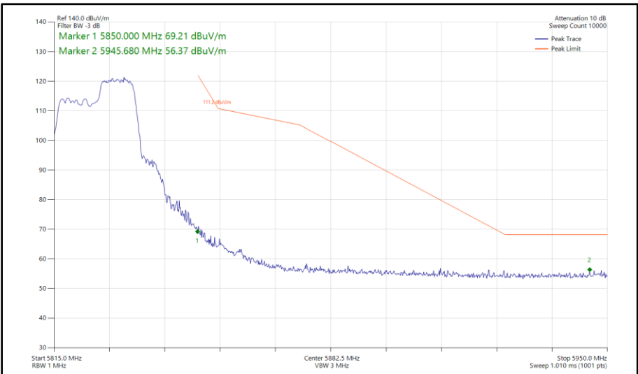
Figure 375 - 802.11ax HE20, RU 106-54, SISO, Core 0 - 5825 MHz Band Edge Frequency 5850 MHz
