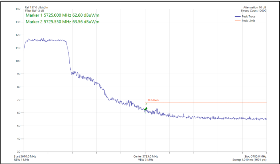
Figure 395 - 802.11ax HE20, SU, SISO, Core 1 - 5680 MHz Band Edge Frequency 5725 MHz
