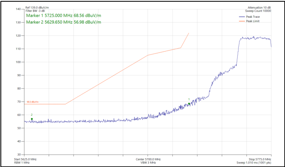
Figure 356 - 802.11ax HE20, SU, SISO, Core 0 - 5765 MHz Band Edge Frequency 5725 MHz
