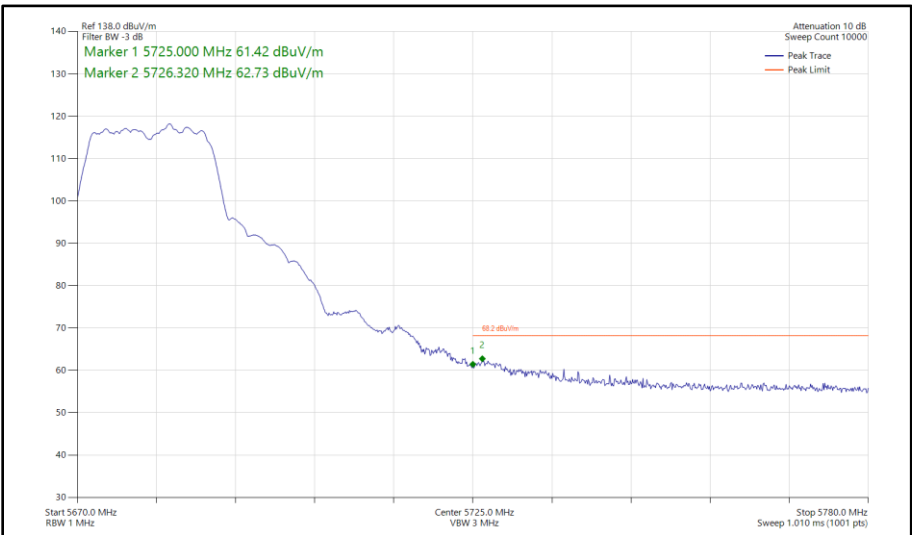
Figure 391 - 802.11a, SISO, Core 1 - 5680 MHz Band Edge Frequency 5725 MHz
