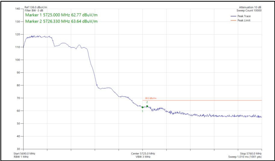
Figure 364 - 802.11ax HE20, RU 106-53, SISO, Core 0 - 5700 MHz Band Edge Frequency 5725 MHz
