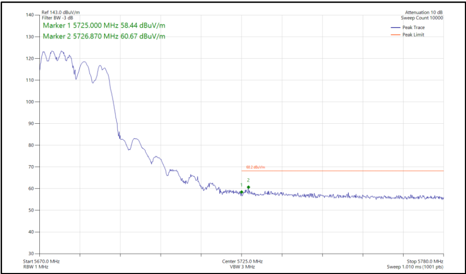
Figure 424 - 802.11ax HE20, RU 106-53, CDD, Core 0 - Core 1 - 5680 MHz Band Edge Frequency 5725 MHz
