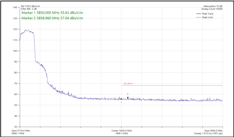
Figure 371 - 802.11ax HE20, SU, SISO, Core 0 - 5720 MHz Band Edge Frequency 5850 MHz
