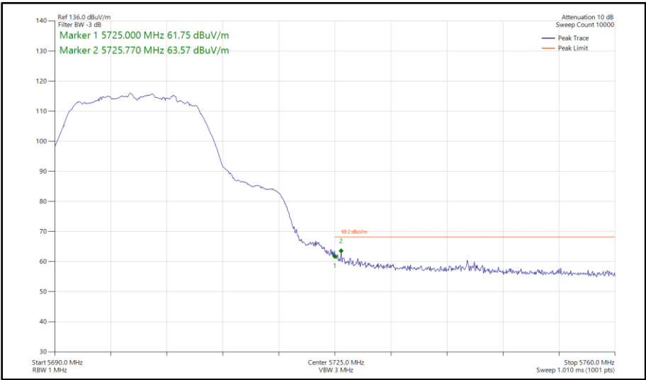
Figure 358 - 802.11a, SISO, Core 0 - 5700 MHz Band Edge Frequency 5725 MHz
