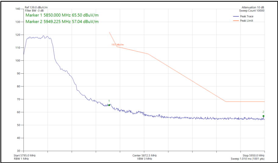
Figure 366 - 802.11a, SISO, Core 0 - 5805 MHz Band Edge Frequency 5850 MHz
