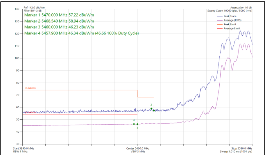
Figure 415 - 802.11ax HE20, RU 106-54, CDD, Core 0 - Core 1 - 5520 MHz Band Edge Frequency 5470 MHz
