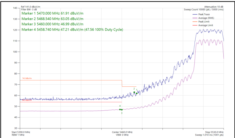
Figure 411 - 802.11n HT20, CDD, Core 0 - Core 1 - 5520 MHz Band Edge Frequency 5470 MHz
