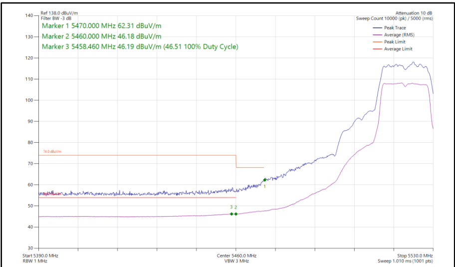
Figure 377 - 802.11a, SISO, Core 1 - 5520 MHz Band Edge Frequency 5470 MHz
