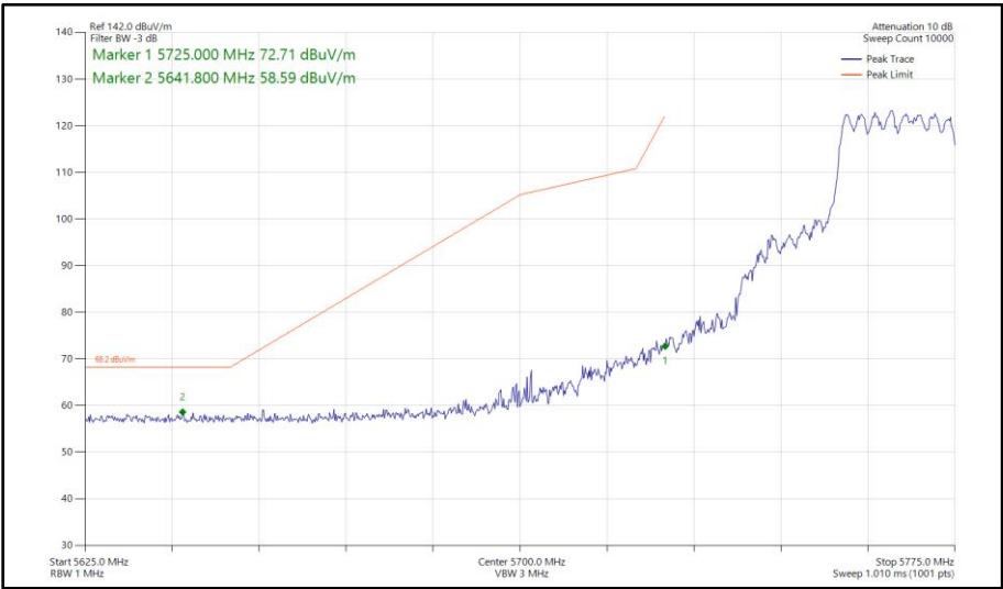
Figure 420 - 802.11ax HE20, SU, CDD, Core 0 - Core 1 - 5765 MHz Band Edge Frequency 5725 MHz
