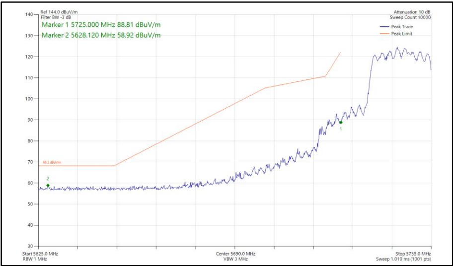
Figure 418 - 802.11ax HE20, SU, CDD, Core 0 - Core 1 - 5745 MHz Band Edge Frequency 5725 MHz
