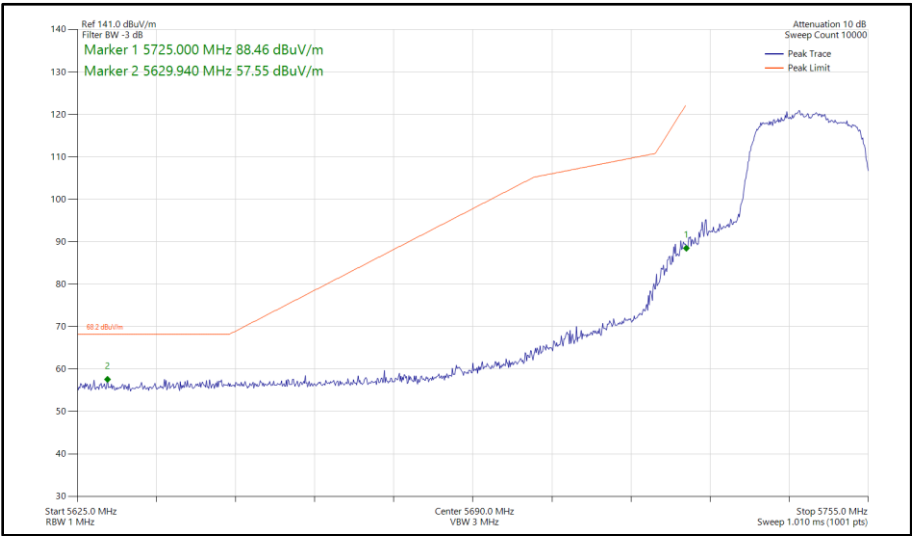
Figure 386 - 802.11n HT20, SISO, Core 1 - 5745 MHz Band Edge Frequency 5725 MHz
