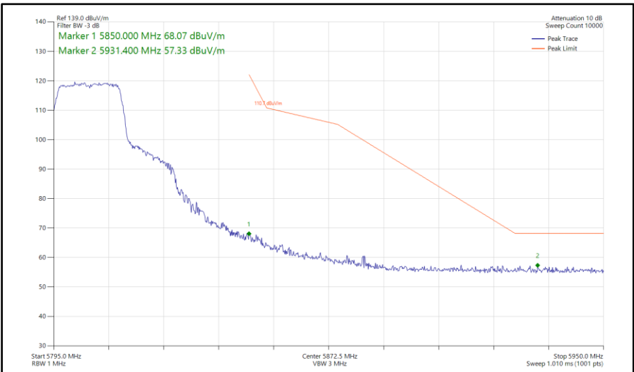
Figure 403 - 802.11n HT20, SISO, Core 1 - 5805 MHz Band Edge Frequency 5850 MHz
