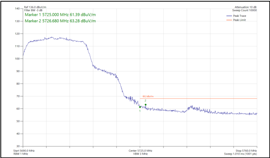
Figure 394 - 802.11n HT20, SISO, Core 1 - 5700 MHz Band Edge Frequency 5725 MHz
