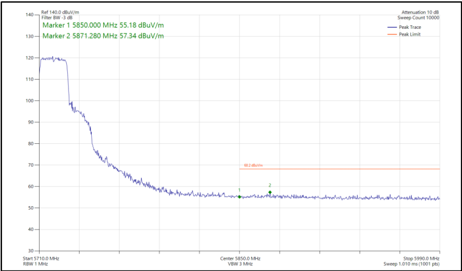
Figure 405 - 802.11ax HE20, SU, SISO, Core 1 - 5720 MHz Band Edge Frequency 5850 MHz
