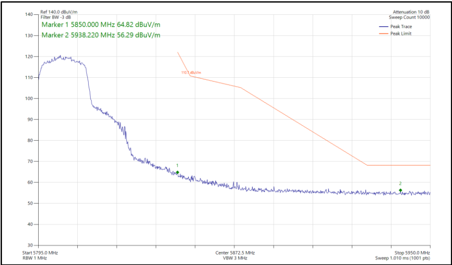
Figure 369 - 802.11n HT20, SISO, Core 0 - 5805 MHz Band Edge Frequency 5850 MHz
