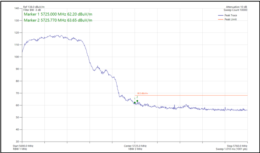
Figure 422 - 802.11n HT20, CDD, Core 0 - Core 1 - 5700 MHz Band Edge Frequency 5725 MHz
