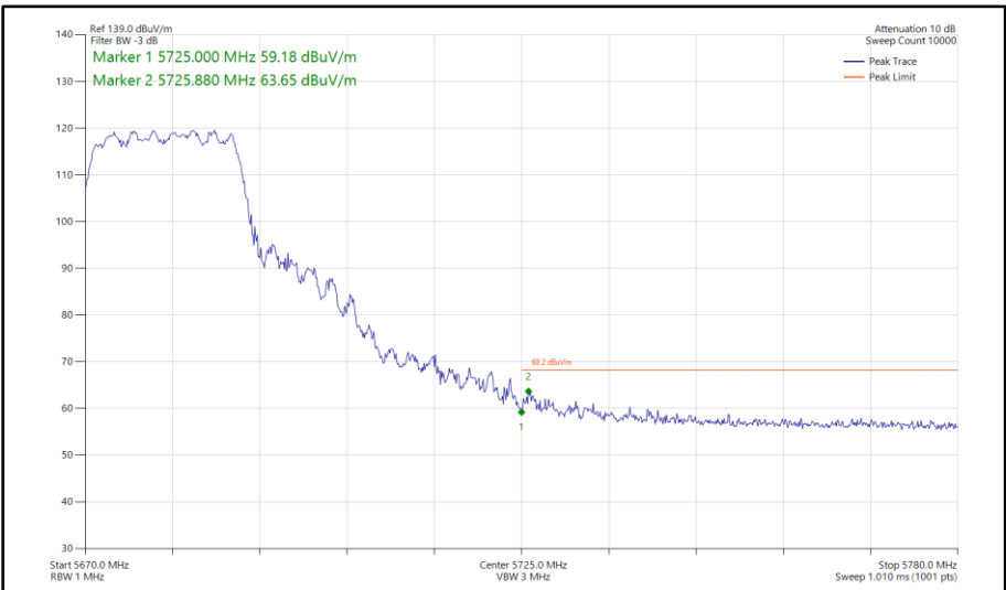
Figure 421 - 802.11n HT20, CDD, Core 0 - Core 1 - 5680 MHz Band Edge Frequency 5725 MHz
