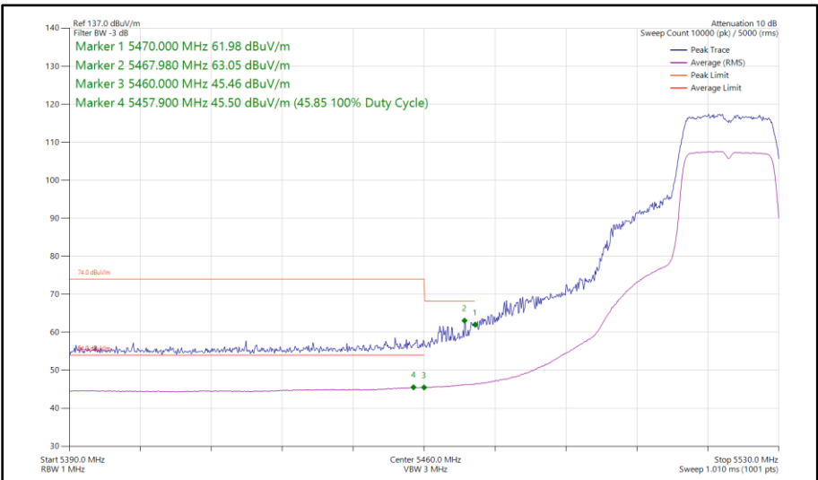
Figure 379 - 802.11n HT20, SISO, Core 1 - 5520 MHz Band Edge Frequency 5470 MHz
