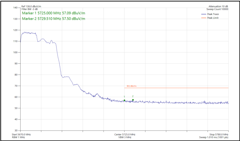
Figure 362 - 802.11ax HE20, RU 106-53, SISO, Core 0 - 5680 MHz Band Edge Frequency 5725 MHz
