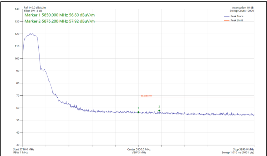
Figure 399 - 802.11a, SISO, Core 1 - 5720 MHz Band Edge Frequency 5850 MHz
