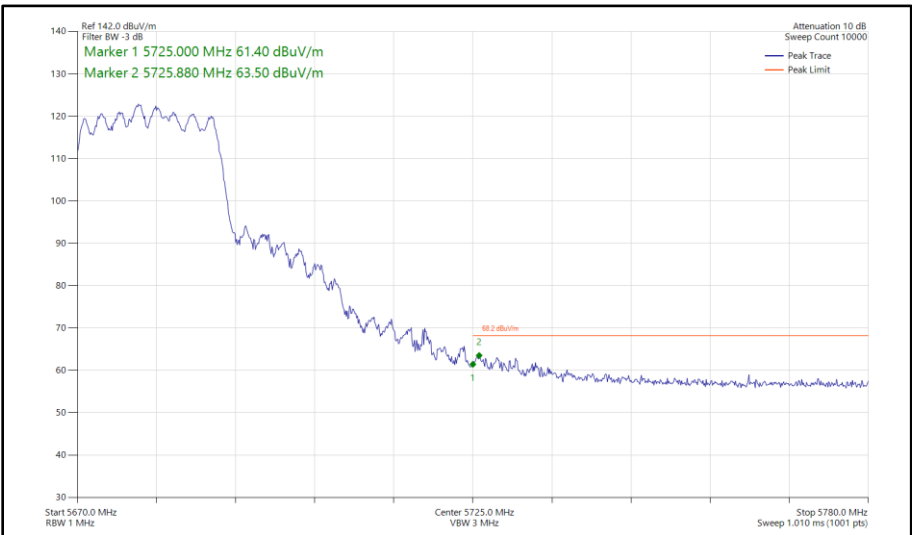
Figure 423 - 802.11ax HE20, SU, CDD, Core 0 - Core 1 - 5680 MHz Band Edge Frequency 5725 MHz
