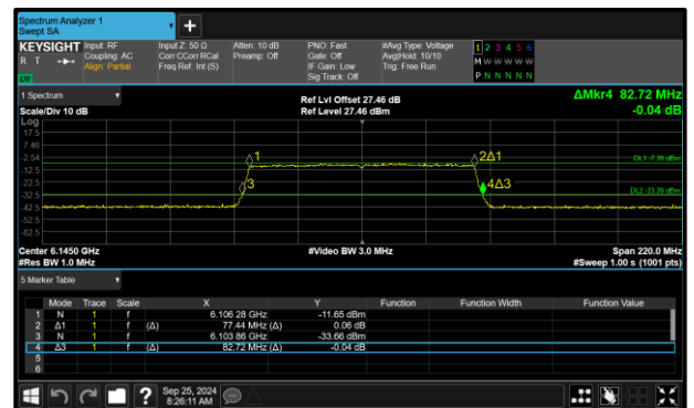
Figure 50 - 802.11ax HE80 SU VLP Maximum 99% OBW
