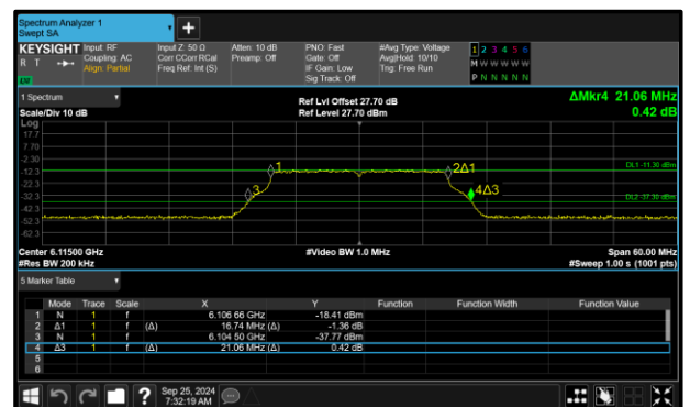
Figure 22 - 802.11a VLP Maximum 99% OBW
