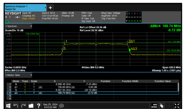
Figure 52 - 802.11ax HE160 SU VLP Maximum 99% OBW
