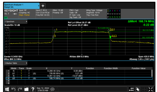
Figure 20 - 802.11ax HE160 SU SP Maximum 99% OBW
