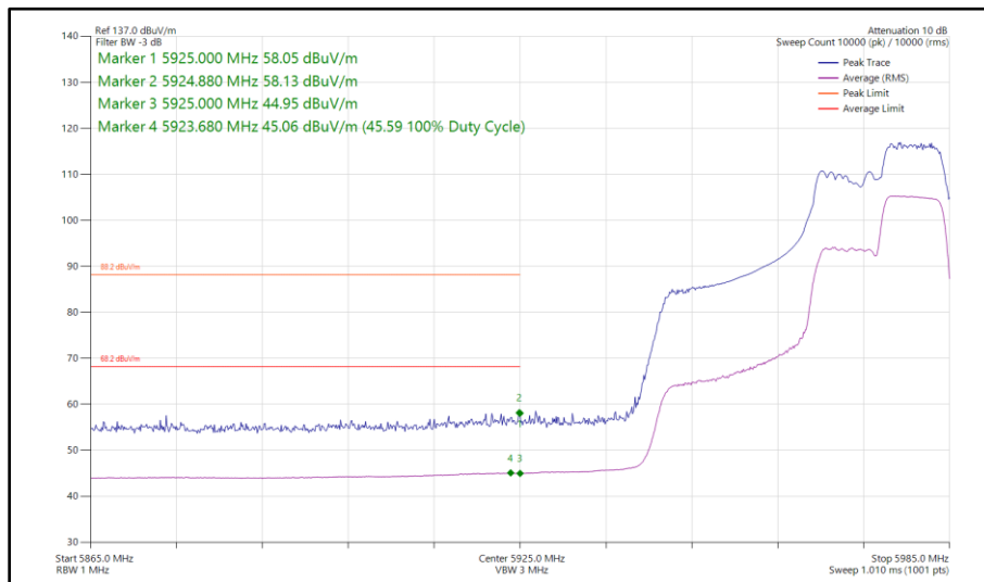
Figure 225 - 802.11ax HE40, RU 106-56, SISO, Core 1 - 5965 MHz Band Edge Frequency 5925 MHz
