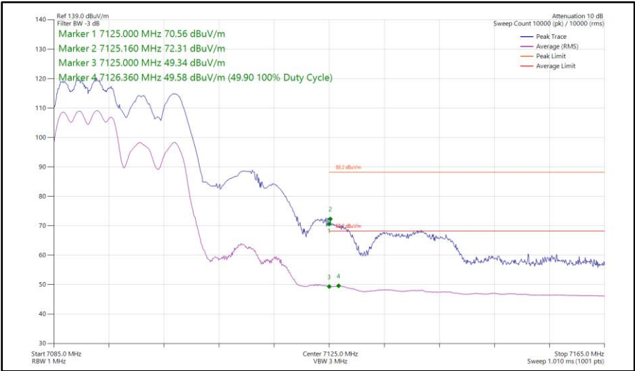
Figure 205 - 802.11ax HE20, RU 106-53, CDD, Core 0 - Core 1 - 7095 MHz Band Edge Frequency 7125 MHz
