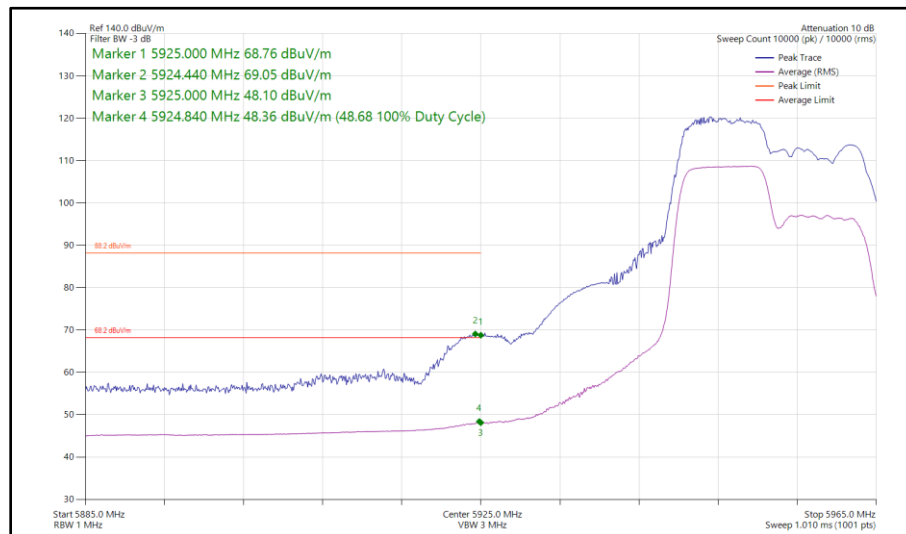
Figure 179 - 802.11ax HE20, RU 106-53, SISO, Core 0 - 5955 MHz Band Edge Frequency 5925 MHz
