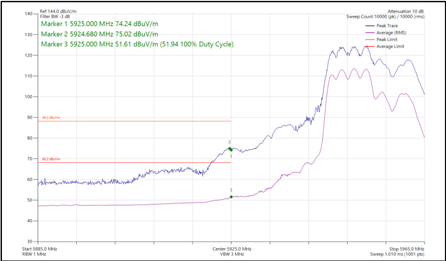
Figure 201 - 802.11ax HE20, RU 106-53, CDD, Core 0 - Core 1 - 5955 MHz Band Edge Frequency 5925 MHz
