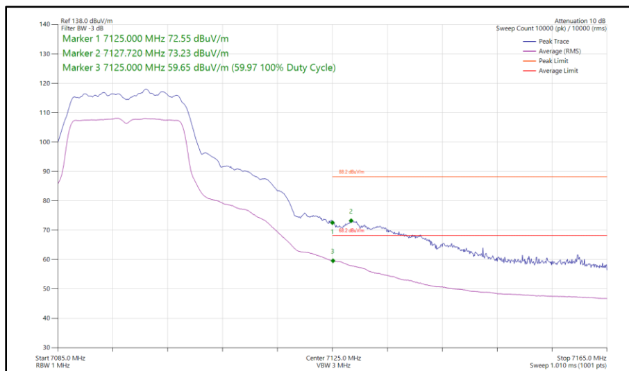
Figure 194 - 802.11a, SISO, Core 1 - 7095 MHz Band Edge Frequency 7125 MHz
