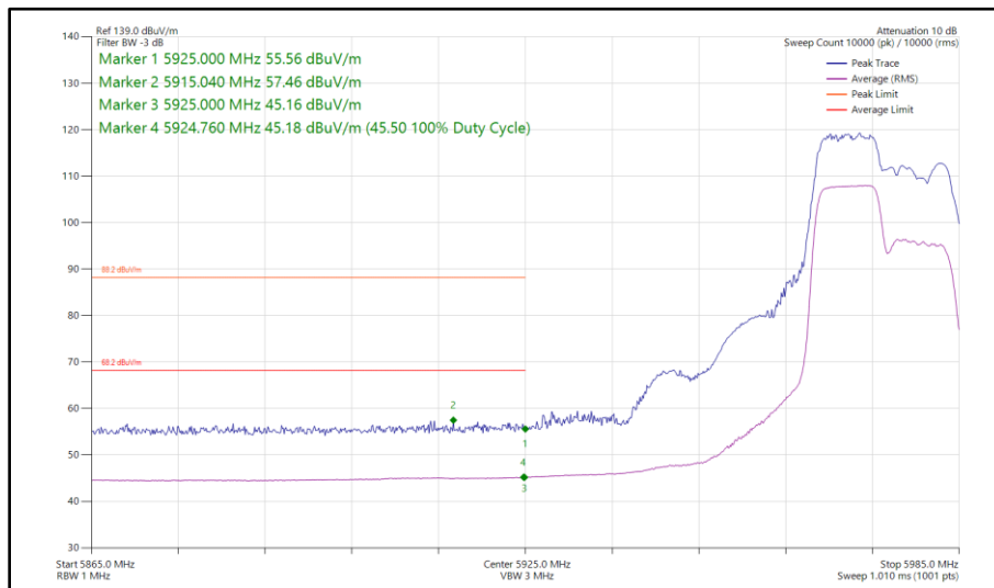
Figure 181 - 802.11ax HE20, RU 106-53, SISO, Core 0 - 5975 MHz Band Edge Frequency 5925 MHz
