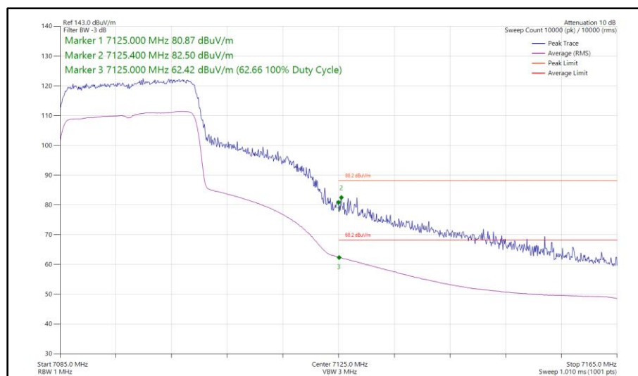
Figure 215 - 802.11ax HE20, SU, TxBF, Core 0 - Core 1 - 7095 MHz Band Edge Frequency 7125 MHz
