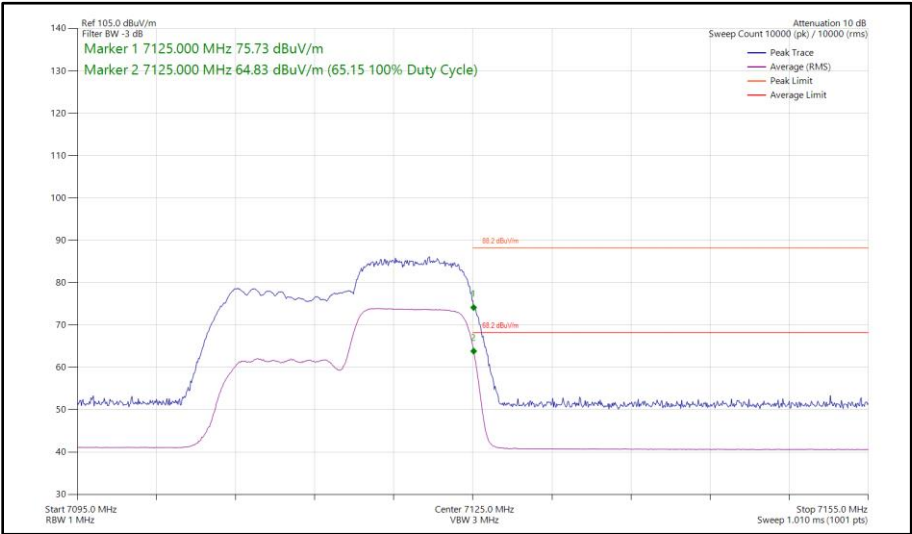
Figure 199 - 802.11ax HE20, RU 106-54, SISO, Core 1 - 7115 MHz Band Edge Frequency 7125 MHz
