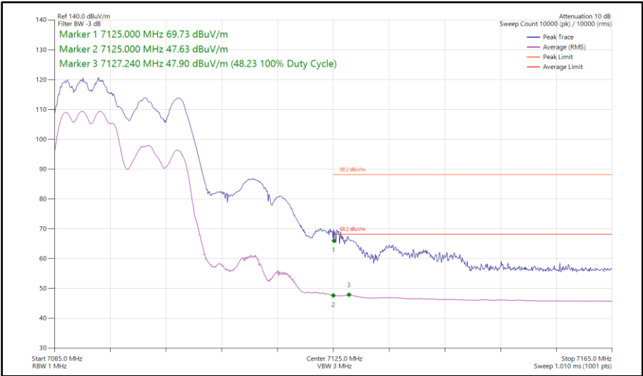
Figure 211 - 802.11ax HE20, RU 106-53, SDM, Core 0 - Core 1 - 7095 MHz Band Edge Frequency 7125 MHz
