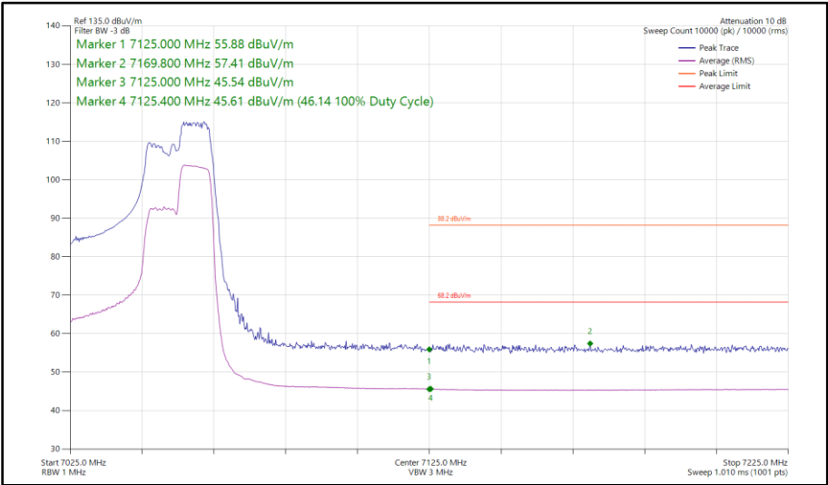
Figure 221 - 802.11ax HE40, RU 106-56, SISO, Core 0 - 7045 MHz Band Edge Frequency 7125 MHz
