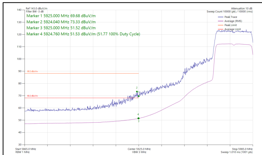
Figure 213 - 802.11ax HE20, SU, TxBF, Core 0 - Core 1 - 5975 MHz Band Edge Frequency 5925 MHz
