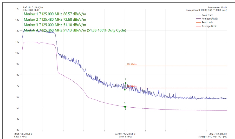
Figure 214 - 802.11ax HE20, SU, TxBF, Core 0 - Core 1 - 7075 MHz Band Edge Frequency 7125 MHz
