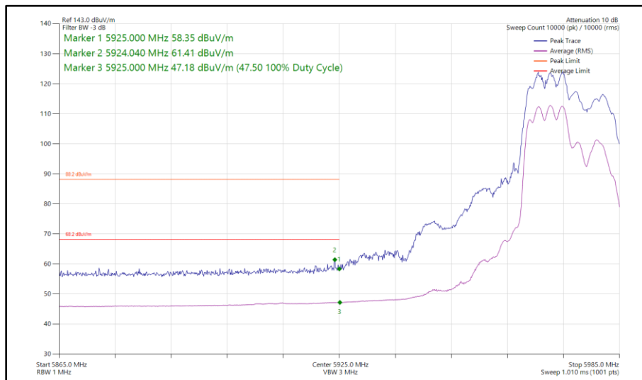
Figure 203 - 802.11ax HE20, RU 106-53, CDD, Core 0 - Core 1 - 5975 MHz Band Edge Frequency 5925 MHz
