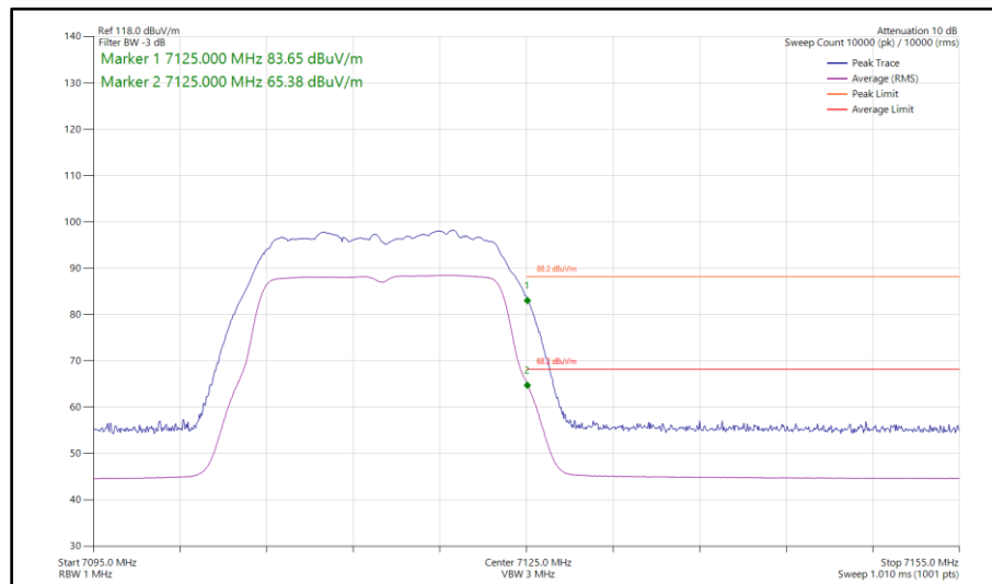
Figure 183 - 802.11a, SISO, Core 0 - 7115 MHz Band Edge Frequency 7125 MHz
