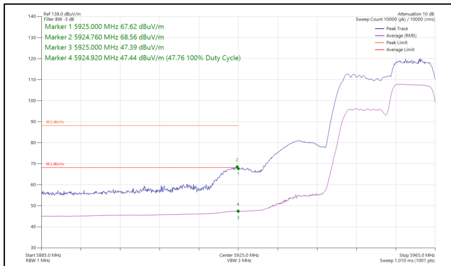
Figure 191 - 802.11ax HE20, RU 106-54, SISO, Core 1 - 5955 MHz Band Edge Frequency 5925 MHz
