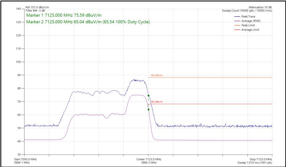
Figure 187 - 802.11ax HE20, RU 52-40, SISO, Core 0 - 7115 MHz Band Edge Frequency 7125 MHz
