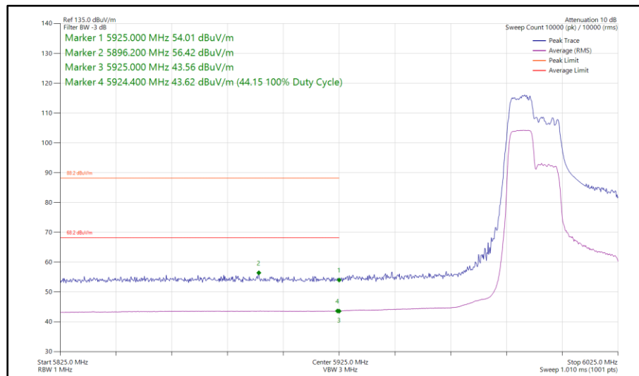
Figure 219 - 802.11ax HE40, RU 106-53, SISO, Core 0 - 6005 MHz Band Edge Frequency 5925 MHz
