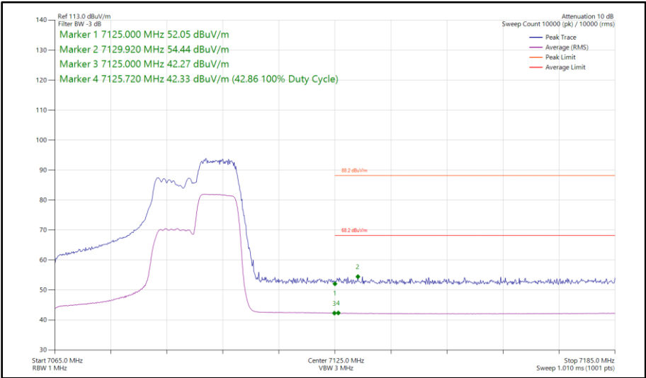
Figure 223 - 802.11ax HE40, RU 106-56, SISO, Core 0 - 7085 MHz Band Edge Frequency 7125 MHz
