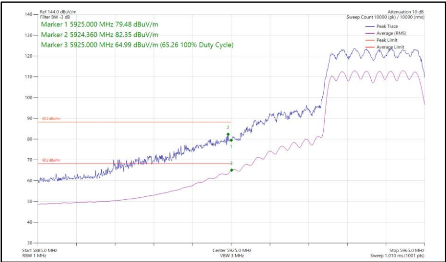
Figure 200 - 802.11ax HE20, SU, CDD, Core 0 - Core 1 - 5955 MHz Band Edge Frequency 5925 MHz
