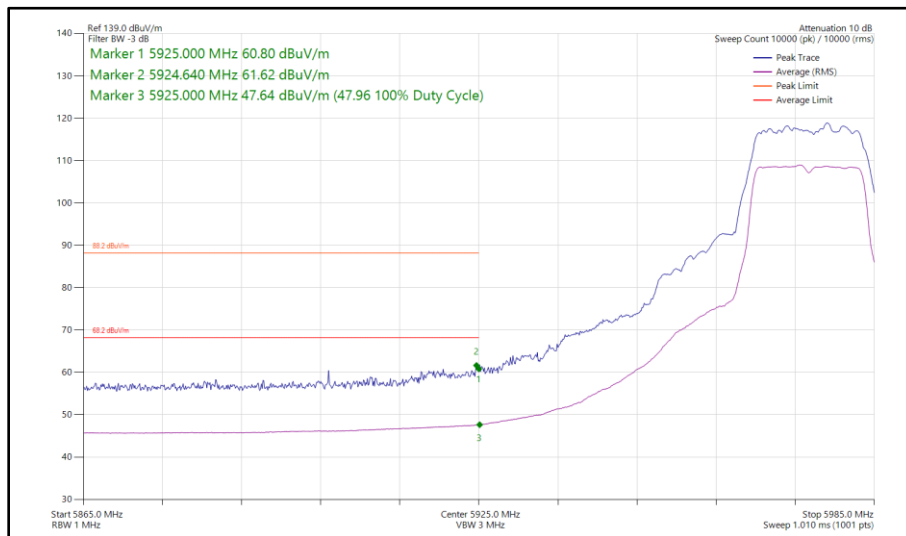
Figure 177 - 802.11a, SISO, Core 0 - 5975 MHz Band Edge Frequency 5925 MHz
