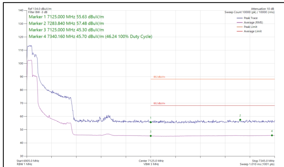
Figure 257 - 802.11ax HE80, RU 106-53, SISO, Core 0 - 6945 MHz Band Edge Frequency 7125 MHz
