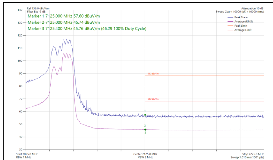
Figure 245 - 802.11ax HE40, RU 106-56, SDM, Core 0 - Core 1 - 7045 MHz Band Edge Frequency 7125 MHz
