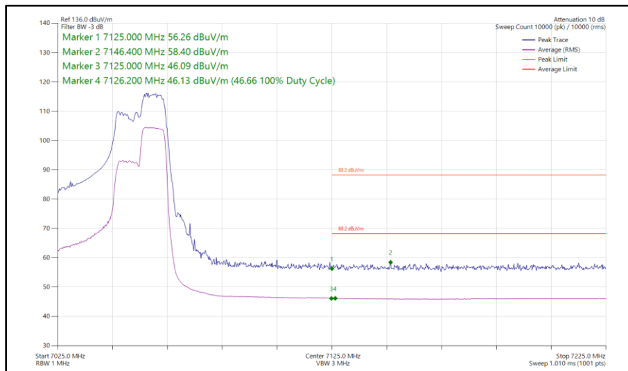
Figure 229 - 802.11ax HE40, RU 106-56, SISO, Core 1 - 7045 MHz Band Edge Frequency 7125 MHz
