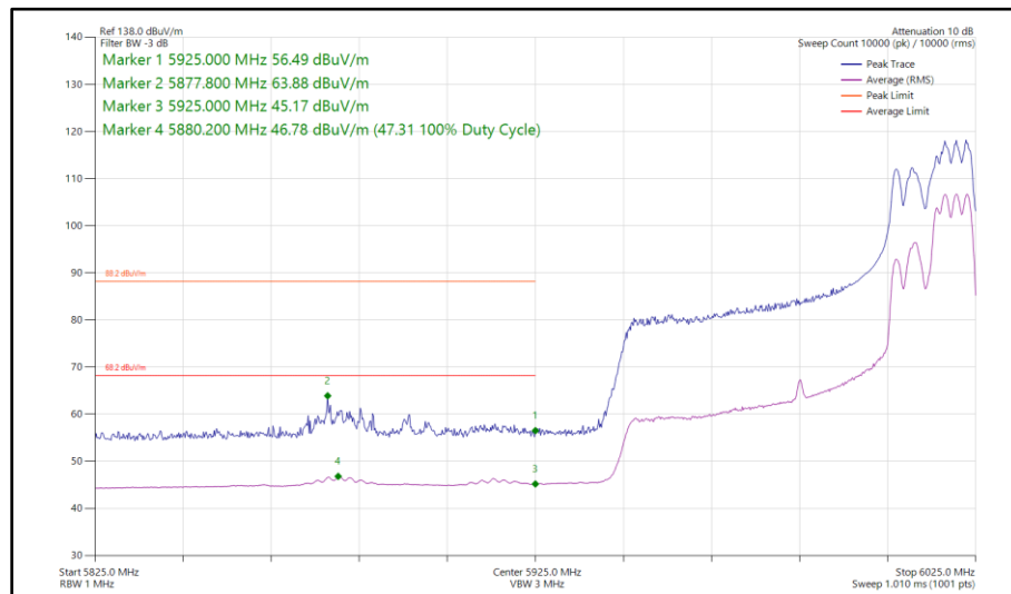
Figure 269 - 802.11ax HE80, RU 106-60, CDD, Core 0 - Core 1 - 5985 MHz Band Edge Frequency 5925 MHz
