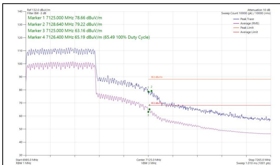
Figure 274 - 802.11ax HE80, SU, CDD, Core 0 - Core 1 - 7025 MHz Band Edge Frequency 7125 MHz
