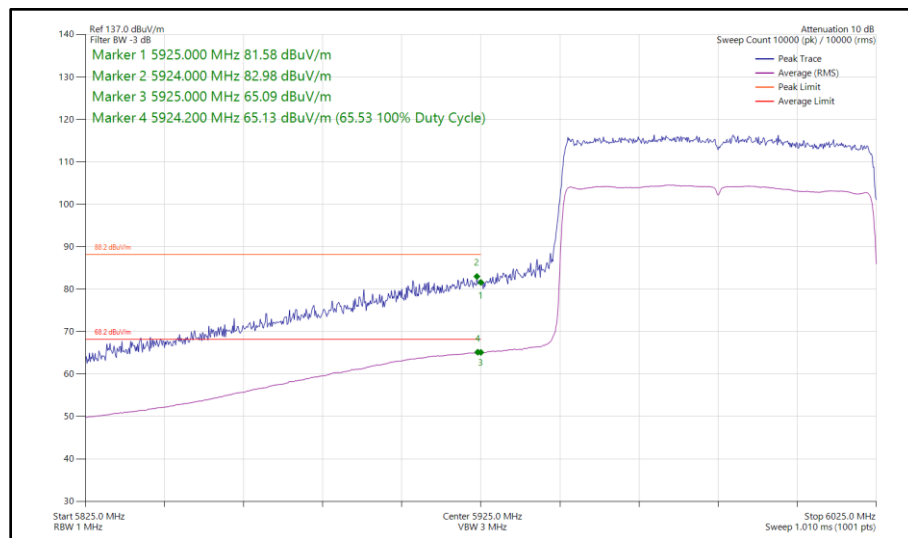
Figure 284 - 802.11ax HE80, SU, TxBF, Core 0 - Core 1 - 5985 MHz Band Edge Frequency 5925 MHz
