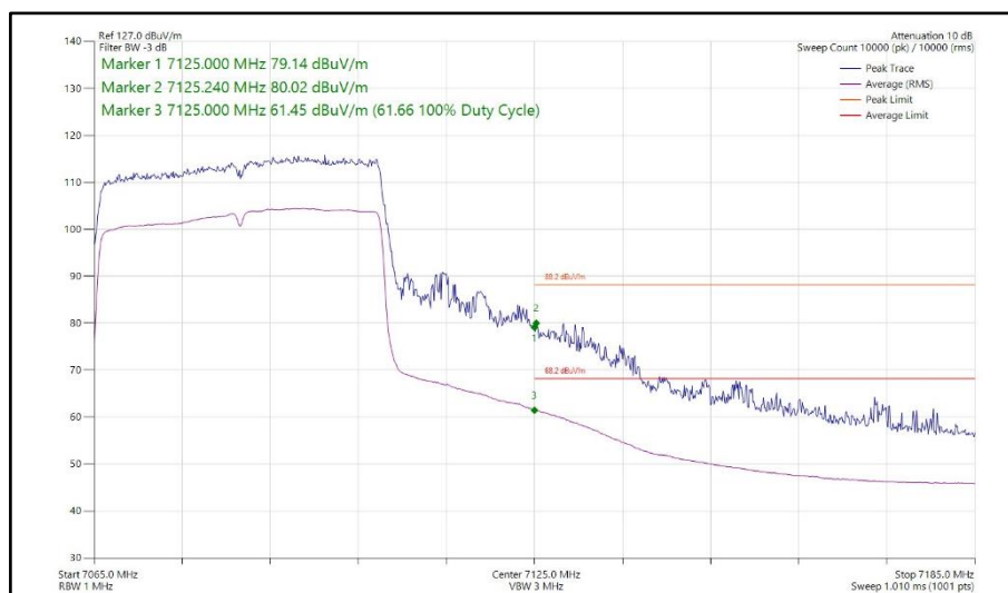
Figure 251 - 802.11ax HE40, SU, TxBF, Core 0 - Core 1 - 7085 MHz Band Edge Frequency 7125 MHz
