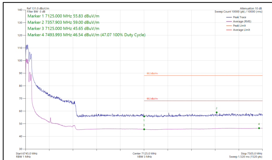
Figure 309 - 802.11ax HE160, RU 106-53P, CDD, Core 0 - Core 1 - 6825 MHz Band Edge Frequency 7125 MHz
