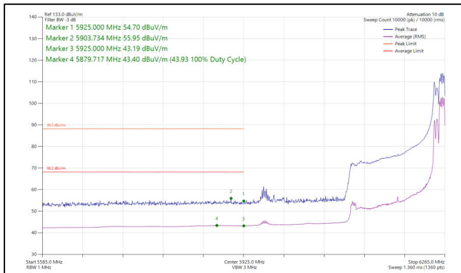
Figure 307 - 802.11ax HE160, RU 106-60S, CDD, Core 0 - Core 1 - 6185 MHz Band Edge Frequency 5925 MHz
