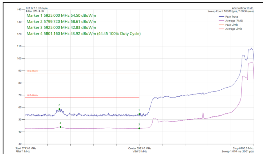
Figure 297 - 802.11ax HE160, RU 106-60S, SISO, Core 1 - 6025 MHz Band Edge Frequency 5925 MHz
