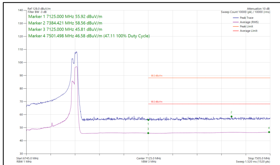
Figure 301 - 802.11ax HE160, RU 106-60S, SISO, Core 1 - 6825 MHz Band Edge Frequency 7125 MHz
