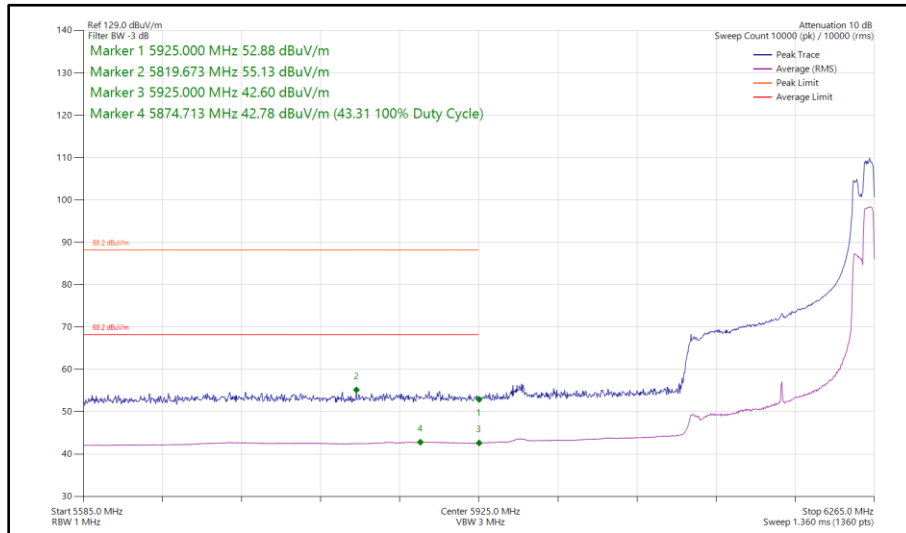
Figure 291 - 802.11ax HE160, RU 106-60S, SISO, Core 0 - 6185 MHz Band Edge Frequency 5925 MHz
