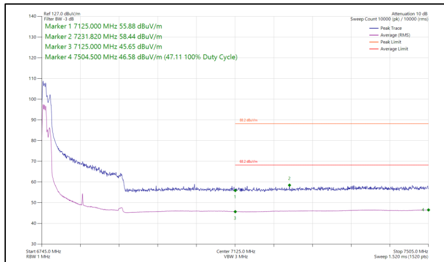
Figure 317 - 802.11ax HE160, RU 106-53P, SDM, Core 0 - Core 1 - 6825 MHz Band Edge Frequency 7125 MHz
