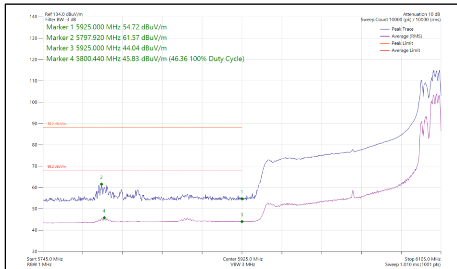
Figure 305 - 802.11ax HE160, RU 106-60S, CDD, Core 0 - Core 1 - 6025 MHz Band Edge Frequency 5925 MHz
