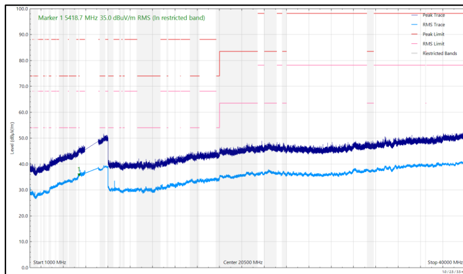
Figure 329 - 6435 MHz (CH97), HE20, SU, CDD, Core 0 + Core 1, 1 GHz to 40 GHz, Horizontal
