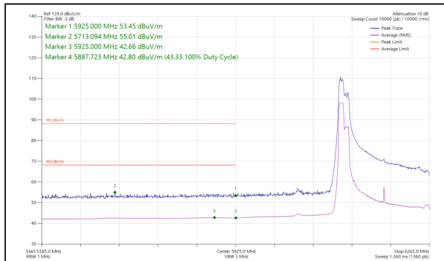
Figure 299 - 802.11ax HE160, RU 106-53P, SISO, Core 1 - 6185 MHz Band Edge Frequency 5925 MHz
