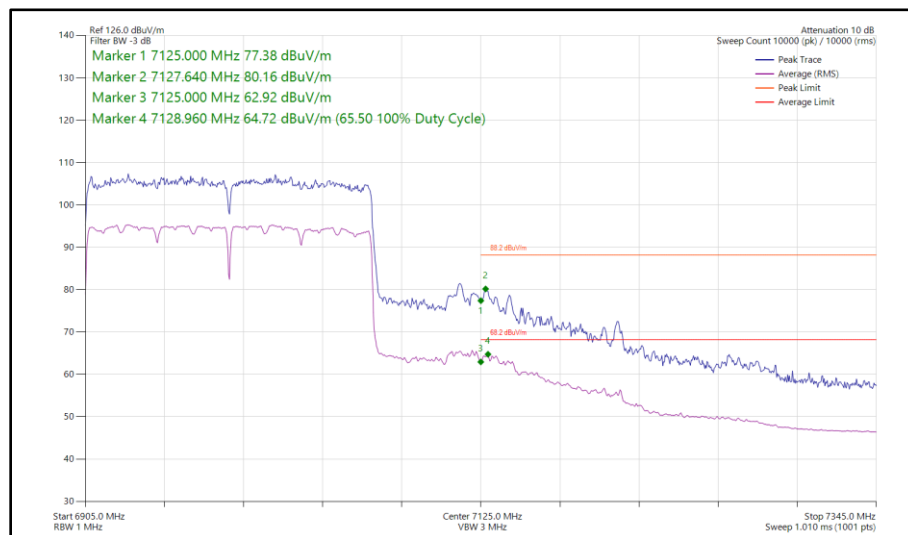
Figure 302 - 802.11ax HE160, SU, SISO, Core 1 - 6985 MHz Band Edge Frequency 7125 MHz
