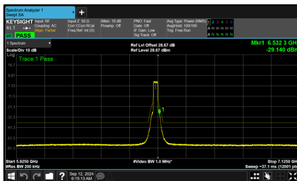
Figure 361 - A (Core 0) 802.11a SP 6515 MHz (CH113)
