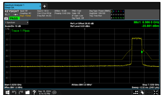
Figure 356 - A (Core 0) 802.11ax HE80 SU LPI 6945 MHz (CH199)
