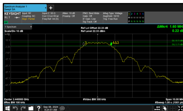
Figure 14 - Core 0 (A) 2440 MHz (CH18) 6 dB Bandwidth
