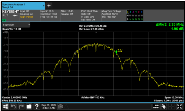
Figure 17 - Core 1 (B) 2405 MHz (CH11) 99% Bandwidth
