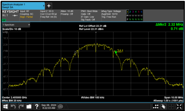
Figure 11 - Core 0 (A) 2405 MHz (CH11) 99% Bandwidth
