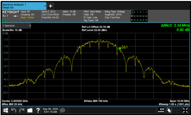
Figure 35 - Core 1 (B) 2405 MHz (CH11) 99% Bandwidth
