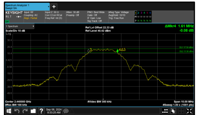
Figure 32 - Core 0 (A) 2440 MHz (CH18) 6 dB Bandwidth
