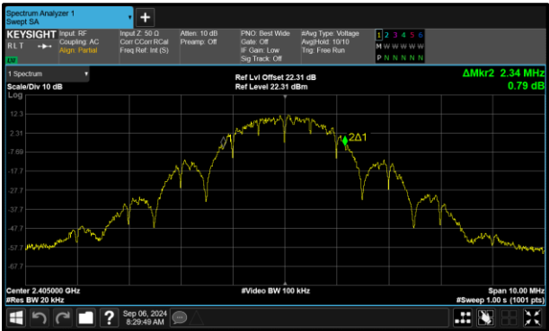
Figure 29 - Core 0 (A) 2405 MHz (CH11) 99% Bandwidth
