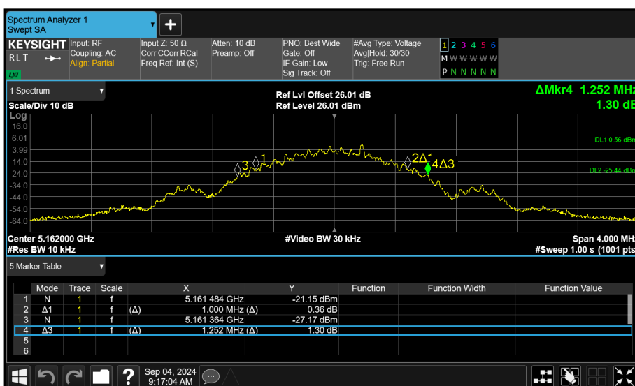
Figure 77 - Core 1 (B) 5162 MHz (CH12) 26 dB and 99% Bandwidth
