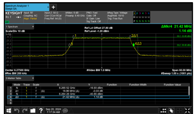
Figure 122 - 802.11a VLP Maximum 26 dB EBW
