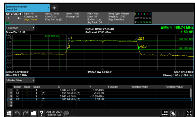
Figure 144 - 802.11ax HE160 SU SP Maximum 99% OBW
