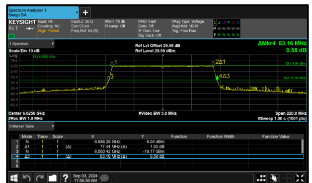
Figure 162 - 802.11ax HE80 SU SP Maximum 26 dB EBW
