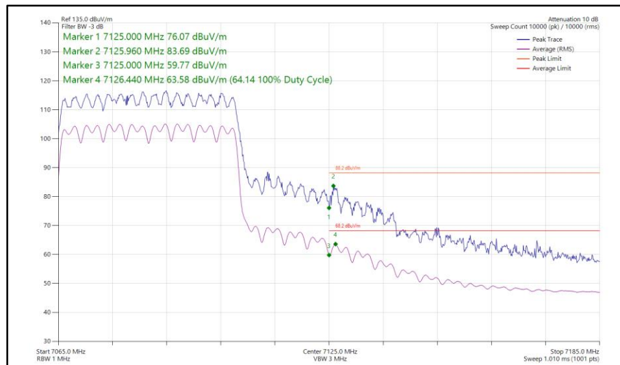
Figure 216 - 802.11ax HE40, SU, CDD, Core 0 - Core 1 - 7085 MHz Band Edge Frequency 7125 MHz
