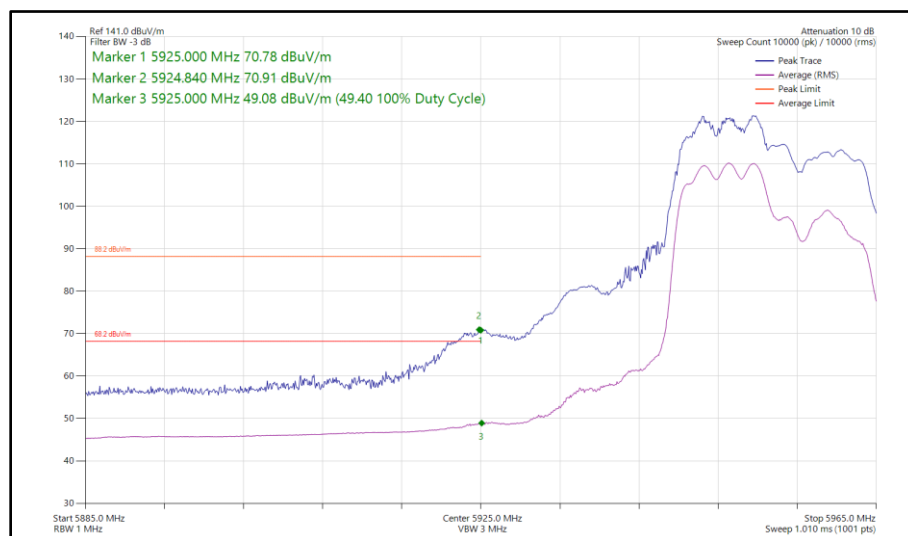
Figure 199 - 802.11ax HE20, RU 106-53, SDM, Core 0 - Core 1 - 5955 MHz Band Edge Frequency 5925 MHz
