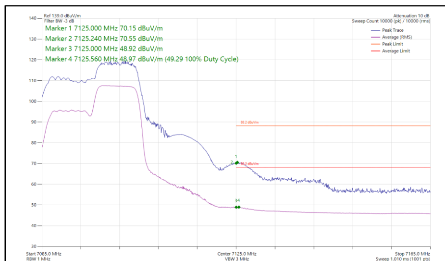
Figure 190 - 802.11ax HE20, RU 106-54, SISO, Core 1 - 7095 MHz Band Edge Frequency 7125 MHz
