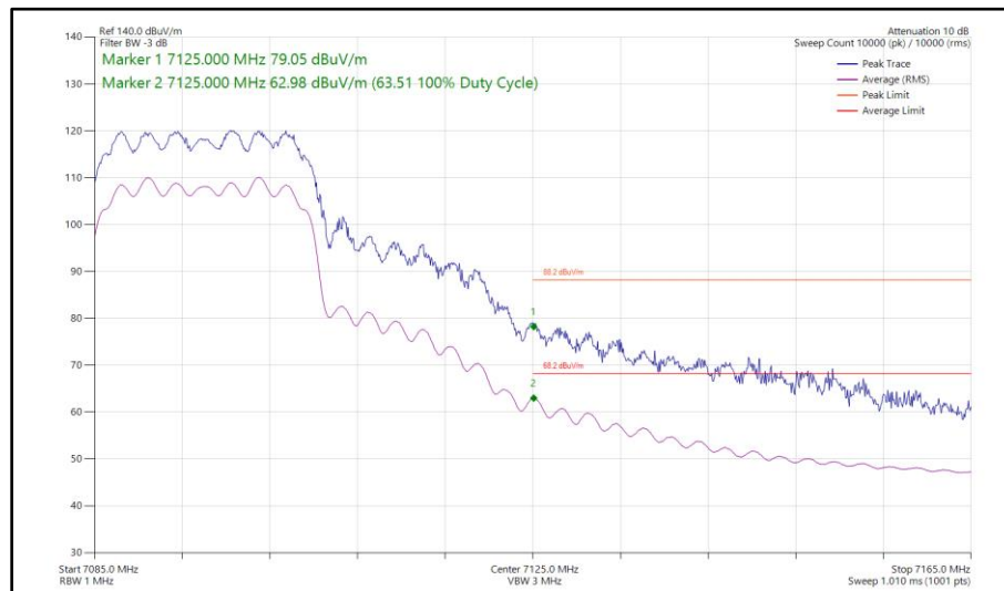
Figure 195 - 802.11ax HE20, SU, CDD, Core 0 - Core 1 - 7095 MHz Band Edge Frequency 7125 MHz
