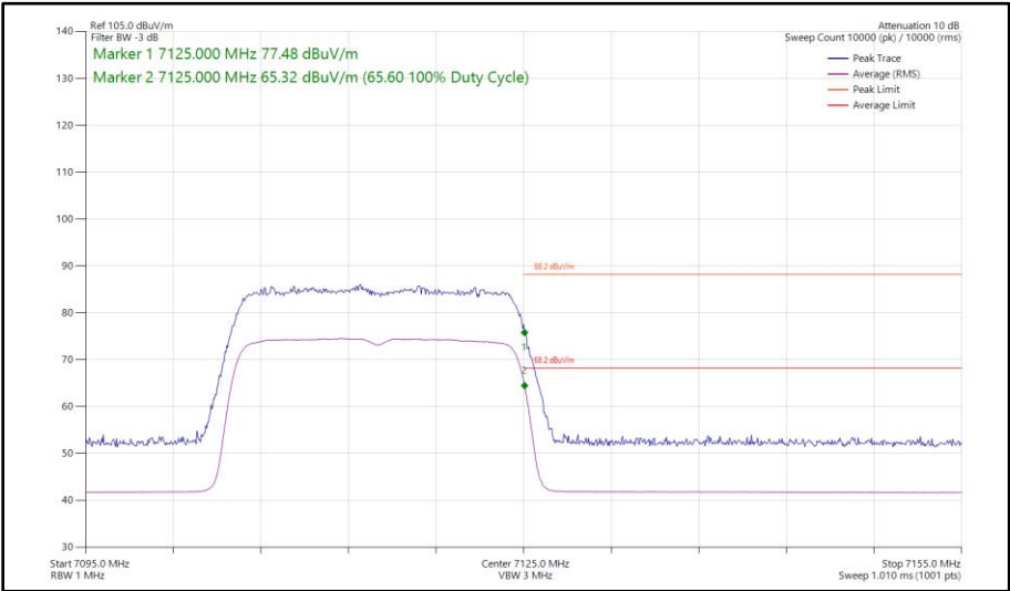
Figure 191 - 802.11ax HE20, SU, SISO, Core 1 - 7115 MHz Band Edge Frequency 7125 MHz
