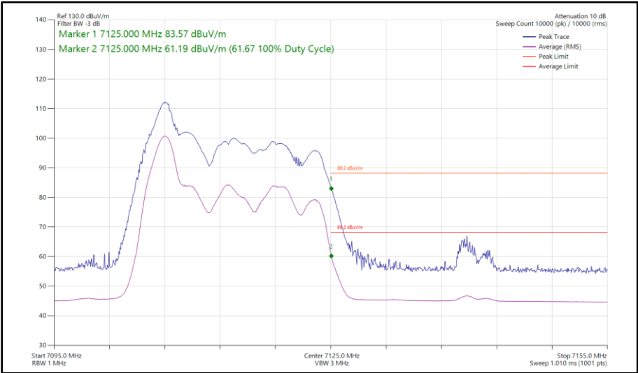
Figure 202 - 802.11ax HE20, RU 26-0, SDM, Core 0 - Core 1 - 7115 MHz Band Edge Frequency 7125 MHz
