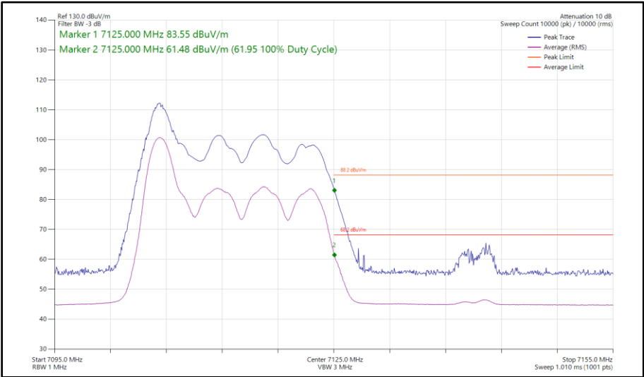
Figure 197 - 802.11ax HE20, RU 26-0, CDD, Core 0 - Core 1 - 7115 MHz Band Edge Frequency 7125 MHz
