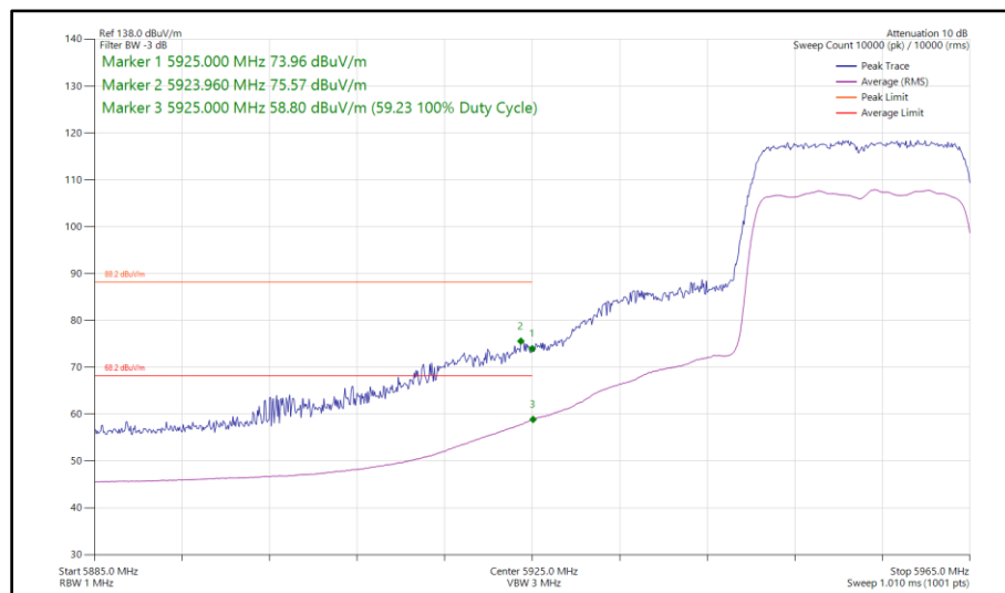
Figure 198 - 802.11ax HE20, SU, SDM, Core 0 - Core 1 - 5955 MHz Band Edge Frequency 5925 MHz
