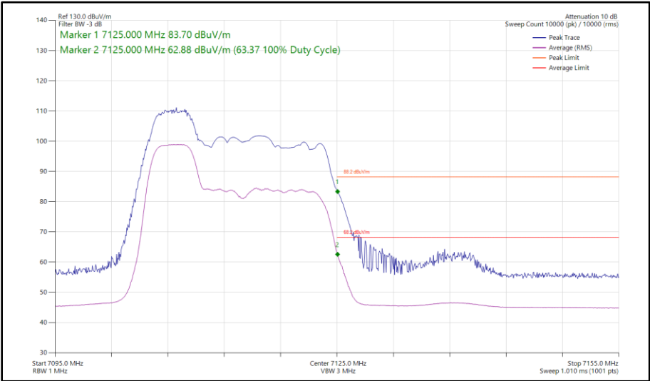
Figure 183 - 802.11ax HE20, RU 52-37, SISO, Core 0 - 7115 MHz Band Edge Frequency 7125 MHz
