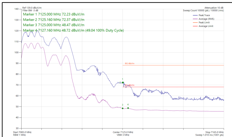
Figure 201 - 802.11ax HE20, RU 106-53, SDM, Core 0 - Core 1 - 7095 MHz Band Edge Frequency 7125 MHz
