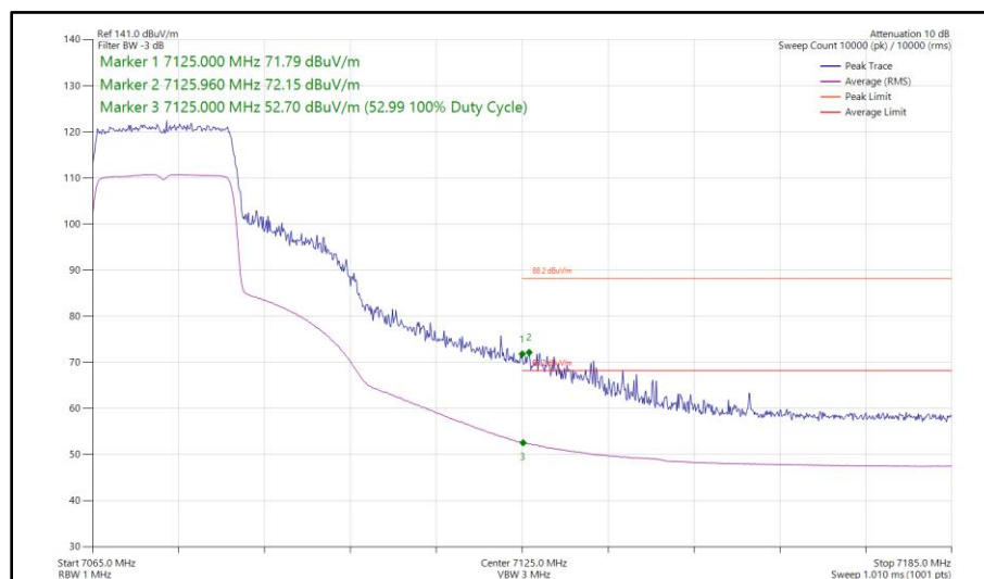
Figure 204 - 802.11ax HE20, SU, TxBF, Core 0 - Core 1 - 7075 MHz Band Edge Frequency 7125 MHz
