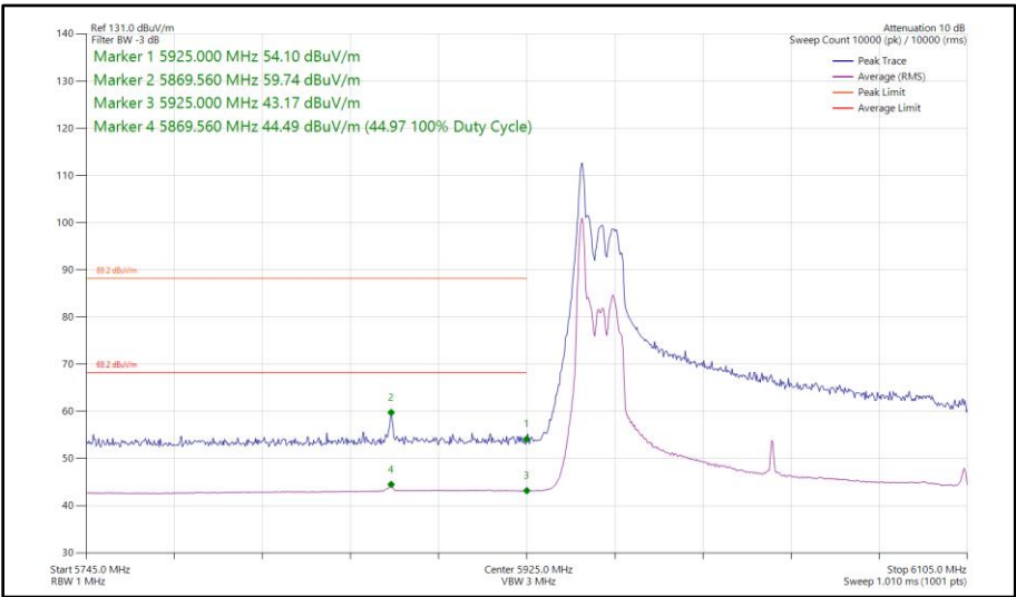
Figure 259 - 802.11ax HE160, RU 26-0P, SDM, Core 0 - Core 1 - 6025 MHz Band Edge Frequency 5925 MHz
