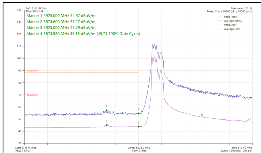
Figure 255 - 802.11ax HE160, RU 106-53P, CDD, Core 0 - Core 1 - 6025 MHz Band Edge Frequency 5925 MHz
