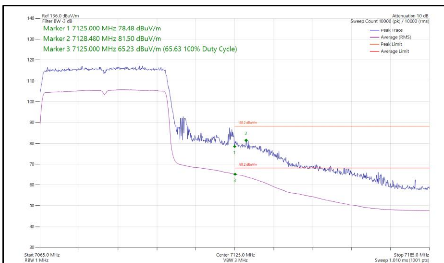
Figure 225 - 802.11ax HE40, SU, TxBF, Core 0 - Core 1 - 7085 MHz Band Edge Frequency 7125 MHz
