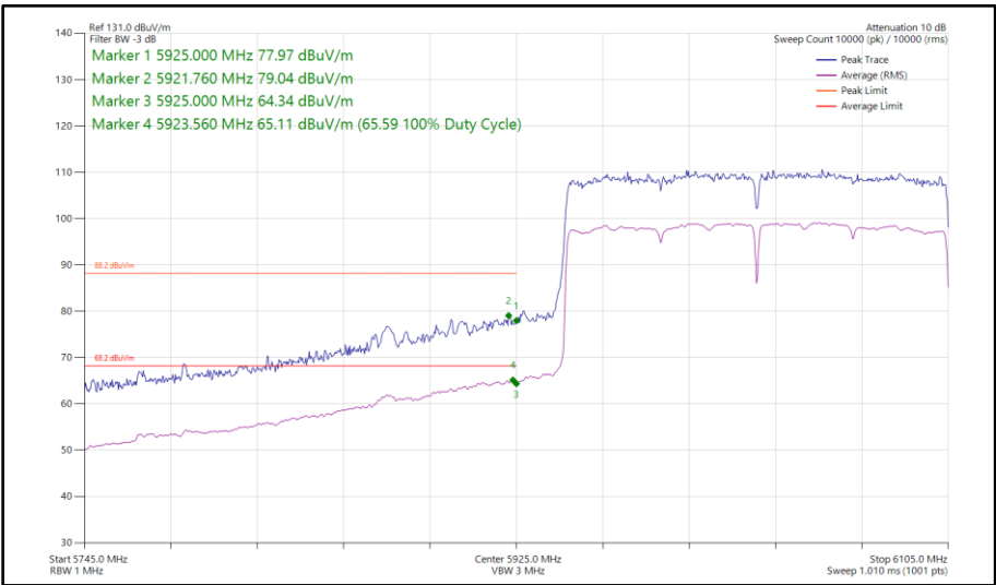
Figure 250 - 802.11ax HE160, SU, SISO, Core 1 - 6025 MHz Band Edge Frequency 5925 MHz
