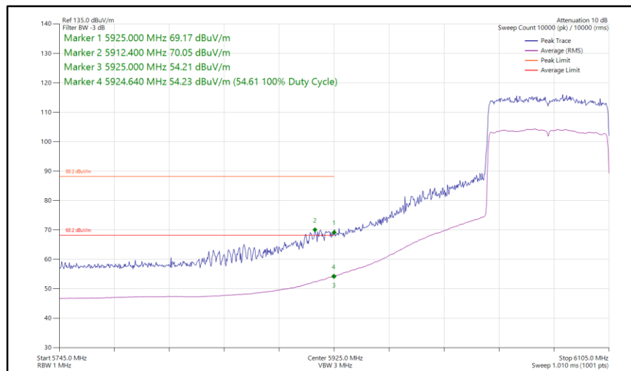
Figure 243 - 802.11ax HE80, SU, TxBF, Core 0 - Core 1 - 6065 MHz Band Edge Frequency 5925 MHz
