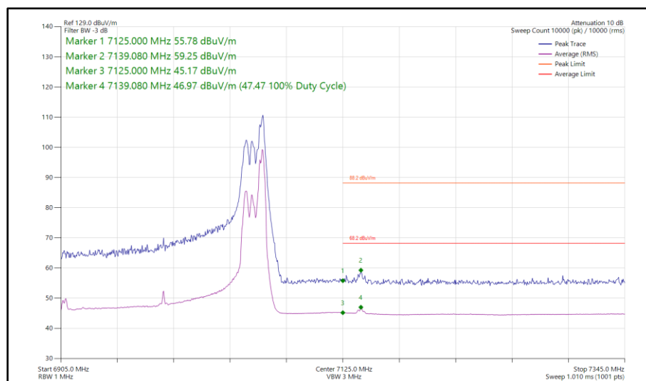
Figure 261 - 802.11ax HE160, RU 52-52S, SDM, Core 0 - Core 1 - 6985 MHz Band Edge Frequency 7125 MHz
