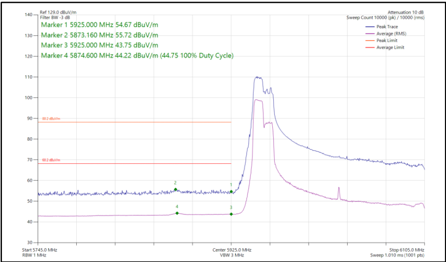
Figure 251 - 802.11ax HE160, RU 106-53P, SISO, Core 1 - 6025 MHz Band Edge Frequency 5925 MHz
