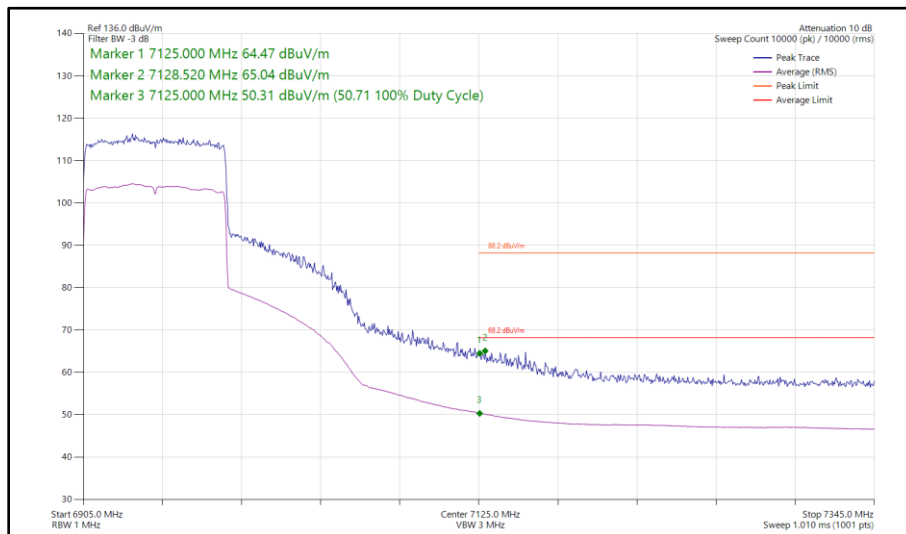
Figure 244 - 802.11ax HE80, SU, TxBF, Core 0 - Core 1 - 6945 MHz Band Edge Frequency 7125 MHz
