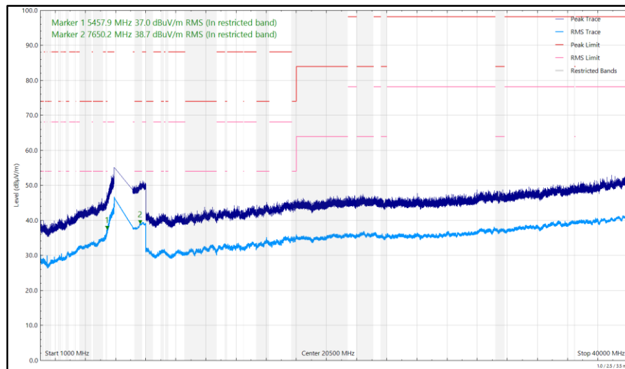
Figure 263 - U-NII-5 - 5955 MHz (CH1), HE20, SU, CDD, Core 0 + Core 1 1 GHz to 40 GHz, Horizontal
