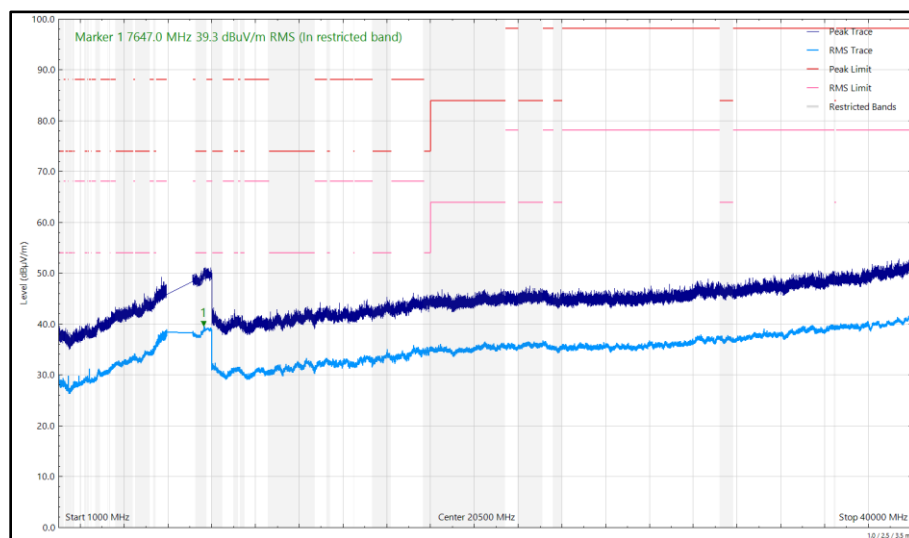
Figure 274 - U-NII-6 - 6475 MHz (CH105), HE20, SU, CDD, Core 0 + Core 1 1 GHz to 40 GHz, Horizontal
