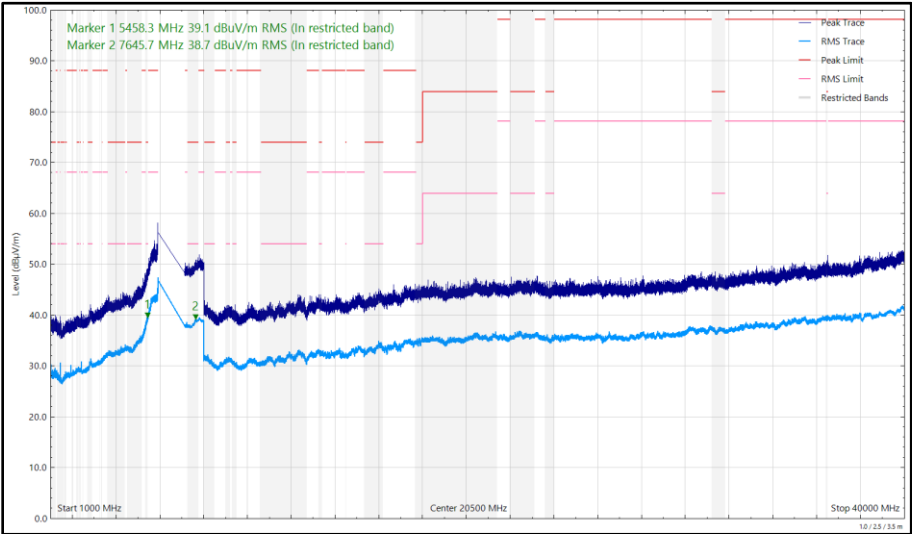
Figure 264 - U-NII-5 - 5955 MHz (CH1), HE20, SU, CDD, Core 0 + Core 1 1 GHz to 40 GHz, Vertical
