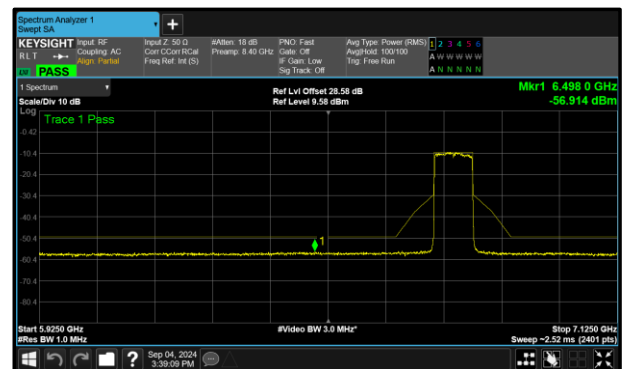
Figure 298 - A (Core 0) 802.11ax HE80 SU LPI 6785 MHz (CH167)
