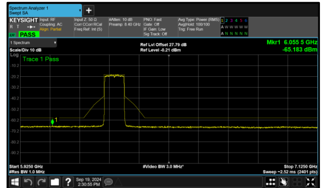
Figure 330 - B (Core 1) 802.11ax HE80 SU VLP 6305 MHz (CH71)
