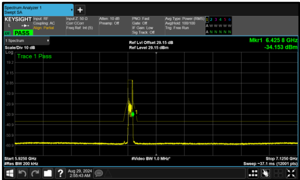
Figure 309 - A (Core 0) 802.11ax HE20 RU26 SP 6415 MHz (CH93)
