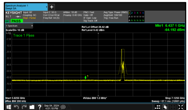
Figure 301 - A (Core 0) 802.11ax HE20 RU26 LPI 6695 MHz (CH149)
