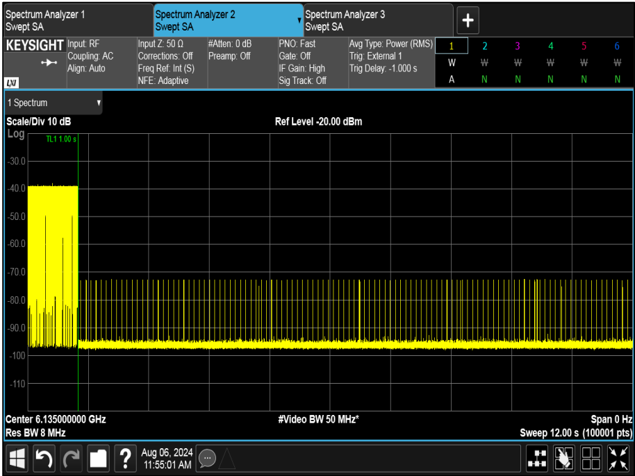
Figure 360 - U-NII-5, Maximum Bandwidth (AWGN High)
