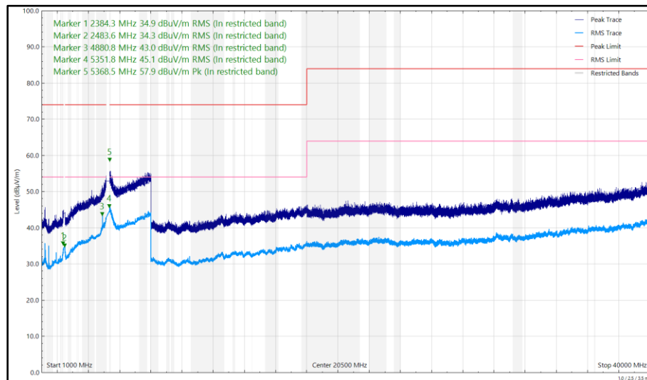
Figure 65 - U-NII-1 - 5240 MHz (CH48), HT20, CDD, Core 0 + Core 1 and 2440 MHz (CH18), Core1, ePA, Core 1, 1 GHz to 40 GHz, Vertical
