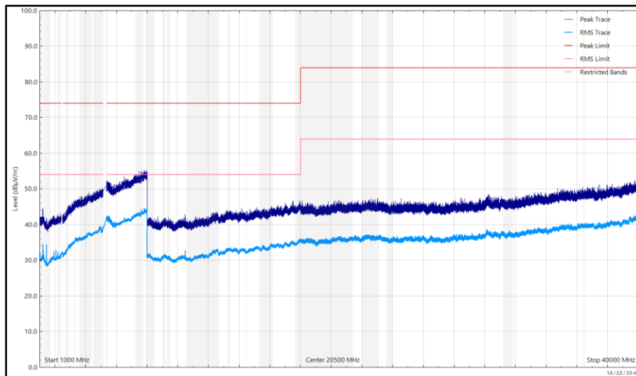
Figure 63 - U-NII-1 - 5240 MHz (CH48), HT20, CDD, Core 0 + Core 1 and 2440 MHz (CH18), Core1, ePA, Core 1, 1 GHz to 40 GHz, Horizontal
