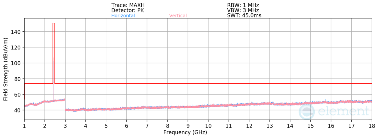
Plot 7-58. Radiated Spurious Emissions 1-18GHz Antenna 0 (Common) (1Mbps, iPA – Ch. 19)
