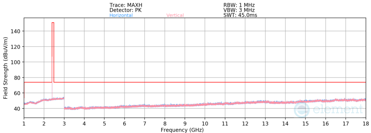
Plot 7-57. Radiated Spurious Emissions 1-18GHz Antenna 0 (Common) (1Mbps, iPA – Ch. 0)
