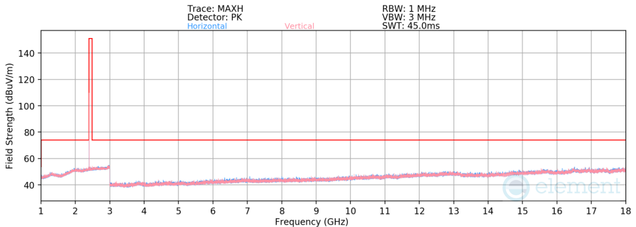
Plot 7-60. Radiated Spurious Emissions 1-18GHz Antenna 0 (Dedicated) (1Mbps, iPA – Ch. 0)
