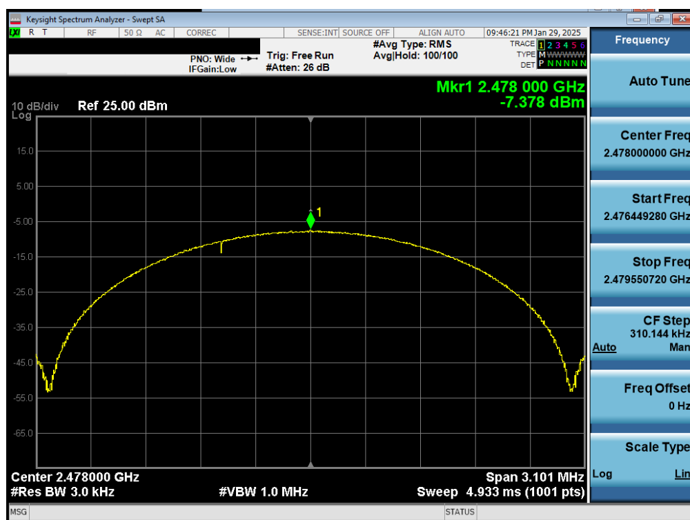
Plot 7-36. Power Spectral Density Plot Antenna 0 (Dedicated) (Bluetooth (LE), 2Mbps, iPA – Ch. 38)
