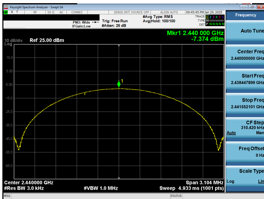
Plot 7-35. Power Spectral Density Plot Antenna 0 (Dedicated) (Bluetooth (LE), 2Mbps, iPA – Ch. 19)
