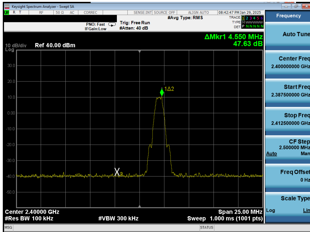
Plot 7-37. Band Edge Plot Antenna 0 (Common) (Bluetooth (LE), 1Mbps, iPA – Ch.0)
