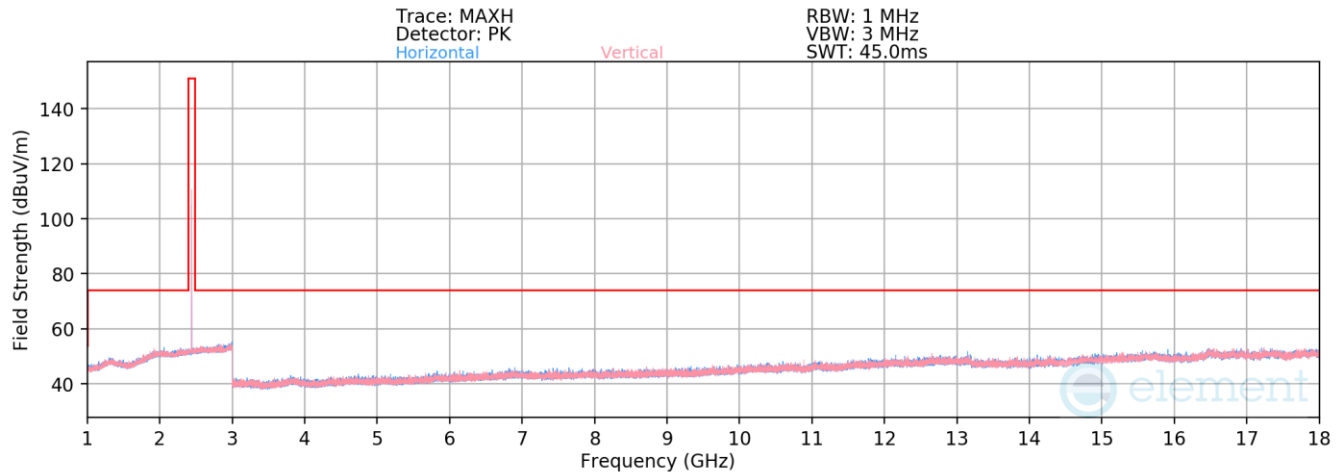
Plot 7-62. Radiated Spurious Emissions 1-18GHz Antenna 0 (Dedicated) (1Mbps, iPA – Ch. 19)
