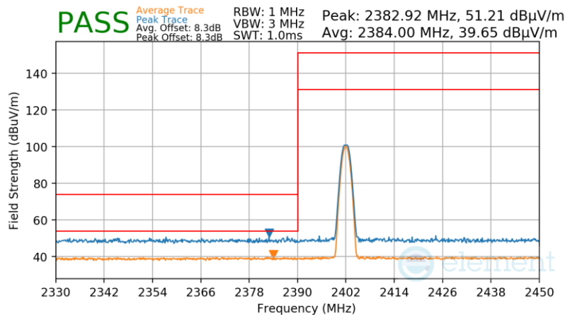
Plot 7-64. Radiated Restricted Lower Band Edge Measurement Antenna 0 (Common) (Average & Peak)
