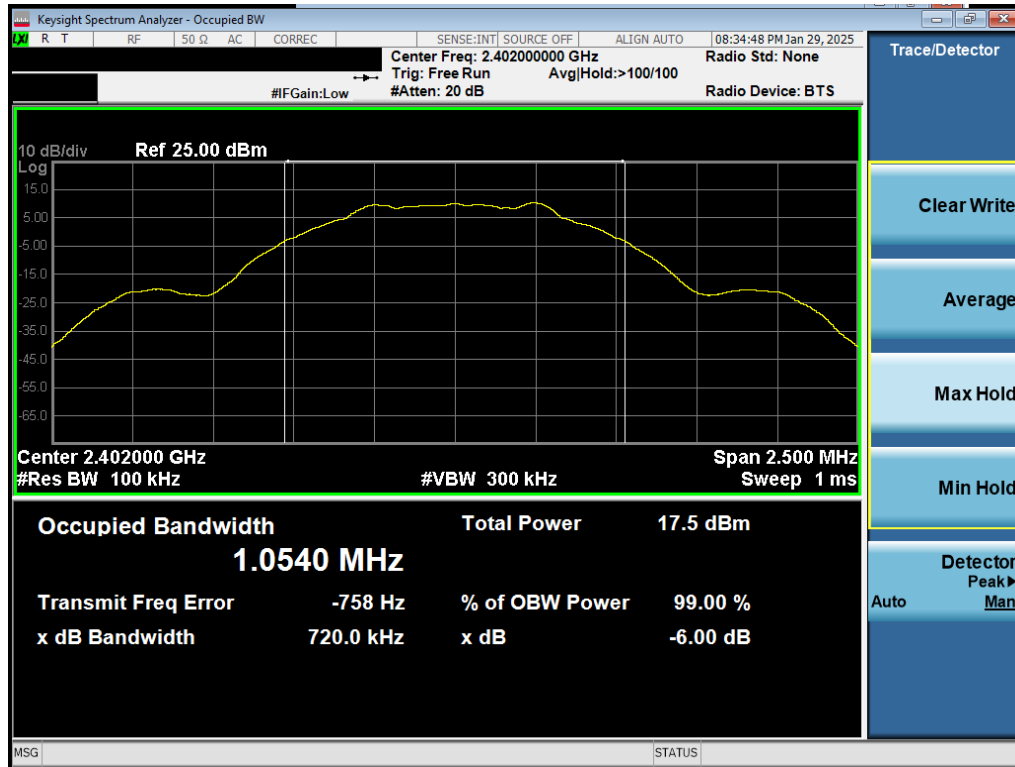
Plot 7-13. 6dB BW Plot Antenna 0 (Common) (Bluetooth (LE), 1Mbps, iPA – Ch. 0)
