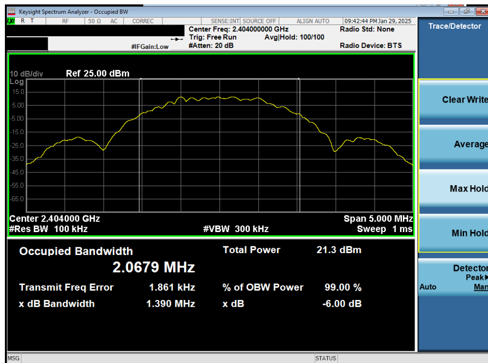
Plot 7-22. 6dB BW Plot Antenna 0 (Dedicated) (Bluetooth (LE), 2Mbps, iPA – Ch. 1)
