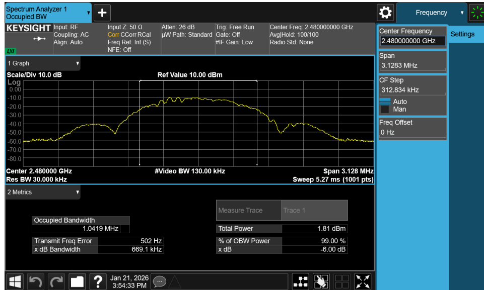
Plot 7-9. 99% OBW Plot Antenna 0 (Dedicated) (Bluetooth (LE), 1Mbps, iPA – Ch. 39)
