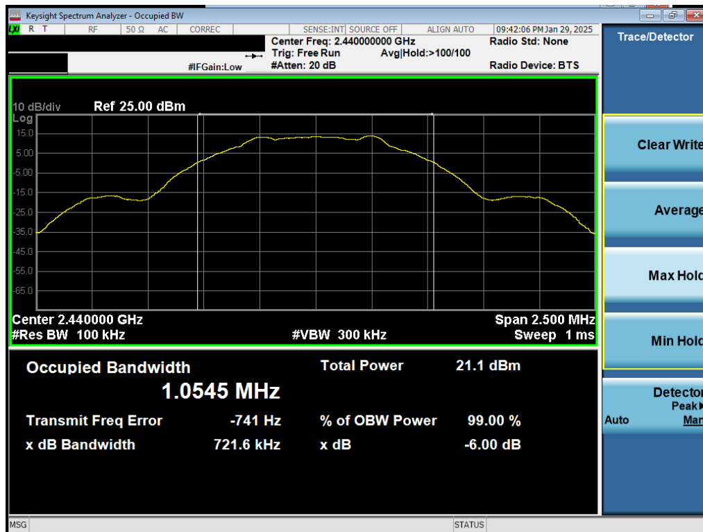
Plot 7-20. 6dB BW Plot Antenna 0 (Dedicated) (Bluetooth (LE), 1Mbps, iPA – Ch. 19)
