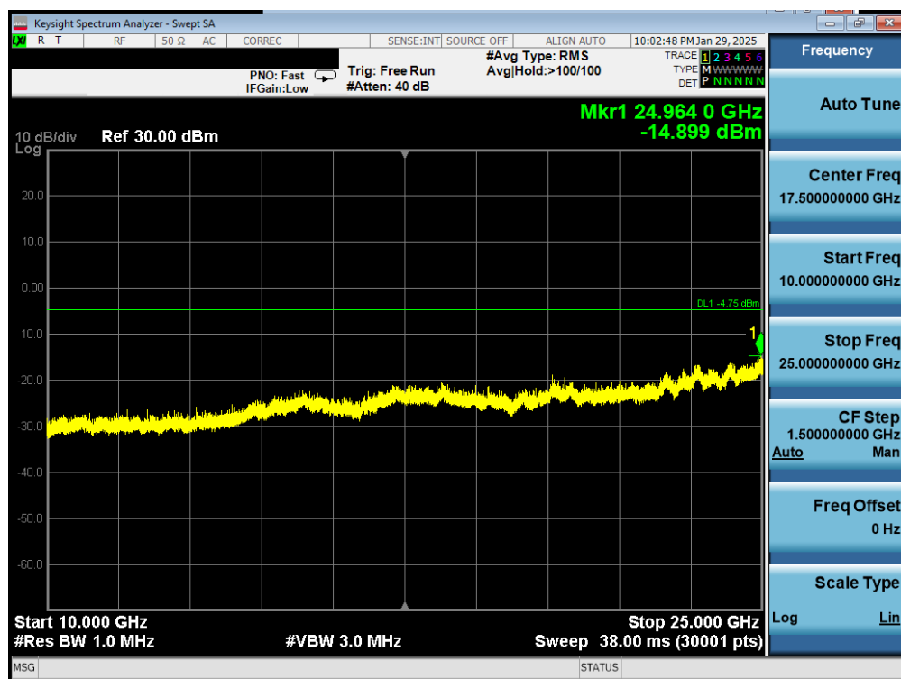
Plot 7-56. Conducted Spurious Plot Antenna 0 (Dedicated) (Bluetooth (LE), 1Mbps, iPA – Ch. 39)
