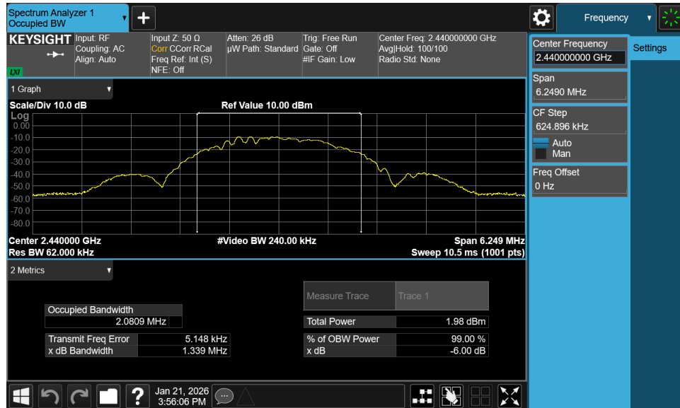
Plot 7-11. 99% OBW Plot Antenna 0 (Dedicated) (Bluetooth (LE), 2Mbps, iPA – Ch. 19)
