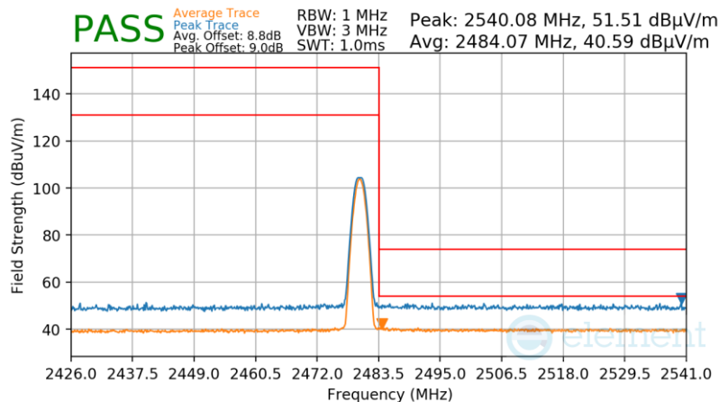
Plot 7-69. Radiated Restricted Upper Band Edge Measurement Antenna 0 (Dedicated) (Average & Peak)
