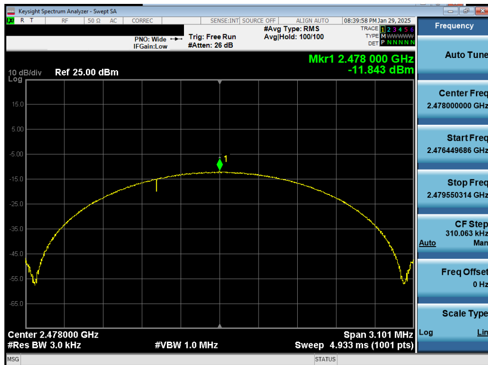
Plot 7-30. Power Spectral Density Plot Antenna 0 (Common) (Bluetooth (LE), 2Mbps, iPA – Ch. 38)
