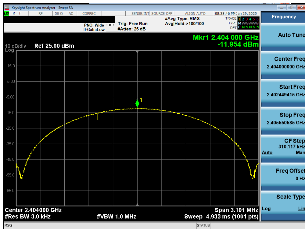
Plot 7-28. Power Spectral Density Plot Antenna 0 (Common) (Bluetooth (LE), 2Mbps, iPA – Ch. 1)
