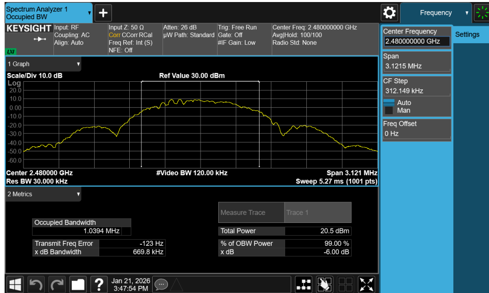
Plot 7-3. 99% OBW Plot Antenna 0 (Common) (Bluetooth (LE), 1Mbps, iPA – Ch. 39)
