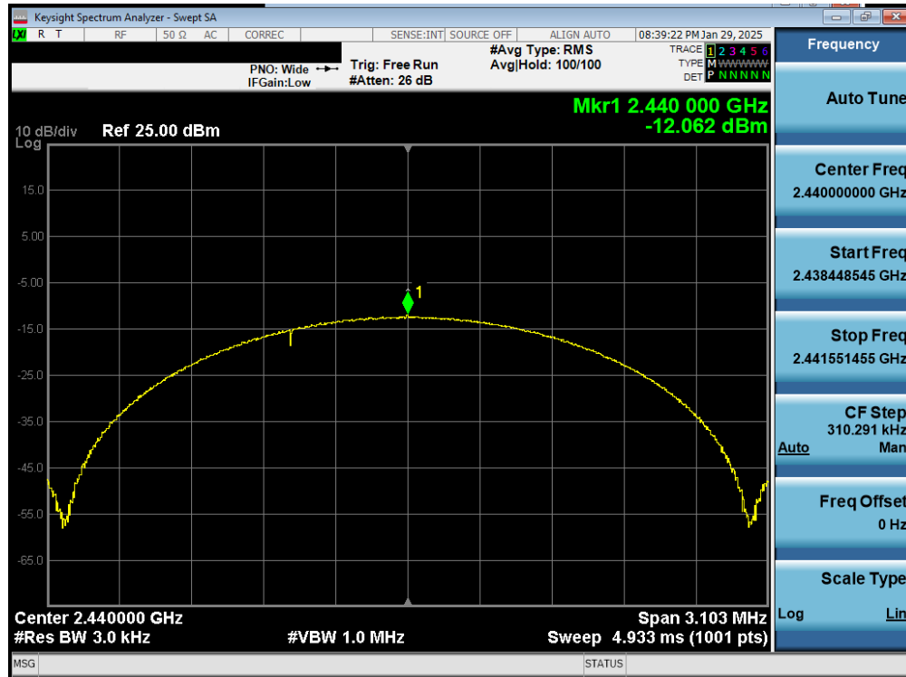
Plot 7-29. Power Spectral Density Plot Antenna 0 (Common) (Bluetooth (LE), 2Mbps, iPA – Ch. 19)
