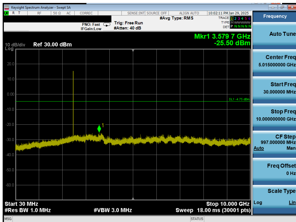
Plot 7-55. Conducted Spurious Plot Antenna 0 (Dedicated) (Bluetooth (LE), 1Mbps, iPA – Ch. 39)
