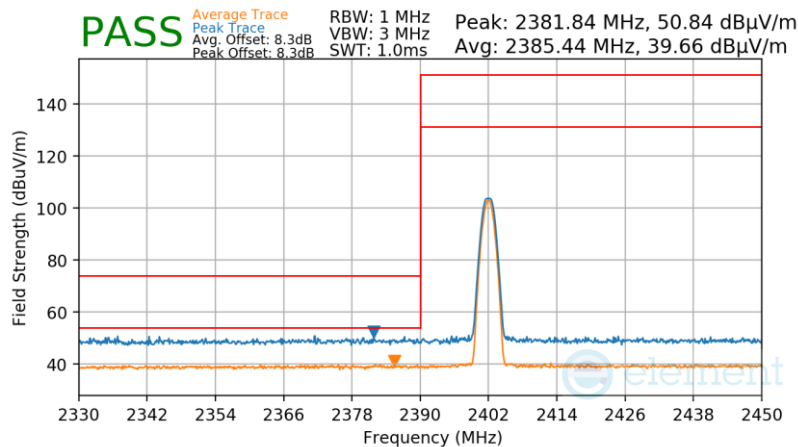
Plot 7-68. Radiated Restricted Lower Band Edge Measurement Antenna 0 (Dedicated) (Average & Peak)
