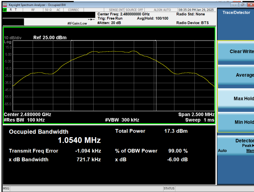
Plot 7-15. 6dB BW Plot Antenna 0 (Common) (Bluetooth (LE), 1Mbps, iPA – Ch. 39)
