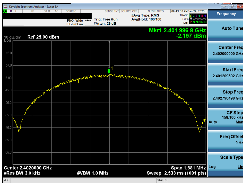
Plot 7-31. Power Spectral Density Plot Antenna 0 (Dedicated) (Bluetooth (LE), 1Mbps, iPA – Ch. 0)
