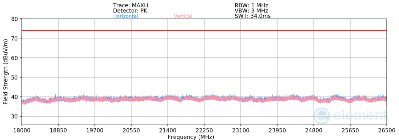
Plot 7-61. Radiated Spurious Emissions Above 18GHz Antenna 0 (Dedicated) (1Mbps, iPA – Ch. 0)
