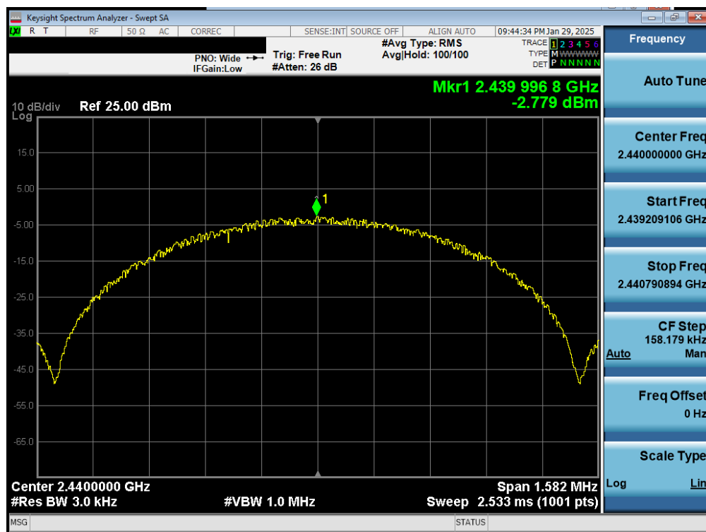
Plot 7-32. Power Spectral Density Plot Antenna 0 (Dedicated) (Bluetooth (LE), 1Mbps, iPA – Ch. 19)
