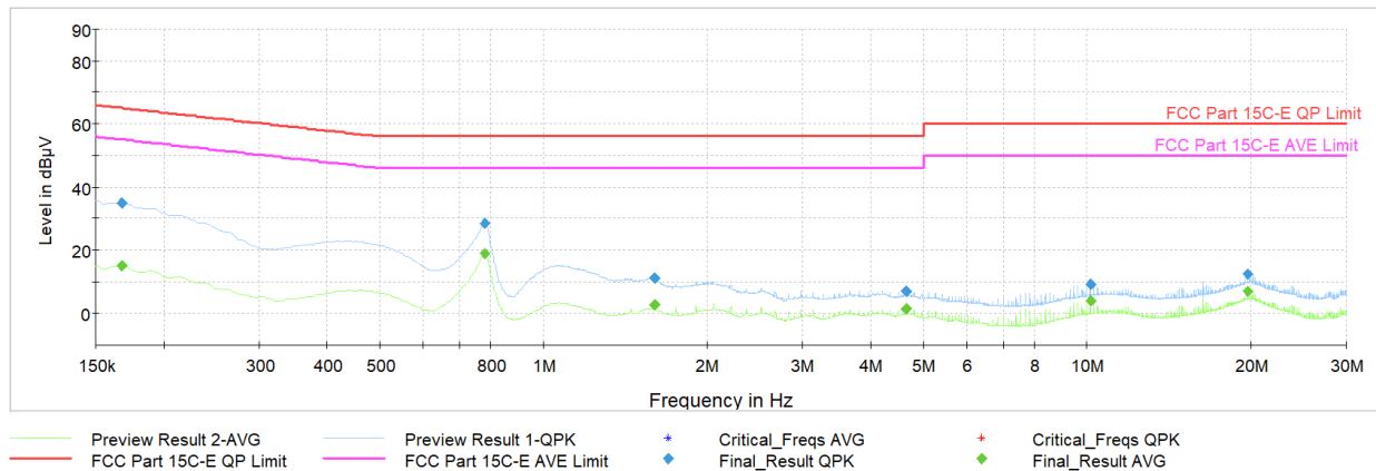
Plot 7-74. AC Line Conducted Plot with Bluetooth LE Antenna 0 Dedicated (N, 1Mbps iPA – Ch.0, with AC/DC Adapter)
