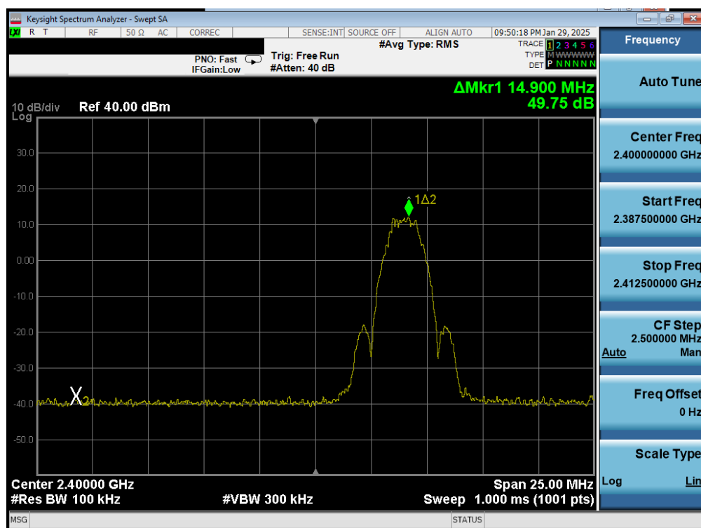
Plot 7-43. Band Edge Plot Antenna 0 (Dedicated) (Bluetooth (LE), 2Mbps, iPA – Ch. 1)
