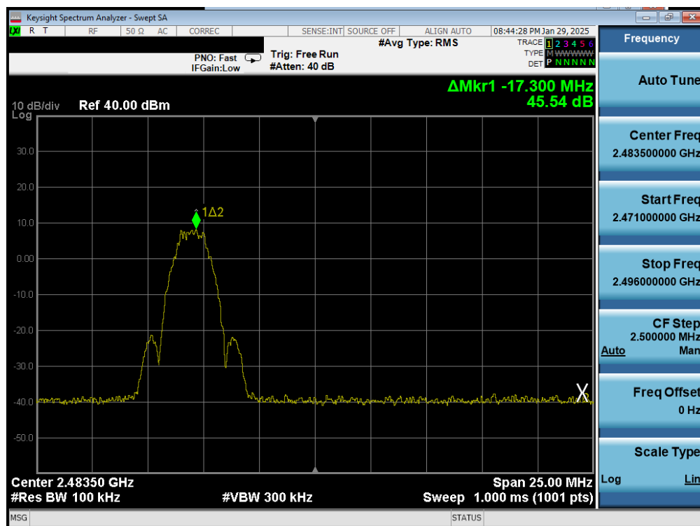
Plot 7-40. Band Edge Plot Antenna 0 (Common) (Bluetooth (LE), 2Mbps, iPA – Ch. 38)
