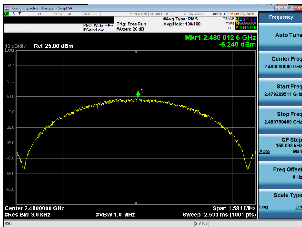
Plot 7-27. Power Spectral Density Plot Antenna 0 (Common) (Bluetooth (LE), 1Mbps, iPA – Ch. 39)
