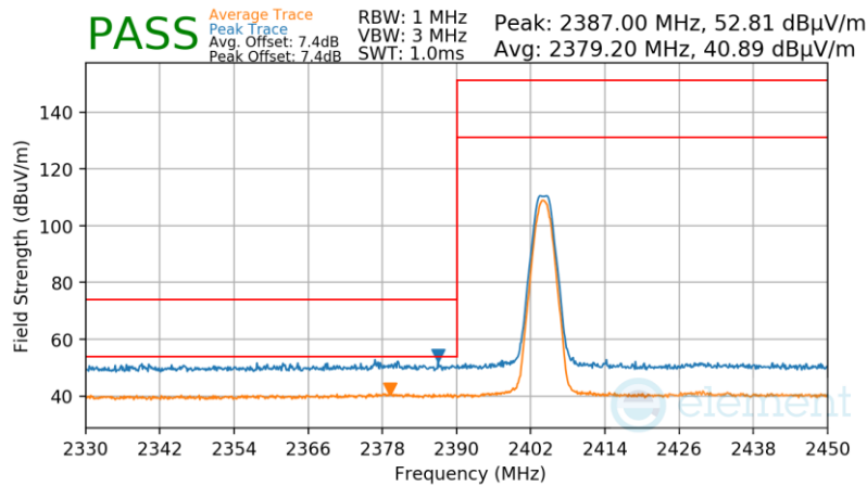
Plot 7-70. Radiated Restricted Lower Band Edge Measurement Antenna 0 (Dedicated) (Average & Peak)
