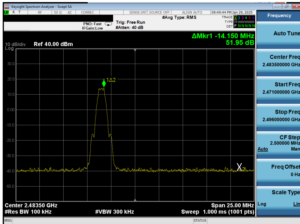
Plot 7-42. Band Edge Plot Antenna 0 (Dedicated) (Bluetooth (LE), 1Mbps, iPA – Ch. 39)
