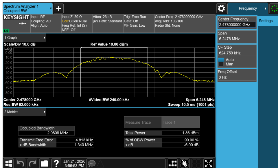
Plot 7-12. 99% OBW Plot Antenna 0 (Dedicated) (Bluetooth (LE), 2Mbps, iPA – Ch. 38)
