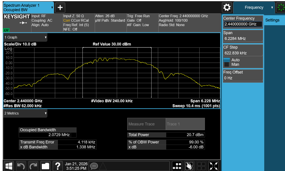
Plot 7-5. 99% OBW Plot Antenna 0 (Common) (Bluetooth (LE), 2Mbps, iPA – Ch. 19)
