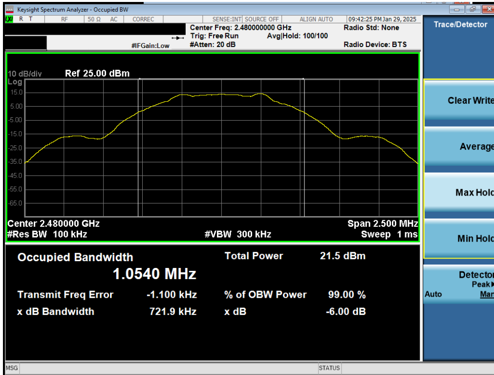
Plot 7-21. 6dB BW Plot Antenna 0 (Dedicated) (Bluetooth (LE), 1Mbps, iPA – Ch. 39)
