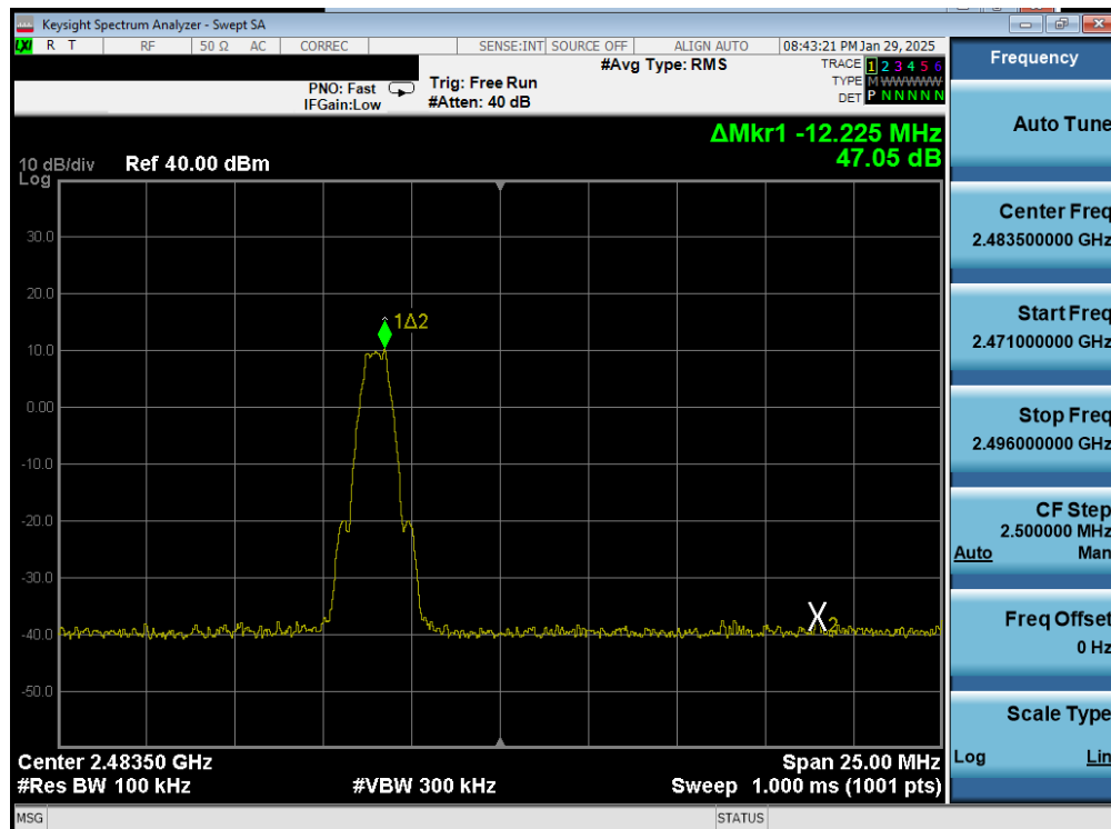
Plot 7-38. Band Edge Plot Antenna 0 (Common) (Bluetooth (LE), 1Mbps, iPA – Ch. 39)
