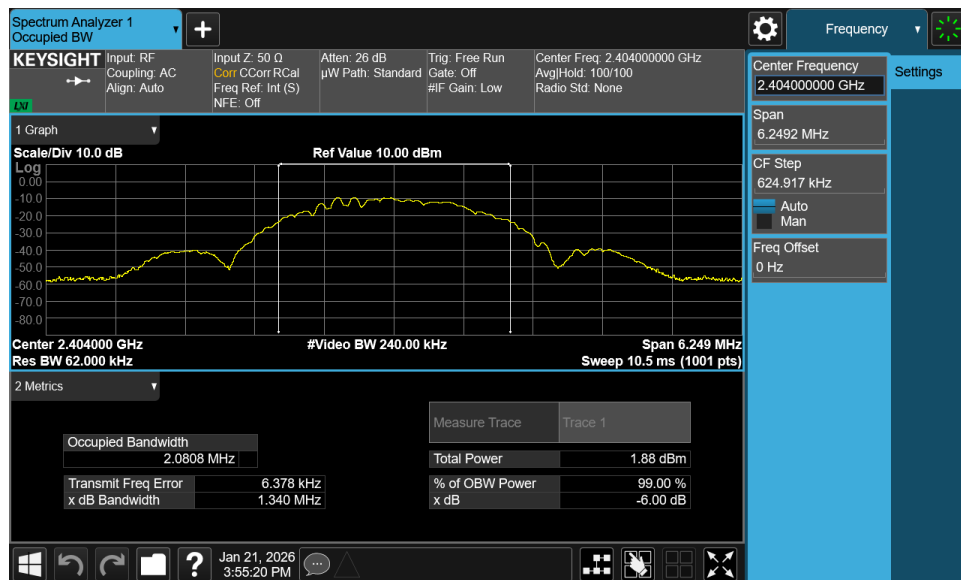
Plot 7-10. 99% OBW Plot Antenna 0 (Dedicated) (Bluetooth (LE), 2Mbps, iPA – Ch. 1)
