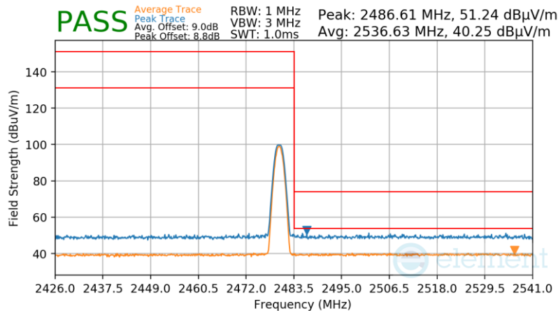
Plot 7-65. Radiated Restricted Upper Band Edge Measurement Antenna 0 (Common) (Average & Peak)
