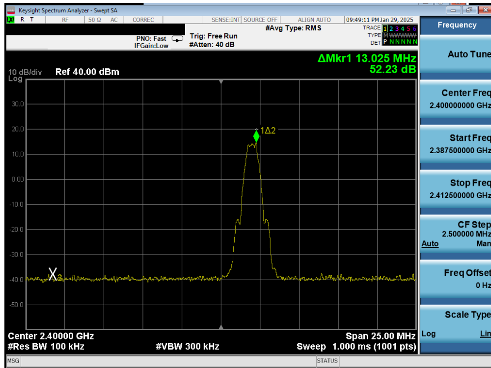
Plot 7-41. Band Edge Plot Antenna 0 (Dedicated) (Bluetooth (LE), 1Mbps, iPA – Ch.0)
