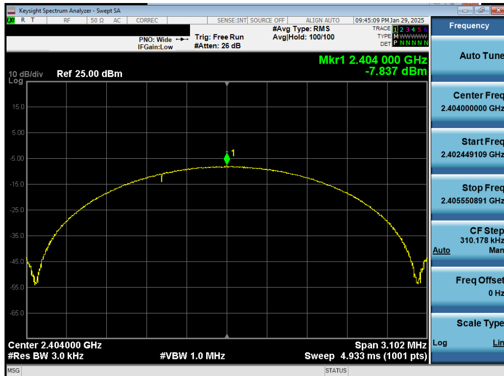
Plot 7-34. Power Spectral Density Plot Antenna 0 (Dedicated) (Bluetooth (LE), 2Mbps, iPA – Ch. 1)
