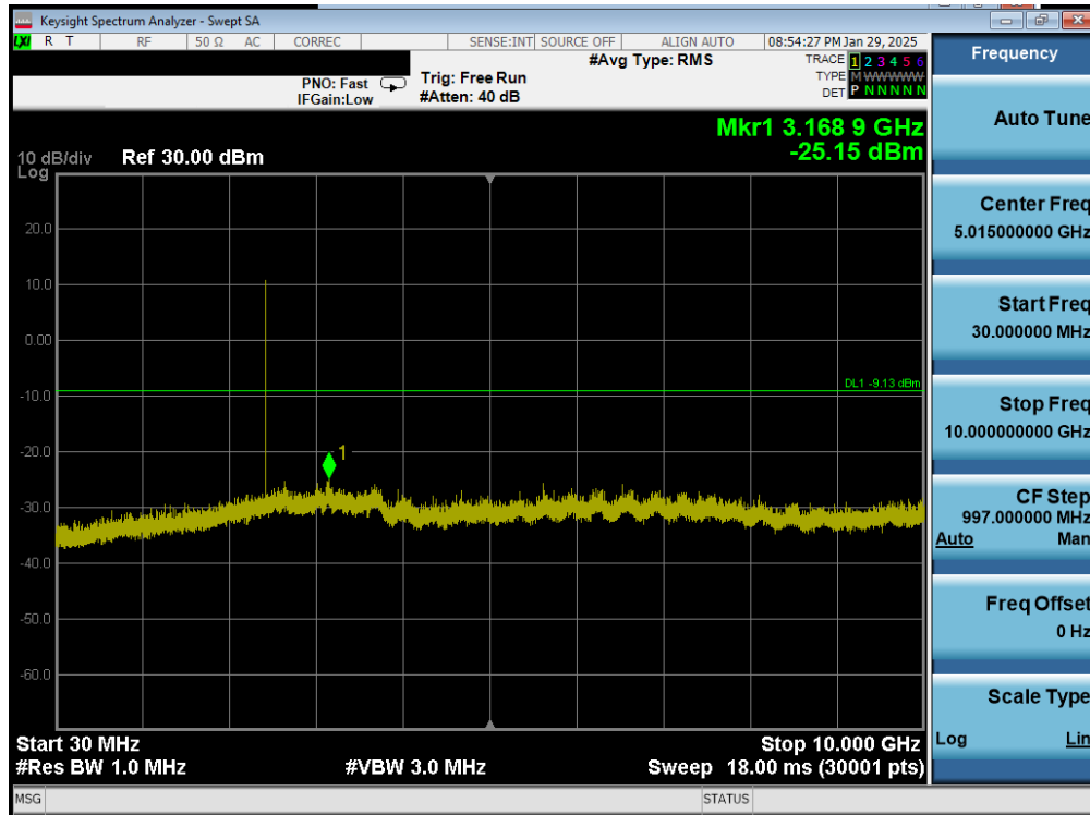
Plot 7-47. Conducted Spurious Plot Antenna 0 (Common) (Bluetooth (LE), 1Mbps, iPA – Ch. 19)
