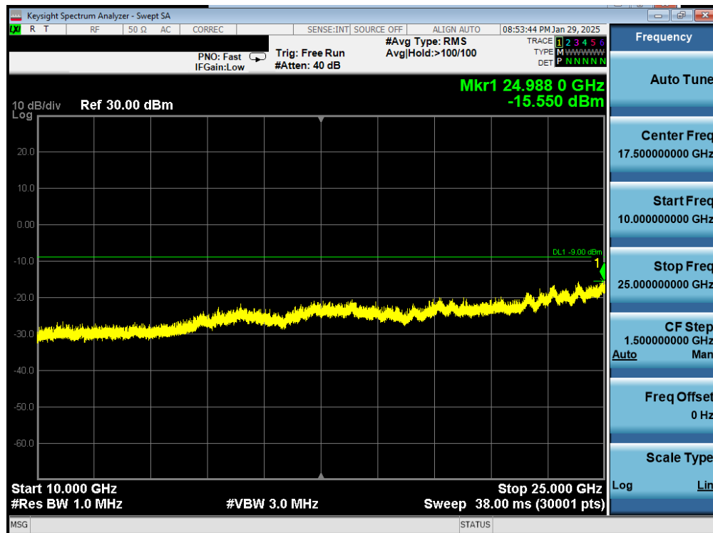
Plot 7-46. Conducted Spurious Plot Antenna 0 (Common) (Bluetooth (LE), 1Mbps, iPA – Ch. 0)
