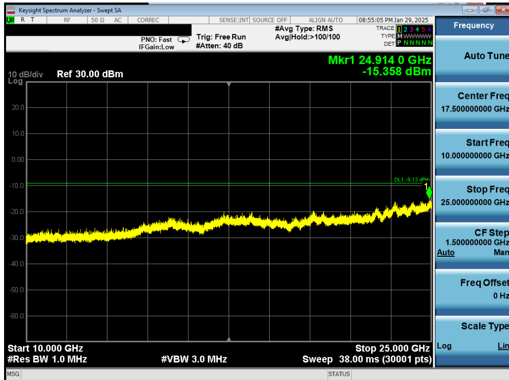
Plot 7-48. Conducted Spurious Plot Antenna 0 (Common) (Bluetooth (LE), 1Mbps, iPA – Ch. 19)
