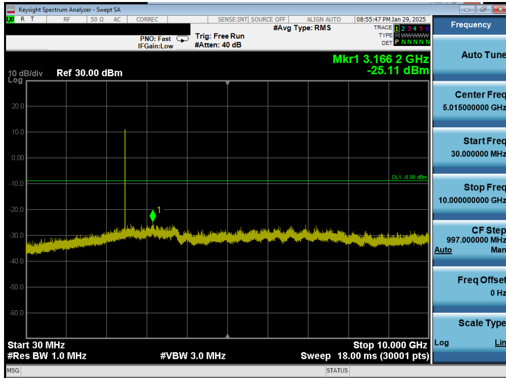
Plot 7-49. Conducted Spurious Plot Antenna 0 (Common) (Bluetooth (LE), 1Mbps, iPA – Ch. 39)
