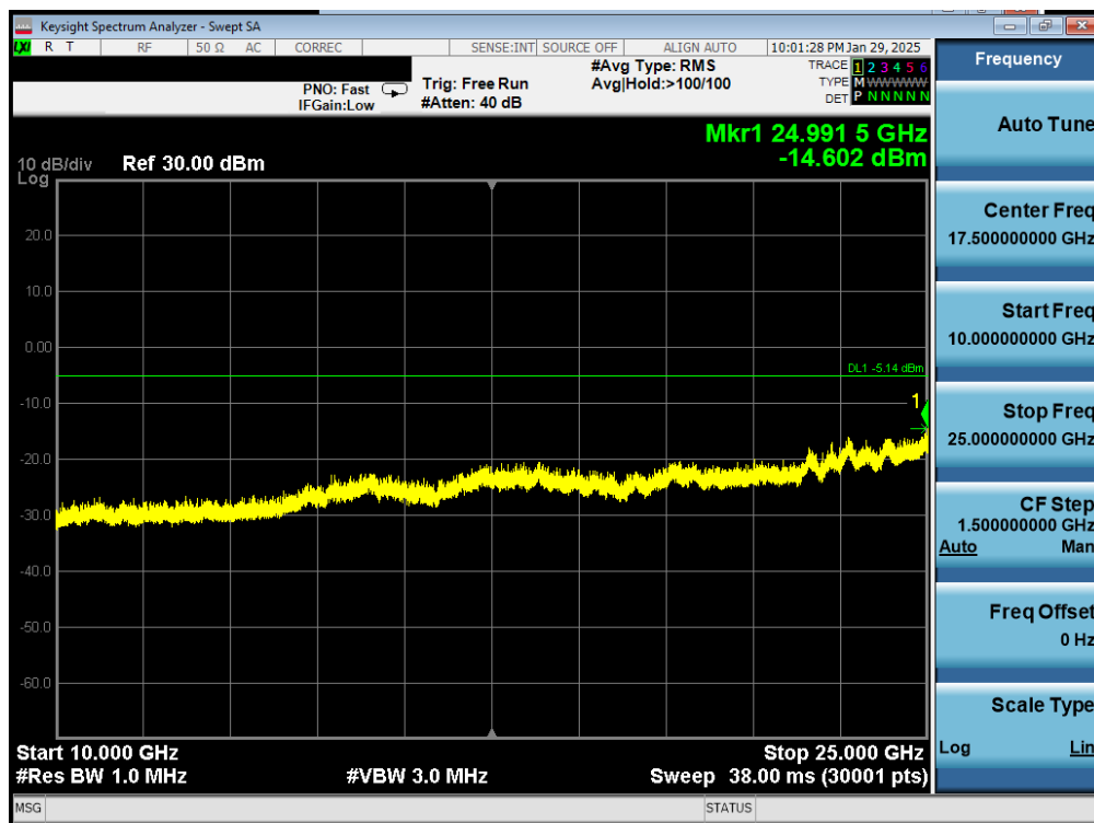
Plot 7-54. Conducted Spurious Plot Antenna 0 (Dedicated) (Bluetooth (LE), 1Mbps, iPA – Ch. 19)
