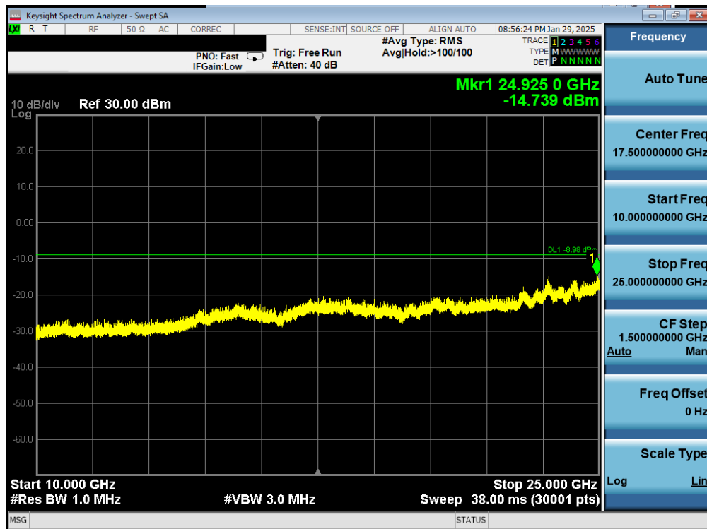
Plot 7-50. Conducted Spurious Plot Antenna 0 (Common) (Bluetooth (LE), 1Mbps, iPA – Ch. 39)
