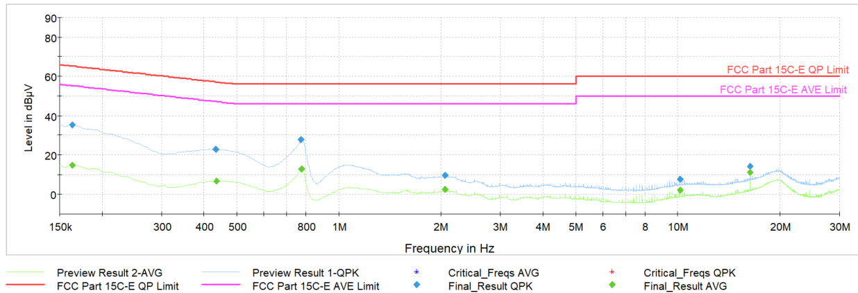
Plot 7-73. AC Line Conducted Plot with Bluetooth LE Antenna 0 Dedicated (L1, 1Mbps iPA – Ch.0 with AC/DC Adapter)
