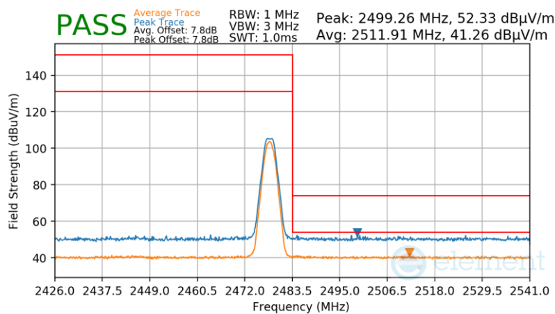
Plot 7-67. Radiated Restricted Upper Band Edge Measurement Antenna 0 (Common) (Average & Peak)
