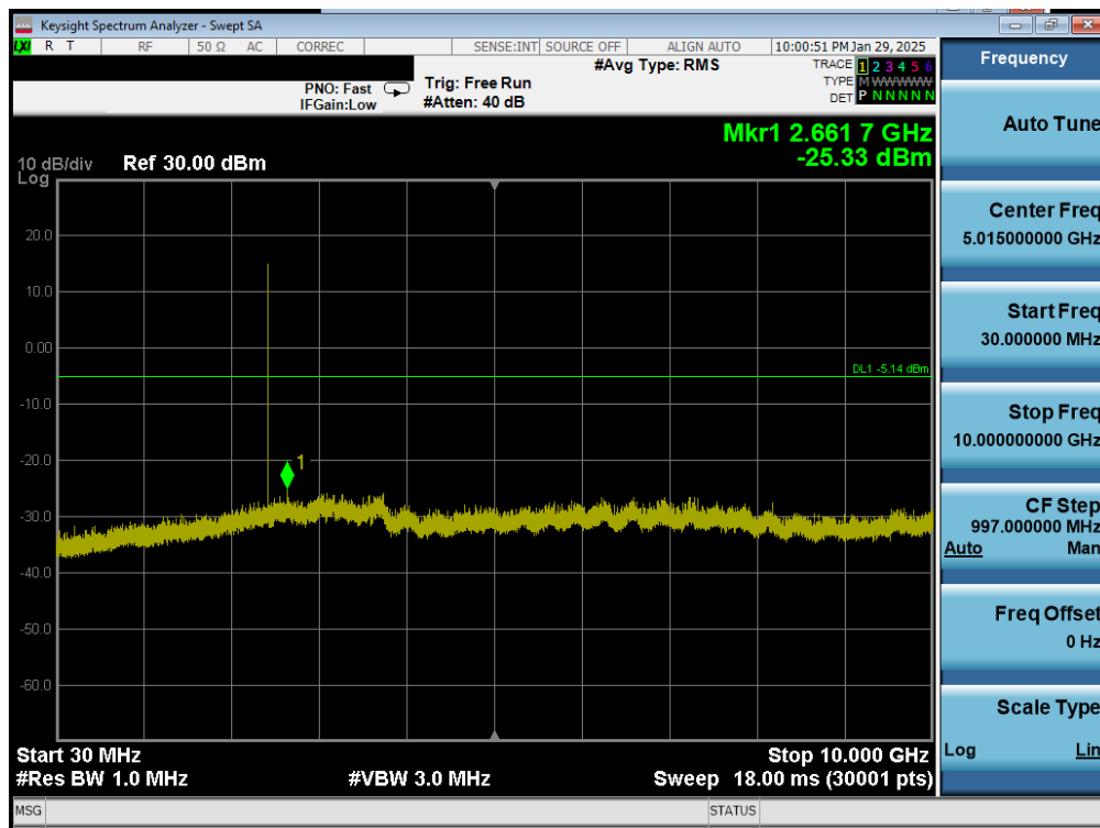
Plot 7-53. Conducted Spurious Plot Antenna 0 (Dedicated) (Bluetooth (LE), 1Mbps, iPA – Ch. 19)
