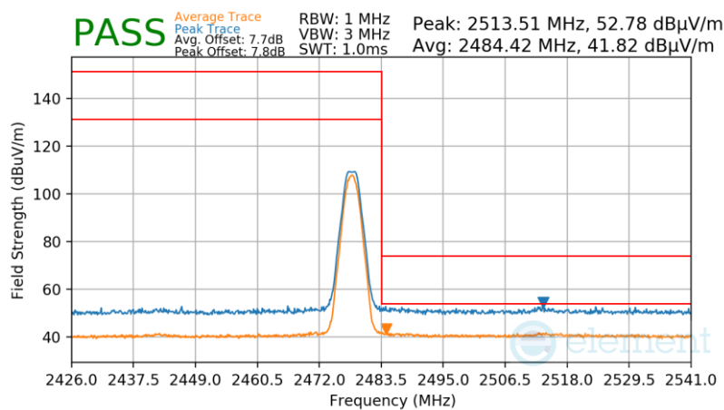
Plot 7-71. Radiated Restricted Upper Band Edge Measurement Antenna 0 (Dedicated) (Average & Peak)
