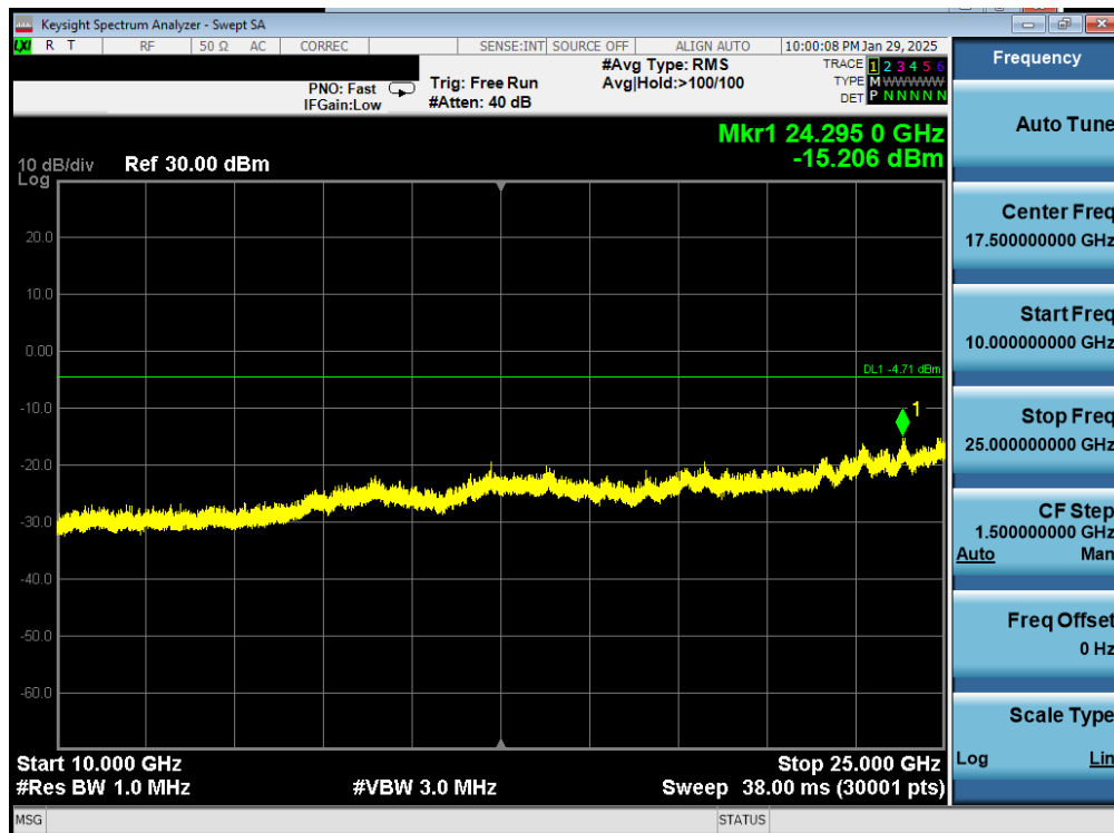
Plot 7-52. Conducted Spurious Plot Antenna 0 (Dedicated) (Bluetooth (LE), 1Mbps, iPA – Ch. 0)
