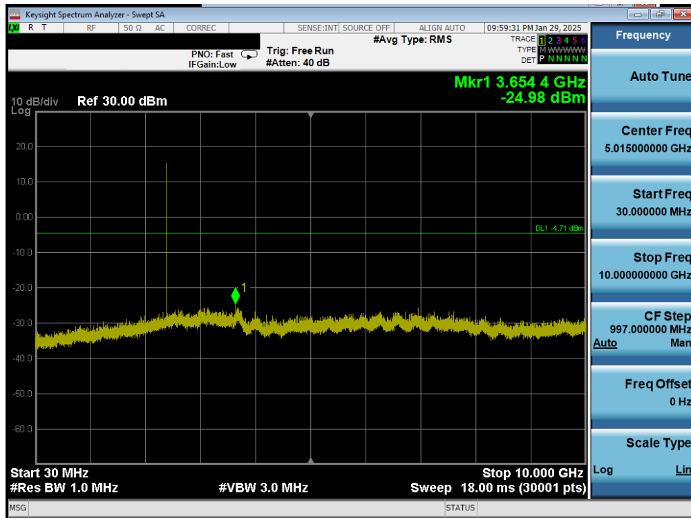
Plot 7-51. Conducted Spurious Plot Antenna 0 (Dedicated) (Bluetooth (LE), 1Mbps, iPA – Ch. 0)
