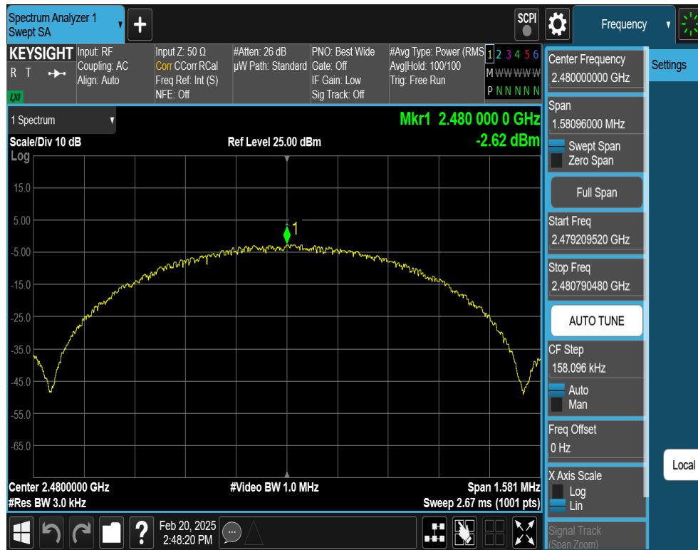
Plot 7-33. Power Spectral Density Plot Antenna 0 (Dedicated) (Bluetooth (LE), 1Mbps, iPA – Ch. 39)
