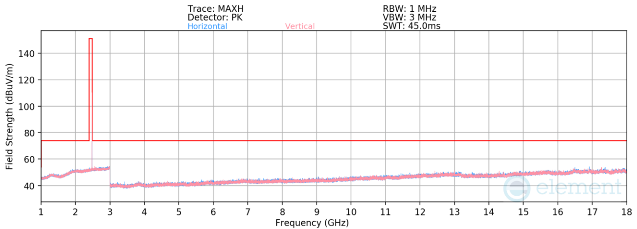
Plot 7-63. Radiated Spurious Emissions 1-18GHz Antenna 0 (Dedicated) (1Mbps iPA – Ch. 39)
