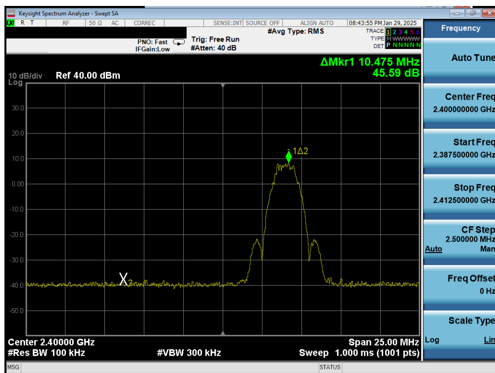
Plot 7-39. Band Edge Plot Antenna 0 (Common) (Bluetooth (LE), 2Mbps, iPA – Ch. 1)
