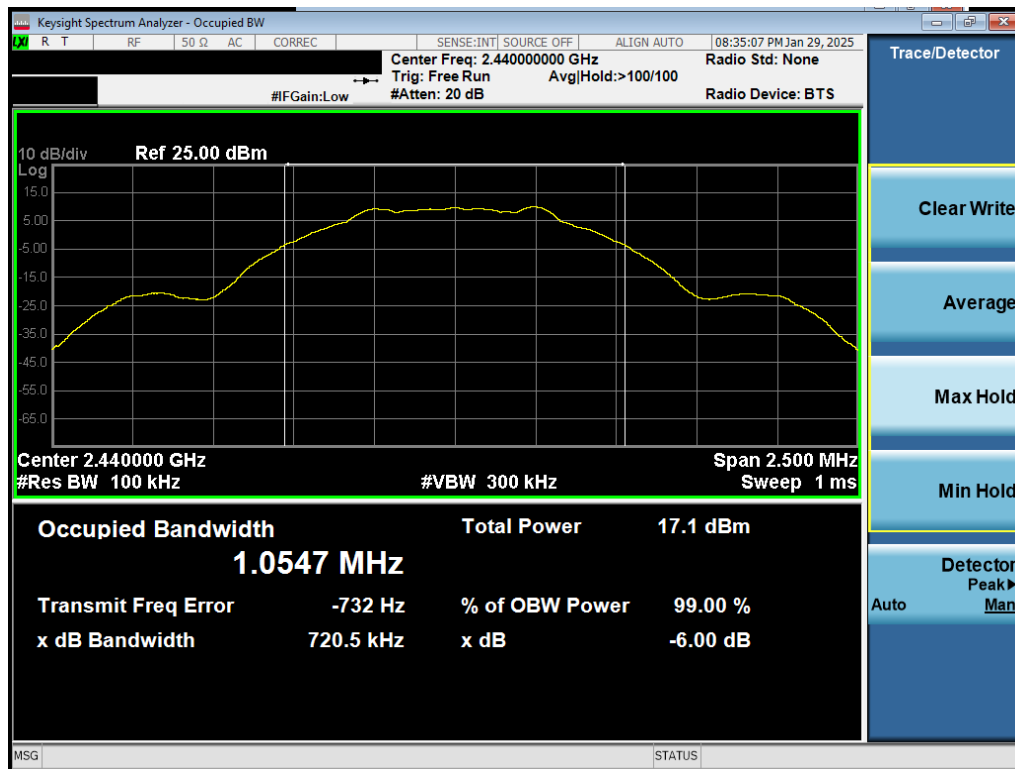
Plot 7-14. 6dB BW Plot Antenna 0 (Common) (Bluetooth (LE), 1Mbps, iPA – Ch. 19)
