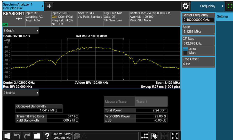
Plot 7-7. 99% OBW Plot Antenna 0 (Dedicated) (Bluetooth (LE), 1Mbps, iPA – Ch. 0)
