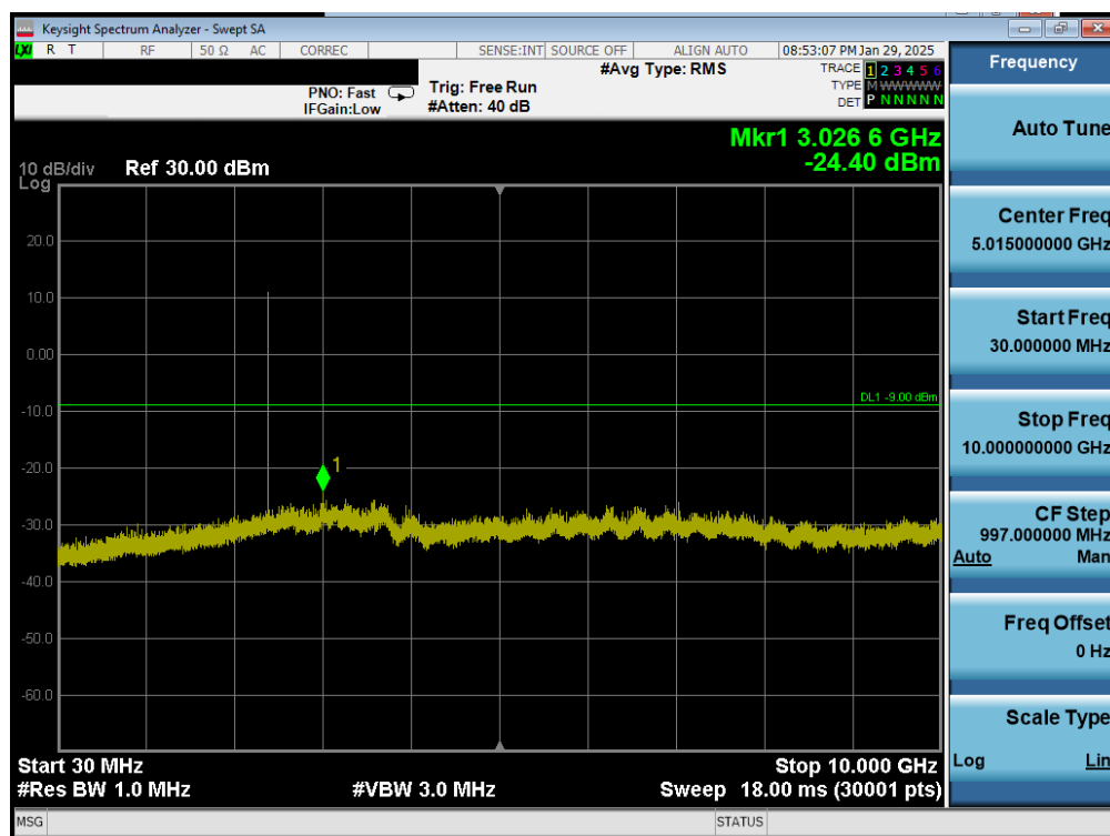
Plot 7-45. Conducted Spurious Plot Antenna 0 (Common) (Bluetooth (LE), 1Mbps, iPA – Ch. 0)
