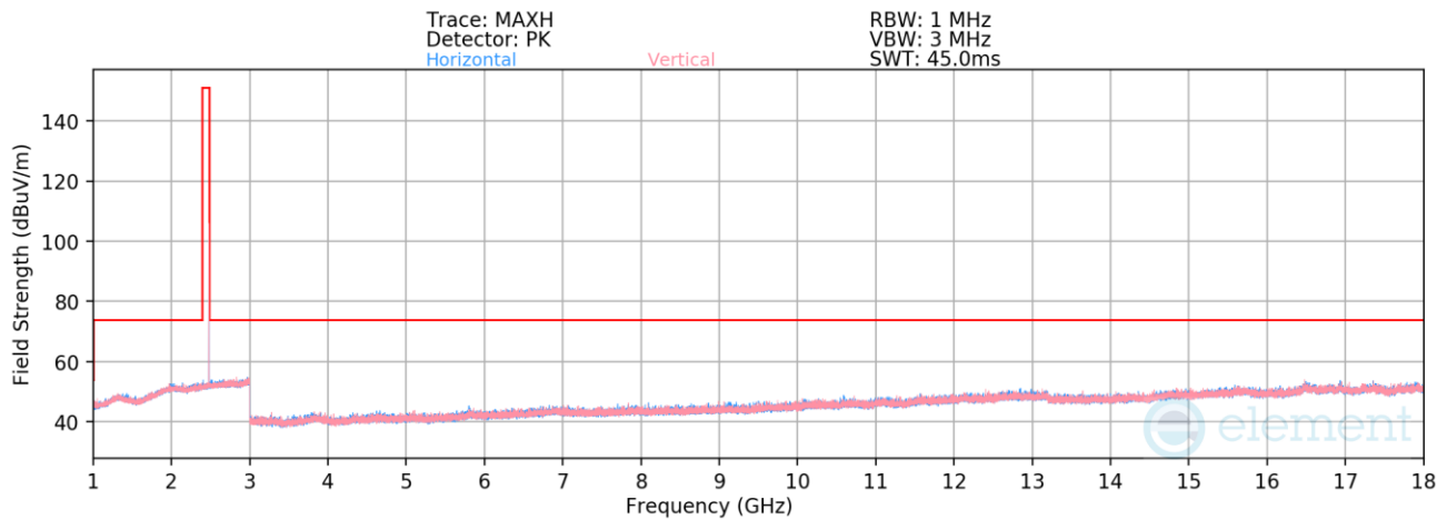
Plot 7-59. Radiated Spurious Emissions 1-18GHz Antenna 0 (Common) (1Mbps iPA – Ch. 39)
