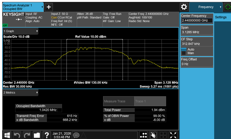
Plot 7-8. 99% OBW Plot Antenna 0 (Dedicated) (Bluetooth (LE), 1Mbps, iPA – Ch. 19)
