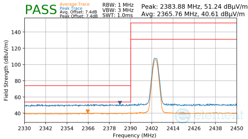
Plot 7-66. Radiated Restricted Lower Band Edge Measurement Antenna 0 (Common) (Average & Peak)
