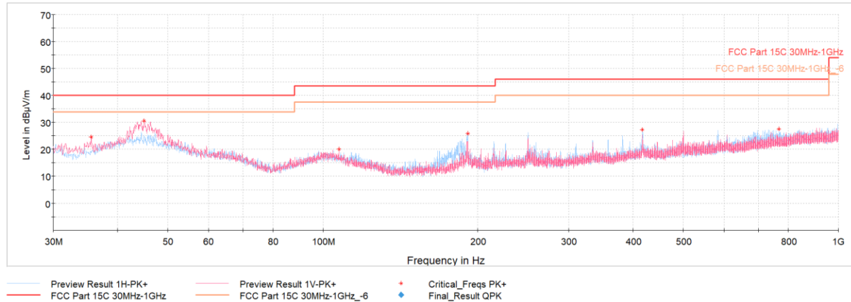
Plot 7-72. Radiated Spurious Emissions Below 1GHz Antenna 0 Dedicated (1Mbps, iPA – Ch.0, Pol. H & V, with AC/DC Adapter)
