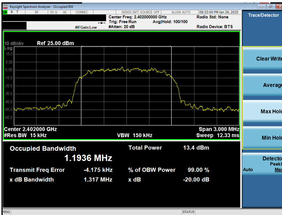
Plot 7-4. 20dB BW and 99% OBW Plot Antenna 0 (Common) (Bluetooth, 8DPSK, iPA – Ch. 0)
