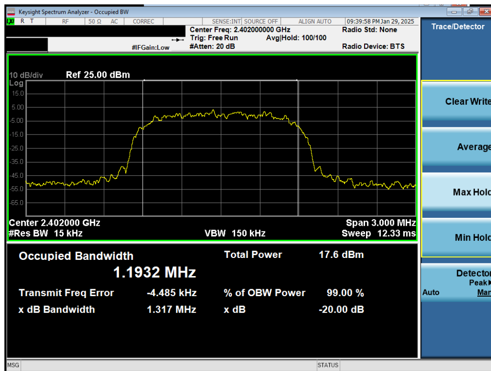
Plot 7-10. 20dB BW and 99% OBW Plot Antenna 0 (Dedicated) (Bluetooth, 8DPSK, iPA – Ch. 0)
