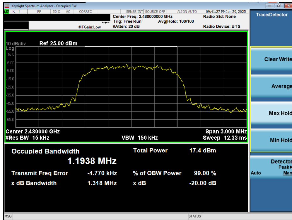
Plot 7-12. 20dB BW and 99% OBW Plot Antenna 0 (Dedicated) (Bluetooth, 8DPSK, iPA – Ch. 78)
