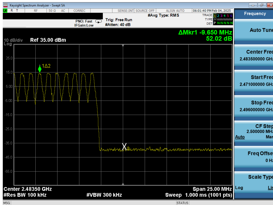
Plot 7-24. Band Edge Plot Antenna 0 (Dedicated) (Bluetooth with Hopping Enabled, GFSK, iPA – Ch.78)
