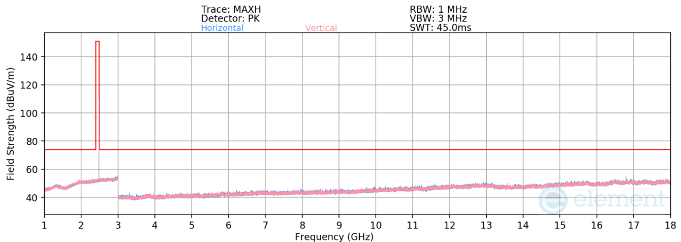
Plot 7-64. Radiated Spurious Emissions above 1GHz Antenna 0 (Dedicated) (BT GFSK iPA – Ch. 78)
