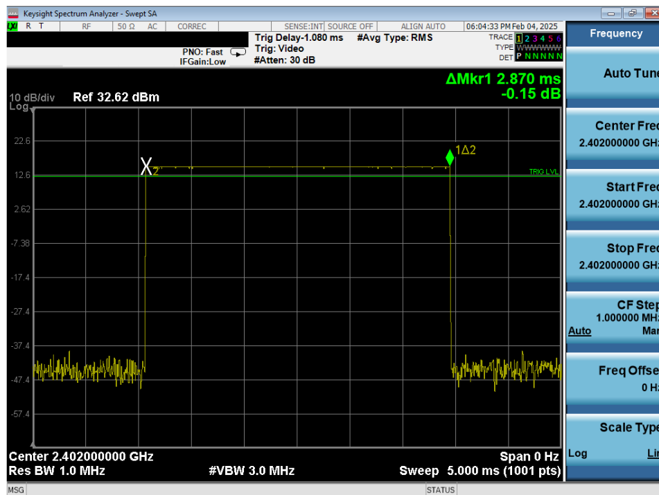
Plot 7-35. Time of Occupancy Plot Antenna 0 (Dedicated) (Bluetooth, GFSK, iPA)
