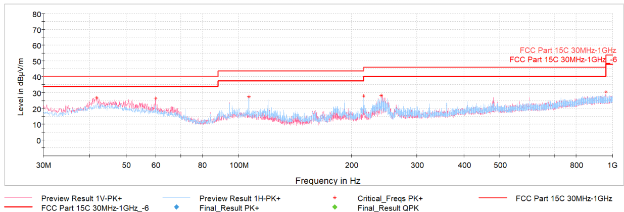
Plot 7-73. Radiated Spurious Emissions Below 1GHz Antenna 0 (Dedicated) (GFSK iPA – Ch.0, with AC/DC Adapter via USB-C cable wire charger)
