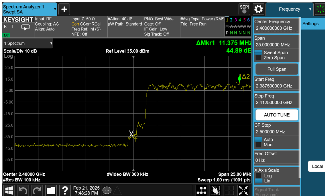
Plot 7-19. Band Edge Plot Antenna 0 (Common) (Bluetooth with Hopping Enabled, 8DPSK, iPA – Ch. 0)
