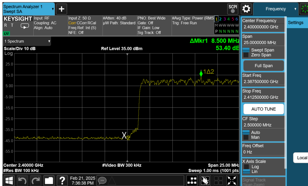
Plot 7-27. Band Edge Plot Antenna 0 (Dedicated) (Bluetooth with Hopping Enabled, 8DPSK, iPA – Ch.0)
