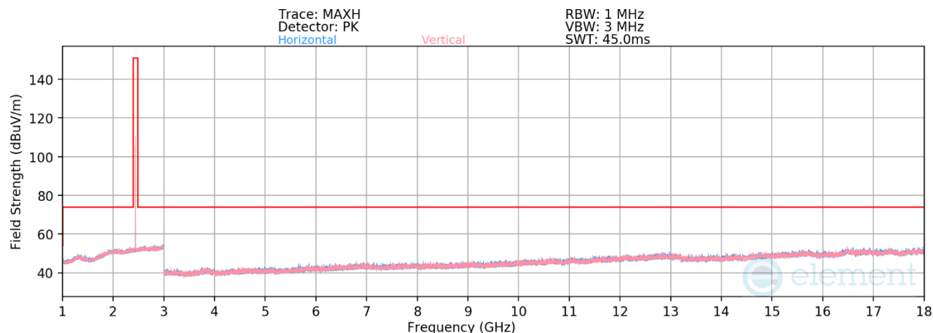
Plot 7-62. Radiated Spurious Emissions above 1GHz Antenna 0 (Dedicated) (BT GFSK iPA – Ch. 39)
