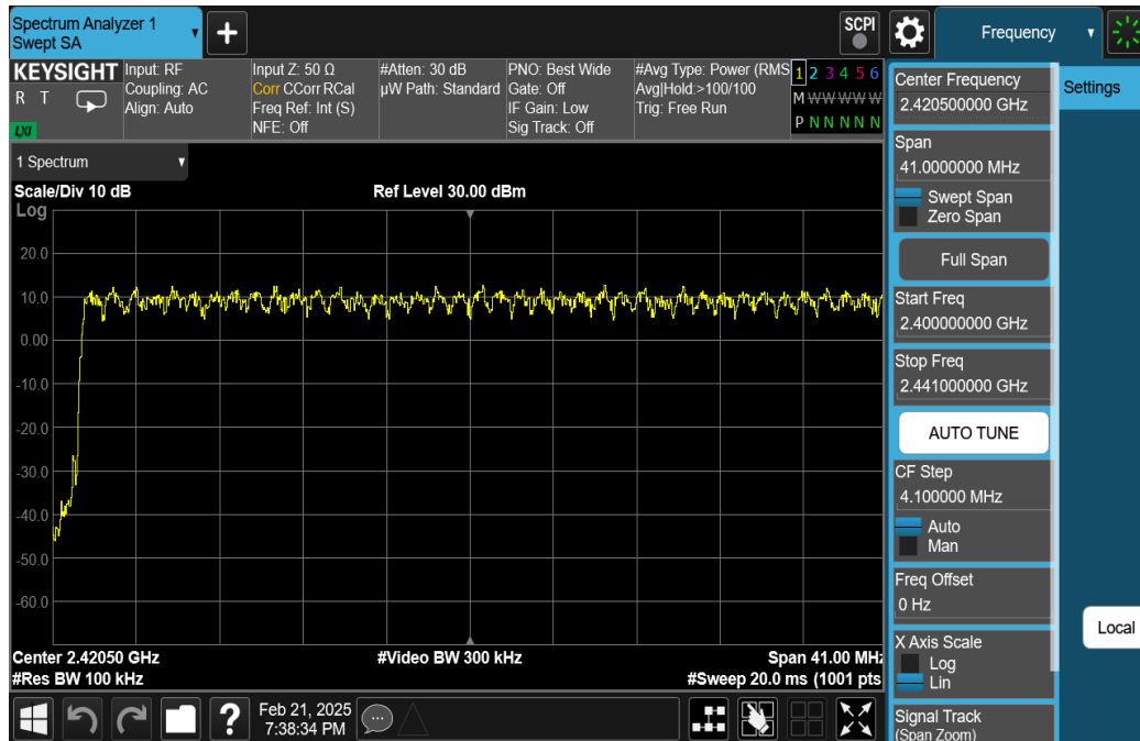
Plot 7-43. Low End Spectrum Channel Hopping Plot Antenna 0 (Dedicated) (Bluetooth, 8DPSK, iPA)
