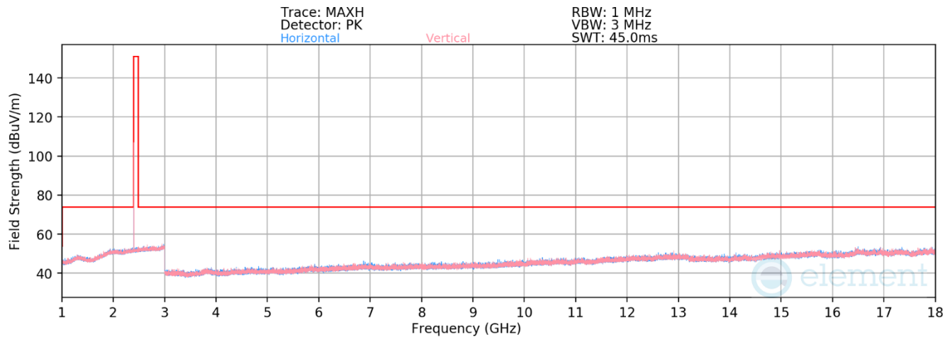
Plot 7-57. Radiated Spurious Emissions above 1GHz Antenna 0 (Common) (BT GFSK iPA – Ch. 0)
