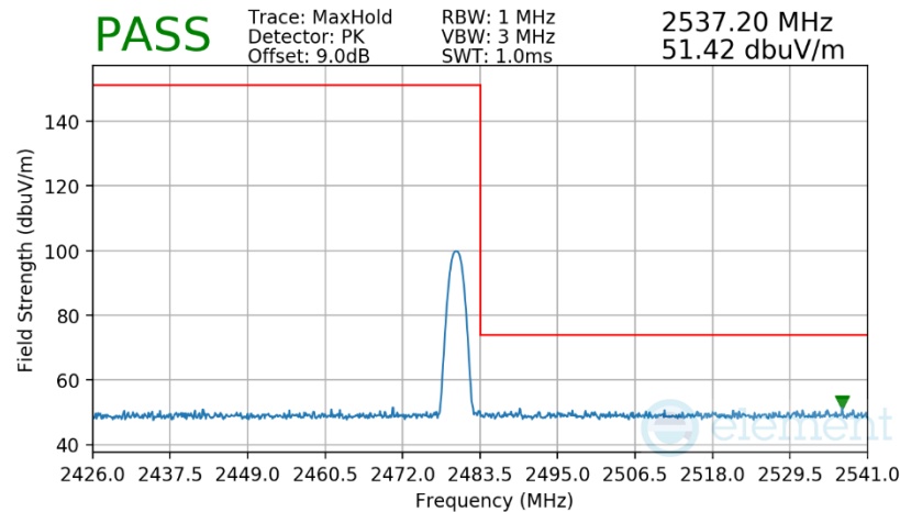
Plot 7-67. Radiated Restricted Upper Band Edge Measurement Antenna 0 (Common)
