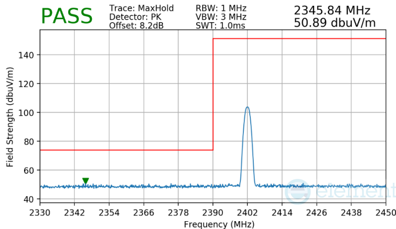
Plot 7-69. Radiated Restricted Lower Band Edge Measurement Antenna 0 (Dedicated)
