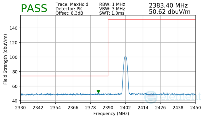
Plot 7-65. Radiated Restricted Lower Band Edge Measurement Antenna 0 (Common)
