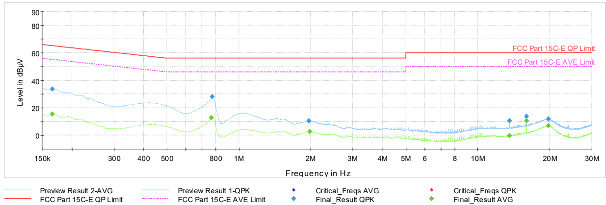
Plot 7-74. AC Line-Conducted Test Plot Antenna 0 (Dedicated) (L1, GFSK iPA – Ch.0, with AC/DC Adapter via USB-C cable wire charger)
