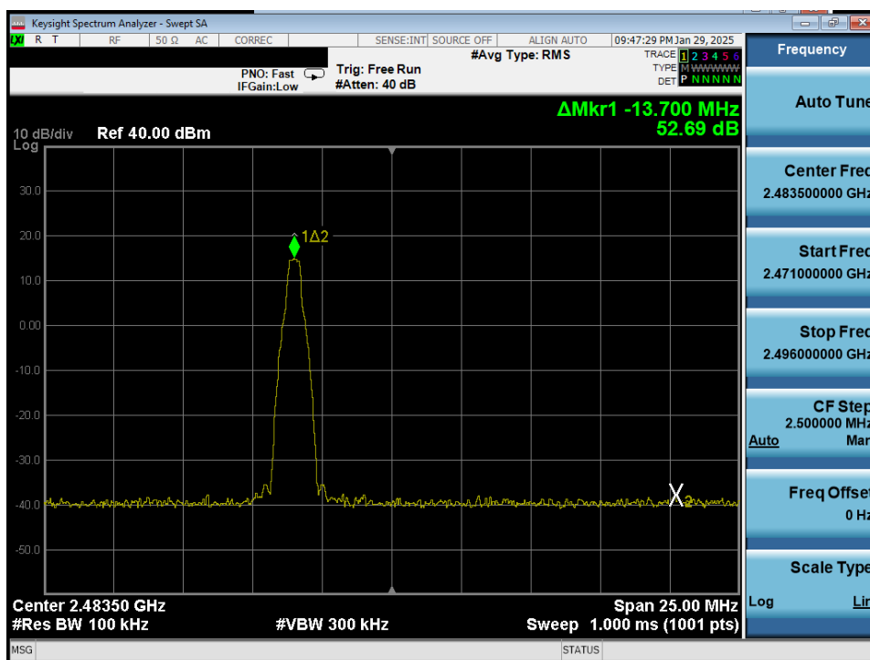
Plot 7-22. Band Edge Plot Antenna 0 (Dedicated) (Bluetooth with Hopping Disabled, GFSK, iPA – Ch.78)
