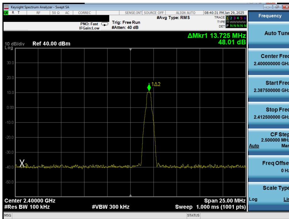
Plot 7-13. Band Edge Plot Antenna 0 (Common) (Bluetooth with Hopping Disabled, GFSK, iPA – Ch.0)
