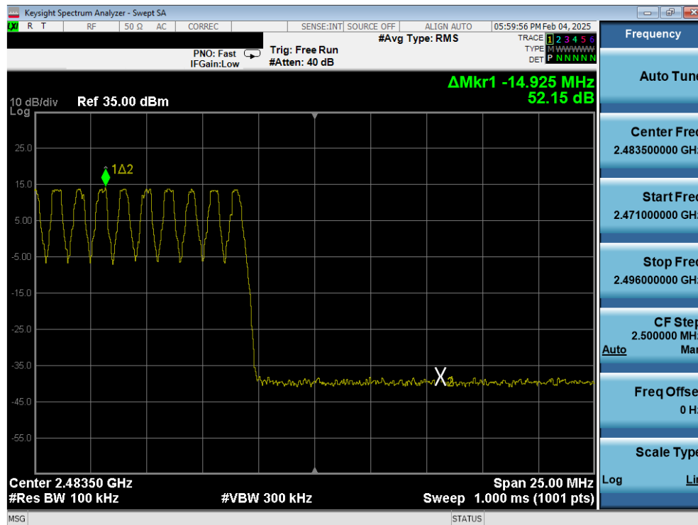
Plot 7-16. Band Edge Plot Antenna 0 (Common) (Bluetooth with Hopping Enabled, GFSK, iPA – Ch.78)
