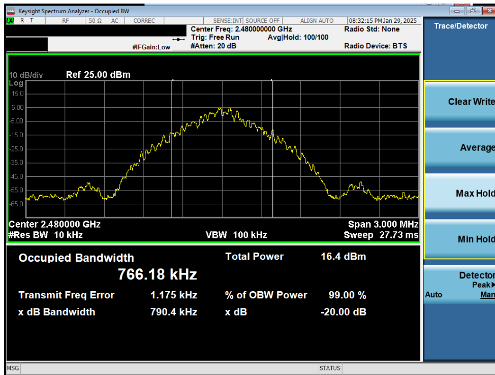
Plot 7-3. 20dB BW and 99% OBW Plot Antenna 0 (Common) (Bluetooth, GFSK, iPA – Ch. 78)
