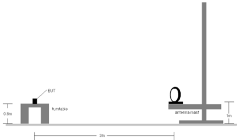
Figure 7-9. Radiated Test Setup < 30MHz
