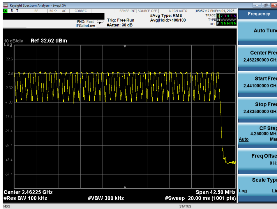
Plot 7-38. High End Spectrum Channel Hopping Plot Antenna 0 (Common) (Bluetooth, GFSK, iPA)
