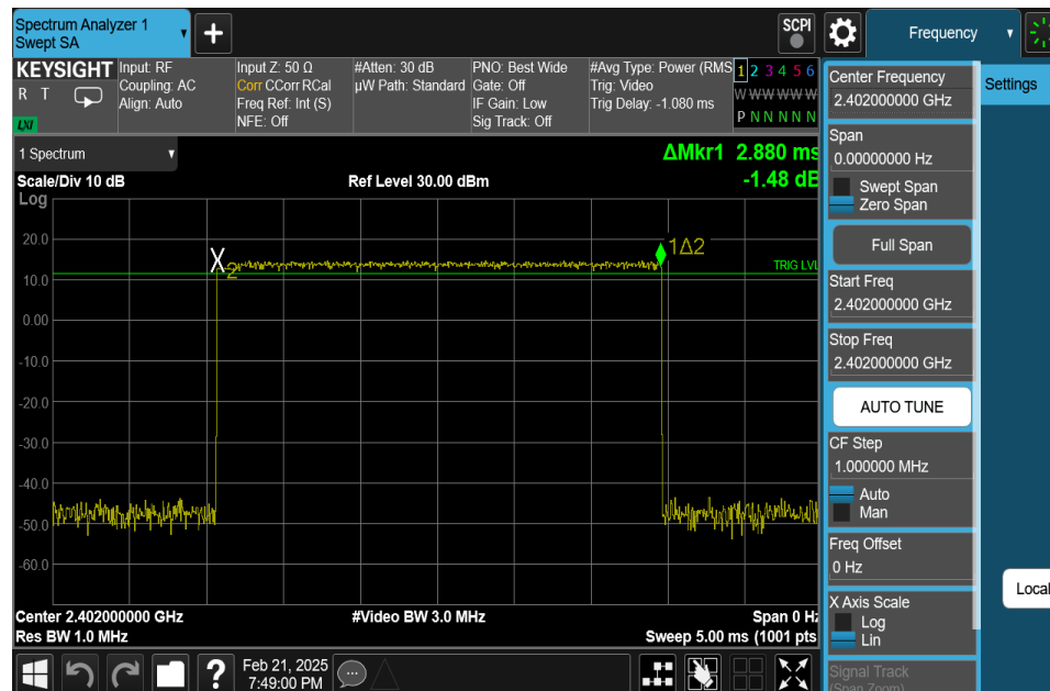
Plot 7-34. Time of Occupancy Plot Antenna 0 (Common) (Bluetooth, 8DPSK, iPA)
