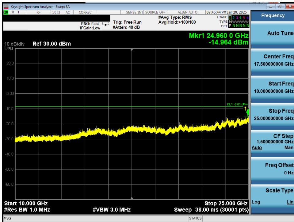
Plot 7-46. Conducted Spurious Plot Antenna 0 (Common) (Bluetooth, GFSK, iPA – Ch. 0)
