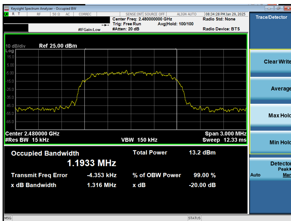
Plot 7-6. 20Db BW and 99% OBW Plot Antenna 0 (Common) (Bluetooth, 8DPSK, iPA – Ch. 78)
