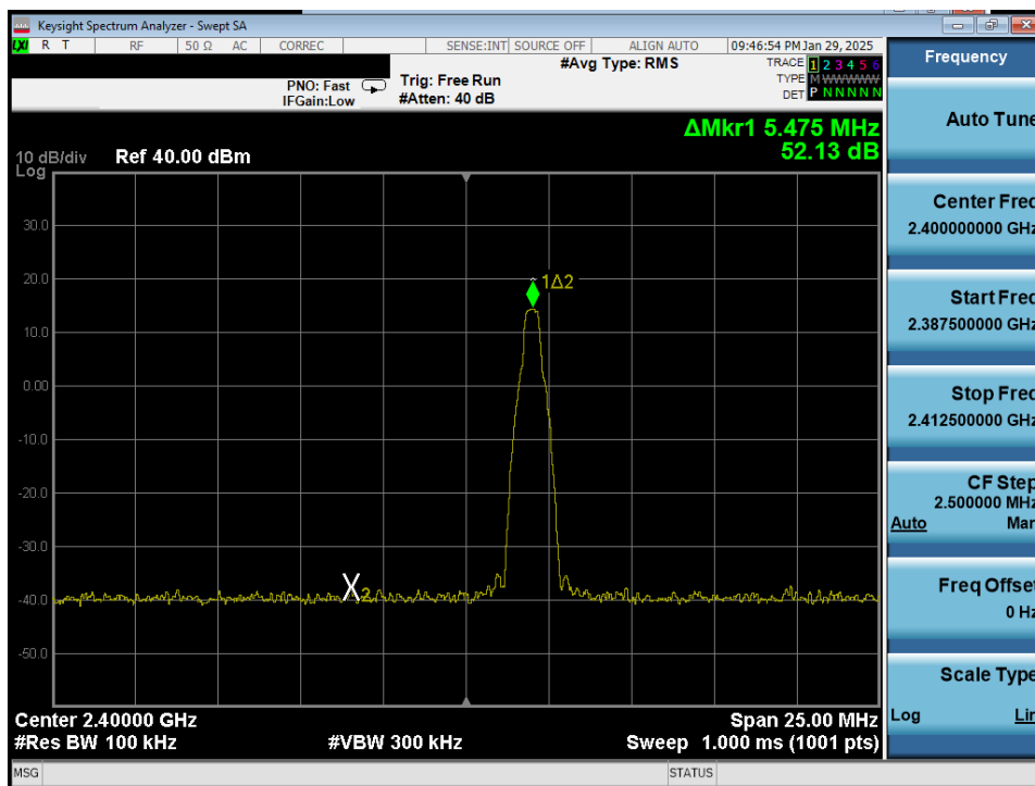
Plot 7-21. Band Edge Plot Antenna 0 (Dedicated) (Bluetooth with Hopping Disabled, GFSK, iPA – Ch.0)
