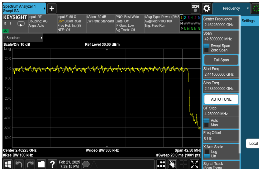
Plot 7-44. High End Spectrum Channel Hopping Plot Antenna 0 (Dedicated) (Bluetooth, 8DPSK, iPA)
