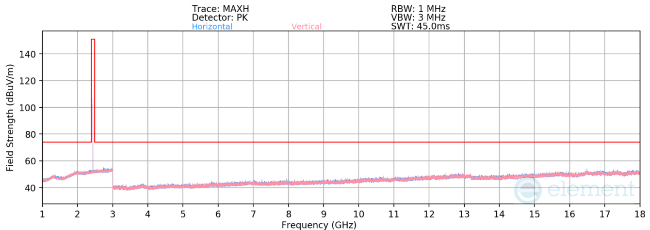
Plot 7-58. Radiated Spurious Emissions above 1GHz Antenna 0 (Common) (BT GFSK iPA – Ch. 39)
