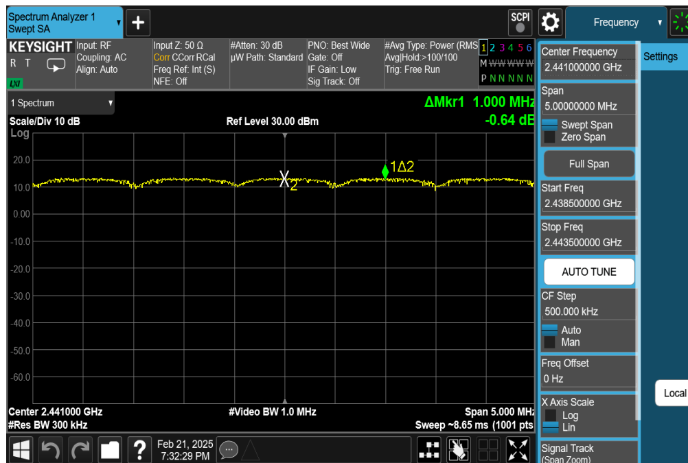
Plot 7-32. Channel Spacing Plot Antenna 0 (Dedicated) (Bluetooth, 8DPSK, iPA)
