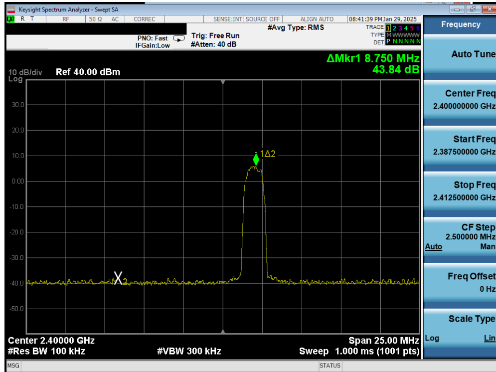
Plot 7-17. Band Edge Plot Antenna 0 (Common) (Bluetooth with Hopping Disabled, 8DPSK, iPA – Ch. 0)
