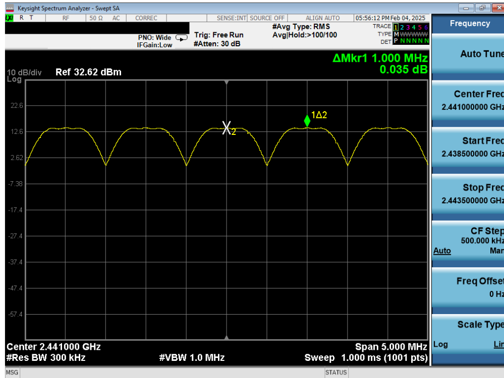
Plot 7-29. Channel Spacing Plot Antenna 0 (Common) (Bluetooth, GFSK, iPA)
