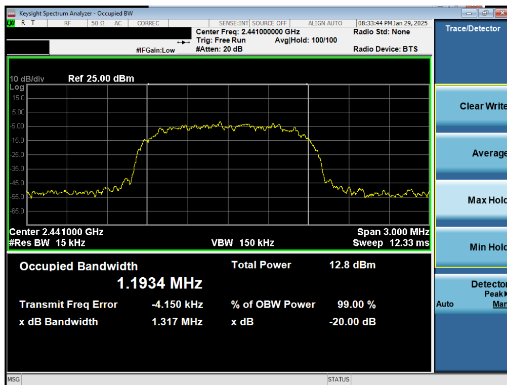
Plot 7-5. 20Db BW and 99% OBW Plot Antenna 0 (Common) (Bluetooth, 8DPSK, iPA – Ch. 39)
