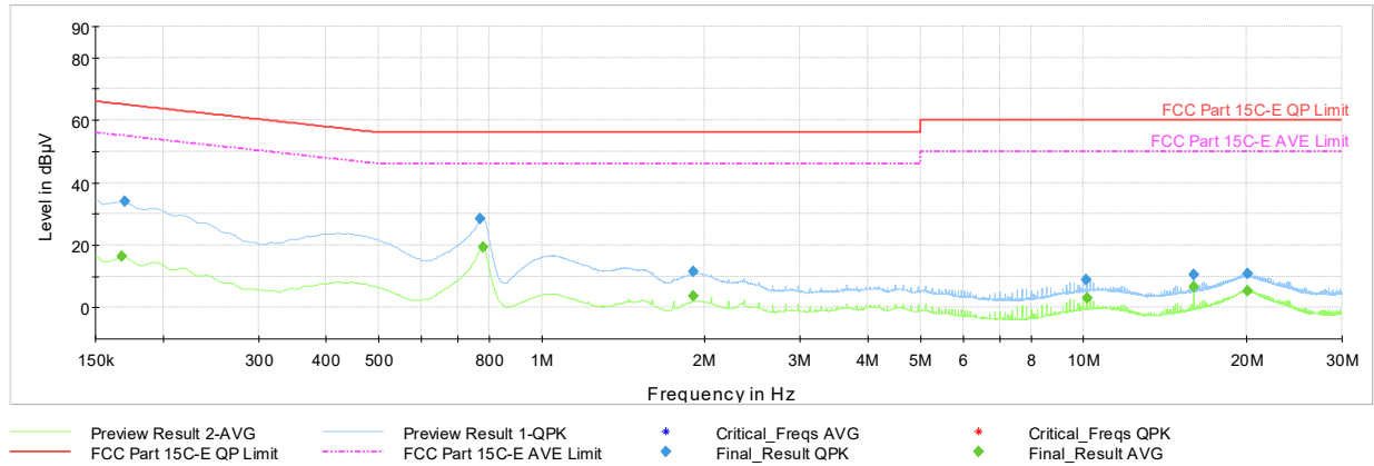
Plot 7-75. AC Line-Conducted Test Plot Antenna 0 (Dedicated) (N, GFSK iPA – Ch.0, with AC/DC Adapter via USB-C cable wire charger)
