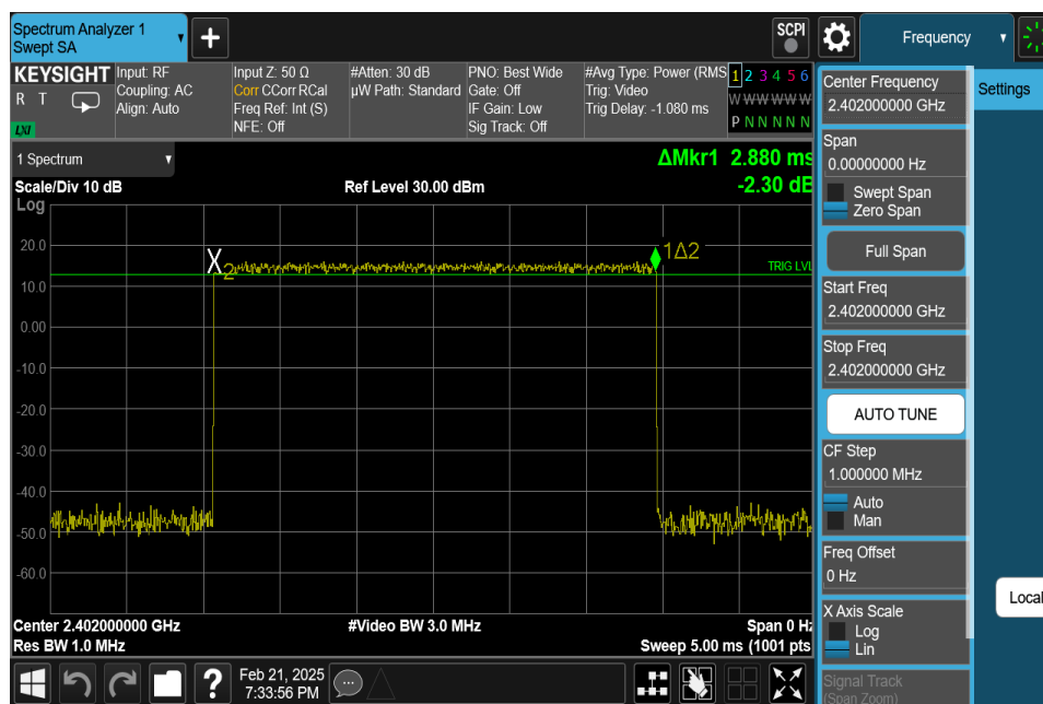
Plot 7-36. Time of Occupancy Plot Antenna 0 (Dedicated) (Bluetooth, 8DPSK, iPA)
