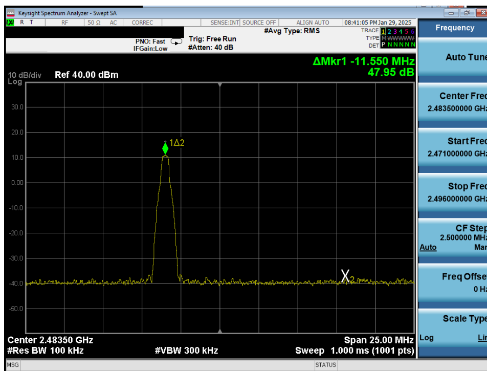
Plot 7-14. Band Edge Plot Antenna 0 (Common) (Bluetooth with Hopping Disabled, GFSK, iPA - Ch.78)
