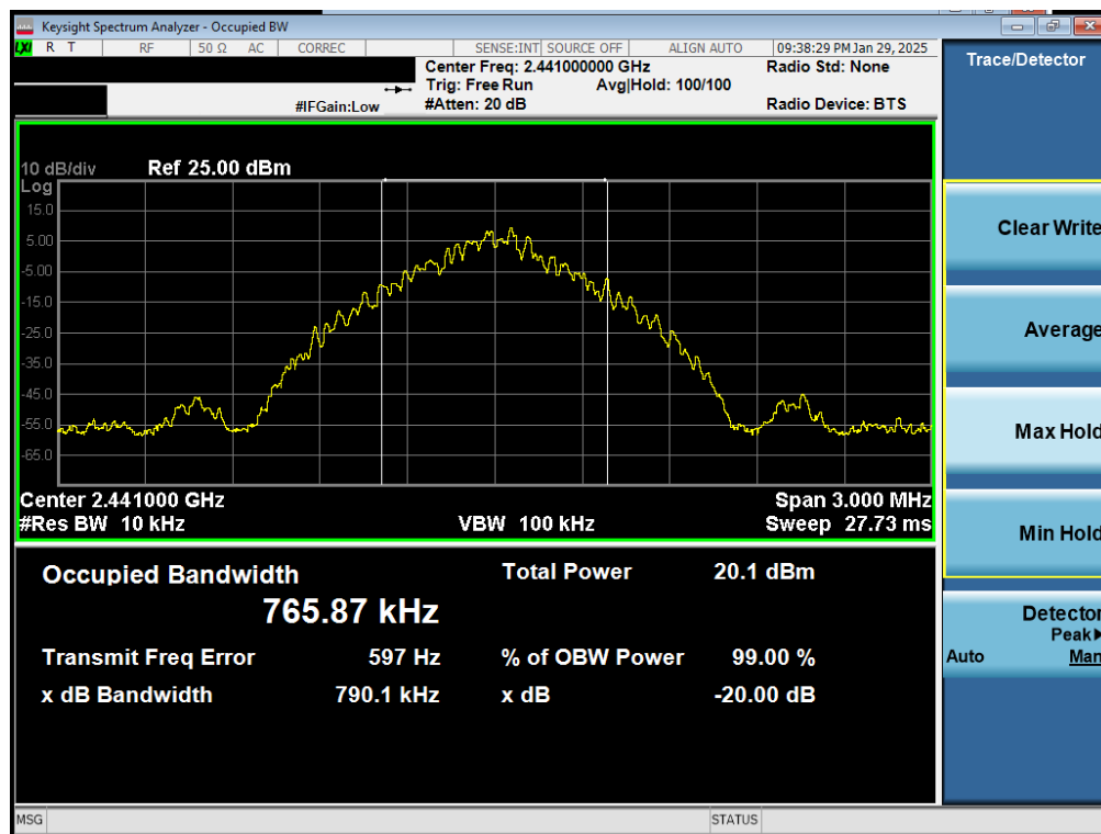
Plot 7-8. 20dB BW and 99% OBW Plot Antenna 0 (Dedicated) (Bluetooth, GFSK, iPA – Ch. 39)
