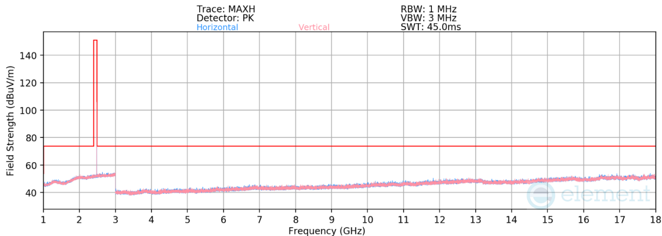
Plot 7-59. Radiated Spurious Emissions above 1GHz Antenna 0 (Common) (BT GFSK iPA – Ch. 78)
