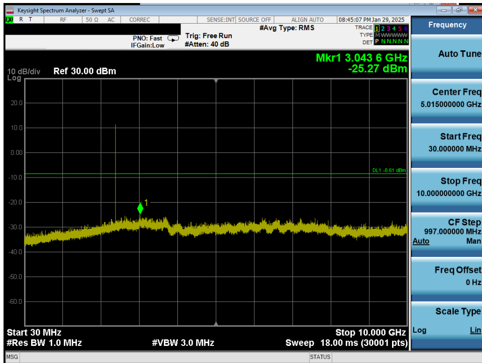
Plot 7-45. Conducted Spurious Plot Antenna 0 (Common) (Bluetooth, GFSK, iPA – Ch. 0)
