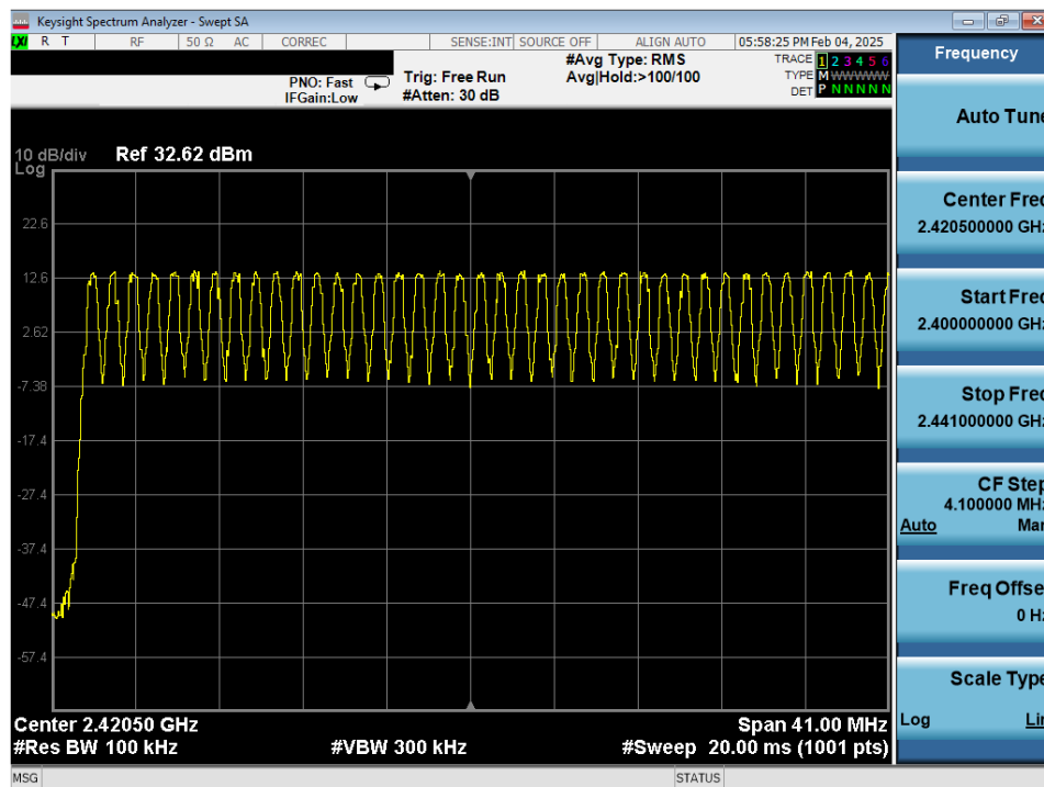
Plot 7-37. Low End Spectrum Channel Hopping Plot Antenna 0 (Common) (Bluetooth, GFSK, iPA)
