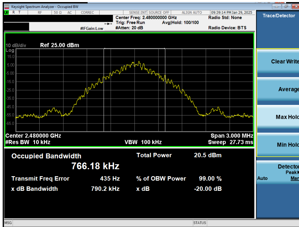
Plot 7-9. 20dB BW and 99% OBW Plot Antenna 0 (Dedicated) (Bluetooth, GFSK, iPA – Ch. 78)
