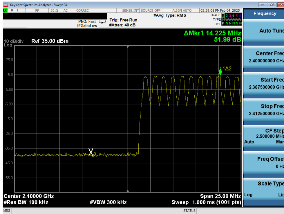
Plot 7-15. Band Edge Plot Antenna 0 (Common) (Bluetooth with Hopping Enabled, GFSK, iPA – Ch. 0)
