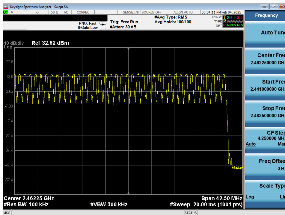
Plot 7-42. High End Spectrum Channel Hopping Plot Antenna 0 (Dedicated) (Bluetooth, GFSK, iPA)
