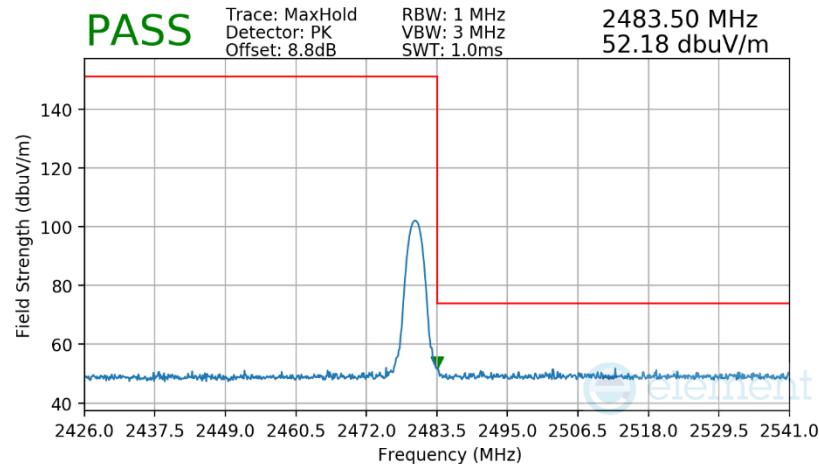
Plot 7-68. Radiated Restricted Upper Band Edge Measurement Antenna 0 (Common)
