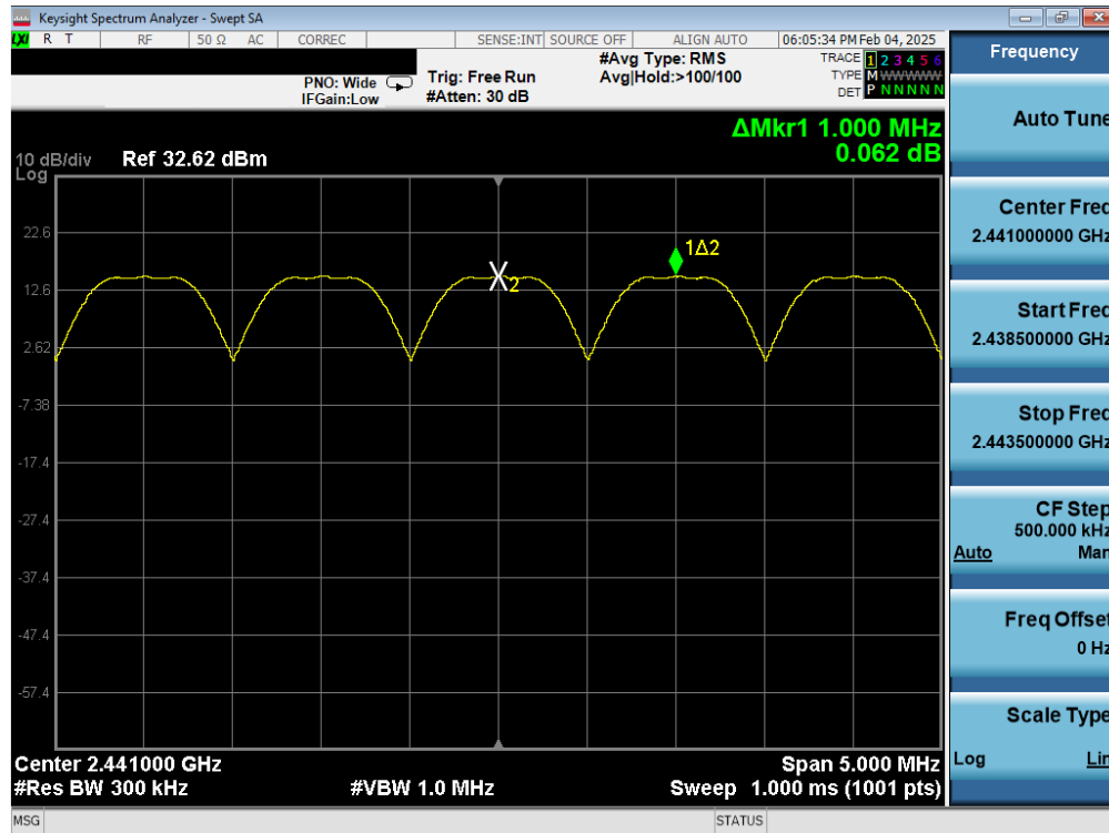
Plot 7-31. Channel Spacing Plot Antenna 0 (Dedicated) (Bluetooth, GFSK, iPA)
