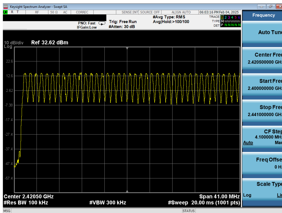
Plot 7-41. Low End Spectrum Channel Hopping Plot Antenna 0 (Dedicated) (Bluetooth, GFSK, iPA)
