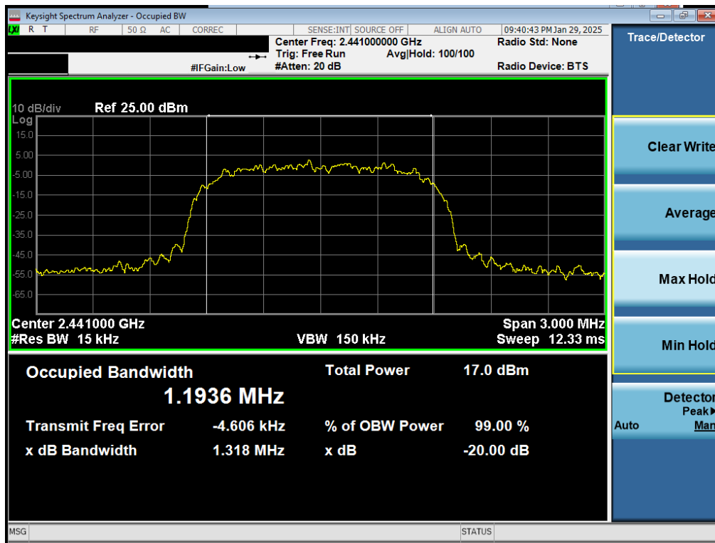
Plot 7-11. 20dB BW and 99% OBW Plot Antenna 0 (Dedicated) (Bluetooth, 8DPSK, iPA – Ch. 39)
