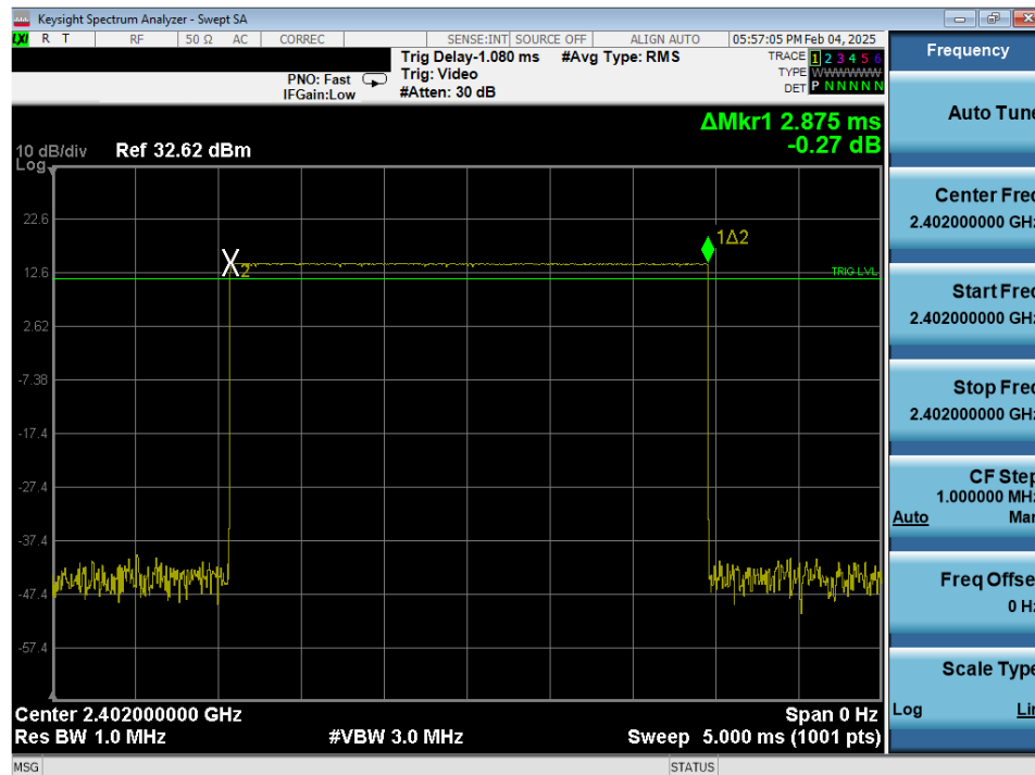
Plot 7-33. Time of Occupancy Plot Antenna 0 (Common) (Bluetooth, GFSK, iPA)
