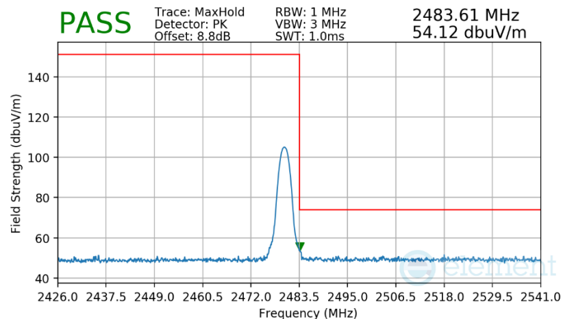
Plot 7-72. Radiated Restricted Upper Band Edge Measurement Antenna 0 (Dedicated)
