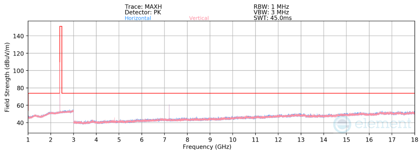
Plot 7-61. Radiated Spurious Emissions above 1GHz Antenna 0 (Dedicated) (BT GFSK iPA – Ch. 0)
