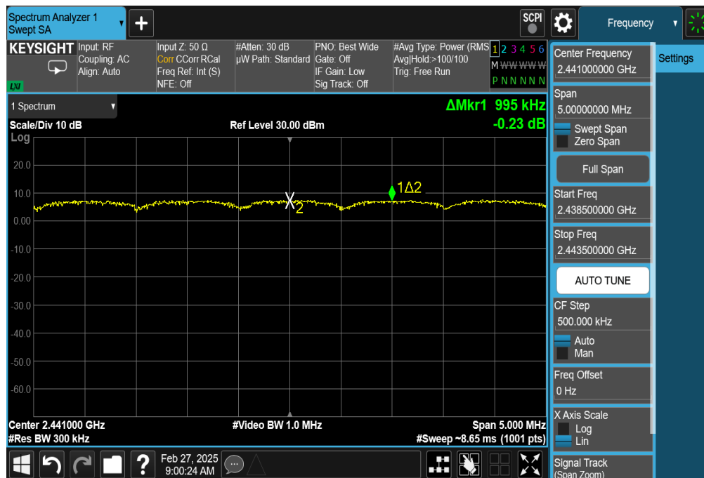
Plot 7-30. Channel Spacing Plot Antenna 0 (Common) (Bluetooth, 8DPSK, iPA)
