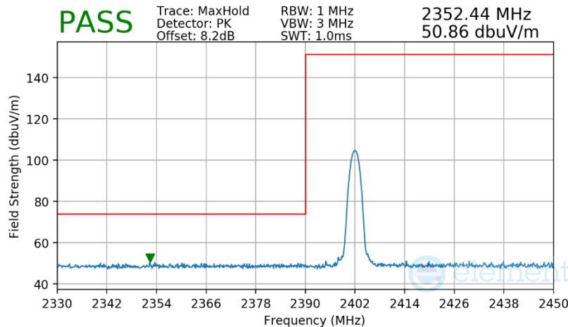
Plot 7-70. Radiated Restricted Lower Band Edge Measurement Antenna 0 (Dedicated)
