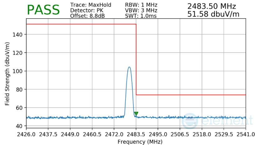
Plot 7-71. Radiated Restricted Upper Band Edge Measurement Antenna 0 (Dedicated)
