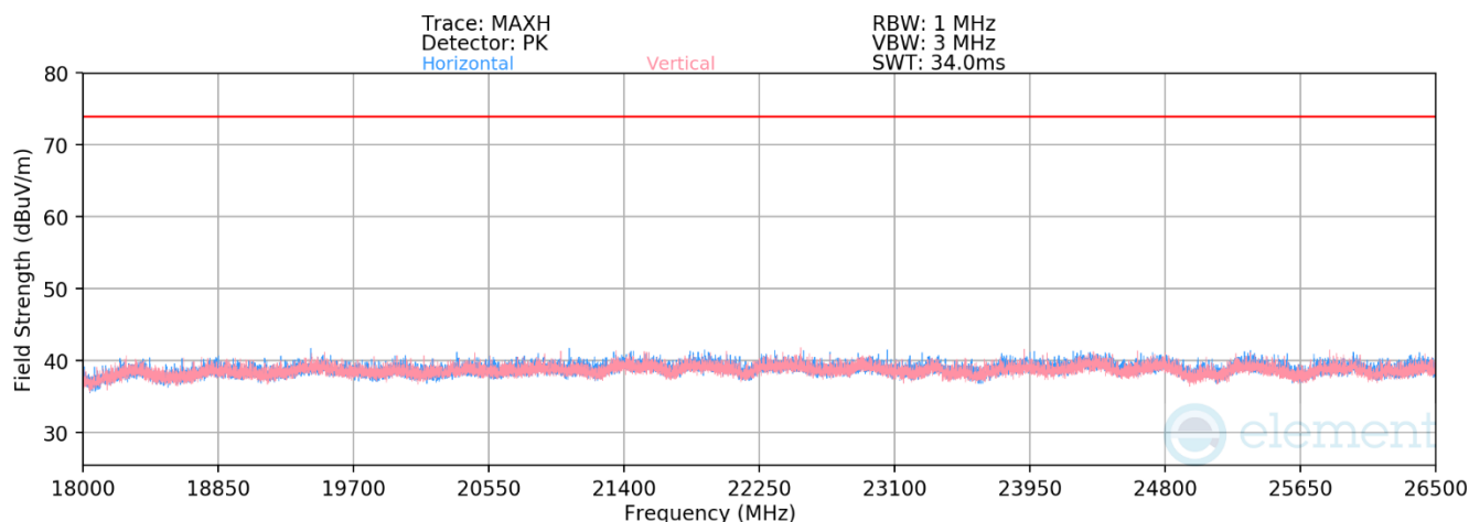
Plot 7-60. Radiated Spurious Emissions above 18GHz Antenna 0 (Common) (BT GFSK iPA – Ch. 78)
