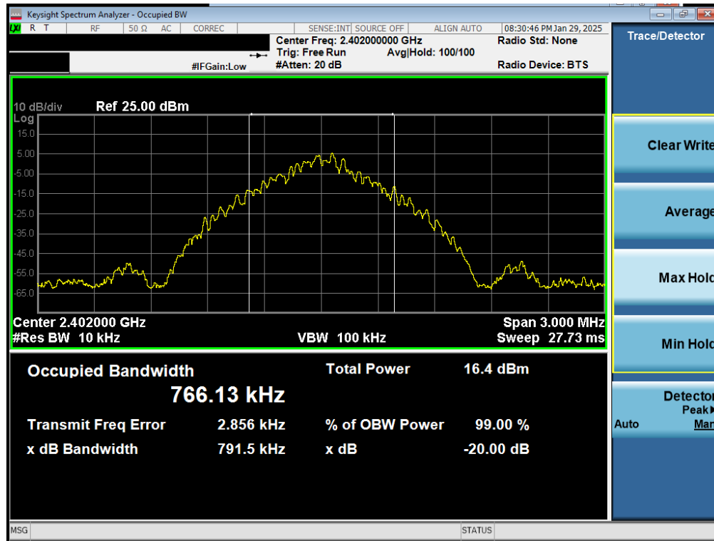
Plot 7-1. 20Db BW and 99% OBW Plot Antenna 0 (Common) (Bluetooth, GFSK, iPA – Ch. 0)
