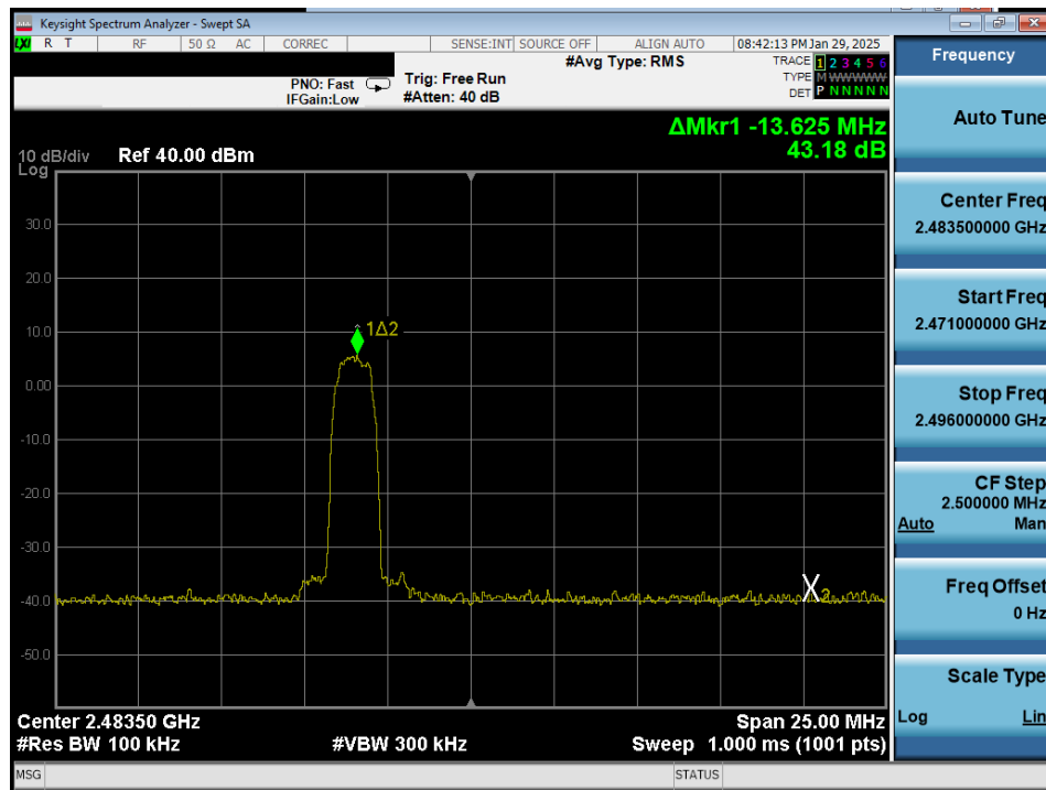
Plot 7-18. Band Edge Plot Antenna 0 (Common) (Bluetooth with Hopping Disabled, 8DPSK, iPA – Ch. 78)
