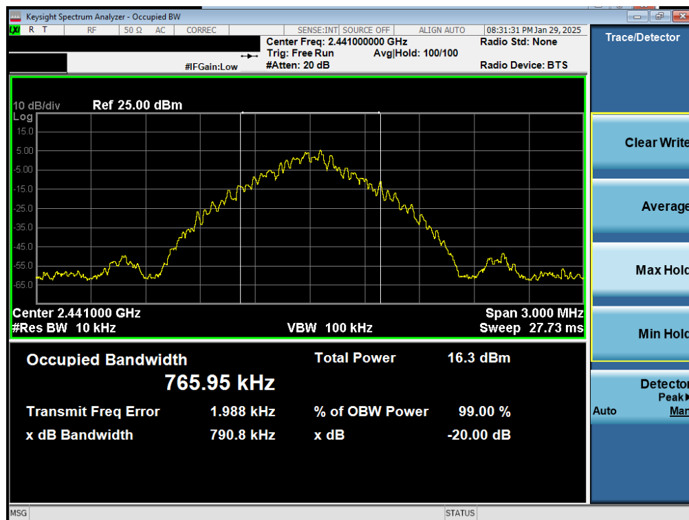
Plot 7-2. 20Db BW and 99% OBW Plot Antenna 0 (Common) (Bluetooth, GFSK, iPA – Ch. 39)
