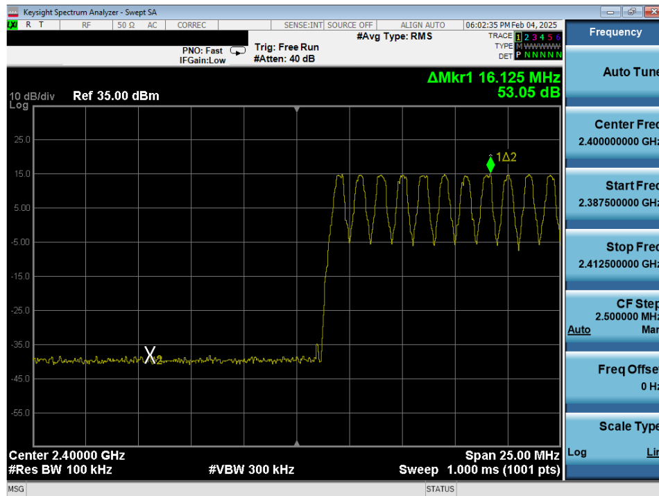
Plot 7-23. Band Edge Plot Antenna 0 (Dedicated) (Bluetooth with Hopping Enabled, GFSK, iPA – Ch.0)
