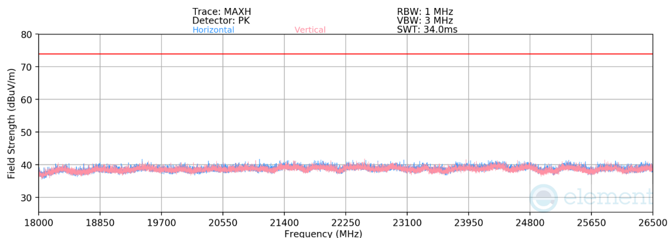
Plot 7-63. Radiated Spurious Emissions above 1GHz Antenna 0 (Dedicated) (BT GFSK iPA – Ch. 39)
