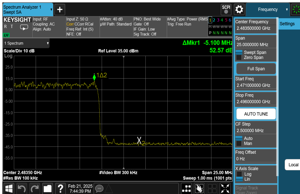
Plot 7-28. Band Edge Plot Antenna 0 (Dedicated) (Bluetooth with Hopping Enabled, 8DPSK, iPA – Ch.78)
