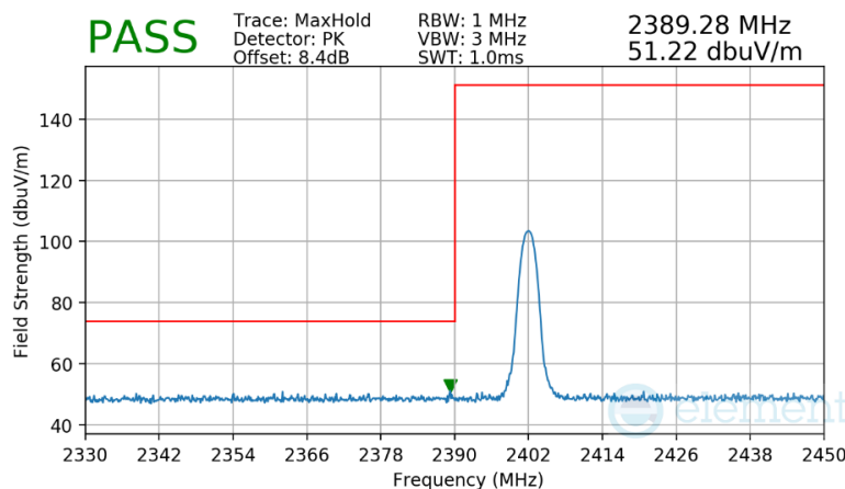
Plot 7-66. Radiated Restricted Lower Band Edge Measurement Antenna 0(Common)
