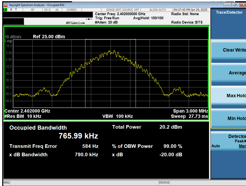
Plot 7-7. 20dB BW and 99% OBW Plot Antenna 0 (Dedicated) (Bluetooth, GFSK, iPA – Ch. 0)
