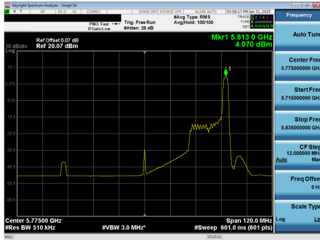
Plot 7-39. PSD Antenna 0 (80MHz BW 11ax Index 36 – RU26 – Ch.155)
