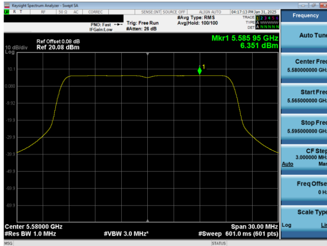
Plot 7-33. PSD Antenna 0 (20MHz BW 11ax- RU242 - Ch.116
