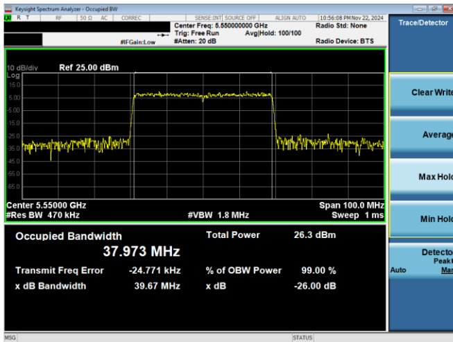
Plot 7-6. 26dB BW & 99% OBW Antenna 0 (40MHz BW 11ax- RU484 - Ch.110)
