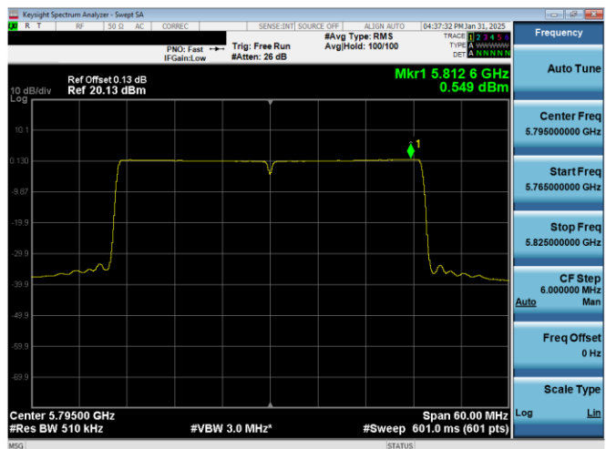
Plot 7-41. PSD Antenna 0 (40MHz BW 11ax – RU484 – Ch.159)
