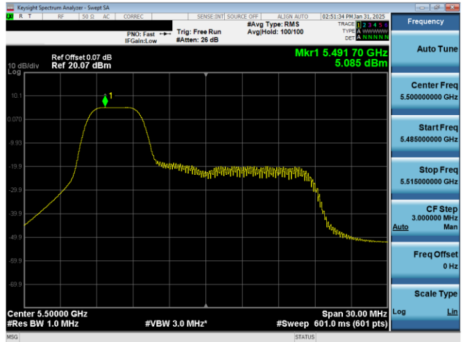
Plot 7-32. PSD Antenna 0 (160MHz BW 11ax Index 37 - RU52 - Ch.100)
