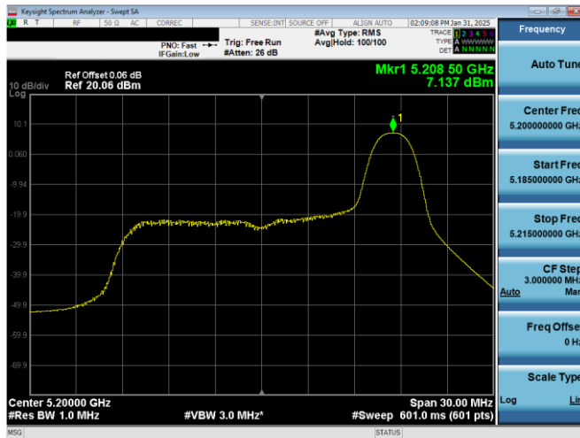
Plot 7-29. PSD Antenna 0 (20MHz BW 11ax Index 8 - RU26 - Ch.40)
