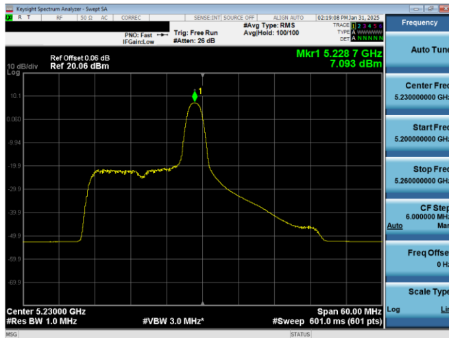
Plot 7-30. PSD Antenna 0 (40MHz BW 11ax Index 8 - RU26 - Ch.46)
