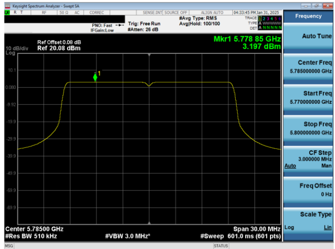
Plot 7-40. PSD Antenna 0 (20MHz BW 11ax – RU242 – Ch.157)
