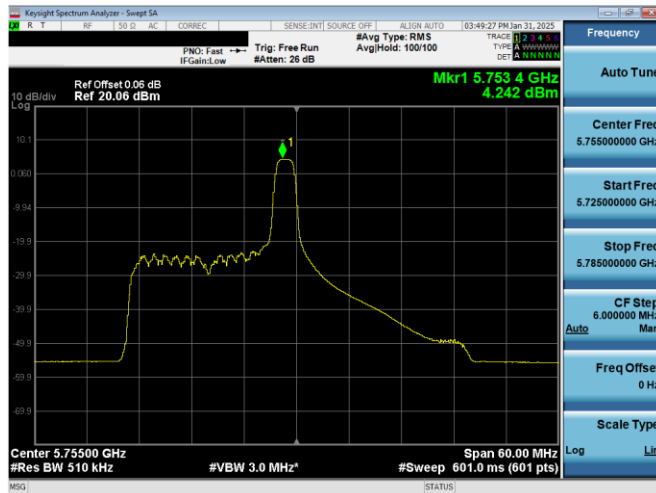
Plot 7-38. PSD Antenna 0 (40MHz BW 11ax Index 8 – RU26 – Ch.151)
