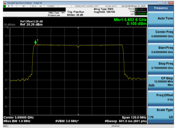
Plot 7-35. PSD Antenna 0 (80MHz BW 11ax- RU996 - Ch.138
