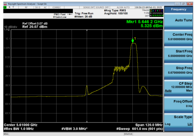
Plot 7-51. (FCC Only) PSD Antenna 1 (80MHz BW 11ax Index52 – RU52 – Ch.122)
