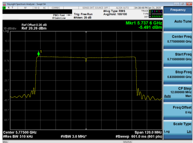
Plot 7-42. PSD Antenna 0 (80MHz BW 11ax – RU996 – Ch.155)
