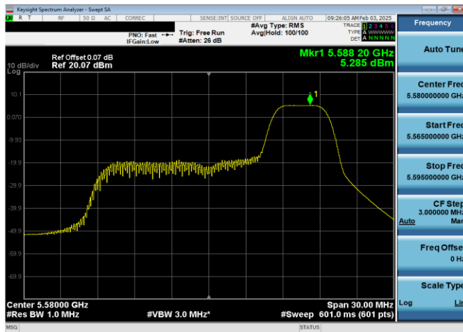
Plot 7-49. (FCC Only) PSD Antenna 1 (20MHz BW 11ax Index40 – RU52 – Ch.116)
