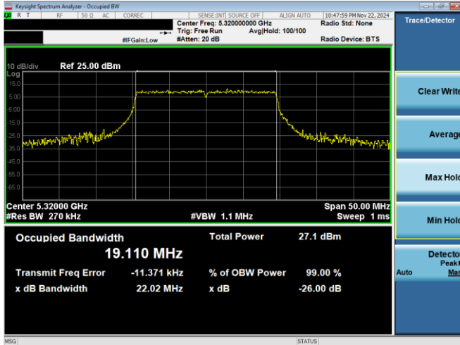
Plot 7-5. 26dB BW & 99% OBW Antenna 0 (20MHz BW 11ax- RU242 - Ch.64)
