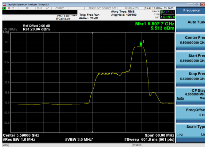
Plot 7-50. (FCC Only) PSD Antenna 1 (40MHz BW 11ax Index44 – RU52 – Ch.118)
