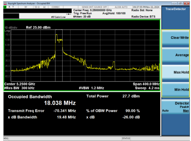
Plot 7-4. 26dB BW & 99% OBW Antenna 0 (160MHz BW 11ax Index 37 – RU52 – Ch.50)
