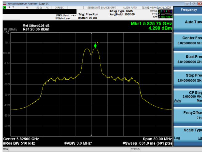
Plot 7-37. PSD Antenna 0 (20MHz BW 11ax Index 4 – RU26 – Ch.165)
