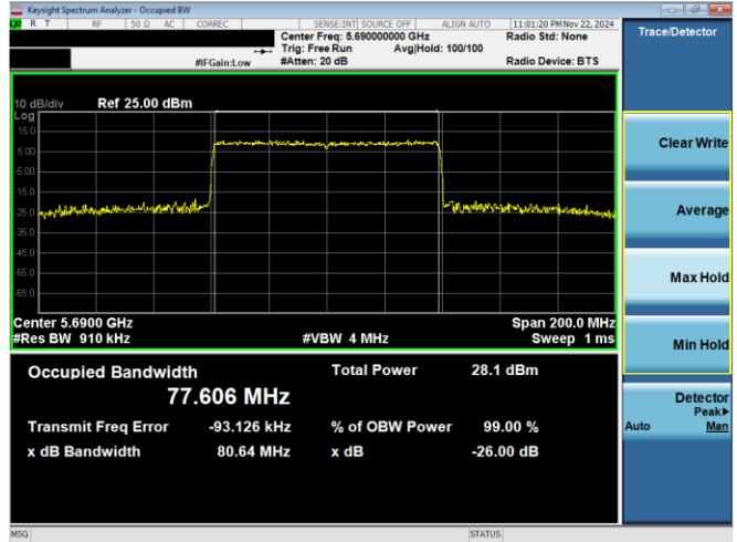
Plot 7-7. 26dB BW & 99% OBW Antenna 0 (80MHz BW 11ax- RU996 - Ch.138)
