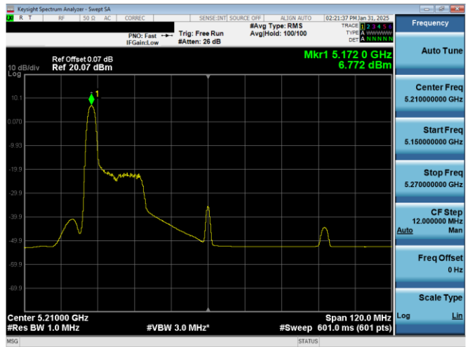
Plot 7-31. PSD Antenna 0 (80MHz BW 11ax Index 0 - RU26 - Ch.42)
