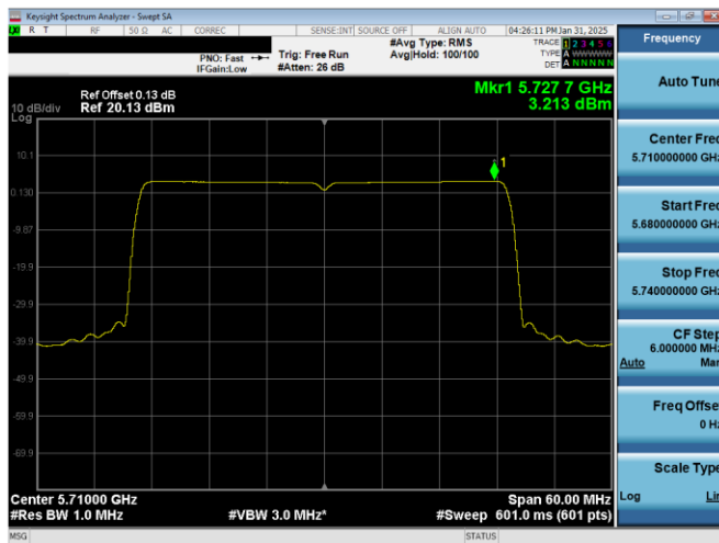
Plot 7-34. PSD Antenna 0 (40MHz BW 11ax- RU484 - Ch.142
