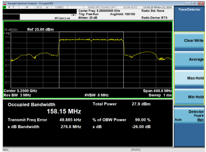
Plot 7-8. 26dB BW & 99% OBW Antenna 0 (160MHz BW 11ax- RU996x2 - Ch.50)
