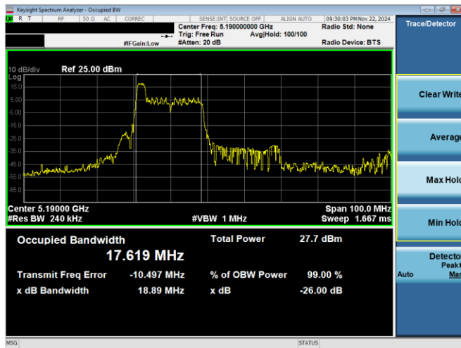
Plot 7-2. 26dB BW & 99% OBW Antenna 0 (40MHz BW 11ax Index 0 – RU26 – Ch.38)
