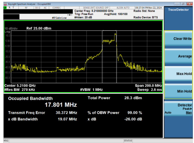
Plot 7-3. 26dB BW & 99% OBW Antenna 0 (80MHz BW 11ax Index 36 – RU26 – Ch.42)
