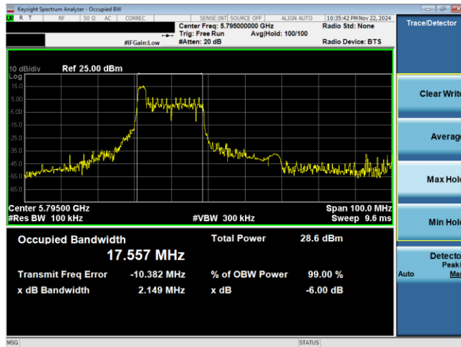
Plot 7-18. 6dB BW OBW Antenna 0 (40MHz BW 11ax Index 0 – RU26 – Ch.159)
