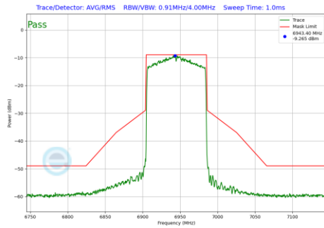
Plot 7-143 In-Band Emission Plot CDD Antenna 0 (80MHz BW 802.11ax(SU) (UNII Band 8) - Ch.199)
