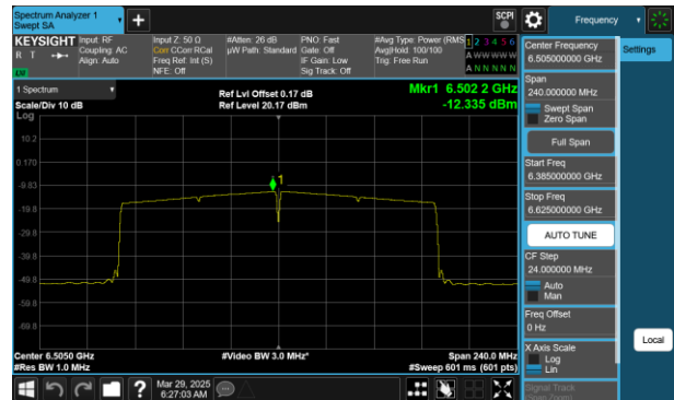
Plot 7-80 PSD CDD Antenna 1 (160MHz BW 802.11ax(SU) - Ch.111)
