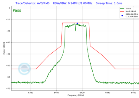
Plot 7-97 In-Band Emission Plot Antenna 0 (20MHz BW 802.11a (UNII Band 5) - Ch.93)
