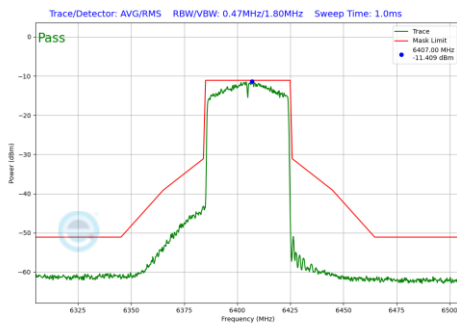
Plot 7-114 In-Band Emission Plot Antenna 1 (40MHz BW 802.11ax(SU) (UNII Band 5) - Ch.91)
