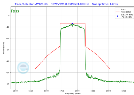
Plot 7-155 In-Band Emission Plot CDD Antenna 1 (80MHz BW 802.11ax(SU) (UNII Band 7) - Ch.167)
