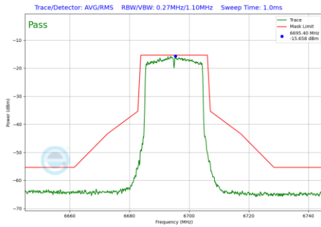
Plot 7-153 In-Band Emission Plot CDD Antenna 1 (20MHz BW 802.11ax(SU) (UNII Band 7) - Ch.149)
