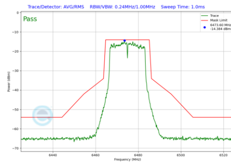
Plot 7-101 In-Band Emission Plot Antenna 0 (20MHz BW 802.11a (UNII Band 6) - Ch.105)
