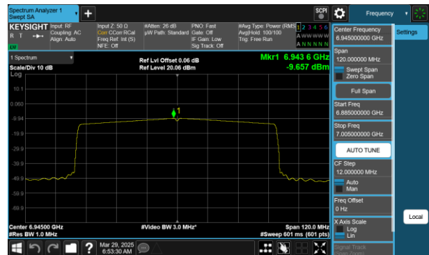
Plot 7-95 PSD CDD Antenna 1 (80MHz BW 802.11ax(SU) - Ch.199)
