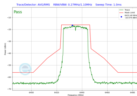
Plot 7-133 In-Band Emission Plot CDD Antenna 0 (20MHz BW 802.11ax(SU) (UNII Band 6) - Ch.97)
