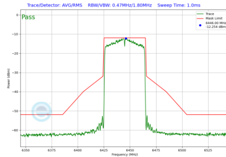
Plot 7-102 In-Band Emission Plot Antenna 0 (40MHz BW 802.11ax(SU) (UNII Band 6) - Ch.99)
