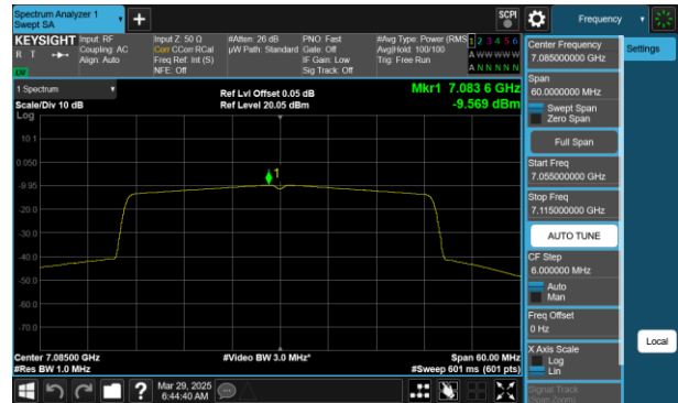
Plot 7-94 PSD CDD Antenna 1 (40MHz BW 802.11ax(SU) - Ch.227)
