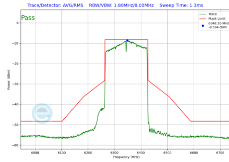
Plot 7-132 In-Band Emission Plot CDD Antenna 0 (160MHz BW 802.11ax(SU) (UNII Band 5) - Ch.79)
