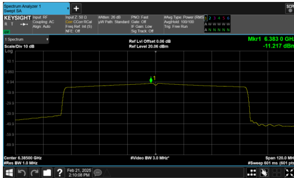
Plot 7-67 PSD CDD Antenna 0 (80MHz BW 802.11ax(SU) - Ch.87)
