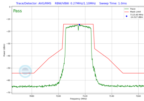
Plot 7-141 In-Band Emission Plot CDD Antenna 0 (20MHz BW 802.11ax(SU) (UNII Band 8) - Ch.233)
