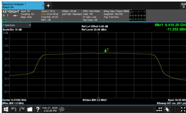
Plot 7-65 PSD CDD Antenna 0 (20MHz BW 802.11ax(SU) - Ch.93)
