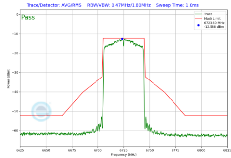
Plot 7-138 In-Band Emission Plot CDD Antenna 0 (40MHz BW 802.11ax(SU) (UNII Band 7) - Ch.155)
