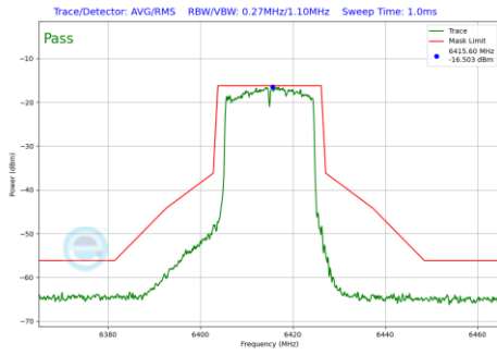
Plot 7-129 In-Band Emission Plot CDD Antenna 0 (20MHz BW 802.11ax(SU) (UNII Band 5) - Ch.93)
