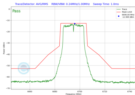
Plot 7-121 In-Band Emission Plot Antenna 1 (20MHz BW 802.11a (UNII Band 7) - Ch.149)
