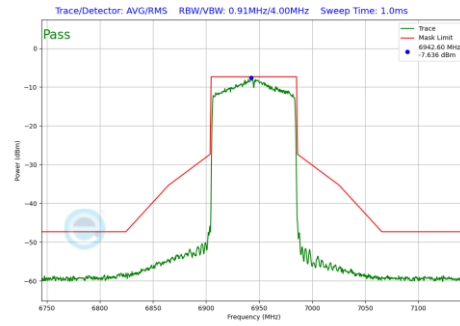
Plot 7-111 In-Band Emission Plot Antenna 0 (80MHz BW 802.11ax(SU) (UNII Band 8) - Ch.199)
