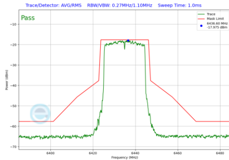
Plot 7-149 In-Band Emission Plot CDD Antenna 1 (20MHz BW 802.11ax(SU) (UNII Band 6) - Ch.97)
