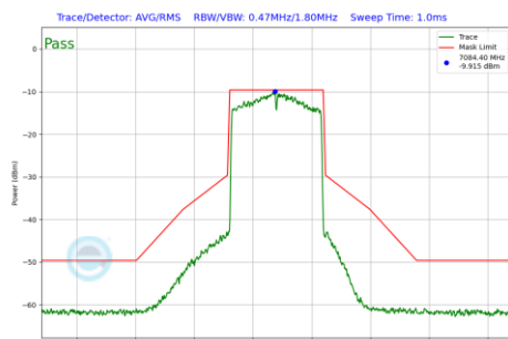
Plot 7-110 In-Band Emission Plot Antenna 0 (40MHz BW 802.11ax(SU) (UNII Band 8) - Ch.227)
