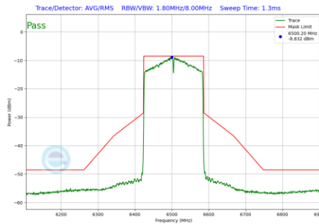
Plot 7-136 In-Band Emission Plot CDD Antenna 0 (160MHz BW 802.11ax(SU) (UNII Band 6) - Ch.111)
