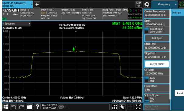
Plot 7-75 PSD CDD Antenna 0 (80MHz BW 802.11ax(SU) - Ch.103)
