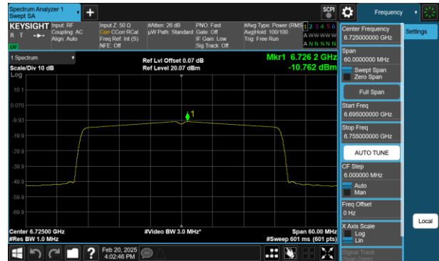
Plot 7-86 PSD CDD Antenna 1 (40MHz BW 802.11ax(SU) - Ch.155)
