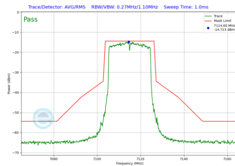
Plot 7-157 In-Band Emission Plot CDD Antenna 1 (20MHz BW 802.11ax(SU) (UNII Band 8) - Ch.233)
