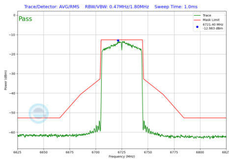
Plot 7-154 In-Band Emission Plot CDD Antenna 1 (40MHz BW 802.11ax(SU) (UNII Band 7) - Ch.155)
