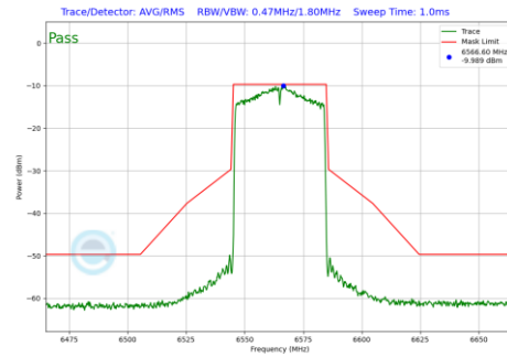
Plot 7-106 In-Band Emission Plot Antenna 0 (40MHz BW 802.11ax(SU) (UNII Band 7) - Ch.123)
