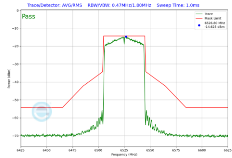
Plot 7-150 In-Band Emission Plot CDD Antenna 1 (40MHz BW 802.11ax(SU) (UNII Band 6) - Ch.115)
