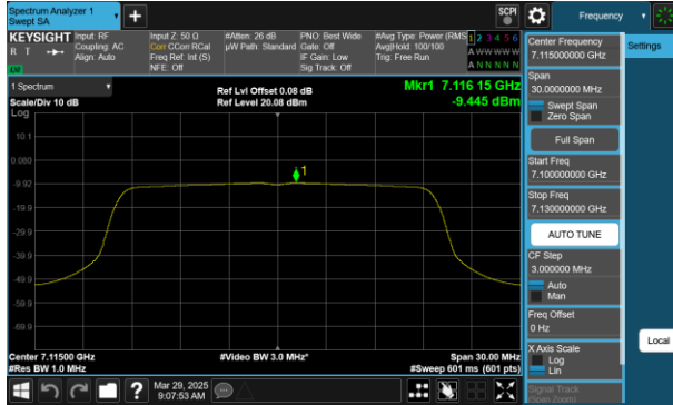
Plot 7-89 PSD CDD Antenna 0 (20MHz BW 802.11ax(SU) - Ch.233)
