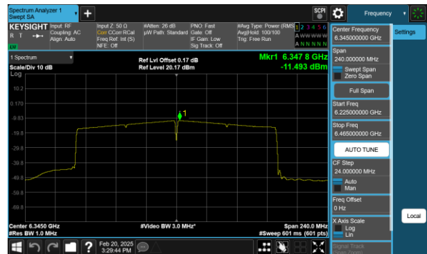
Plot 7-72 PSD CDD Antenna 1 (160MHz BW 802.11ax(SU) - Ch.79)
