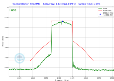
Plot 7-130 In-Band Emission Plot CDD Antenna 0 (40MHz BW 802.11ax(SU) (UNII Band 5) - Ch.91)
