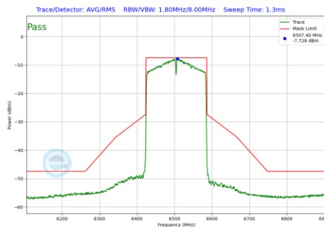
Plot 7-120 In-Band Emission Plot Antenna 1 (160MHz BW 802.11ax(SU) (UNII Band 6) - Ch.111)
