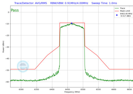
Plot 7-103 In-Band Emission Plot Antenna 0 (80MHz BW 802.11ax(SU) (UNII Band 6) - Ch.103)
