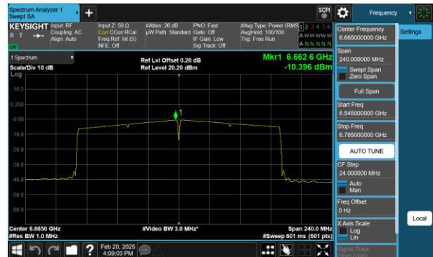
Plot 7-88 PSD CDD Antenna 1 (160MHz BW 802.11ax(SU) - Ch.143)
