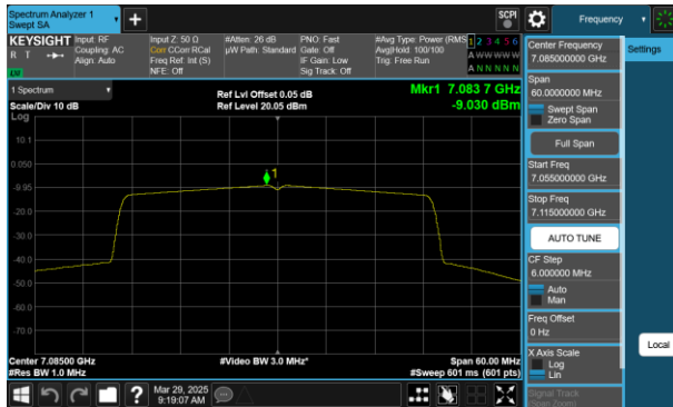
Plot 7-90 PSD CDD Antenna 0 (40MHz BW 802.11ax(SU) - Ch.227)
