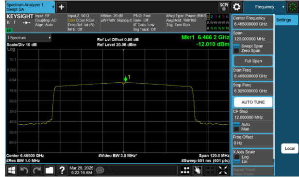
Plot 7-79 PSD CDD Antenna 1 (80MHz BW 802.11ax(SU) - Ch.103)
