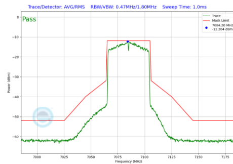
Plot 7-158 In-Band Emission Plot CDD Antenna 1 (40MHz BW 802.11ax(SU) (UNII Band 8) - Ch.227)
