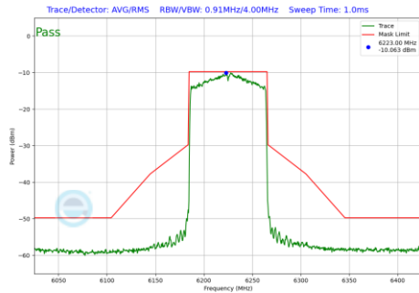
Plot 7-99 In-Band Emission Plot Antenna 0 (80MHz BW 802.11ax(SU) (UNII Band 5) - Ch.55)
