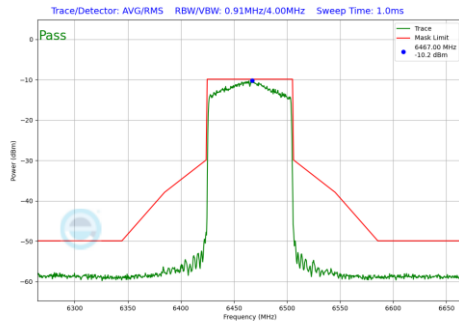
Plot 7-119 In-Band Emission Plot Antenna 1 (80MHz BW 802.11ax(SU) (UNII Band 6) - Ch.103)
