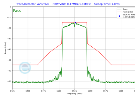
Plot 7-134 In-Band Emission Plot CDD Antenna 0 (40MHz BW 802.11ax(SU) (UNII Band 6) - Ch.115)
