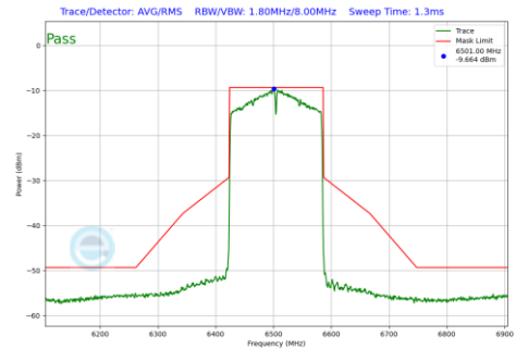
Plot 7-152 In-Band Emission Plot CDD Antenna 1 (160MHz BW 802.11ax(SU) (UNII Band 6) - Ch.111)
