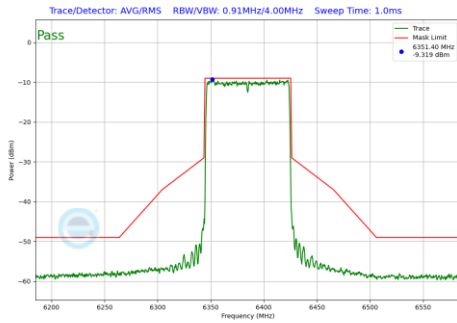
Plot 7-115 In-Band Emission Plot Antenna 1 (80MHz BW 802.11ax(SU) (UNII Band 5) - Ch.87)
