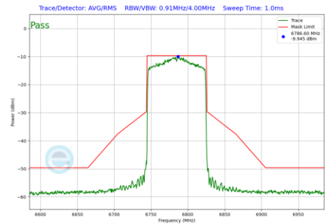
Plot 7-139 In-Band Emission Plot CDD Antenna 0 (80MHz BW 802.11ax(SU) (UNII Band 7) - Ch.167)
