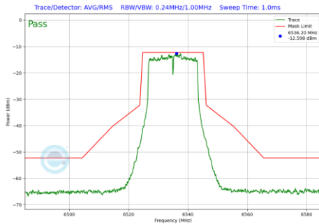
Plot 7-105 In-Band Emission Plot Antenna 0 (20MHz BW 802.11a (UNII Band 7) - Ch.117)
