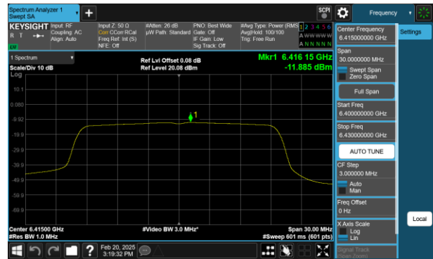
Plot 7-69 PSD CDD Antenna 1 (20MHz BW 802.11ax(SU) - Ch.93)
