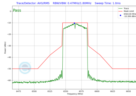
Plot 7-122 In-Band Emission Plot Antenna 1 (40MHz BW 802.11ax(SU) (UNII Band 7) - Ch.123)
