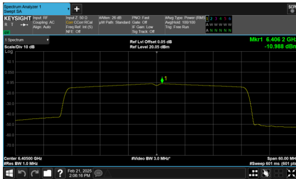
Plot 7-66 PSD CDD Antenna 0 (40MHz BW 802.11ax(SU) - Ch.91)
