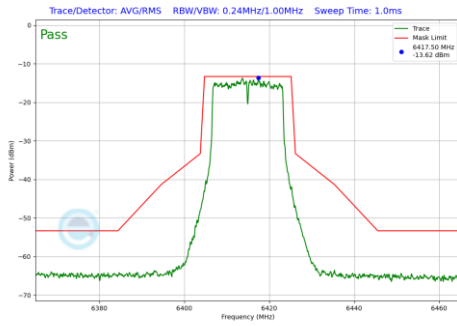
Plot 7-113 In-Band Emission Plot Antenna 1 (20MHz BW 802.11a (UNII Band 5) - Ch.93)
