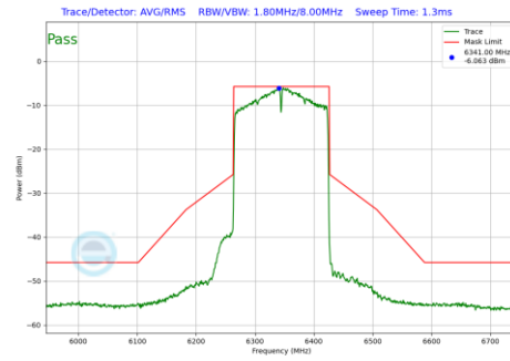
Plot 7-116 In-Band Emission Plot Antenna 1 (160MHz BW 802.11ax(SU) (UNII Band 5) - Ch.79)
