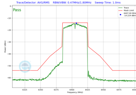
Plot 7-146 In-Band Emission Plot CDD Antenna 0 (40MHz BW 802.11ax(SU) (UNII Band 5) - Ch.91)
