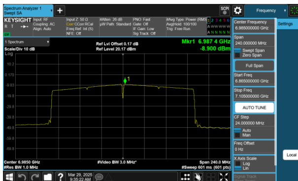
Plot 7-92 PSD CDD Antenna 0 (160MHz BW 802.11ax(SU) - Ch.207)
