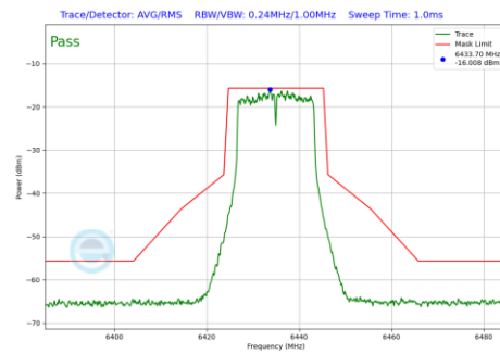
Plot 7-117 In-Band Emission Plot Antenna 1 (20MHz BW 802.11a (UNII Band 6) - Ch.97)
