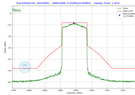
Plot 7-127 In-Band Emission Plot Antenna 1 (80MHz BW 802.11ax(SU) (UNII Band 8) - Ch.199)
