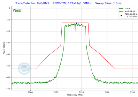
Plot 7-125 In-Band Emission Plot Antenna 1 (20MHz BW 802.11a (UNII Band 8) - Ch.233)
