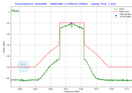
Plot 7-126 In-Band Emission Plot Antenna 1 (40MHz BW 802.11ax(SU) (UNII Band 8) - Ch.227)
