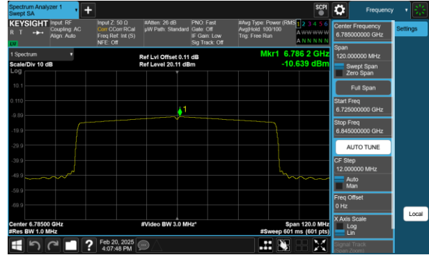
Plot 7-87 PSD CDD Antenna 1 (80MHz BW 802.11ax(SU) - Ch.167)
