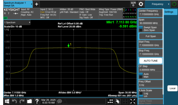
Plot 7-93 PSD CDD Antenna 1 (20MHz BW 802.11ax(SU) - Ch.233)
