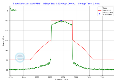
Plot 7-159 In-Band Emission Plot CDD Antenna 1 (80MHz BW 802.11ax(SU) (UNII Band 8) - Ch.199)
