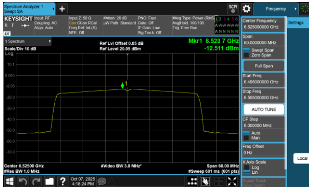
Plot 7-74 PSD CDD Antenna 0 (40MHz BW 802.11ax(SU) - Ch.115)
