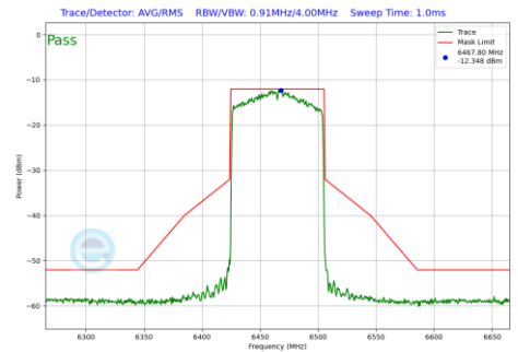
Plot 7-151 In-Band Emission Plot CDD Antenna 1 (80MHz BW 802.11ax(SU) (UNII Band 6) - Ch.103)
