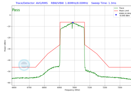
Plot 7-144 In-Band Emission Plot CDD Antenna 0 (160MHz BW 802.11ax(SU) (UNII Band 8) - Ch.207)
