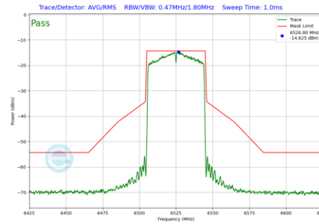
Plot 7-118 In-Band Emission Plot Antenna 1 (40MHz BW 802.11ax(SU) (UNII Band 6) - Ch.115)
