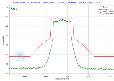
Plot 7-109 In-Band Emission Plot Antenna 0 (20MHz BW 802.11a (UNII Band 8) - Ch.209)
