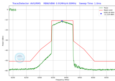
Plot 7-131 In-Band Emission Plot CDD Antenna 0 (80MHz BW 802.11ax(SU) (UNII Band 5) - Ch.87)
