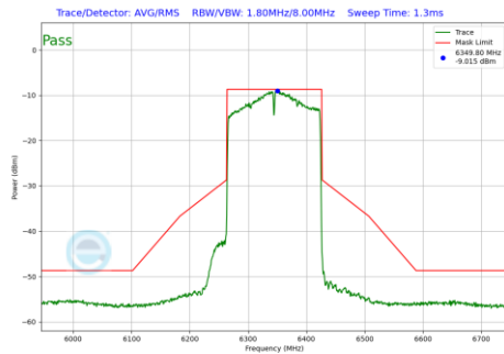
Plot 7-148 In-Band Emission Plot CDD Antenna 1 (160MHz BW 802.11ax(SU) (UNII Band 5) - Ch.79)
