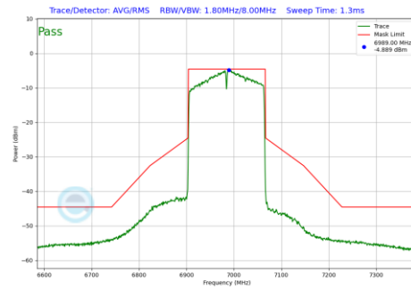
Plot 7-112 In-Band Emission Plot Antenna 0 (160MHz BW 802.11ax(SU) (UNII Band 8) - Ch.207)
