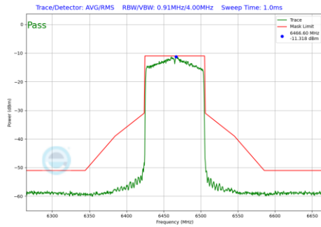
Plot 7-135 In-Band Emission Plot CDD Antenna 0 (80MHz BW 802.11ax(SU) (UNII Band 6) - Ch.103)
