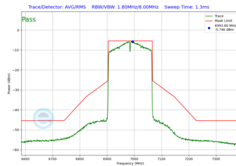
Plot 7-128 In-Band Emission Plot Antenna 1 (160MHz BW 802.11ax(SU) (UNII Band 8) - Ch.207)
