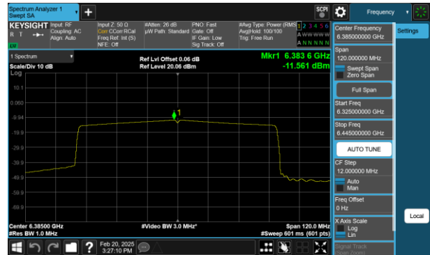
Plot 7-71 PSD CDD Antenna 1 (80MHz BW 802.11ax(SU) - Ch.87)
