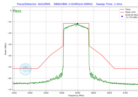
Plot 7-107 In-Band Emission Plot Antenna 0 (80MHz BW 802.11ax(SU) (UNII Band 7) - Ch.119)
