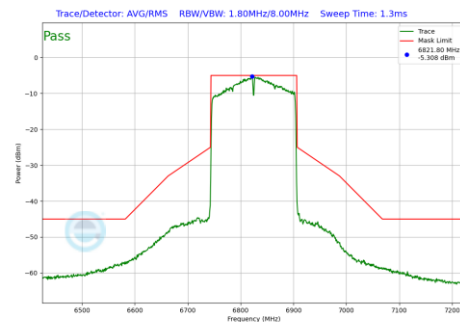
Plot 7-124 In-Band Emission Plot Antenna 1 (160MHz BW 802.11ax(SU) (UNII Band 7) - Ch.175)
