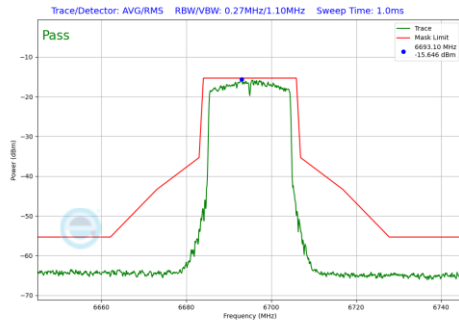
Plot 7-137 In-Band Emission Plot CDD Antenna 0 (20MHz BW 802.11ax(SU) (UNII Band 7) - Ch.149)
