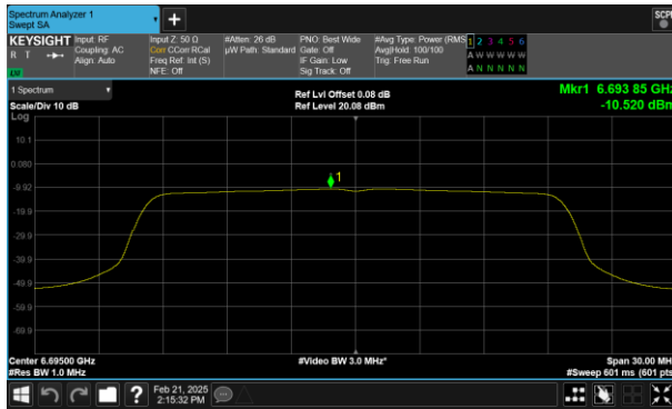
Plot 7-81 PSD CDD Antenna 0 (20MHz BW 802.11ax(SU) - Ch.149)
