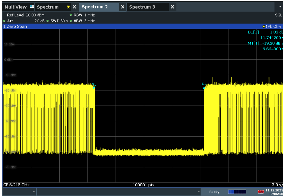
Plot 7-178. Contention Based Protocol Timing Plot – UNII 5 – 20MHz Channel 53
