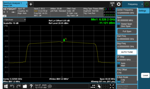
Plot 7-78 PSD CDD Antenna 1 (40MHz BW 802.11ax(SU) - Ch.115)
