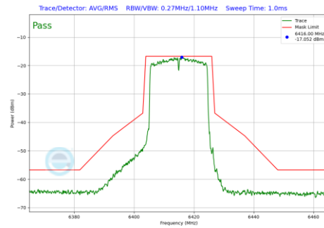
Plot 7-145 In-Band Emission Plot CDD Antenna 0 (20MHz BW 802.11ax(SU) (UNII Band 5) - Ch.93)
