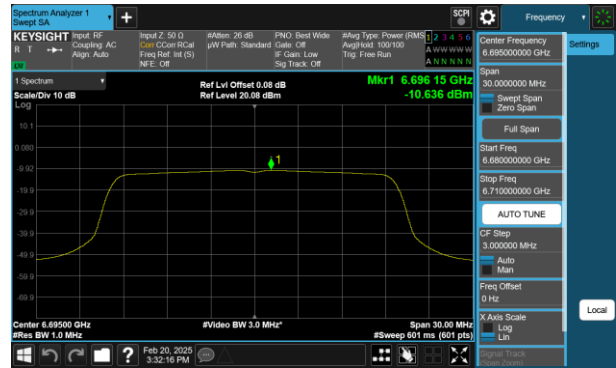
Plot 7-85 PSD CDD Antenna 1 (20MHz BW 802.11ax(SU) - Ch.149)
