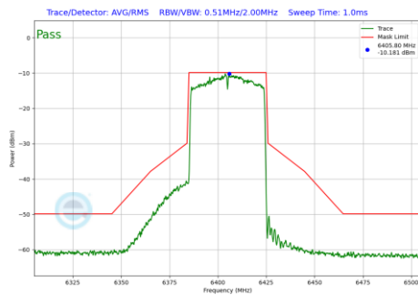
Plot 7-98 In-Band Emission Plot Antenna 0 (40MHz BW 802.11ax(SU) (UNII Band 5) - Ch.91)
