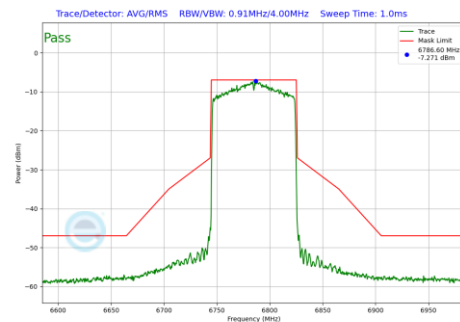
Plot 7-123 In-Band Emission Plot Antenna 1 (80MHz BW 802.11ax(SU) (UNII Band 7) - Ch.167)
