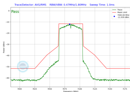
Plot 7-142 In-Band Emission Plot CDD Antenna 0 (40MHz BW 802.11ax(SU) (UNII Band 8) - Ch.227)
