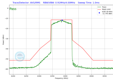
Plot 7-147 In-Band Emission Plot CDD Antenna 1 (80MHz BW 802.11ax(SU) (UNII Band 5) - Ch.87)
