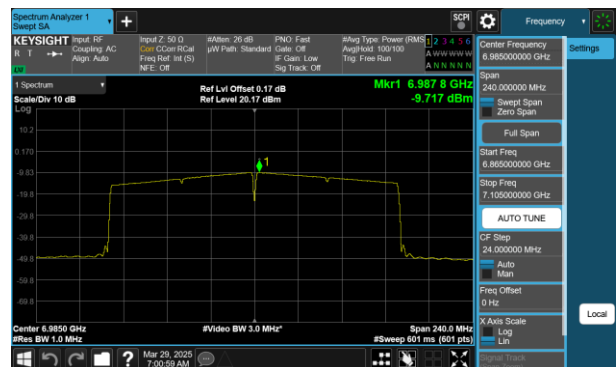
Plot 7-96 PSD CDD Antenna 1 (160MHz BW 802.11ax(SU) - Ch.207)
