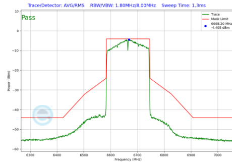
Plot 7-108 In-Band Emission Plot Antenna 0 (160MHz BW 802.11ax(SU) (UNII Band 7) - Ch.143)
