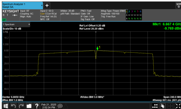
Plot 7-84 PSD CDD Antenna 0 (160MHz BW 802.11ax(SU) - Ch.143)
