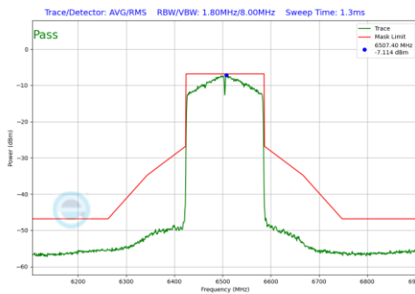
Plot 7-104 In-Band Emission Plot Antenna 0 (160MHz BW 802.11ax(SU) (UNII Band 6) - Ch.111)
