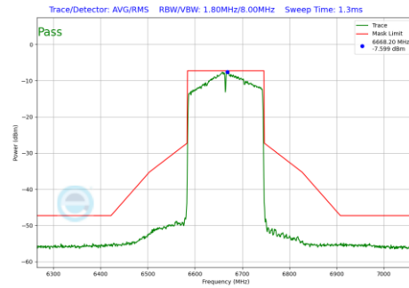
Plot 7-156 In-Band Emission Plot CDD Antenna 1 (160MHz BW 802.11ax(SU) (UNII Band 7) - Ch.143)
