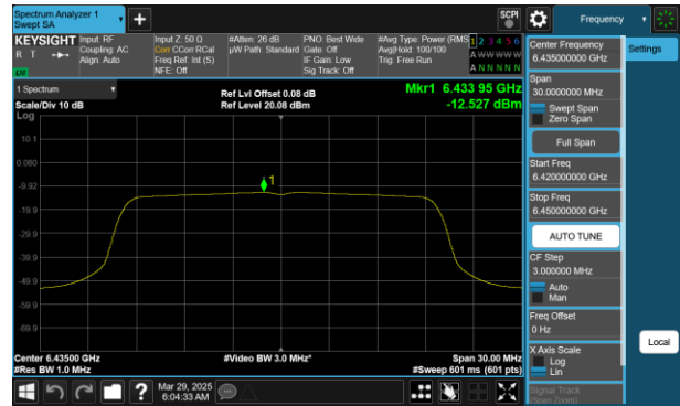
Plot 7-77 PSD CDD Antenna 1 (20MHz BW 802.11ax(SU) - Ch.97)
