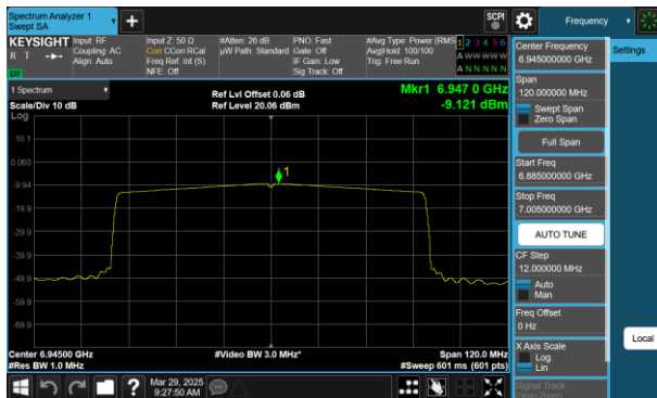
Plot 7-91 PSD CDD Antenna 0 (80MHz BW 802.11ax(SU) - Ch.199)
