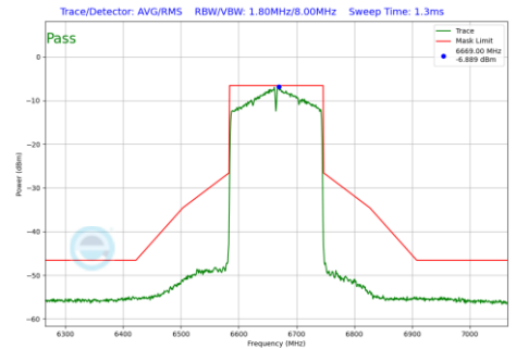
Plot 7-140 In-Band Emission Plot CDD Antenna 0 (160MHz BW 802.11ax(SU) (UNII Band 7) - Ch.143)
