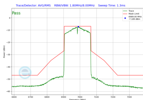
Plot 7-160 In-Band Emission Plot CDD Antenna 1 (160MHz BW 802.11ax(SU) (UNII Band 8) - Ch.207)
