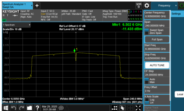
Plot 7-76 PSD CDD Antenna 0 (160MHz BW 802.11ax(SU) - Ch.111)
