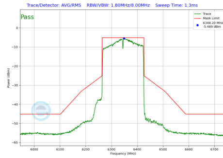
Plot 7-100 In-Band Emission Plot Antenna 0 (160MHz BW 802.11ax(SU) (UNII Band 5) - Ch.79)
