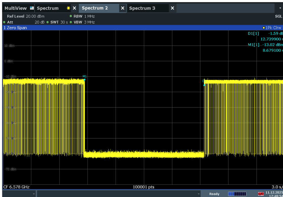
Plot 7-185. Contention Based Protocol Timing Plot – UNII 6 – 160MHz Channel 111 – High
