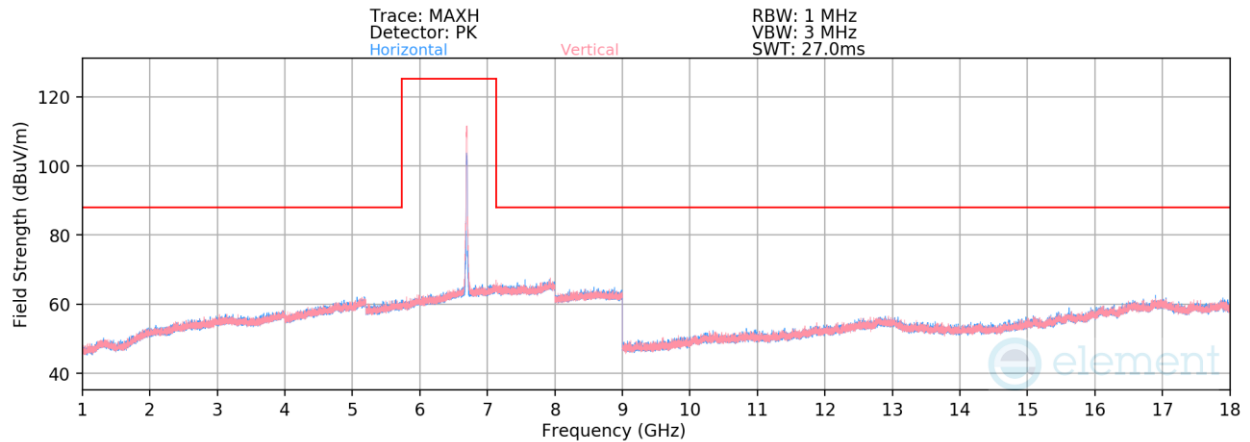
Plot 7-205. Radiated Spurious Emissions 1-18GHz SDM (802.11ax – Ch. 149)
