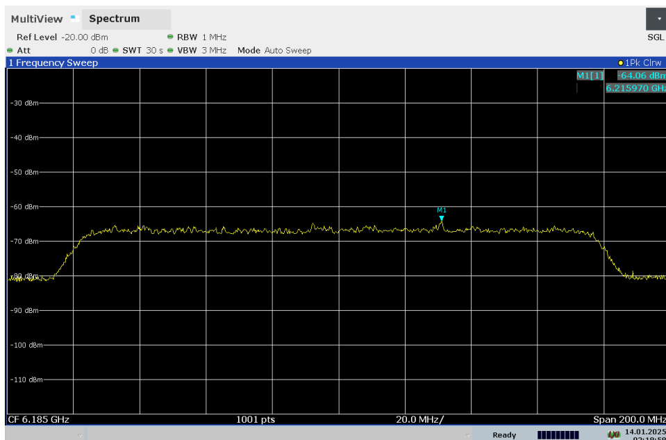
Plot 7-194. 160MHz Bandwidth, Before AWGN Signal Injected – Channel 47
