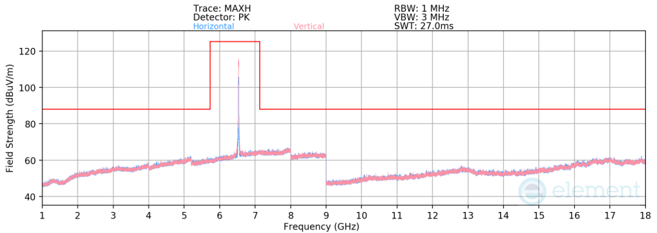
Plot 7-204. Radiated Spurious Emissions 1-18GHz SDM (802.11ax – Ch. 117)
