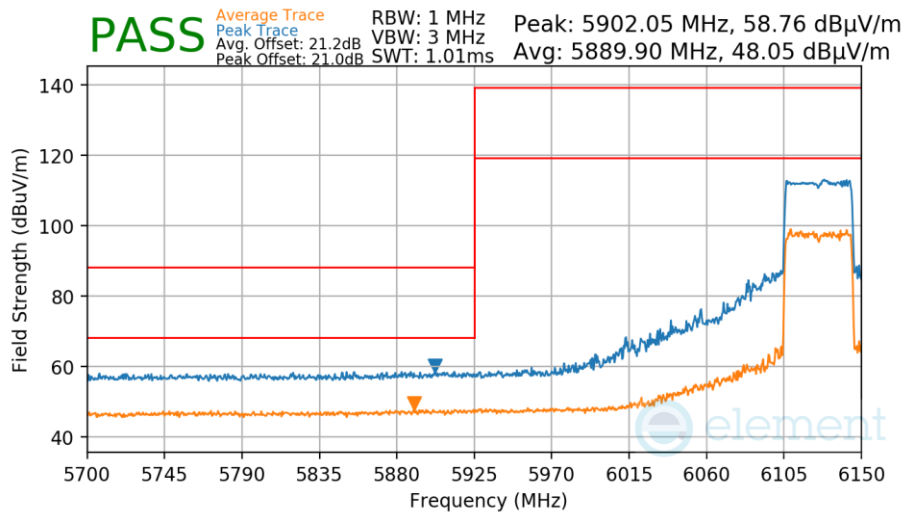
Plot 7-210. Antenna 0 Radiated Lower Band Edge (Peak & Average – UNII Band 5)
