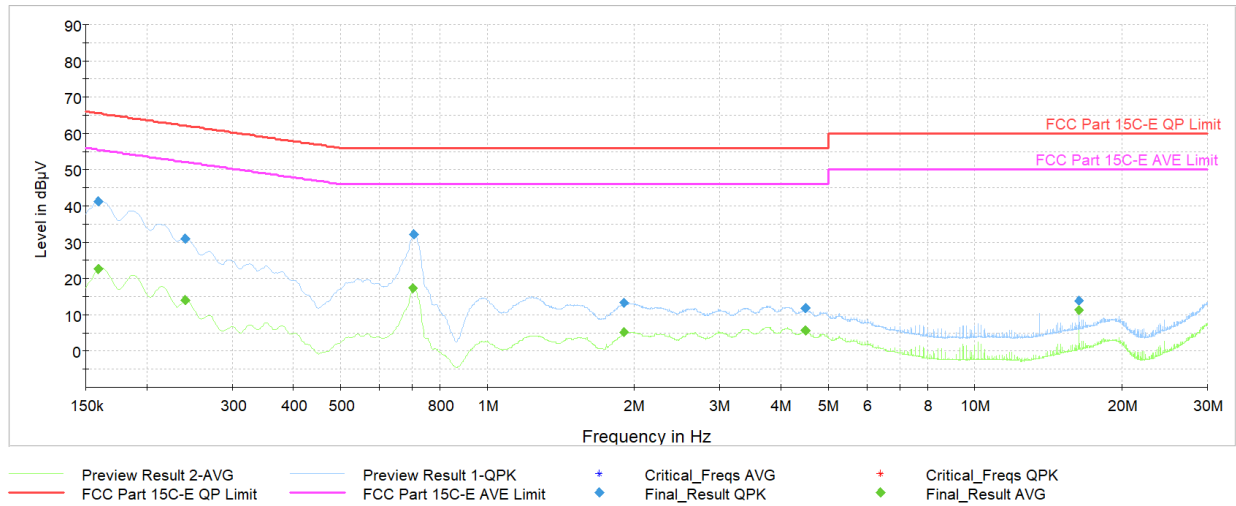
Plot 7-223. AC Line Conducted Plot with 802.11ax SDM – Ch.61 (L1), powered by AC/DC Adapter via USB-C cable
