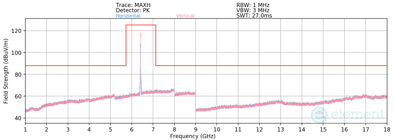
Plot 7-203. Radiated Spurious Emissions 1-18GHz SDM (802.11ax – Ch. 93)
