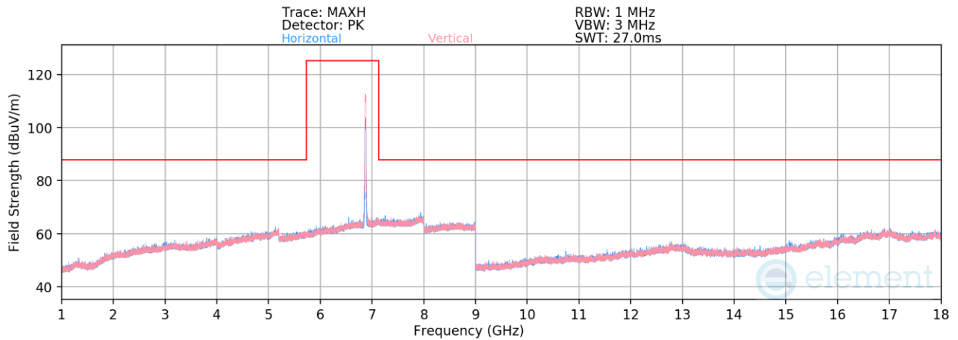
Plot 7-207. Radiated Spurious Emissions 1-18GHz SDM (802.11ax – Ch. 181)
