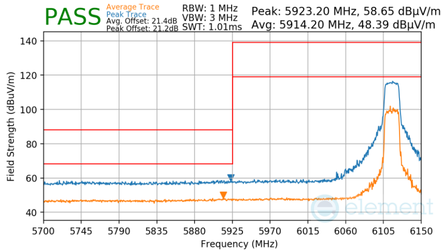
Plot 7-213. Antenna 1 Radiated Lower Band Edge (Peak & Average – UNII Band 5)
