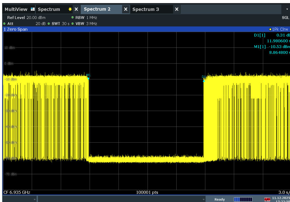
Plot 7-190. Contention Based Protocol Timing Plot – UNII 8 – 20MHz Channel 197
