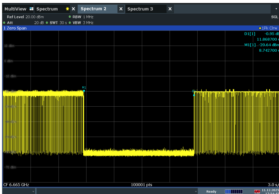
Plot 7-188. Contention Based Protocol Timing Plot – UNII 7 – 160MHz Channel 143 – Mid
