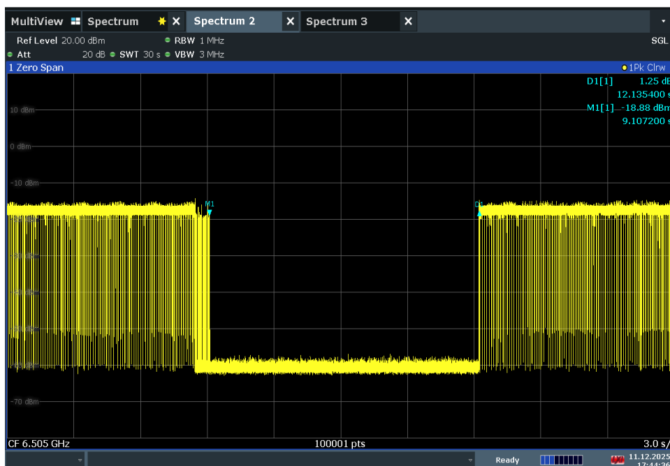
Plot 7-184. Contention Based Protocol Timing Plot – UNII 6 – 160MHz Channel 111 – Mid
