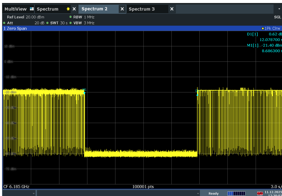
Plot 7-180. Contention Based Protocol Timing Plot –UNII 5 – 160MHz Channel 47 – Mid
