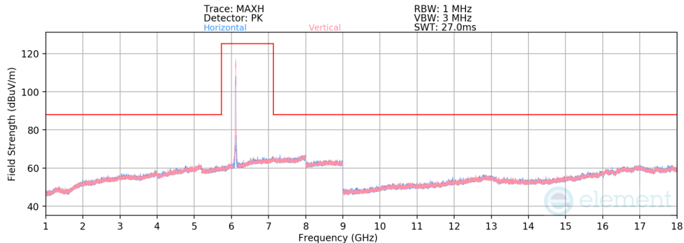
Plot 7-200. Radiated Spurious Emissions 1-18GHz SDM (802.11ax – Ch. 33)
