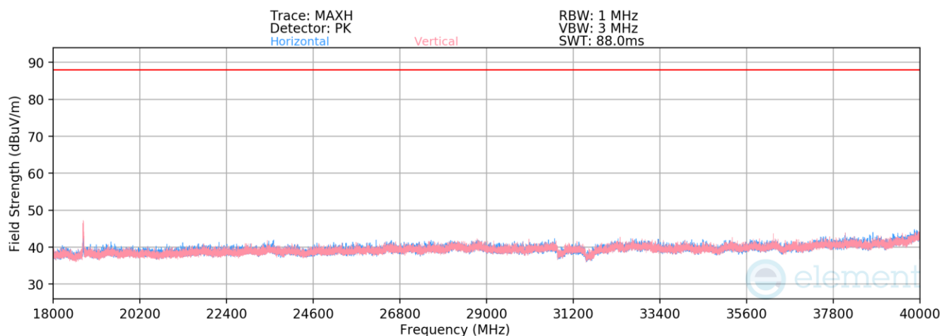
Plot 7-202. Radiated Spurious Emissions 18-40GHz SDM (802.11ax – Ch. 61)
