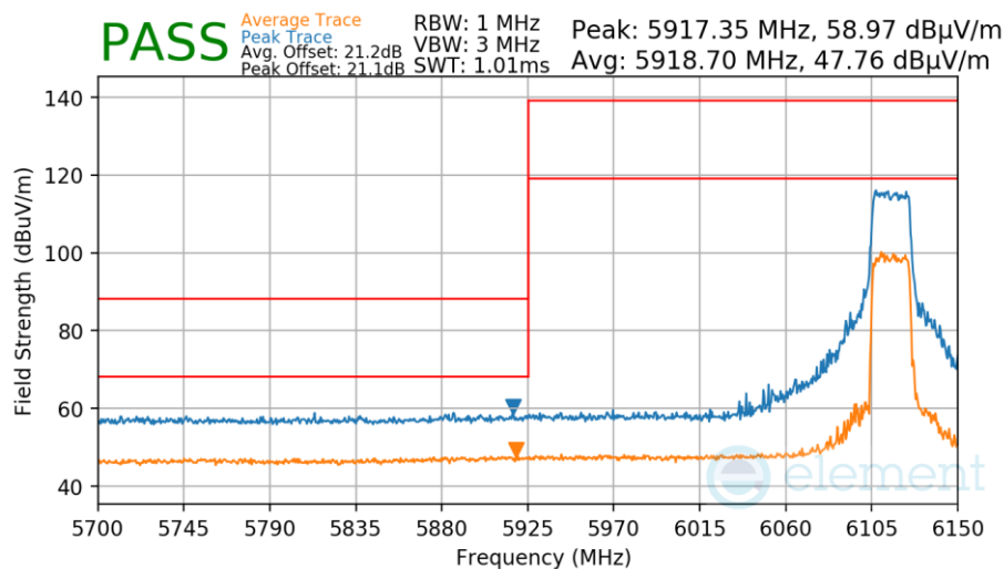
Plot 7-209. Antenna 0 Radiated Lower Band Edge (Peak & Average – UNII Band 5)
