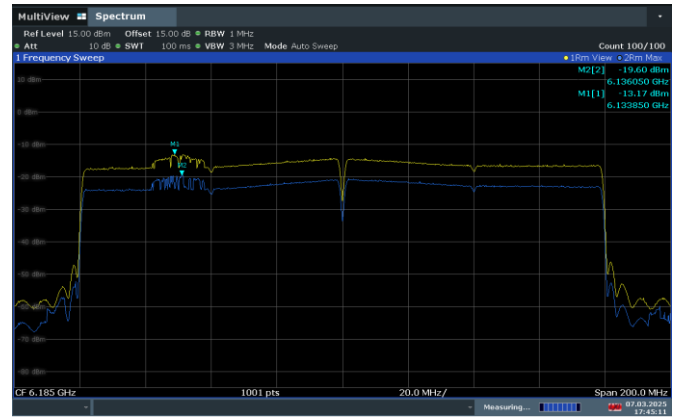
Plot 7-199. 160MHz Bandwidth – 6185MHz Antenna 1
