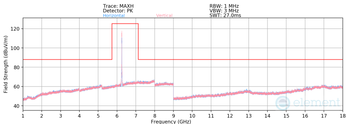
Plot 7-201. Radiated Spurious Emissions 1-18GHz SDM (802.11ax – Ch. 61)
