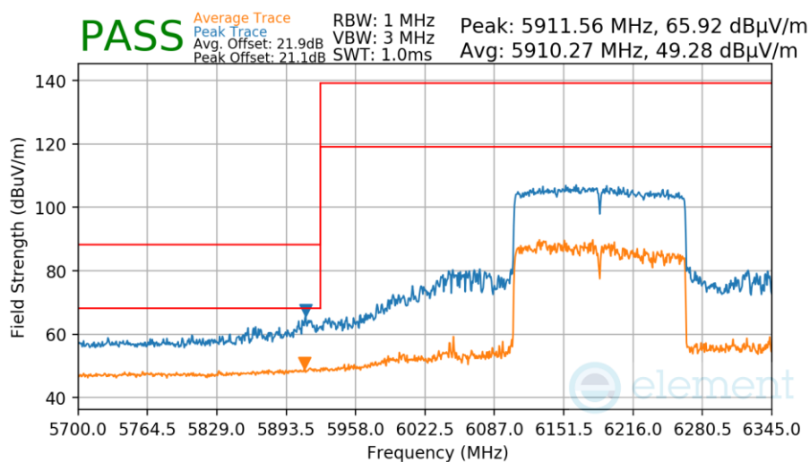
Plot 7-217. Antenna 1 Radiated Lower Band Edge (Peak & Average – UNII Band 5)
