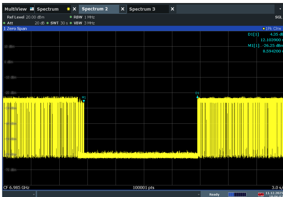
Plot 7-192. Contention Based Protocol Timing Plot – UNII 8 – 160MHz Channel 207 – Mid
