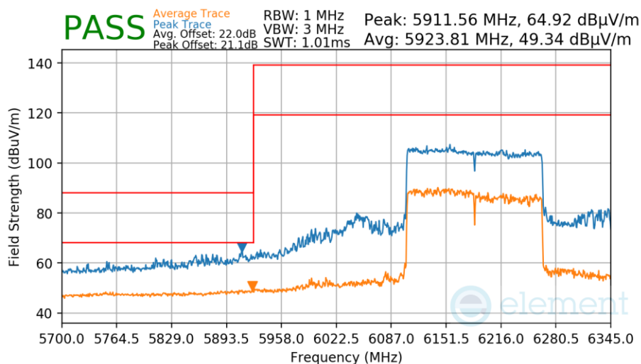
Plot 7-212. Antenna 0 Radiated Lower Band Edge (Peak & Average – UNII Band 5)
