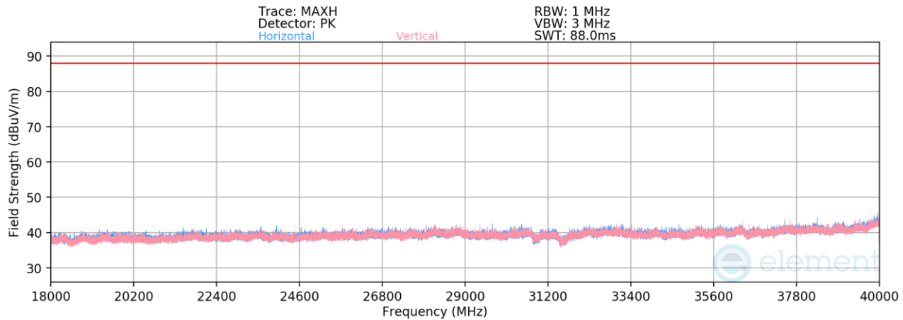
Plot 7-206. Radiated Spurious Emissions 18-40GHz SDM (802.11ax – Ch. 149)
