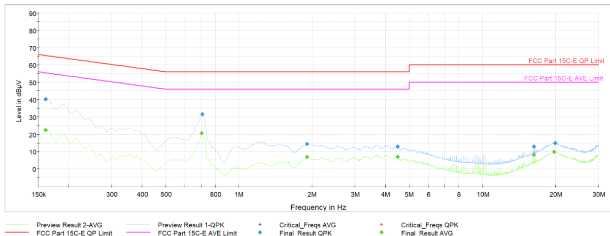
Plot 7-224. AC Line Conducted Plot with 802.11ax SDM – Ch. 61 (N), powered by AC/DC Adapter via USB-C cable
