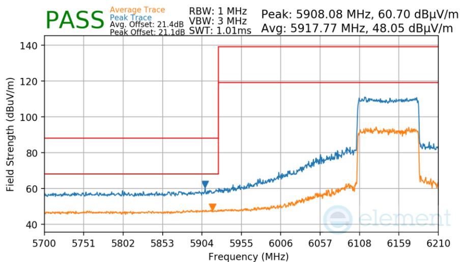
Plot 7-216. Antenna 1 Radiated Lower Band Edge (Peak & Average – UNII Band 5)
