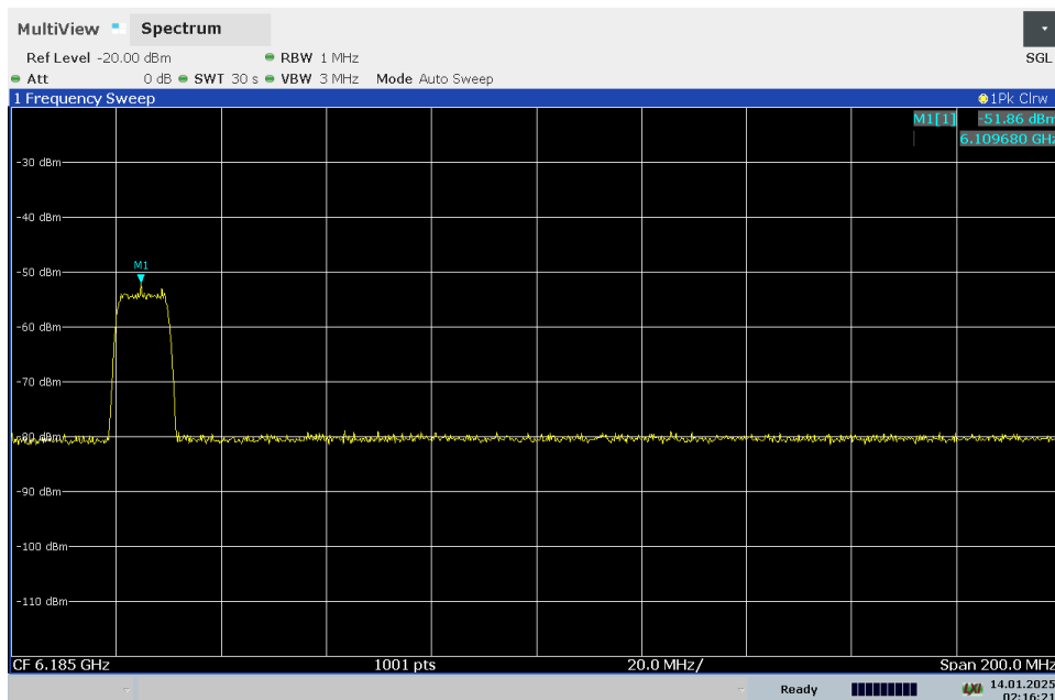
Plot 7-196. 160MHz Bandwidth, AWGN Signal Injected at Center – Channel 47
