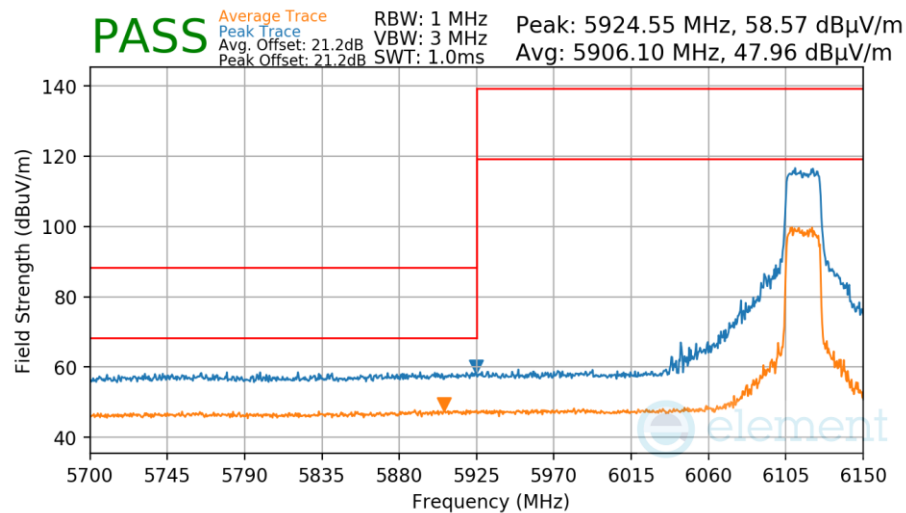
Plot 7-214. Antenna 1 Radiated Lower Band Edge (Peak & Average – UNII Band 5)
