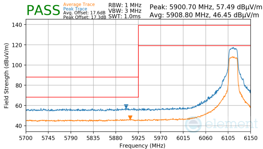
Plot 7-208. Antenna 0 Radiated Lower Band Edge (Peak & Average – UNII Band 5)
