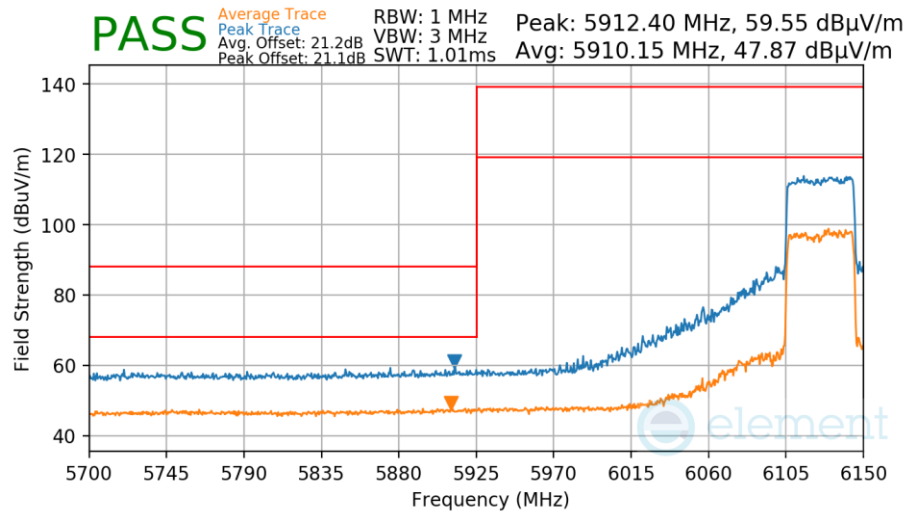
Plot 7-215. Antenna 1 Radiated Lower Band Edge (Peak & Average – UNII Band 5)
