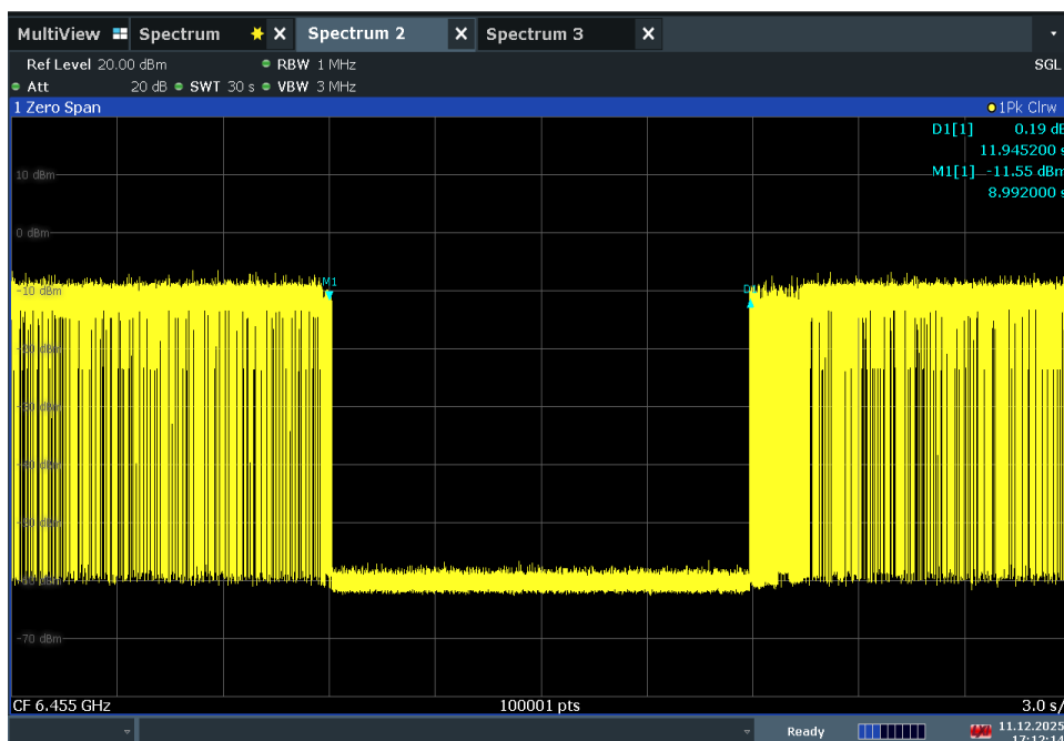
Plot 7-182. Contention Based Protocol Timing Plot – UNII 6 – 20MHz Channel 101
