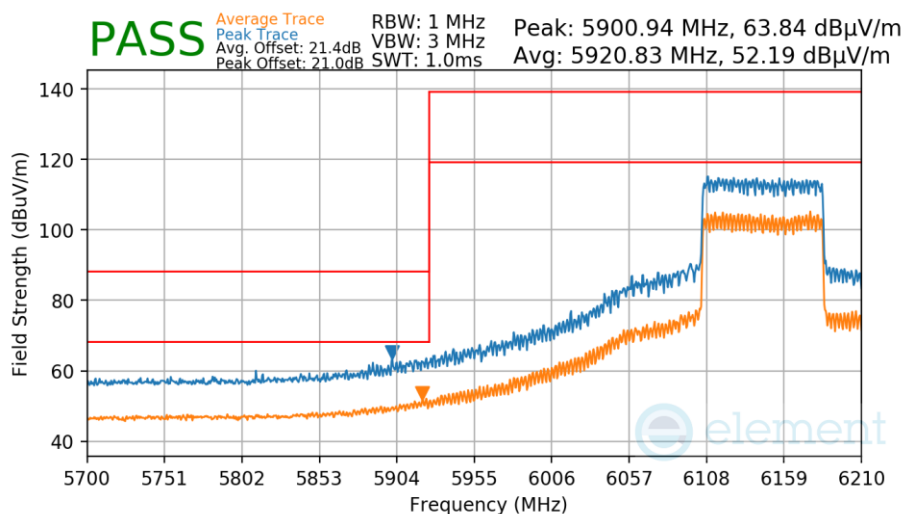
Plot 7-220. SDM Radiated Lower Band Edge (Peak & Average – UNII Band 5)
