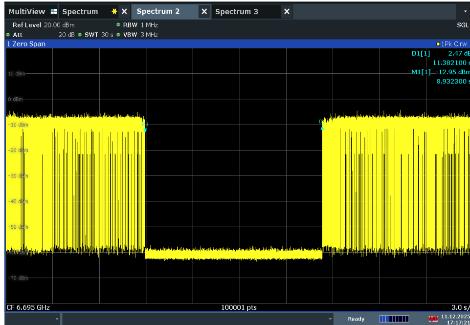
Plot 7-186. Contention Based Protocol Timing Plot – UNII 7 – 20MHz Channel 149
