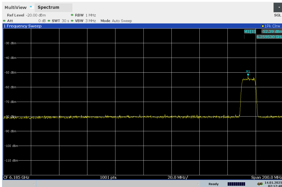
Plot 7-195. 160MHz Bandwidth, AWGN Signal Injected at Low End – Channel 47
