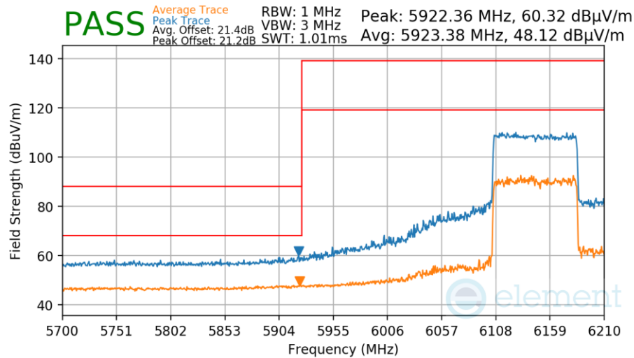
Plot 7-211. Antenna 0 Radiated Lower Band Edge (Peak & Average – UNII Band 5)
