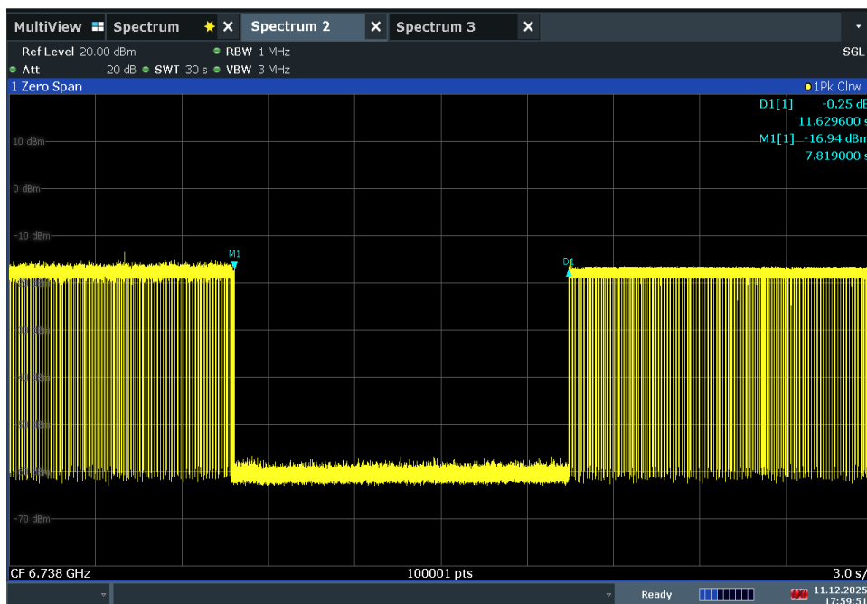
Plot 7-189. Contention Based Protocol Timing Plot – UNII 7 – 160MHz Channel 143 – High
