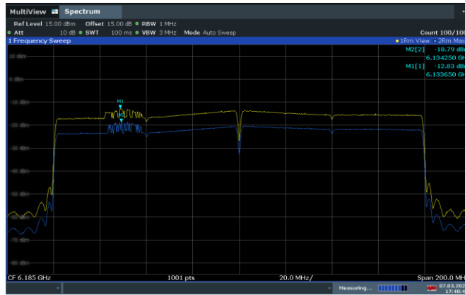
Plot 7-198. 160MHz Bandwidth – 6185MHz Antenna 0
