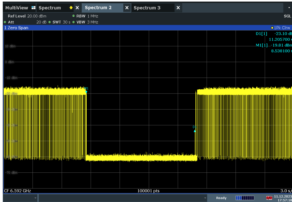
Plot 7-187. Contention Based Protocol Timing Plot – UNII 7 – 160MHz Channel 143 – Low
