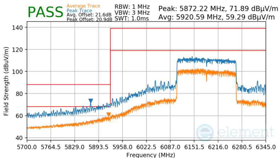
Plot 7-221. SDM Radiated Lower Band Edge (Peak & Average – UNII Band 5)
