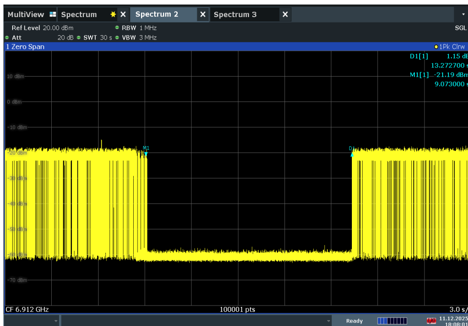
Plot 7-191. Contention Based Protocol Timing Plot – UNII 8 – 160MHz Channel 207 – Low
