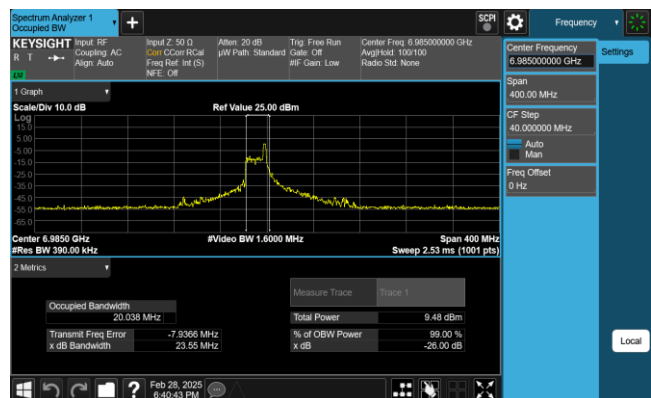
Plot 7-52. 26dB & 99% Bandwidth Plot Antenna 0 (160MHz 802.11ax RU26 (UNII Band 8) – Ch. 207)
