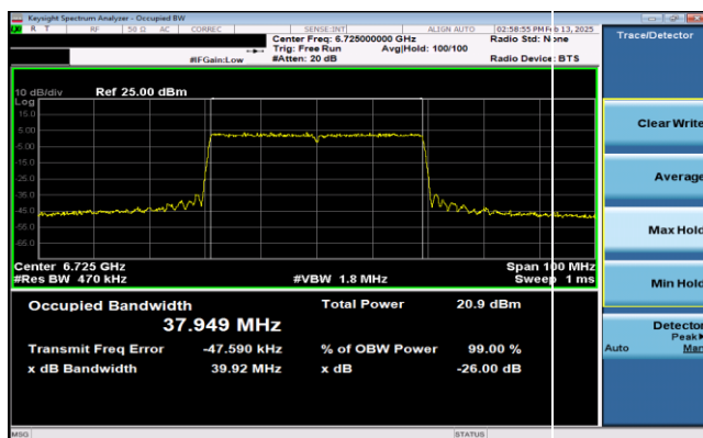
Plot 7-46. 26dB & 99% Bandwidth Plot Antenna 0 (40MHz 802.11ax RU484 (UNII Band 7) – Ch. 155)
