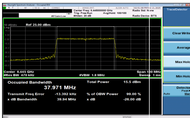
Plot 7-38. 26dB & 99% Bandwidth Plot Antenna 0 (40MHz 802.11ax RU484 (UNII Band 6) – Ch. 99)
