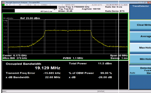
Plot 7-29. 26dB & 99% Bandwidth Plot Antenna 0 (20MHz 802.11ax RU242 (UNII Band 5) – Ch. 45)
