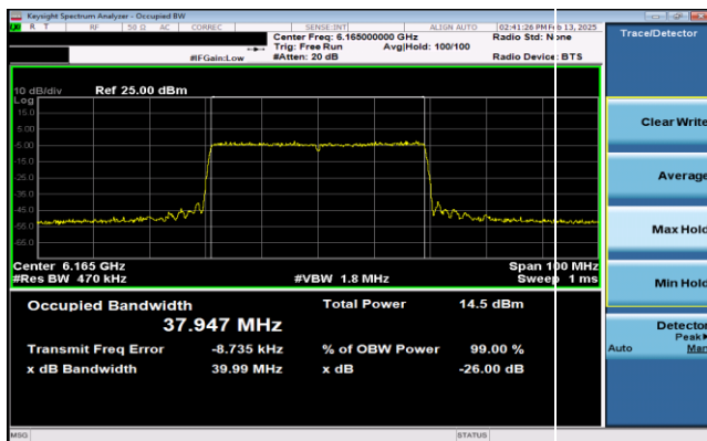
Plot 7-30. 26dB & 99% Bandwidth Plot Antenna 0 (40MHz 802.11ax RU484 (UNII Band 5) – Ch. 43)
