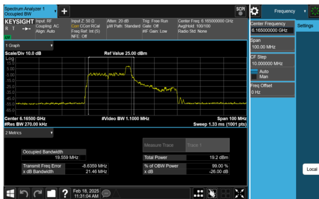
Plot 7-58. 26dB & 99% Bandwidth Plot Antenna 1 (40MHz 802.11ax RU26 (UNII Band 5) – Ch. 43)
