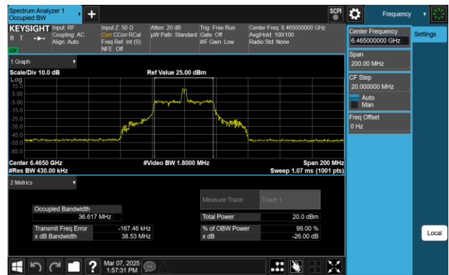
Plot 7-11. 26dB & 99% Bandwidth Plot Antenna 0 (80MHz 802.11ax RU26 (UNII Band 6) – Ch. 103)
