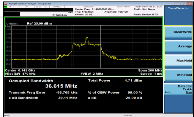
Plot 7-27. 26dB & 99% Bandwidth Plot Antenna 0 (80MHz 802.11ax RU26 (UNII Band 5) – Ch. 39)
