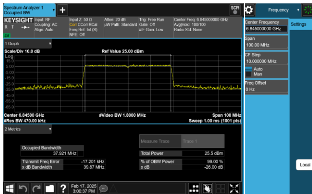
Plot 7-22. 26dB & 99% Bandwidth Plot Antenna 0 (40MHz 802.11ax RU484 (UNII Band 7) – Ch. 179)
