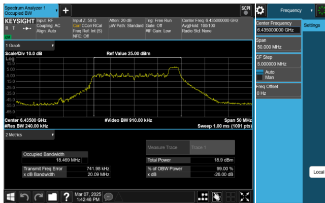
Plot 7-9. 26dB & 99% Bandwidth Plot Antenna 0 (20MHz 802.11ax RU26 (UNII Band 6) – Ch. 97)
