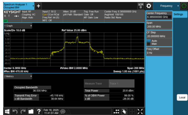
Plot 7-59. 26dB & 99% Bandwidth Plot Antenna 1 (80MHz 802.11ax RU26 (UNII Band 5) – Ch. 87)
