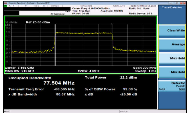
Plot 7-39. 26dB & 99% Bandwidth Plot Antenna 0 (80MHz 802.11ax RU996 (UNII Band 6) – Ch. 103)
