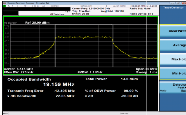
Plot 7-37. 26dB & 99% Bandwidth Plot Antenna 0 (20MHz 802.11ax RU242 (UNII Band 6) – Ch. 113)
