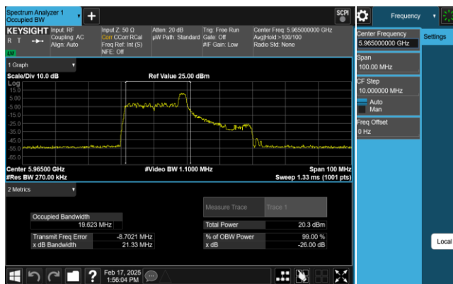
Plot 7-2. 26dB & 99% Bandwidth Plot Antenna 0 (40MHz 802.11ax RU26 (UNII Band 5) – Ch. 3)
