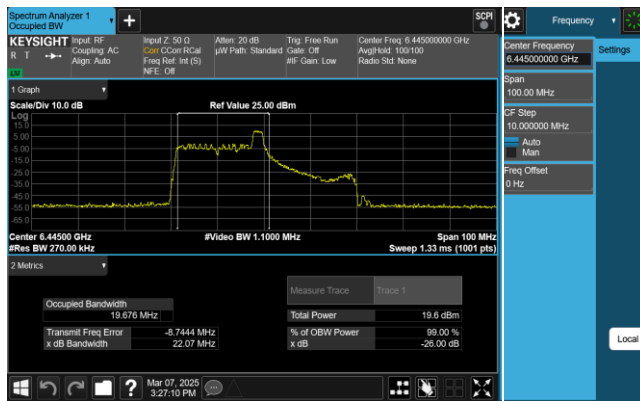
Plot 7-66. 26dB & 99% Bandwidth Plot Antenna 1 (40MHz 802.11ax RU26 (UNII Band 6) – Ch. 99)
