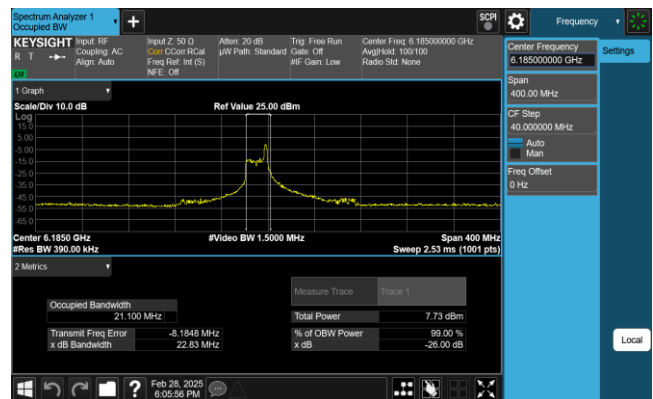
Plot 7-28. 26dB & 99% Bandwidth Plot Antenna 0 (160MHz 802.11ax RU26 (UNII Band 5) – Ch. 47)
