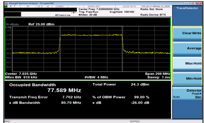
Plot 7-55. 26dB & 99% Bandwidth Plot Antenna 0 (80MHz 802.11ax RU996 (UNII Band 8) – Ch. 215)
