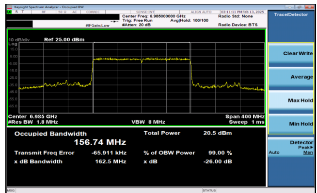
Plot 7-56. 26dB & 99% Bandwidth Plot Antenna 0 (160MHz 802.11ax RU996x2 (UNII Band 8) – Ch. 207)
