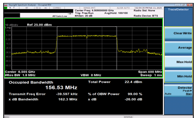
Plot 7-40. 26dB & 99% Bandwidth Plot Antenna 0 (160MHz 802.11ax RU996x2 (UNII Band 6) – Ch. 111)
