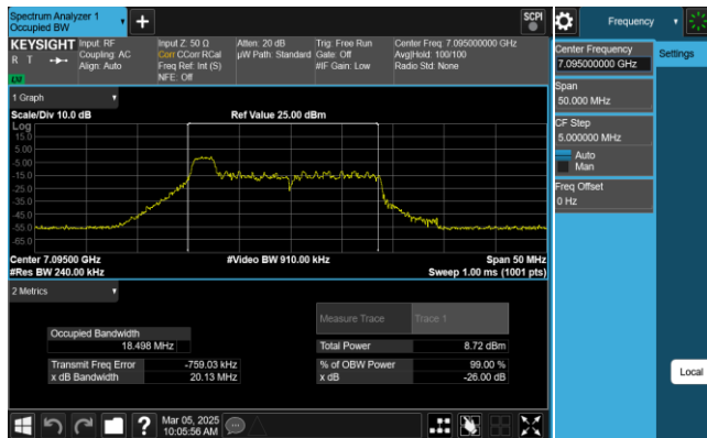
Plot 7-49. 26dB & 99% Bandwidth Plot Antenna 0 (20MHz 802.11ax RU26 (UNII Band 8) – Ch. 229)
