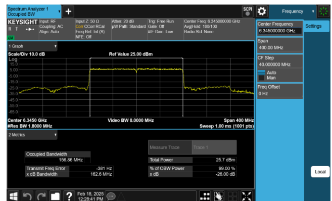
Plot 7-64. 26dB & 99% Bandwidth Plot Antenna 1 (160MHz 802.11ax RU996x2 (UNII Band 5) – Ch. 79)
