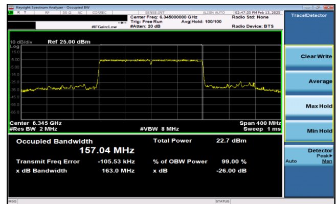
Plot 7-32. 26dB & 99% Bandwidth Plot Antenna 0 (160MHz 802.11ax RU996x2 (UNII Band 5) – Ch. 79)
