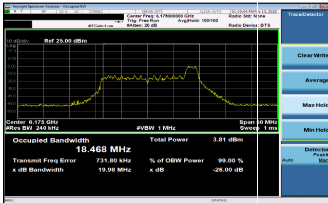
Plot 7-25. 26dB & 99% Bandwidth Plot Antenna 0 (20MHz 802.11ax RU26 (UNII Band 5) – Ch. 45)
