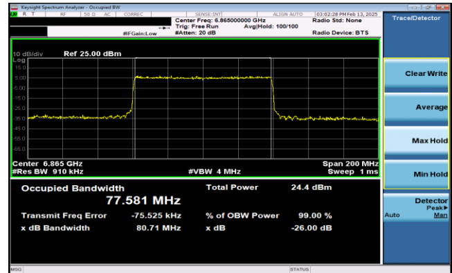
Plot 7-47. 26dB & 99% Bandwidth Plot Antenna 0 (80MHz 802.11ax RU996 (UNII Band 7) – Ch. 183)
