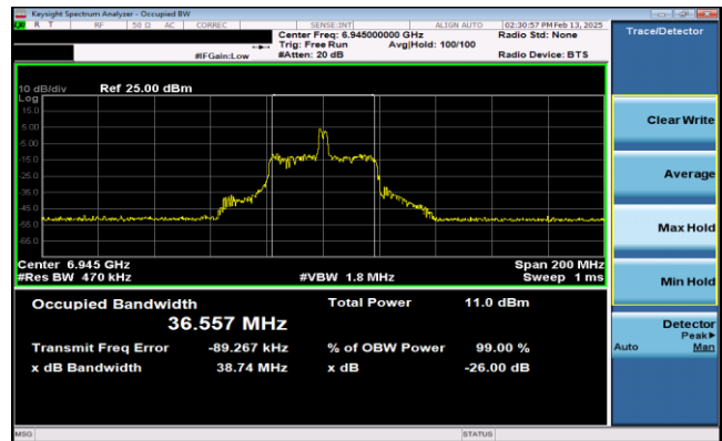
Plot 7-51. 26dB & 99% Bandwidth Plot Antenna 0 (80MHz 802.11ax RU26 (UNII Band 8) – Ch. 199)
