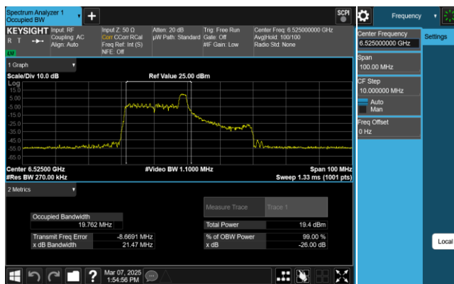
Plot 7-10. 26dB & 99% Bandwidth Plot Antenna 0 (40MHz 802.11ax RU26 (UNII Band 6) – Ch. 115)
