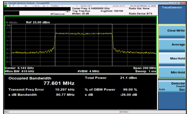
Plot 7-31. 26dB & 99% Bandwidth Plot Antenna 0 (80MHz 802.11ax RU996 (UNII Band 5) – Ch. 39)
