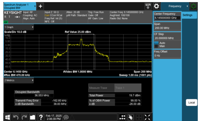
Plot 7-3. 26dB & 99% Bandwidth Plot Antenna 0 (80MHz 802.11ax RU26 (UNII Band 5) – Ch. 39)
