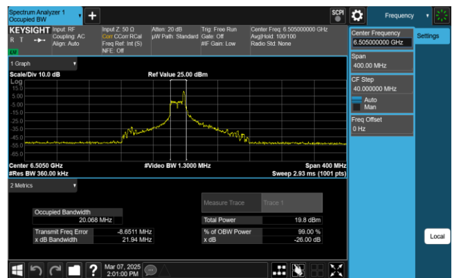
Plot 7-12. 26dB & 99% Bandwidth Plot Antenna 0 (160MHz 802.11ax RU26 (UNII Band 6) – Ch. 111)
