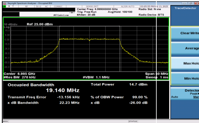
Plot 7-53. 26dB & 99% Bandwidth Plot Antenna 0 (20MHz 802.11ax RU242 (UNII Band 8) – Ch. 209)
