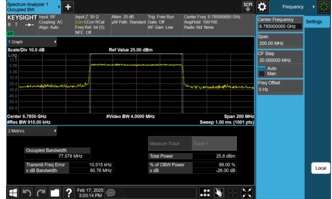
Plot 7-23. 26dB & 99% Bandwidth Plot Antenna 0 (80MHz 802.11ax RU996 (UNII Band 7) – Ch. 167)
