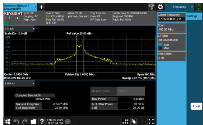
Plot 7-4. 26dB & 99% Bandwidth Plot Antenna 0 (160MHz 802.11ax RU26 (UNII Band 5) – Ch. 47)
