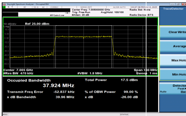
Plot 7-54. 26dB & 99% Bandwidth Plot Antenna 0 (40MHz 802.11ax RU484 (UNII Band 8) – Ch. 211)
