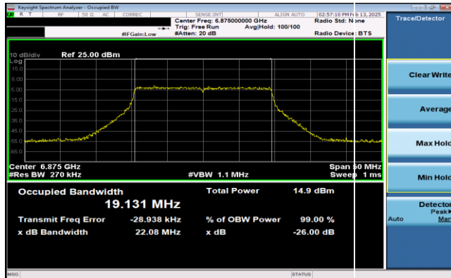
Plot 7-45. 26dB & 99% Bandwidth Plot Antenna 0 (20MHz 802.11ax RU242 (UNII Band 7) – Ch. 185)
