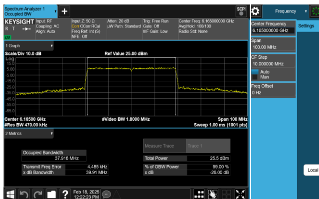
Plot 7-62. 26dB & 99% Bandwidth Plot Antenna 1 (40MHz 802.11ax RU484 (UNII Band 5) – Ch. 43)
