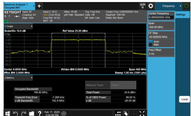
Plot 7-24. 26dB & 99% Bandwidth Plot Antenna 0 (160MHz 802.11ax RU996x2 (UNII Band 7) – Ch. 143)
