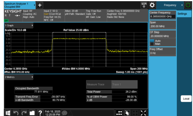
Plot 7-63. 26dB & 99% Bandwidth Plot Antenna 1 (80MHz 802.11ax RU996 (UNII Band 5) – Ch. 87)
