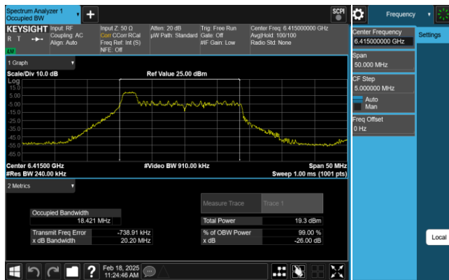
Plot 7-57. 26dB & 99% Bandwidth Plot Antenna 1 (20MHz 802.11ax RU26 (UNII Band 5) – Ch. 93)
