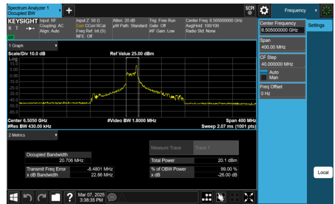
Plot 7-68. 26dB & 99% Bandwidth Plot Antenna 1 (160MHz 802.11ax RU26 (UNII Band 6) – Ch. 111)
