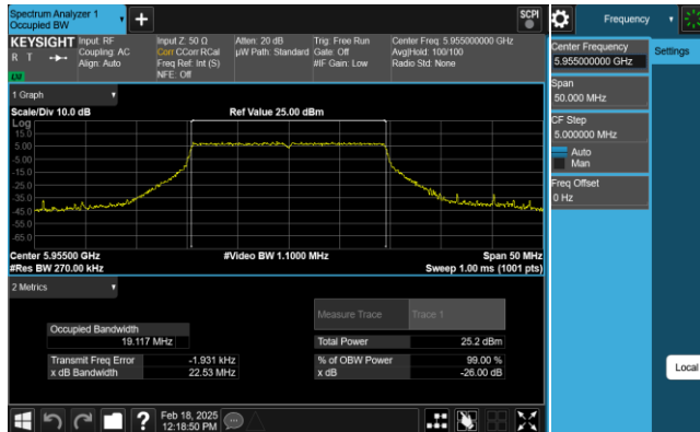
Plot 7-61. 26dB & 99% Bandwidth Plot Antenna 1 (20MHz 802.11ax RU242 (UNII Band 5) – Ch. 1)
