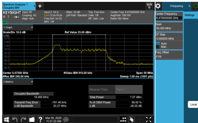
Plot 7-89. 26dB & 99% Bandwidth Plot Antenna 1 (20MHz 802.11ax RU26 (UNII Band 6) – Ch. 105)
