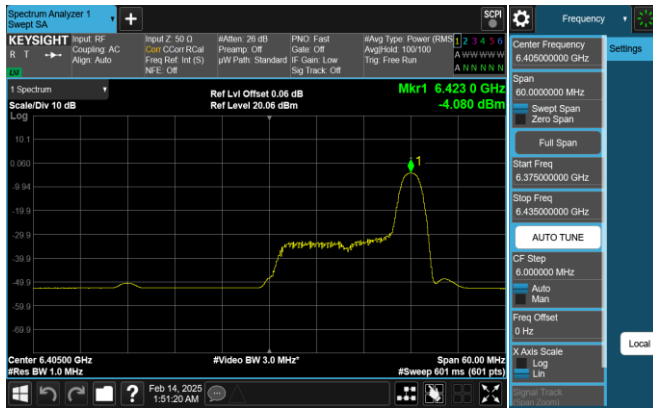
Plot 7-138. PSD Plot Antenna 0 (40MHz 802.11ax RU26 (UNII Band 5) – Ch. 91)
