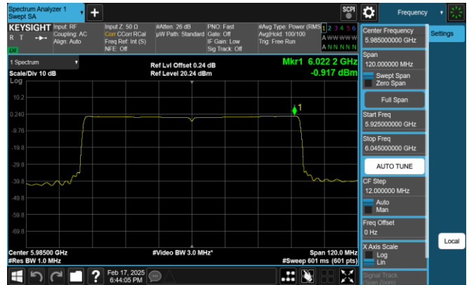
Plot 7-119. PSD Plot Antenna 0 (80MHz 802.11ax RU996 (UNII Band 5) - Ch. 7)
