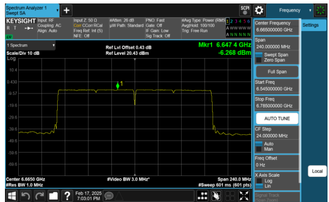
Plot 7-136. PSD Plot Antenna 0 (160MHz 802.11ax RU996x2 (UNII Band 7) – Ch. 143)
