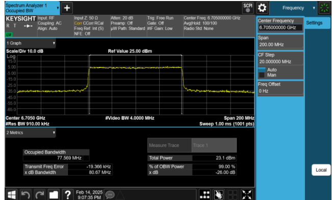
Plot 7-103. 26dB & 99% Bandwidth Plot Antenna 1 (80MHz 802.11ax RU996 (UNII Band 7) – Ch. 151)
