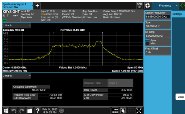
Plot 7-105. 26dB & 99% Bandwidth Plot Antenna 1 (20MHz 802.11ax RU26 (UNII Band 8) - Ch. 189)
