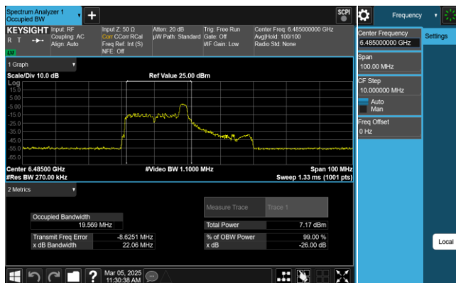
Plot 7-90. 26dB & 99% Bandwidth Plot Antenna 1 (40MHz 802.11ax RU26 (UNII Band 6) – Ch. 107)
