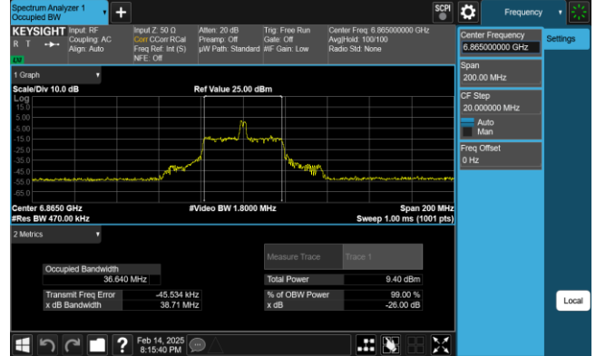
Plot 7-99. 26dB & 99% Bandwidth Plot Antenna 1 (80MHz 802.11ax RU26 (UNII Band 7) – Ch. 183)
