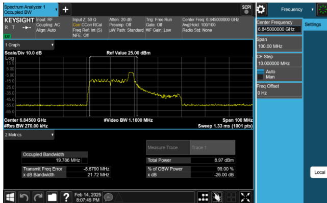
Plot 7-98. 26dB & 99% Bandwidth Plot Antenna 1 (40MHz 802.11ax RU26 (UNII Band 7) – Ch. 179)
