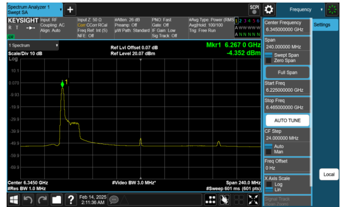
Plot 7-140. PSD Plot Antenna 0 (160MHz 802.11ax RU26 (UNII Band 5) – Ch. 79)
