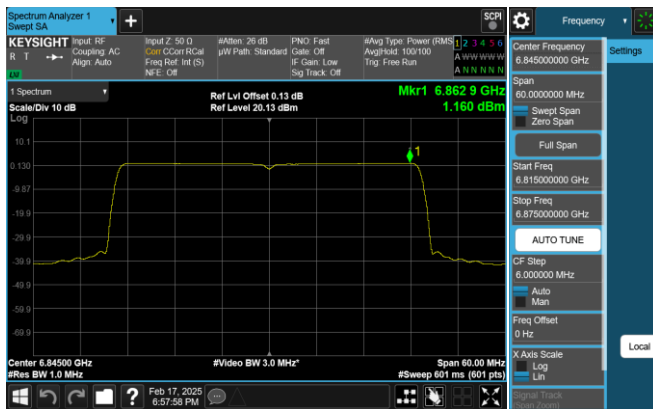
Plot 7-134. PSD Plot Antenna 0 (40MHz 802.11ax RU484 (UNII Band 7) – Ch. 179)
