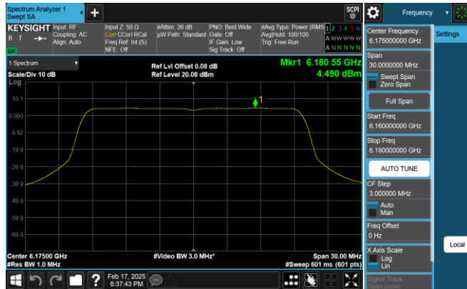
Plot 7-117. PSD Plot Antenna 0 (20MHz 802.11ax RU242 (UNII Band 5) - Ch. 45)
