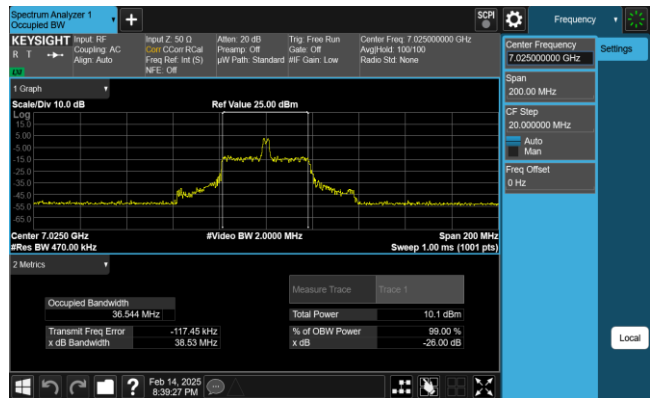
Plot 7-107. 26dB & 99% Bandwidth Plot Antenna 1 (80MHz 802.11ax RU26 (UNII Band 8) - Ch.215)
