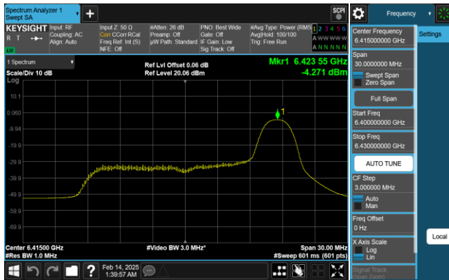
Plot 7-137. PSD Plot Antenna 0 (20MHz 802.11ax RU26 (UNII Band 5) – Ch. 93)
