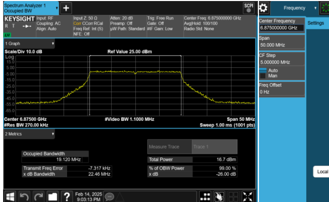
Plot 7-101. 26dB & 99% Bandwidth Plot Antenna 1 (20MHz 802.11ax RU242 (UNII Band 7) – Ch. 185)
