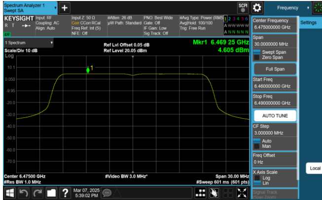
Plot 7-125. PSD Plot Antenna 0 (20MHz 802.11ax RU242 (UNII Band 6) – Ch. 105)
