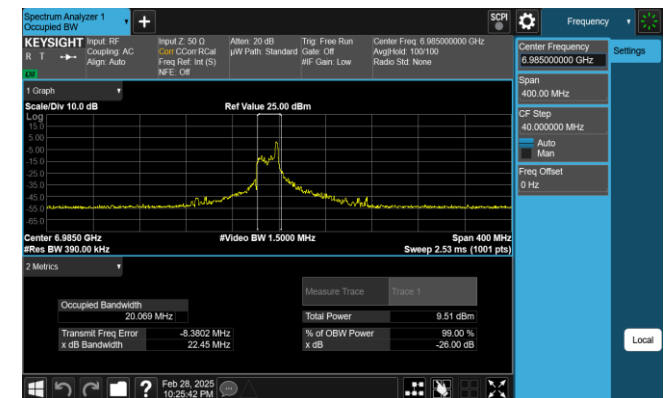
Plot 7-108. 26dB & 99% Bandwidth Plot Antenna 1 (160MHz 802.11ax RU26 (UNII Band 8) - Ch. 207)
