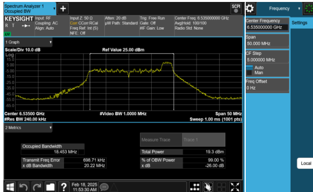
Plot 7-73. 26dB & 99% Bandwidth Plot Antenna 1 (20MHz 802.11ax RU26 (UNII Band 7) – Ch. 117)
