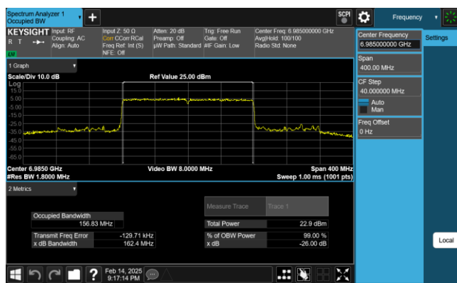
Plot 7-112. 26dB & 99% Bandwidth Plot Antenna 1 (160MHz 802.11ax RU996x2 (UNII Band 8) – Ch. 207)
