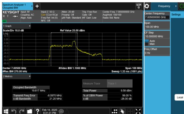
Plot 7-106. 26dB & 99% Bandwidth Plot Antenna 1 (40MHz 802.11ax RU26 (UNII Band 8) - Ch. 211)
