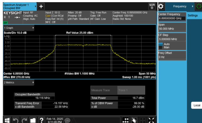
Plot 7-109. 26dB & 99% Bandwidth Plot Antenna 1 (20MHz 802.11ax RU242 (UNII Band 8) – Ch. 189)
