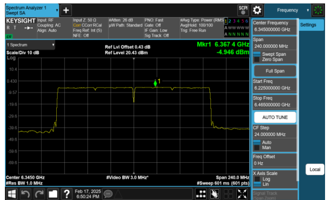
Plot 7-120. PSD Plot Antenna 0 (160MHz 802.11ax RU996x2 (UNII Band 5) - Ch. 79)
