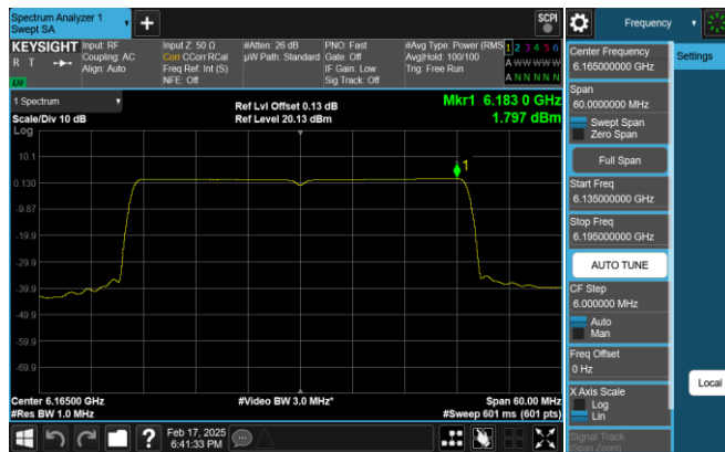
Plot 7-118. PSD Plot Antenna 0 (40MHz 802.11ax RU484 (UNII Band 5) - Ch. 43)
