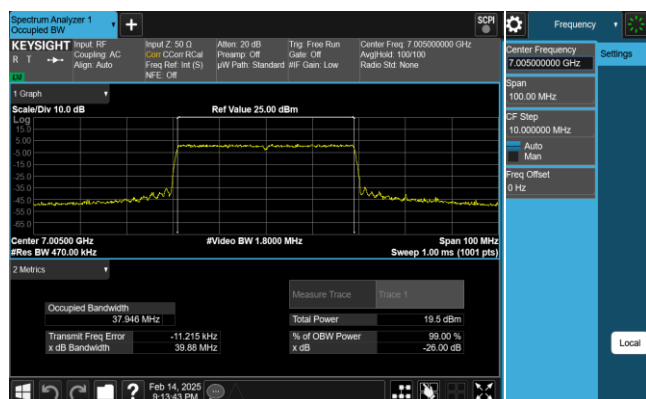
Plot 7-110. 26dB & 99% Bandwidth Plot Antenna 1 (40MHz 802.11ax RU484 (UNII Band 8) – Ch. 211)
