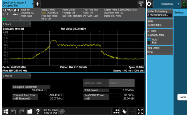
Plot 7-97. 26dB & 99% Bandwidth Plot Antenna 1 (20MHz 802.11ax RU26 (UNII Band 7) – Ch. 149)
