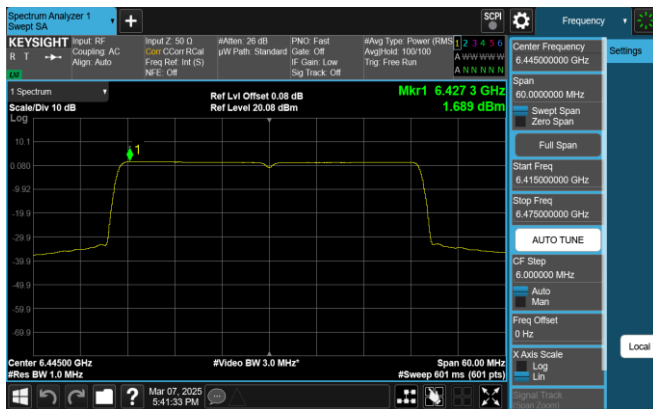
Plot 7-126. PSD Plot Antenna 0 (40MHz 802.11ax RU484 (UNII Band 6) – Ch. 99)
