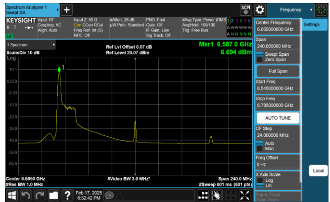
Plot 7-132. PSD Plot Antenna 0 (160MHz 802.11ax RU26 (UNII Band 7) – Ch. 143)
