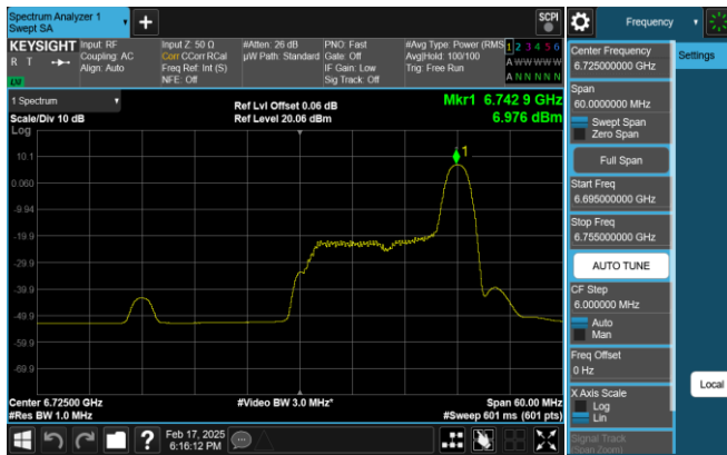
Plot 7-130. PSD Plot Antenna 0 (40MHz 802.11ax RU26 (UNII Band 7) – Ch. 155)
