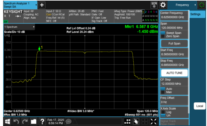
Plot 7-135. PSD Plot Antenna 0 (80MHz 802.11ax RU996 (UNII Band 7) – Ch. 135)
