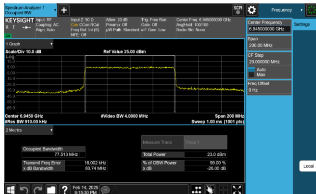
Plot 7-111. 26dB & 99% Bandwidth Plot Antenna 1 (80MHz 802.11ax RU996 (UNII Band 8) – Ch. 199)
