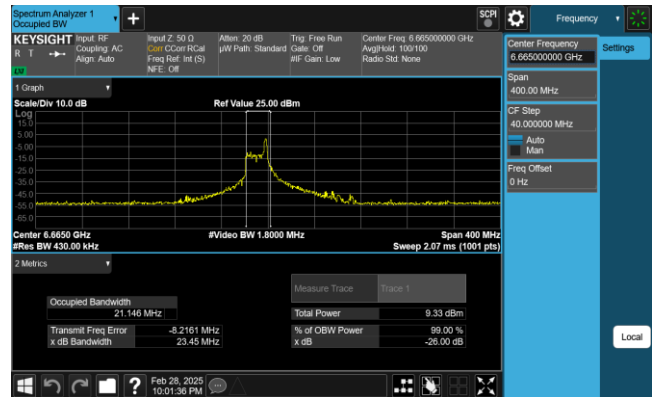
Plot 7-100. 26dB & 99% Bandwidth Plot Antenna 1 (160MHz 802.11ax RU26 (UNII Band 7) – Ch. 143)
