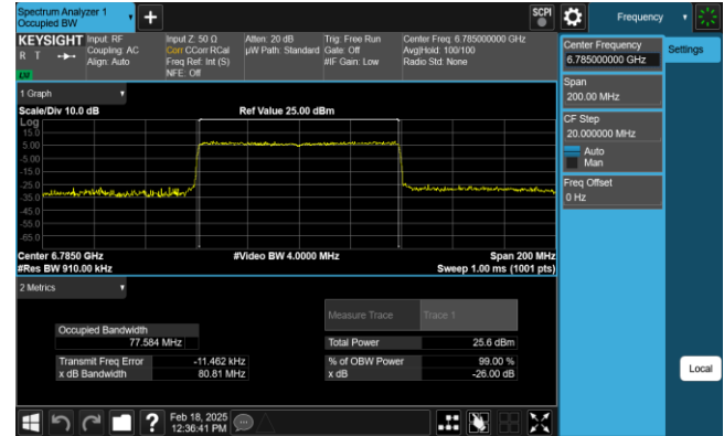
Plot 7-79. 26dB & 99% Bandwidth Plot Antenna 1 (80MHz 802.11ax RU996 (UNII Band 7) – Ch. 167)
