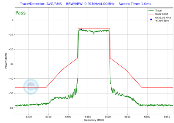
Plot 7-375. In-Band Emission Plot Antenna 0 (80MHz 802.11ax RU996 (UNII Band 6) – Ch. 103)
