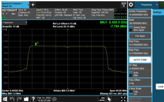
Plot 7-299. PSD Plot SDM Antenna 0 (40MHz 802.11ax RU484 (UNII Band 6) - Ch. 99)
