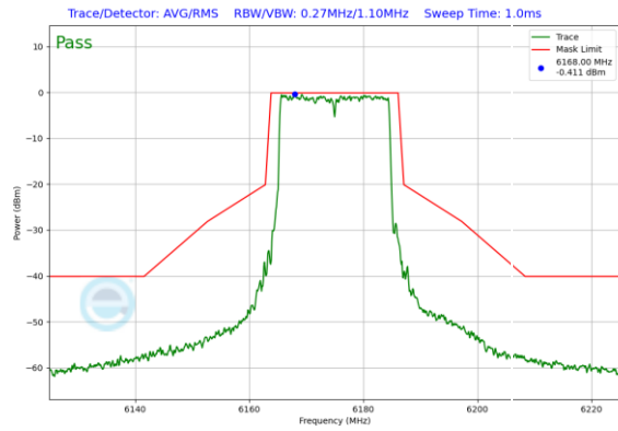
Plot 7-341. In-Band Emission Plot Antenna 0 (20MHz 802.11ax RU242 (UNII Band 5) – Ch. 45)
