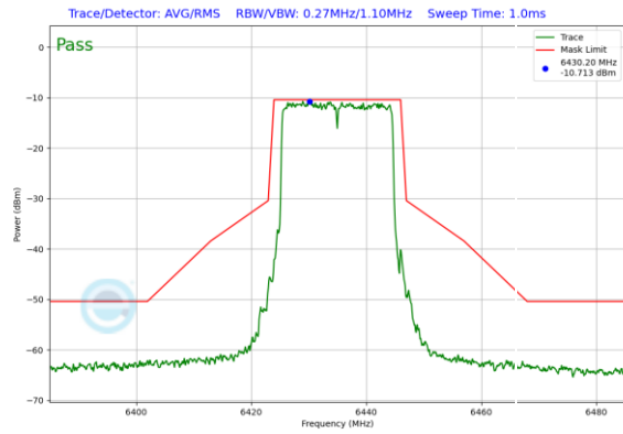
Plot 7-373. In-Band Emission Plot Antenna 0 (20MHz 802.11ax RU242 (UNII Band 6) – Ch. 97)
