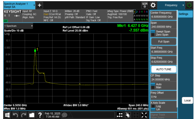
Plot 7-296. PSD Plot SDM Antenna 1 (160MHz 802.11ax RU26 (UNII Band 6) - Ch. 111)
