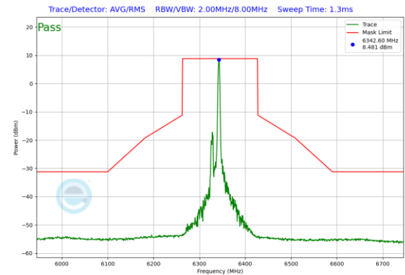
Plot 7-340. In-Band Emission Plot Antenna 0 (160MHz 802.11ax RU26 (UNII Band 5) – Ch. 79)
