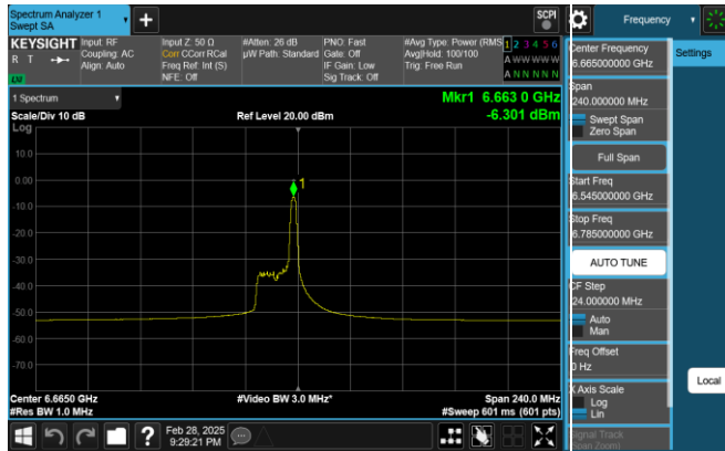
Plot 7-311. PSD Plot SDM Antenna 0 (160MHz 802.11ax RU26 (UNII Band 7) - Ch. 143)
