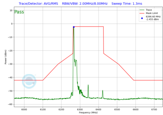
Plot 7-364. In-Band Emission Plot Antenna 0 (160MHz 802.11ax RU26 (UNII Band 5) – Ch. 79)
