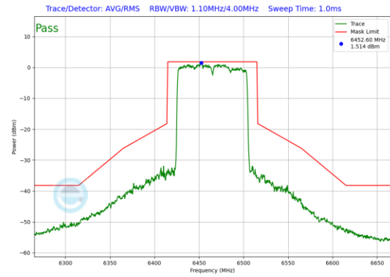
Plot 7-351. In-Band Emission Plot Antenna 0 (80MHz 802.11ax RU996 (UNII Band 6) – Ch. 103)
