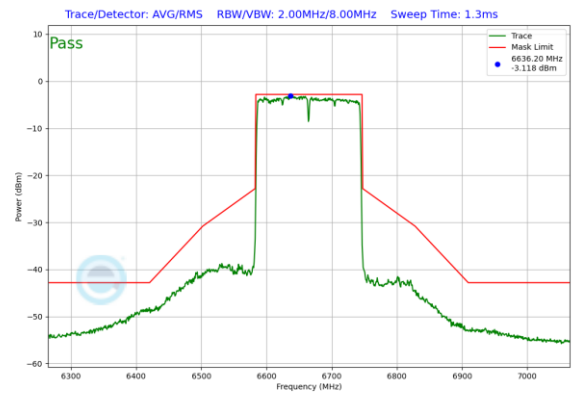
Plot 7-360. In-Band Emission Plot Antenna 0 (160MHz 802.11ax RU996x2 (UNII Band 7) – Ch. 143)
