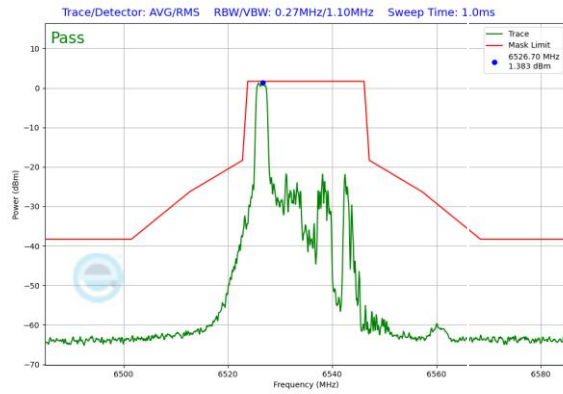
Plot 7-353. In-Band Emission Plot Antenna 0 (20MHz 802.11ax RU26 (UNII Band 7) – Ch. 117)
