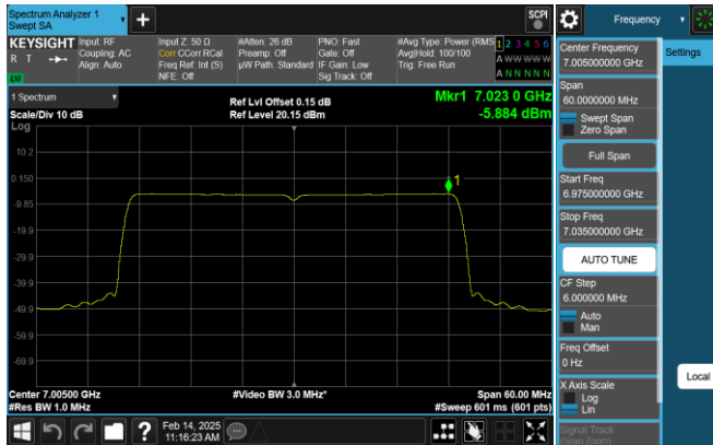
Plot 7-331. PSD Plot SDM Antenna 0 (40MHz 802.11ax RU484 (UNII Band 8) - Ch. 211)
