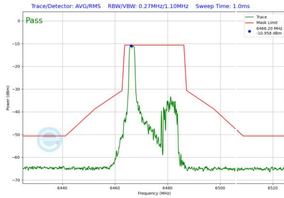
Plot 7-369. In-Band Emission Plot Antenna 0 (20MHz 802.11ax RU26 (UNII Band 6) – Ch. 105)
