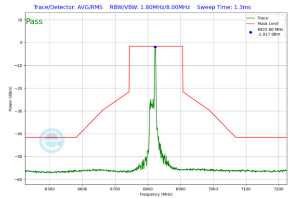
Plot 7-380. In-Band Emission Plot Antenna 0 (160MHz 802.11ax RU26 (UNII Band 7) – Ch. 175)
