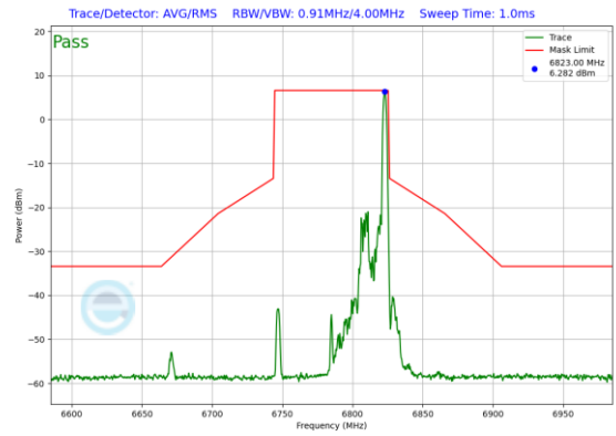
Plot 7-355. In-Band Emission Plot Antenna 0 (80MHz 802.11ax RU26 (UNII Band 7) – Ch. 167)
