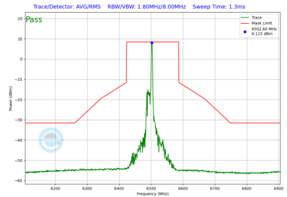
Plot 7-348. In-Band Emission Plot Antenna 0 (160MHz 802.11ax RU26 (UNII Band 6) – Ch. 111)
