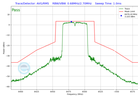
Plot 7-350. In-Band Emission Plot Antenna 0 (40MHz 802.11ax RU484 (UNII Band 6) – Ch. 107)
