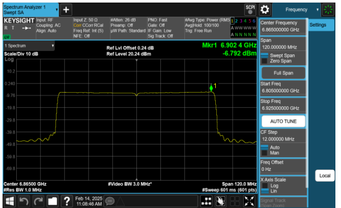
Plot 7-317. PSD Plot SDM Antenna 0 (80MHz 802.11ax RU996 (UNII Band 7) - Ch. 183)
