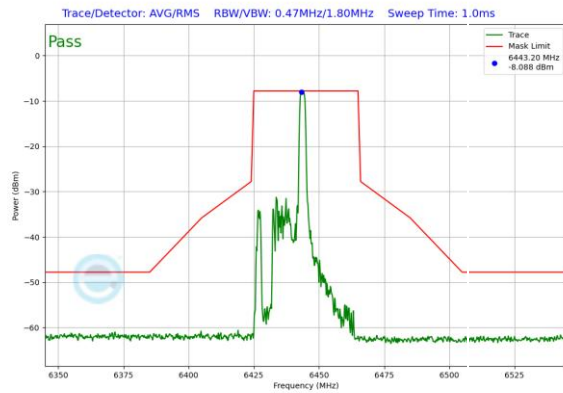
Plot 7-370. In-Band Emission Plot Antenna 0 (40MHz 802.11ax RU26 (UNII Band 6) – Ch. 99)
