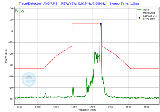
Plot 7-339. In-Band Emission Plot Antenna 0 (80MHz 802.11ax RU26 (UNII Band 5) – Ch. 87)
