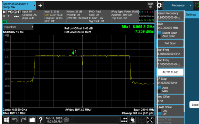
Plot 7-335. PSD Plot SDM Antenna 0 (160MHz 802.11ax RU996x2 (UNII Band 8) – Ch. 207)
