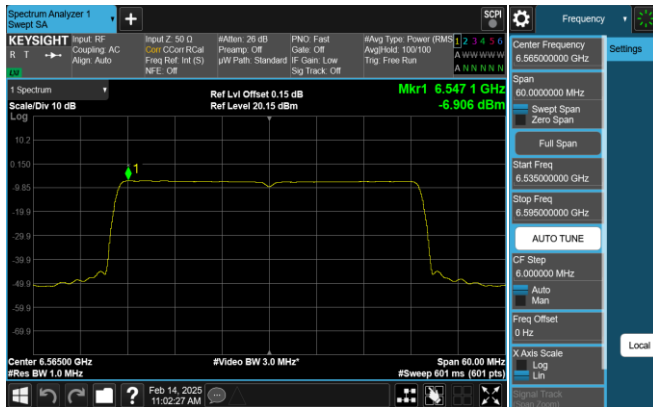
Plot 7-315. PSD Plot SDM Antenna 0 (40MHz 802.11ax RU484 (UNII Band 7) - Ch. 123)
