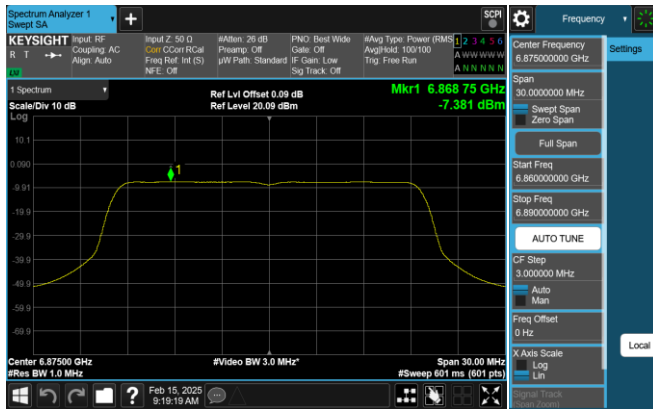
Plot 7-314. PSD Plot SDM Antenna 1 (20MHz 802.11ax RU242 (UNII Band 7) - Ch. 185)
