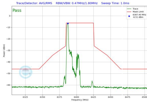
Plot 7-362. In-Band Emission Plot Antenna 0 (40MHz 802.11ax RU26 (UNII Band 5) – Ch. 91)
