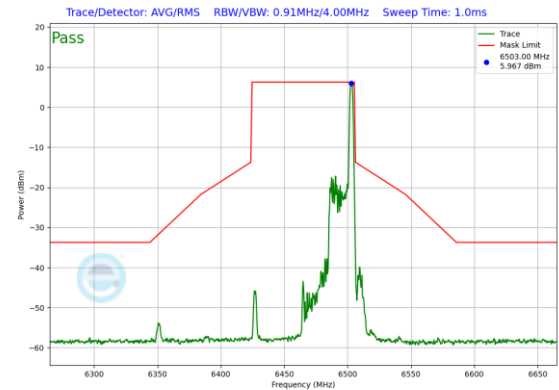
Plot 7-347. In-Band Emission Plot Antenna 0 (80MHz 802.11ax RU26 (UNII Band 6) – Ch. 103)
