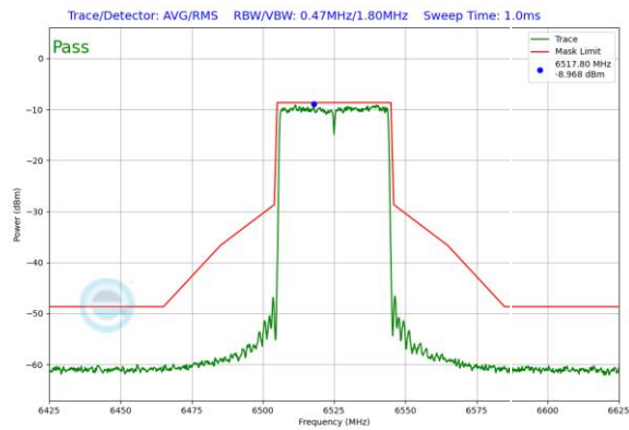
Plot 7-374. In-Band Emission Plot Antenna 0 (40MHz 802.11ax RU484 (UNII Band 6) – Ch. 115)
