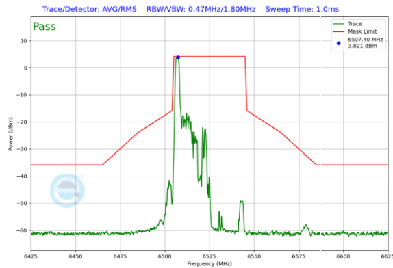
Plot 7-346. In-Band Emission Plot Antenna 0 (40MHz 802.11ax RU26 (UNII Band 6) – Ch. 115)
