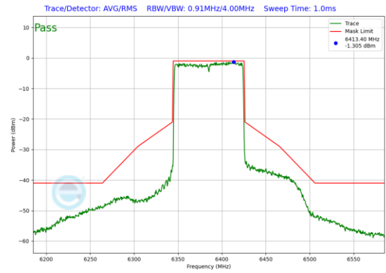
Plot 7-343. In-Band Emission Plot Antenna 0 (80MHz 802.11ax RU996 (UNII Band 5) – Ch. 87)
