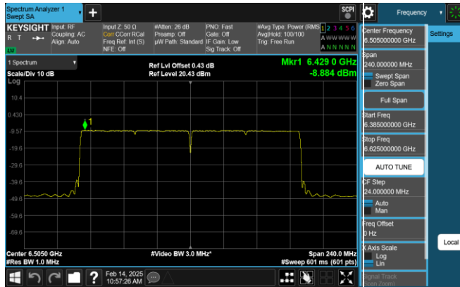
Plot 7-303. PSD Plot SDM Antenna 0 (160MHz 802.11ax RU996x2 (UNII Band 6) – Ch. 111)
