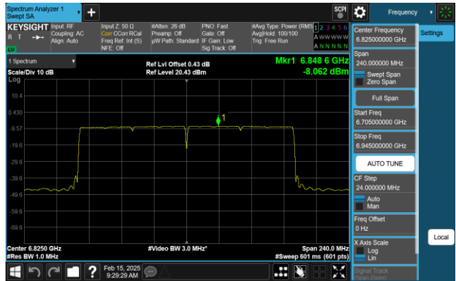
Plot 7-320. PSD Plot SDM Antenna 1 (160MHz 802.11ax RU996x2 (UNII Band 7) – Ch. 175)
