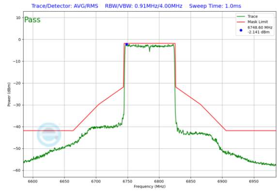
Plot 7-359. In-Band Emission Plot Antenna 0 (80MHz 802.11ax RU996 (UNII Band 7) – Ch. 167)
