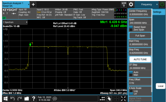
Plot 7-304. PSD Plot SDM Antenna 1 (160MHz 802.11ax RU996x2 (UNII Band 6) – Ch. 111)
