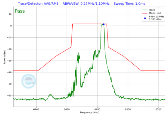
Plot 7-345. In-Band Emission Plot Antenna 0 (20MHz 802.11ax RU26 (UNII Band 6) – Ch. 105)
