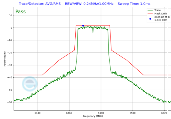
Plot 7-349. In-Band Emission Plot Antenna 0 (20MHz 802.11ax RU242 (UNII Band 6) – Ch. 105)
