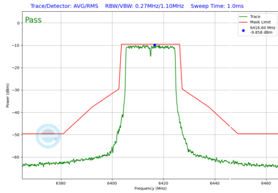
Plot 7-365. In-Band Emission Plot Antenna 0 (20MHz 802.11ax RU242 (UNII Band 5) – Ch93)
