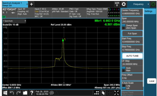
Plot 7-312. PSD Plot SDM Antenna 1 (160MHz 802.11ax RU26 (UNII Band 7) - Ch. 143)
