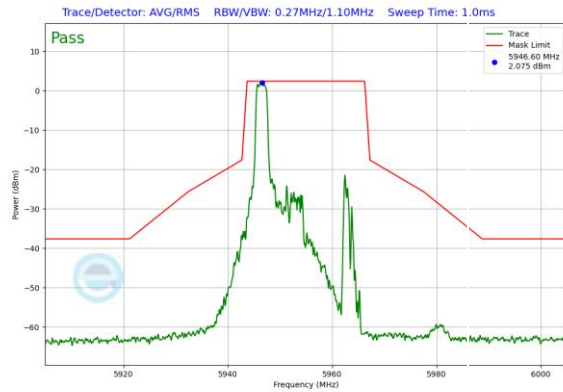
Plot 7-337. In-Band Emission Plot Antenna 0 (20MHz 802.11ax RU26 (UNII Band 5) – Ch. 1)
