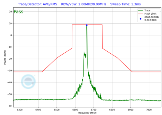
Plot 7-356. In-Band Emission Plot Antenna 0 (160MHz 802.11ax RU26 (UNII Band 7) – Ch. 143)
