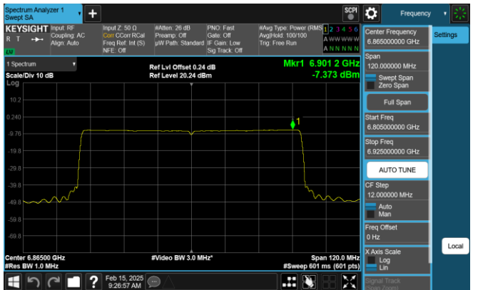
Plot 7-318. PSD Plot SDM Antenna 1 (80MHz 802.11ax RU996 (UNII Band 7) - Ch. 183)
