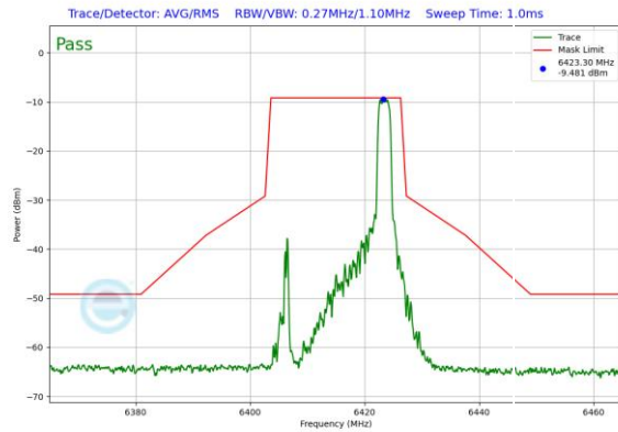
Plot 7-361. In-Band Emission Plot Antenna 0 (20MHz 802.11ax RU26 (UNII Band 5) – Ch. 93)
