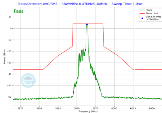
Plot 7-338. In-Band Emission Plot Antenna 0 (40MHz 802.11ax RU26 (UNII Band 5) – Ch. 3)
