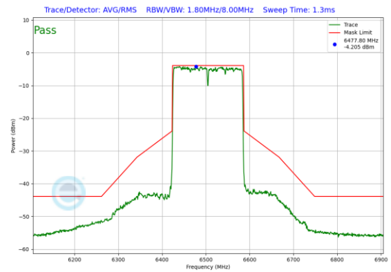
Plot 7-376. In-Band Emission Plot Antenna 0 (160MHz 802.11ax RU996x2 (UNII Band 6) – Ch. 111)
