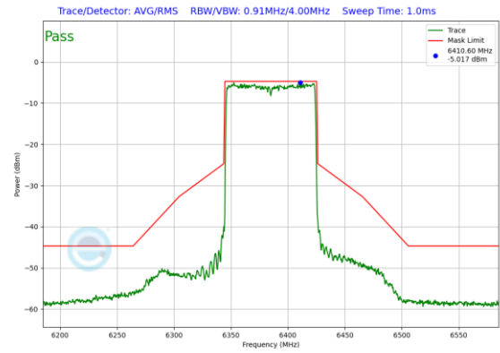
Plot 7-367. In-Band Emission Plot Antenna 0 (80MHz 802.11ax RU996 (UNII Band 5) – Ch. 87)
