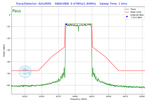
Plot 7-366. In-Band Emission Plot Antenna 0 (40MHz 802.11ax RU484 (UNII Band 5) – Ch. 91)
