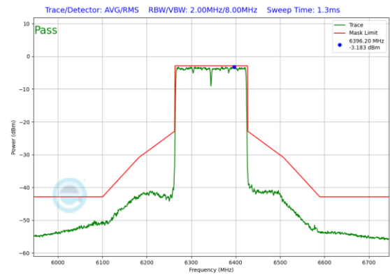
Plot 7-368. In-Band Emission Plot Antenna 0 (160MHz 802.11ax RU996x2 (UNII Band 5) – Ch. 79)
