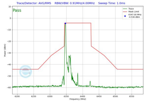
Plot 7-363. In-Band Emission Plot Antenna 0 (80MHz 802.11ax RU26 (UNII Band 5) – Ch. 87)
