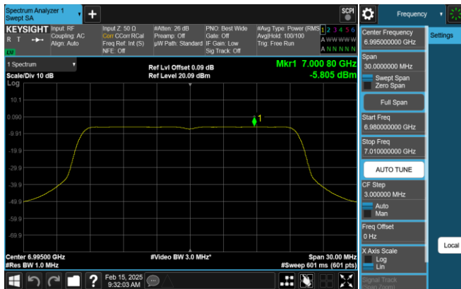
Plot 7-330. PSD Plot SDM Antenna 1 (20MHz 802.11ax RU242 (UNII Band 8) - Ch. 209)
