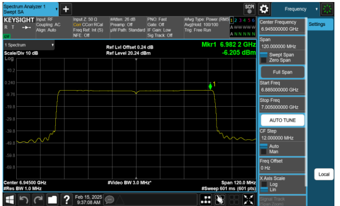
Plot 7-334. PSD Plot SDM Antenna 1 (80MHz 802.11ax RU996 (UNII Band 8) - Ch. 199)
