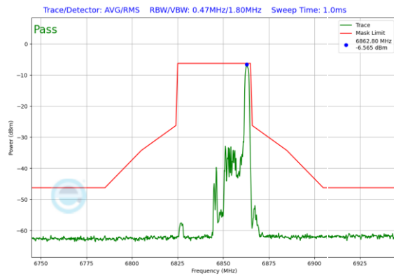
Plot 7-378. In-Band Emission Plot Antenna 0 (40MHz 802.11ax RU26 (UNII Band 7) – Ch. 179)
