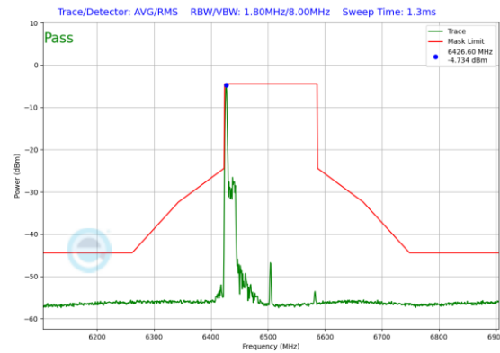
Plot 7-372. In-Band Emission Plot Antenna 0 (160MHz 802.11ax RU26 (UNII Band 6) – Ch. 111)
