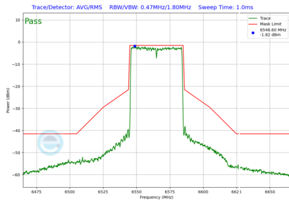
Plot 7-358. In-Band Emission Plot Antenna 0 (40MHz 802.11ax RU484 (UNII Band 7) – Ch. 123)
