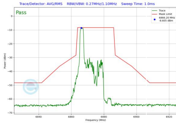
Plot 7-377. In-Band Emission Plot Antenna 0 (20MHz 802.11ax RU26 (UNII Band 7) – Ch. 185)
