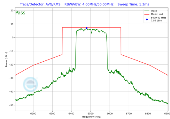
Plot 7-352. In-Band Emission Plot Antenna 0 (160MHz 802.11ax RU996x2 (UNII Band 6) – Ch. 111)
