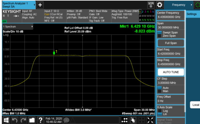
Plot 7-297. PSD Plot SDM Antenna 0 (20MHz 802.11ax RU242 (UNII Band 6) - Ch. 97)
