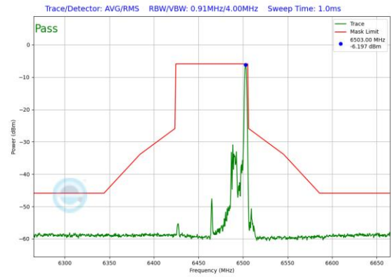
Plot 7-371. In-Band Emission Plot Antenna 0 (80MHz 802.11ax RU26 (UNII Band 6) – Ch. 103)
