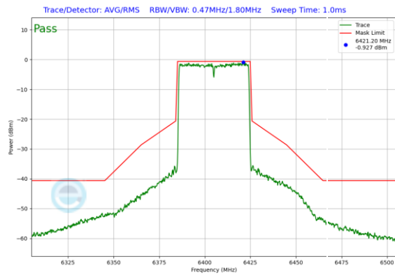
Plot 7-342. In-Band Emission Plot Antenna 0 (40MHz 802.11ax RU484 (UNII Band 5) – Ch. 91)
