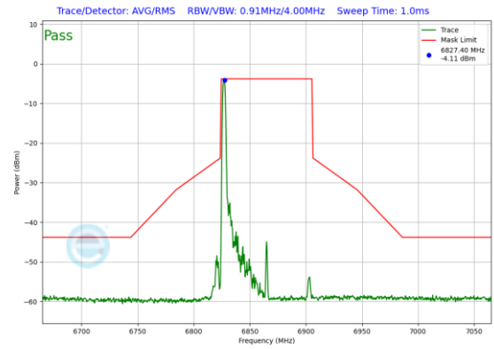
Plot 7-379. In-Band Emission Plot Antenna 0 (80MHz 802.11ax RU26 (UNII Band 7) – Ch. 183)
