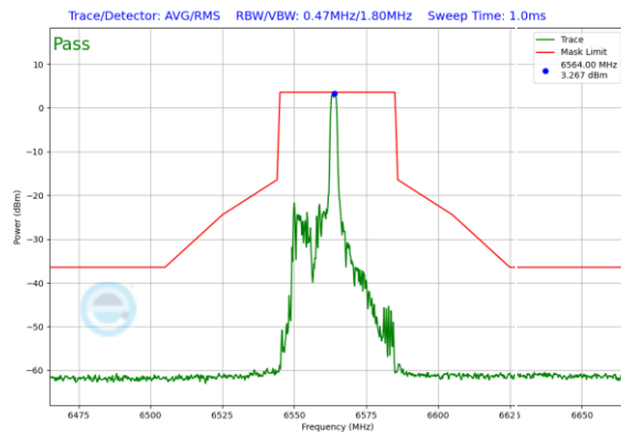
Plot 7-354. In-Band Emission Plot Antenna 0 (40MHz 802.11ax RU26 (UNII Band 7) – Ch. 123)
