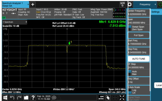
Plot 7-319. PSD Plot SDM Antenna 0 (160MHz 802.11ax RU996x2 (UNII Band 7) – Ch. 175)
