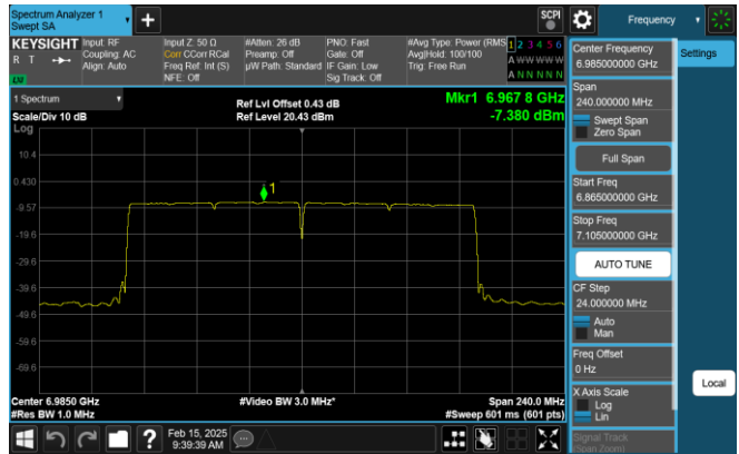
Plot 7-336. PSD Plot SDM Antenna 1 (160MHz 802.11ax RU996x2 (UNII Band 8) – Ch. 207)
