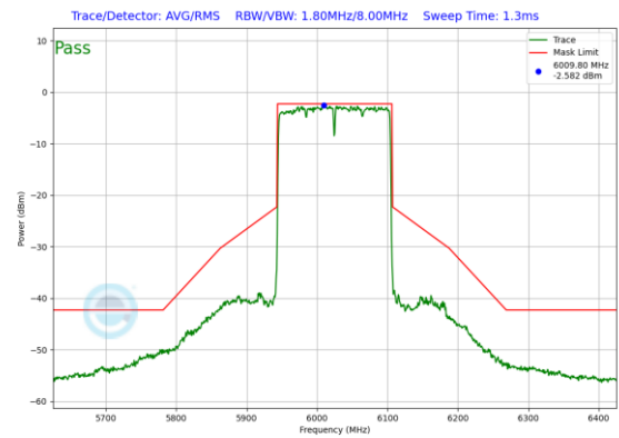
Plot 7-344. In-Band Emission Plot Antenna 0 (160MHz 802.11ax RU996x2 (UNII Band 5) – Ch. 15)
