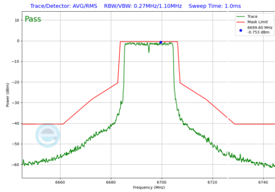
Plot 7-357. In-Band Emission Plot Antenna 0 (20MHz 802.11ax RU242 (UNII Band 7) – Ch. 149)
