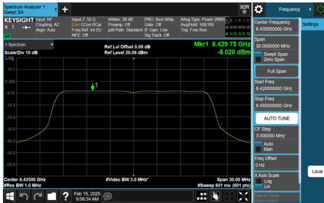
Plot 7-298. PSD Plot SDM Antenna 1 (20MHz 802.11ax RU242 (UNII Band 6) - Ch. 97)
