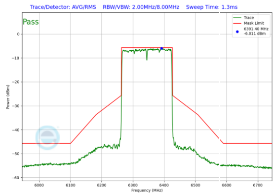
Plot 7-511. In-Band Emission Plot SDM Antenna 0 (160MHz 802.11ax RU996x2 (UNII Band 5) – Ch. 79)
