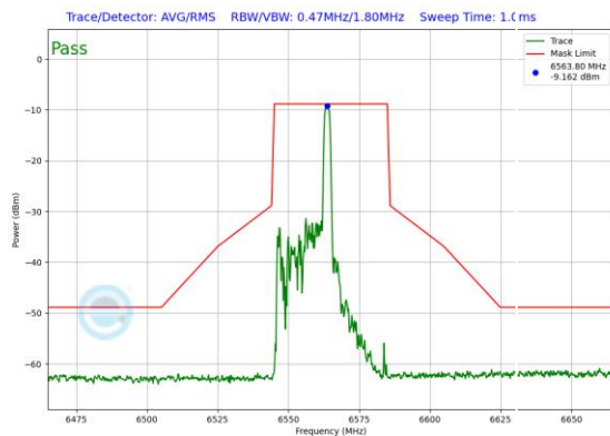
Plot 7-531. In-Band Emission Plot SDM Antenna 0 (40MHz 802.11ax RU26 (UNII Band 7) – Ch. 123)
