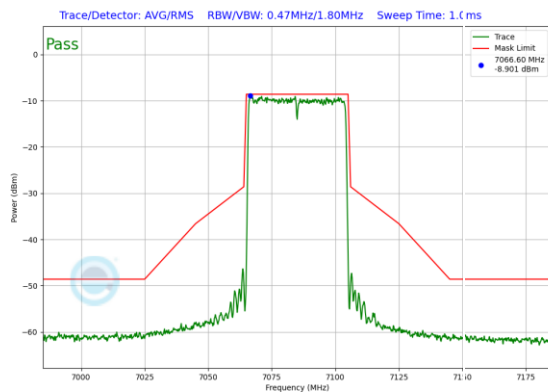
Plot 7-555. In-Band Emission Plot SDM Antenna 0 (40MHz 802.11ax RU484 (UNII Band 8) – Ch. 227)
