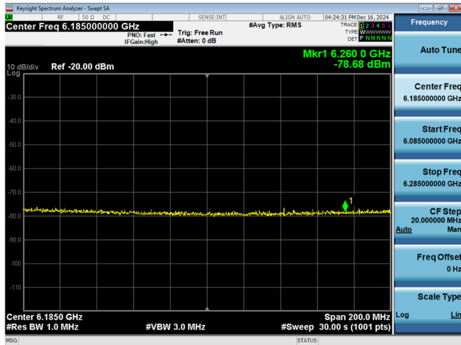
Plot 7-597. 160MHz Bandwidth, AWGN Signal Injected at High End – Channel 47
