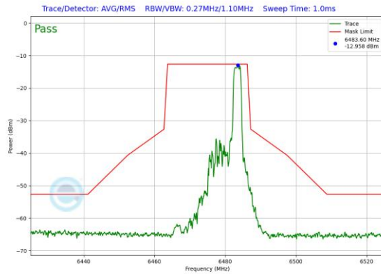
Plot 7-513. In-Band Emission Plot SDM Antenna 0 (20MHz 802.11ax RU26 (UNII Band 6) – Ch. 105)
