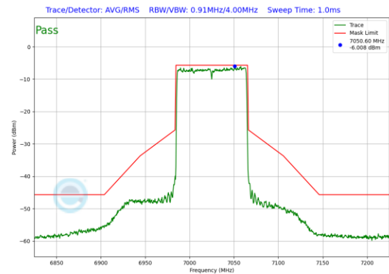
Plot 7-557. In-Band Emission Plot SDM Antenna 0 (80MHz 802.11ax RU996 (UNII Band 8) – Ch. 215)
