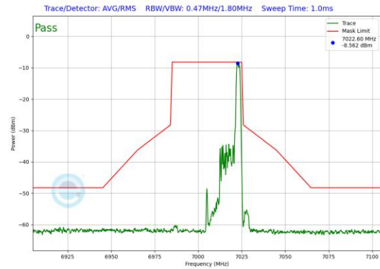
Plot 7-548. In-Band Emission Plot SDM Antenna 1 (40MHz 802.11ax RU26 (UNII Band 8) – Ch. 211)
