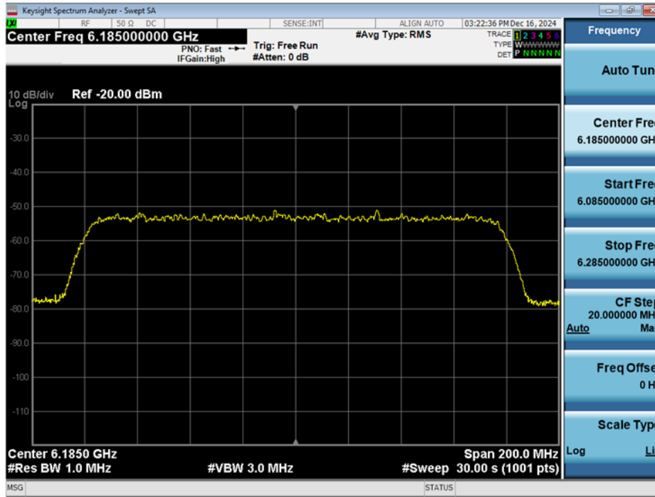
Plot 7-594. 160MHz Bandwidth, Before AWGN Signal Injected – Channel 47
