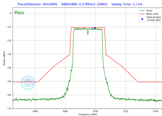
Plot 7-554. In-Band Emission Plot SDM Antenna 1 (20MHz 802.11ax RU242 (UNII Band 8) – Ch. 229)
