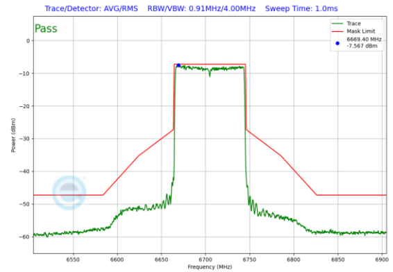
Plot 7-541. In-Band Emission Plot SDM Antenna 0 (80MHz 802.11ax RU996 (UNII Band 7) – Ch. 151)
