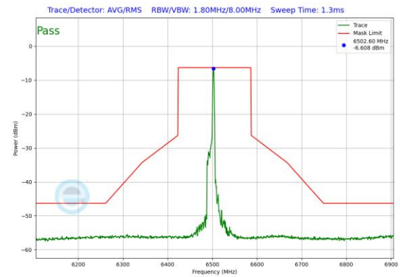
Plot 7-520. In-Band Emission Plot SDM Antenna 1 (160MHz 802.11ax RU26 (UNII Band 6) – Ch. 111)
