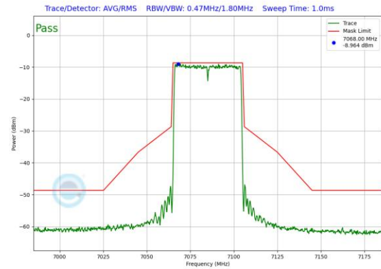
Plot 7-556. In-Band Emission Plot SDM Antenna 1 (40MHz 802.11ax RU484 (UNII Band 8) – Ch. 227)
