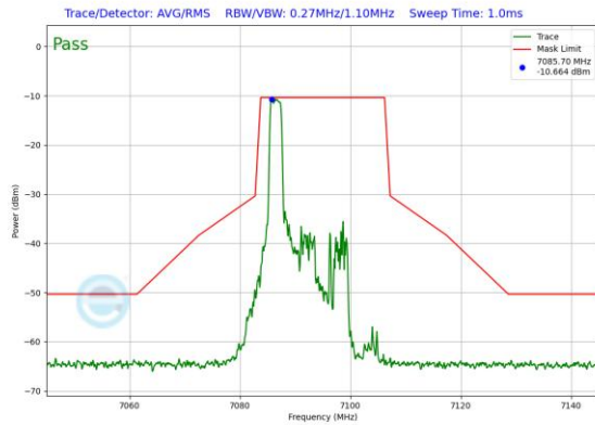
Plot 7-545. In-Band Emission Plot SDM Antenna 0 (20MHz 802.11ax RU26 (UNII Band 8) – Ch. 229)
