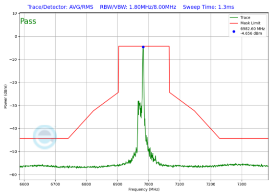
Plot 7-552. In-Band Emission Plot SDM Antenna 1 (160MHz 802.11ax RU26 (UNII Band 8) – Ch. 207)
