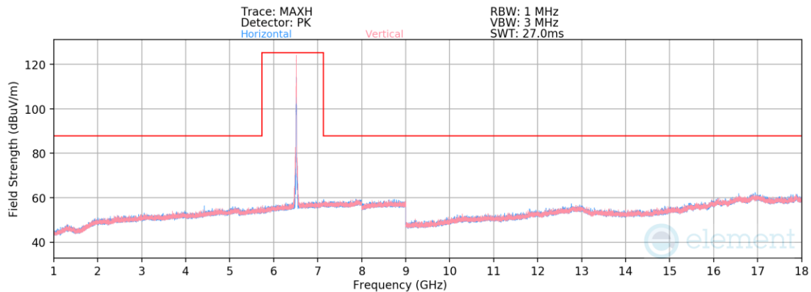
Plot 7-605. Radiated Spurious Emissions above 1GHz SDM (802.11ax – Ch. 113 – RU26)
