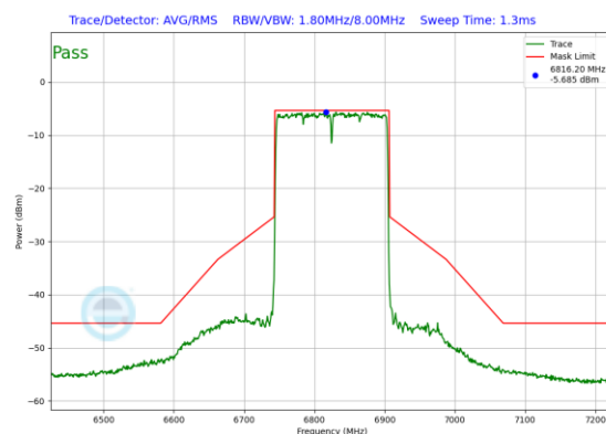
Plot 7-544. In-Band Emission Plot SDM Antenna 1 (160MHz 802.11ax RU996x2 (UNII Band 7) – Ch. 175)
