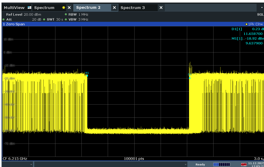
Plot 7-578. Contention Based Protocol Timing Plot – UNII 5 – 20MHz Channel 53
