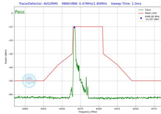
Plot 7-516. In-Band Emission Plot SDM Antenna 1 (40MHz 802.11ax RU26 (UNII Band 6) – Ch. 107)
