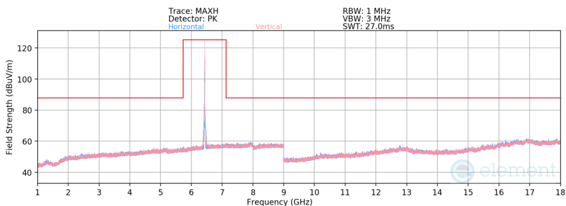
Plot 7-602. Radiated Spurious Emissions above 1GHz SDM (802.11ax – Ch. 97 – RU26)
