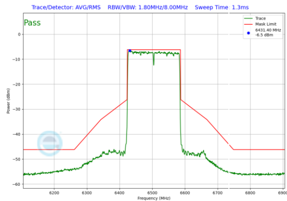
Plot 7-527. In-Band Emission Plot SDM Antenna 0 (160MHz 802.11ax RU996x2 (UNII Band 6) – Ch. 111)
