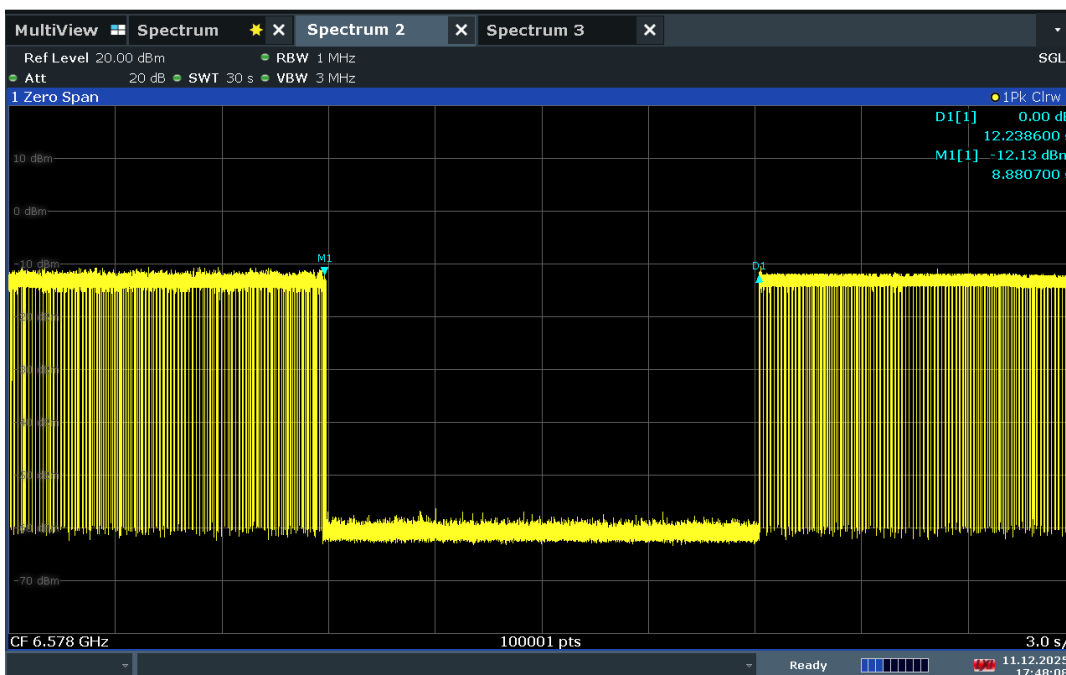
Plot 7-585. Contention Based Protocol Timing Plot – UNII 6 – 160MHz Channel 111 – High
