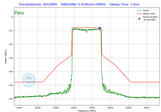
Plot 7-510. In-Band Emission Plot SDM Antenna 1 (80MHz 802.11ax RU996 (UNII Band 5) – Ch. 87)
