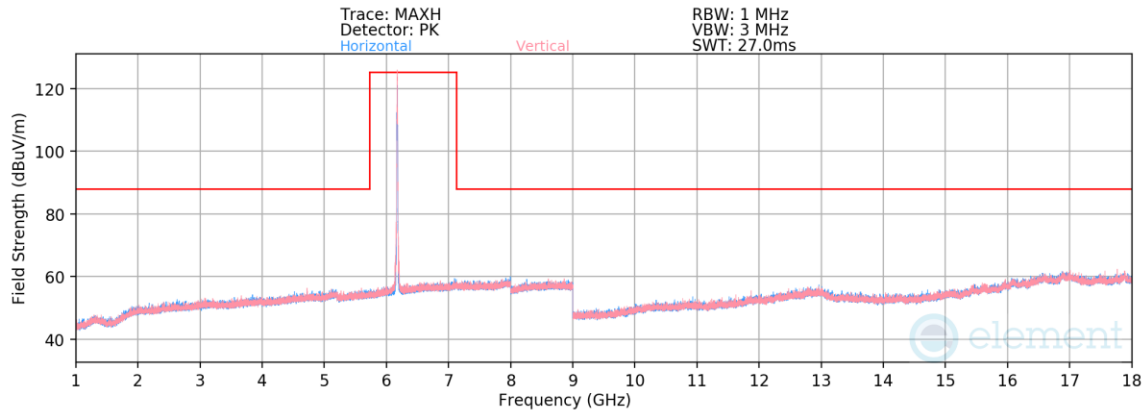
Plot 7-600. Radiated Spurious Emissions above 1GHz SDM (802.11ax – Ch. 45 – RU26)
