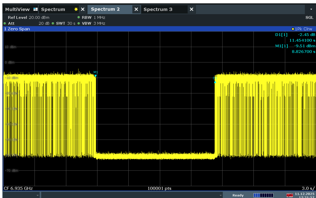
Plot 7-590. Contention Based Protocol Timing Plot – UNII 8 – 20MHz Channel 197
