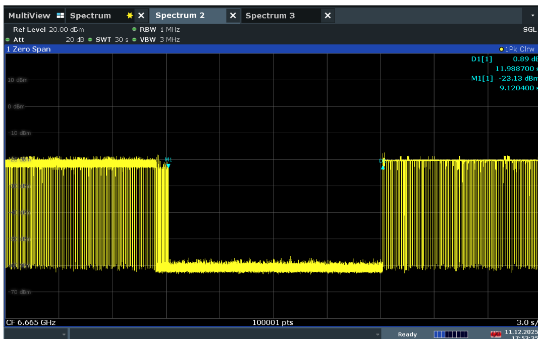
Plot 7-588. Contention Based Protocol Timing Plot – UNII 7 – 160MHz Channel 143 – Mid
