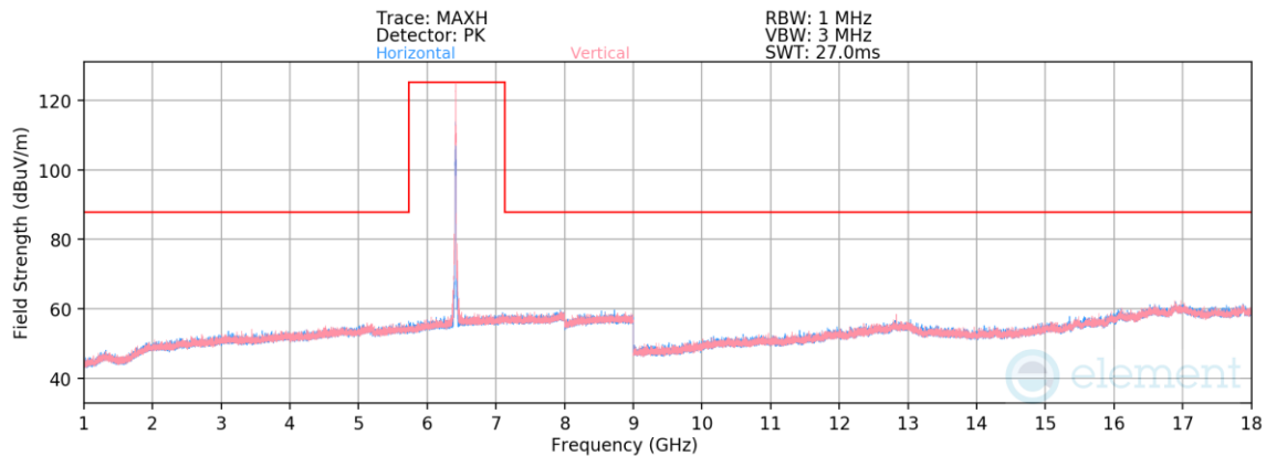
Plot 7-601. Radiated Spurious Emissions above 1GHz SDM (802.11ax – Ch. 93 – RU26)
