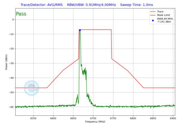
Plot 7-534. In-Band Emission Plot SDM Antenna 1 (80MHz 802.11ax RU26 (UNII Band 7) – Ch. 151)
