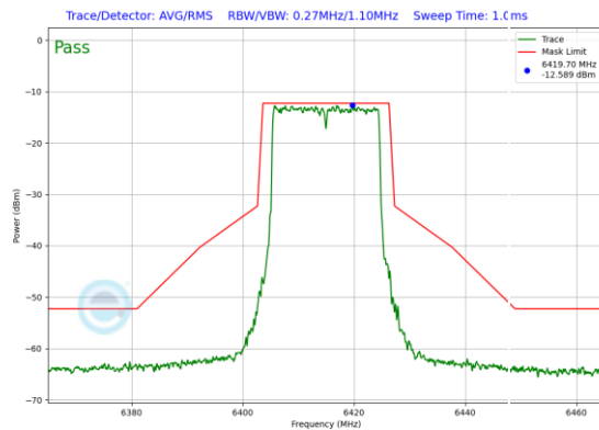
Plot 7-506. In-Band Emission Plot SDM Antenna 1 (20MHz 802.11ax RU242 (UNII Band 5) – Ch. 93)
