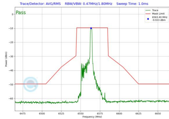
Plot 7-532. In-Band Emission Plot SDM Antenna 1 (40MHz 802.11ax RU26 (UNII Band 7) – Ch. 123)
