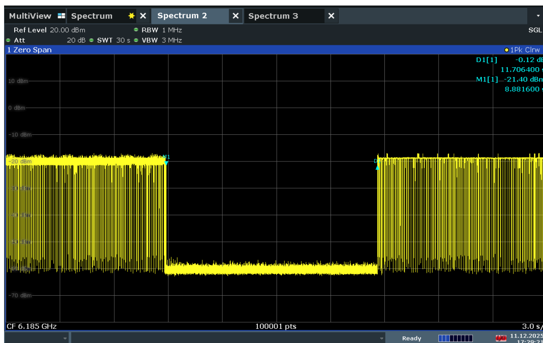
Plot 7-580. Contention Based Protocol Timing Plot –UNII 5 – 160MHz Channel 47 – Mid
