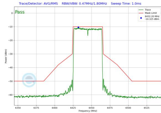
Plot 7-524. In-Band Emission Plot SDM Antenna 1 (40MHz 802.11ax RU484 (UNII Band 6) – Ch. 99)
