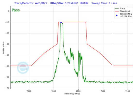
Plot 7-546. In-Band Emission Plot SDM Antenna 1 (20MHz 802.11ax RU26 (UNII Band 8) – Ch. 229)
