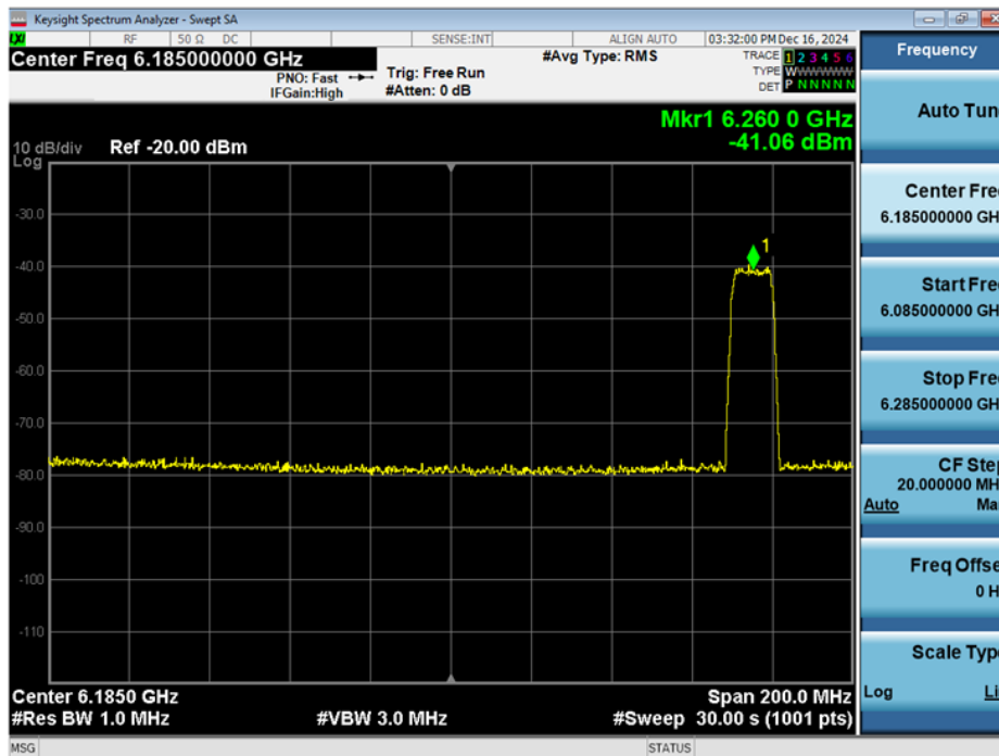
Plot 7-595. 160MHz Bandwidth, AWGN Signal Injected at Low End – Channel 47
