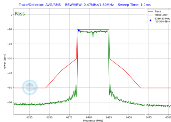
Plot 7-507. In-Band Emission Plot SDM Antenna 0 (40MHz 802.11ax RU484 (UNII Band 5) – Ch. 91)
