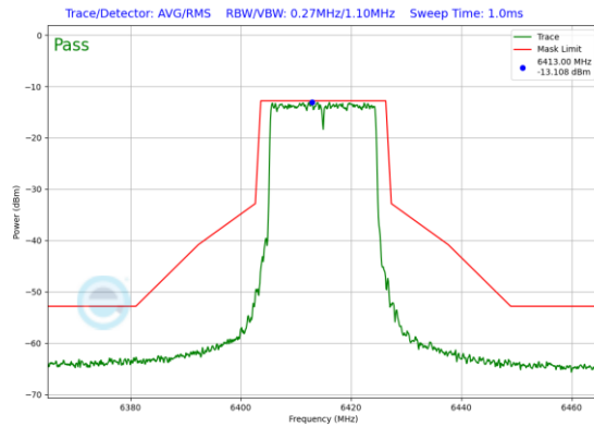
Plot 7-505. In-Band Emission Plot SDM Antenna 0 (20MHz 802.11ax RU242 (UNII Band 5) – Ch. 93)
