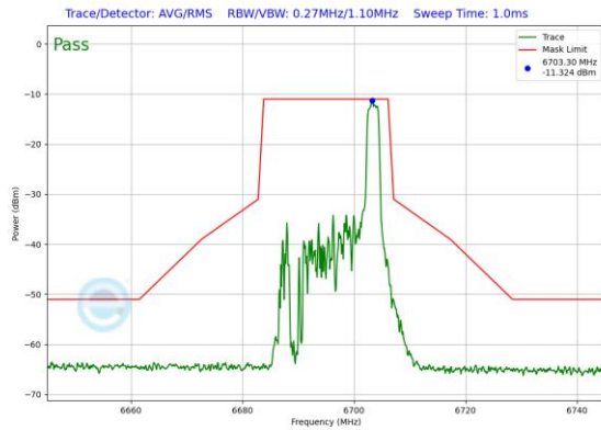
Plot 7-529. In-Band Emission Plot SDM Antenna 0 (20MHz 802.11ax RU26 (UNII Band 7) – Ch. 149)
