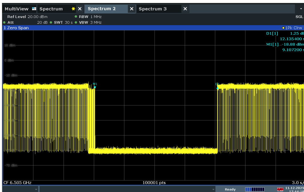
Plot 7-584. Contention Based Protocol Timing Plot – UNII 6 – 160MHz Channel 111 – Mid
