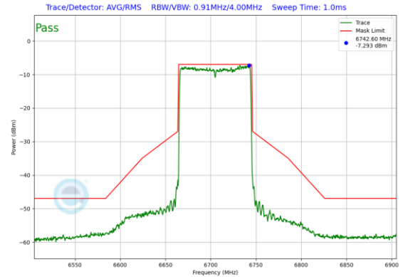
Plot 7-542. In-Band Emission Plot SDM Antenna 1 (80MHz 802.11ax RU996 (UNII Band 7) – Ch. 151)
