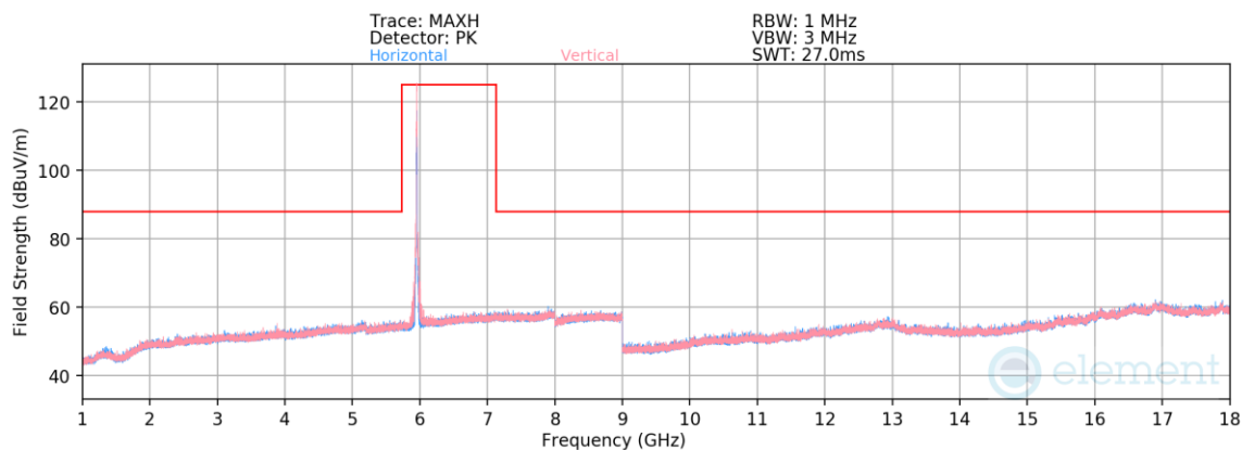
Plot 7-598. Radiated Spurious Emissions above 1GHz SDM (802.11ax – Ch. 1 – RU26)
