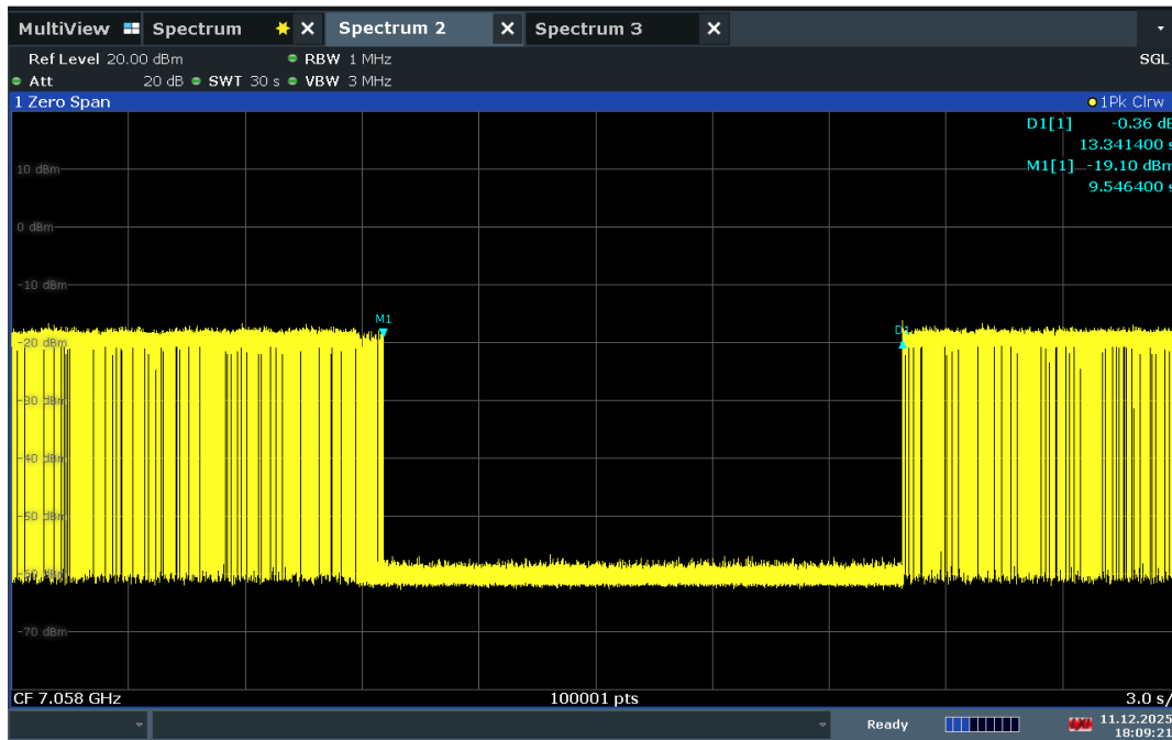
Plot 7-593. Contention Based Protocol Timing Plot – UNII 8 – 160MHz Channel 207 – High
