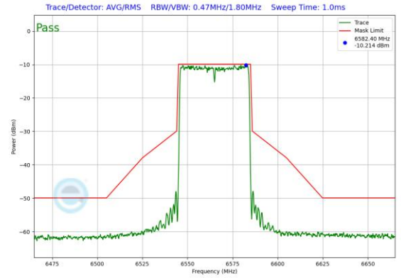
Plot 7-540. In-Band Emission Plot SDM Antenna 1 (40MHz 802.11ax RU484 (UNII Band 7) – Ch. 123)
