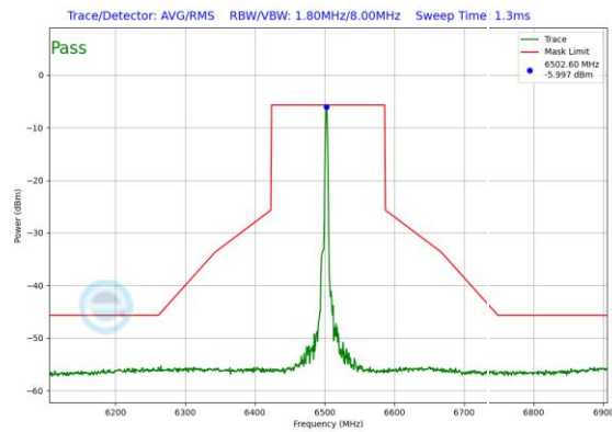
Plot 7-519. In-Band Emission Plot SDM Antenna 0 (160MHz 802.11ax RU26 (UNII Band 6) – Ch. 111)
