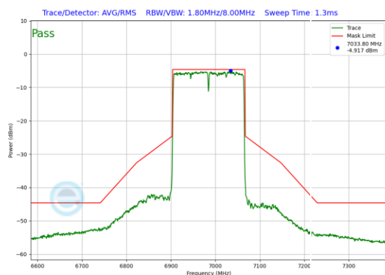
Plot 7-559. In-Band Emission Plot SDM Antenna 0 (160MHz 802.11ax RU996x2 (UNII Band 8) – Ch. 207)
