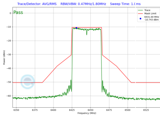
Plot 7-523. In-Band Emission Plot SDM Antenna 0 (40MHz 802.11ax RU484 (UNII Band 6) – Ch. 99)
