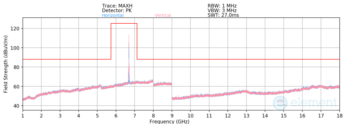
Plot 7-607. Radiated Spurious Emissions above 1GHz SDM (802.11ax – Ch. 149 – RU26)
