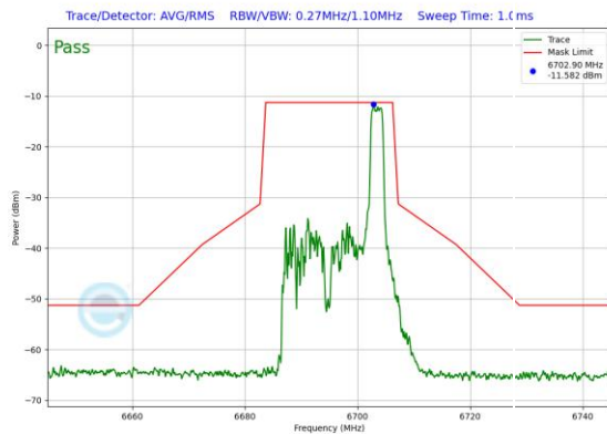
Plot 7-530. In-Band Emission Plot SDM Antenna 1 (20MHz 802.11ax RU26 (UNII Band 7) – Ch. 149)
