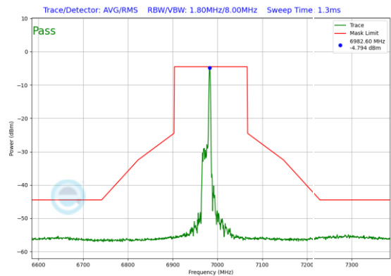
Plot 7-551. In-Band Emission Plot SDM Antenna 0 (160MHz 802.11ax RU26 (UNII Band 8) – Ch. 207)
