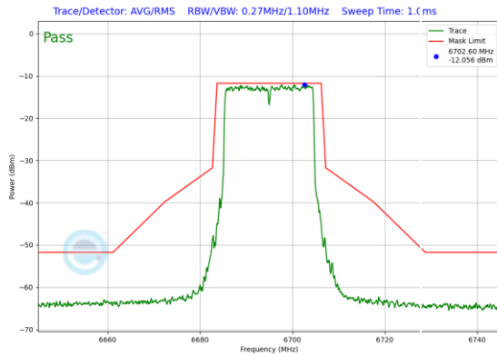
Plot 7-538. In-Band Emission Plot SDM Antenna 1 (20MHz 802.11ax RU242 (UNII Band 7) – Ch. 149)
