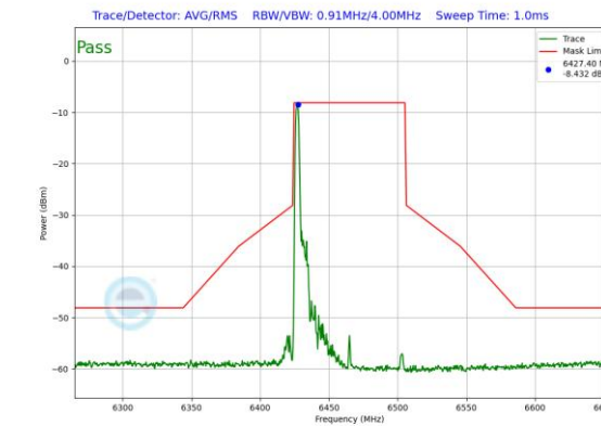
Plot 7-517. In-Band Emission Plot SDM Antenna 0 (80MHz 802.11ax RU26 (UNII Band 6) – Ch. 103)
