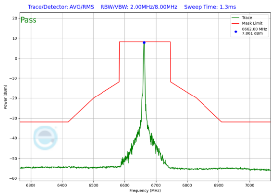
Plot 7-536. In-Band Emission Plot SDM Antenna 1 (160MHz 802.11ax RU26 (UNII Band 7) – Ch. 143)
