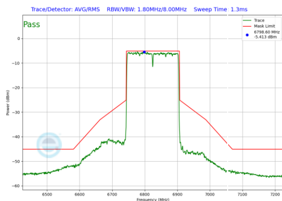
Plot 7-543. In-Band Emission Plot SDM Antenna 0 (160MHz 802.11ax RU996x2 (UNII Band 7) – Ch. 175)
