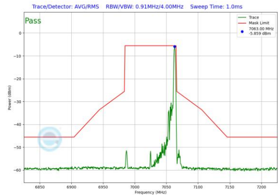
Plot 7-549. In-Band Emission Plot SDM Antenna 0 (80MHz 802.11ax RU26 (UNII Band 8) – Ch. 215)
