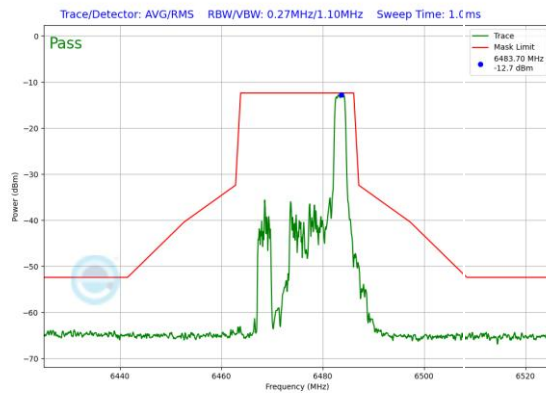
Plot 7-514. In-Band Emission Plot SDM Antenna 1 (20MHz 802.11ax RU26 (UNII Band 6) – Ch. 105)
