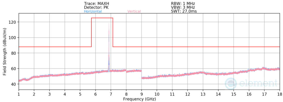
Plot 7-609. Radiated Spurious Emissions above 1GHz SDM (802.11ax – Ch. 185 – RU26)
