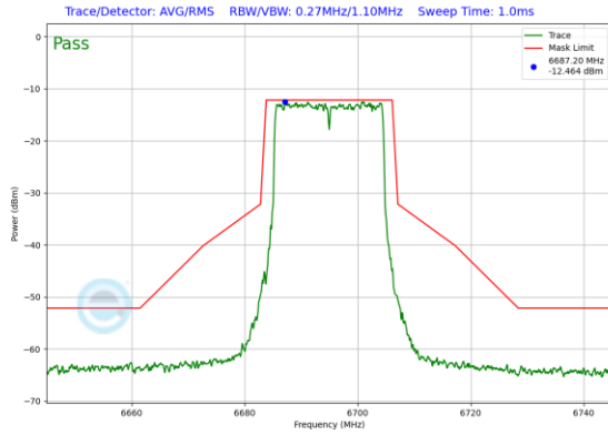
Plot 7-537. In-Band Emission Plot SDM Antenna 0 (20MHz 802.11ax RU242 (UNII Band 7) – Ch. 149)
