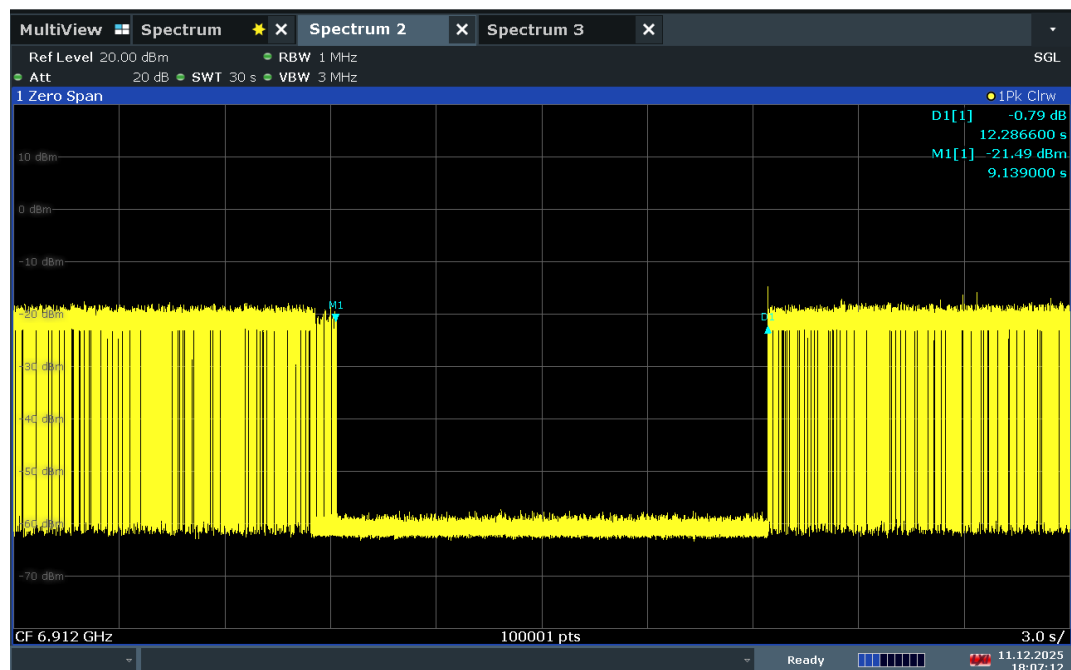
Plot 7-591. Contention Based Protocol Timing Plot – UNII 8 – 160MHz Channel 207 – Low
