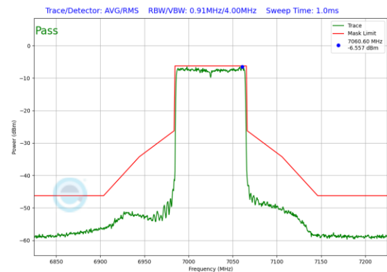
Plot 7-558. In-Band Emission Plot SDM Antenna 1 (80MHz 802.11ax RU996 (UNII Band 8) – Ch. 215)
