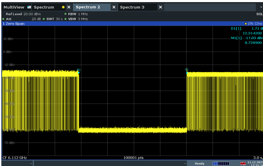
Plot 7-579. Contention Based Protocol Timing Plot – UNII 5 – 160MHz Channel 47 – Low
