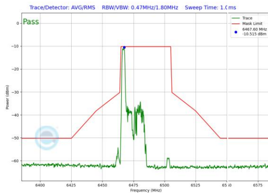
Plot 7-515. In-Band Emission Plot SDM Antenna 0 (40MHz 802.11ax RU26 (UNII Band 6) – Ch. 107)
