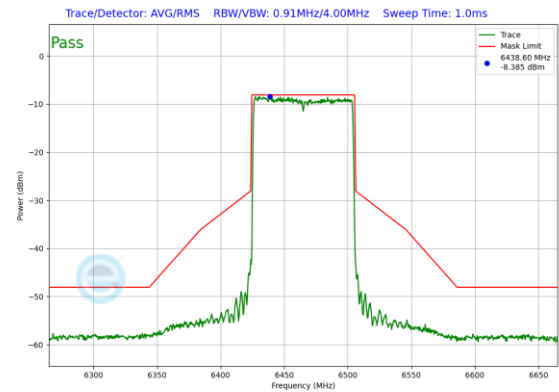
Plot 7-526. In-Band Emission Plot SDM Antenna 1 (80MHz 802.11ax RU996 (UNII Band 6) – Ch. 103)
