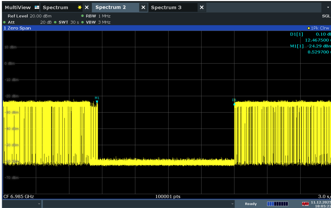
Plot 7-592. Contention Based Protocol Timing Plot – UNII 8 – 160MHz Channel 207 – Mid
