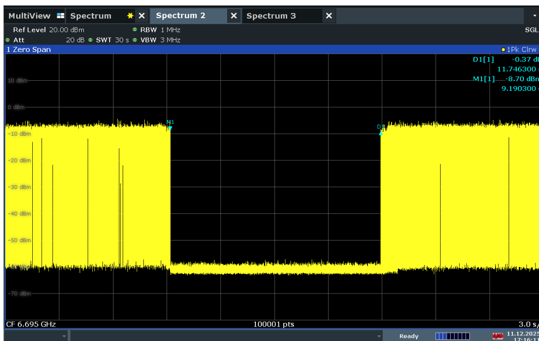
Plot 7-586. Contention Based Protocol Timing Plot – UNII 7 – 20MHz Channel 149
