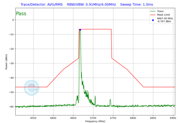
Plot 7-533. In-Band Emission Plot SDM Antenna 0 (80MHz 802.11ax RU26 (UNII Band 7) – Ch. 151)
