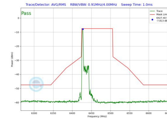
Plot 7-518. In-Band Emission Plot SDM Antenna 1 (80MHz 802.11ax RU26 (UNII Band 6) – Ch. 103)
