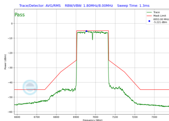
Plot 7-560. In-Band Emission Plot SDM Antenna 1 (160MHz 802.11ax RU996x2 (UNII Band 8) – Ch. 207)
