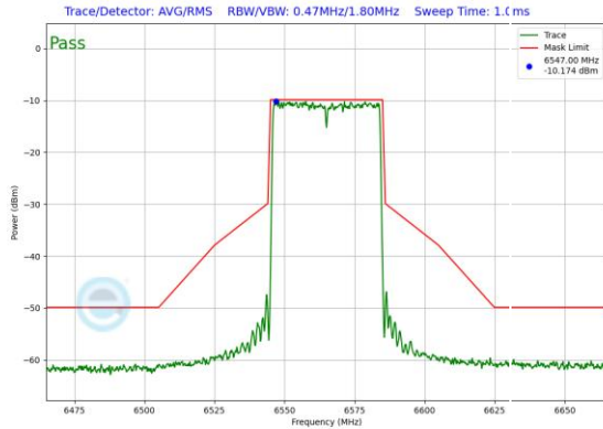
Plot 7-539. In-Band Emission Plot SDM Antenna 0 (40MHz 802.11ax RU484 (UNII Band 7) – Ch. 123)
