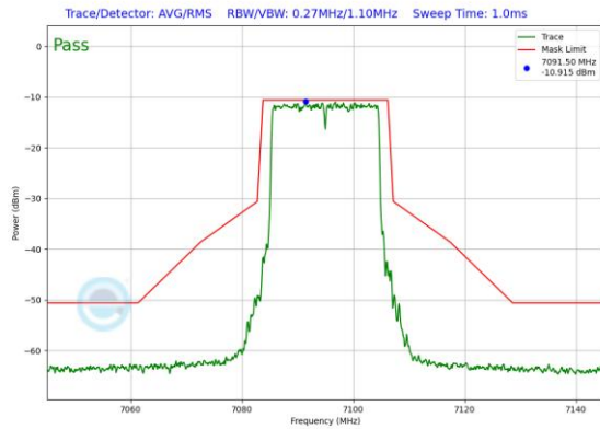
Plot 7-553. In-Band Emission Plot SDM Antenna 0 (20MHz 802.11ax RU242 (UNII Band 8) – Ch. 229)
