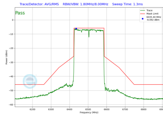
Plot 7-528. In-Band Emission Plot SDM Antenna 1 (160MHz 802.11ax RU996x2 (UNII Band 6) – Ch. 111)
