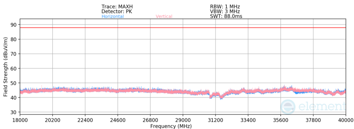
Plot 7-603. Radiated Spurious Emissions 18-40GHz SDM (802.11ax – Ch. 97 – RU26)
