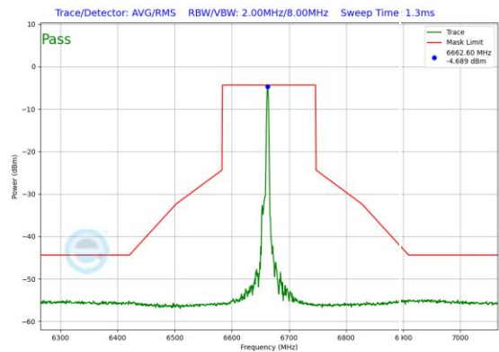
Plot 7-535. In-Band Emission Plot SDM Antenna 0 (160MHz 802.11ax RU26 (UNII Band 7) – Ch. 143)
