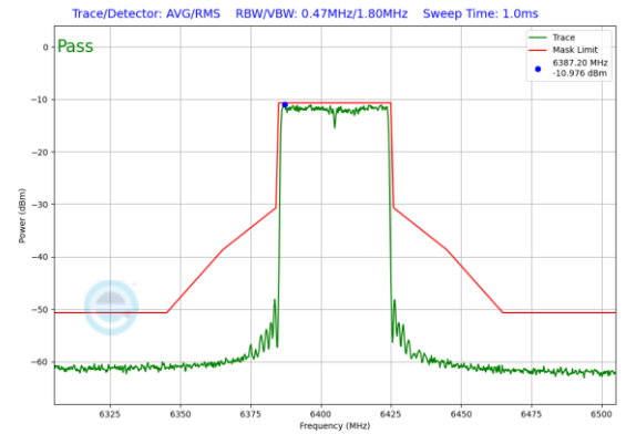
Plot 7-508. In-Band Emission Plot SDM Antenna 1 (40MHz 802.11ax RU484 (UNII Band 5) – Ch. 91)
