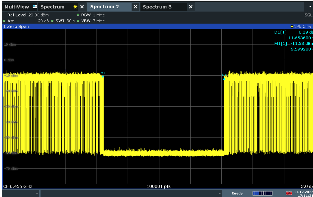
Plot 7-582. Contention Based Protocol Timing Plot – UNII 6 – 20MHz Channel 101
