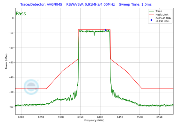
Plot 7-509. In-Band Emission Plot SDM Antenna 0 (80MHz 802.11ax RU996 (UNII Band 5) – Ch. 87)
