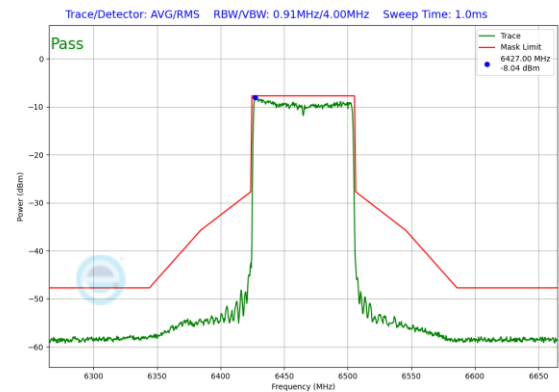
Plot 7-525. In-Band Emission Plot SDM Antenna 0 (80MHz 802.11ax RU996 (UNII Band 6) – Ch. 103)
