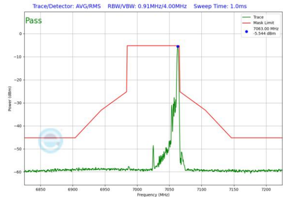
Plot 7-550. In-Band Emission Plot SDM Antenna 1 (80MHz 802.11ax RU26 (UNII Band 8) – Ch. 215)
