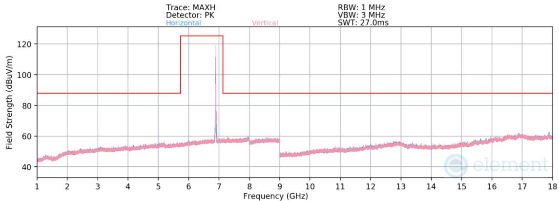
Plot 7-610. Radiated Spurious Emissions above 1GHz SDM (802.11ax – Ch. 189 – RU26)
