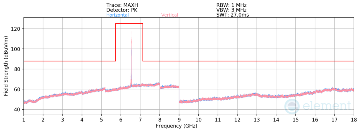
Plot 7-606. Radiated Spurious Emissions above 1GHz SDM (802.11ax – Ch. 117 – RU26)
