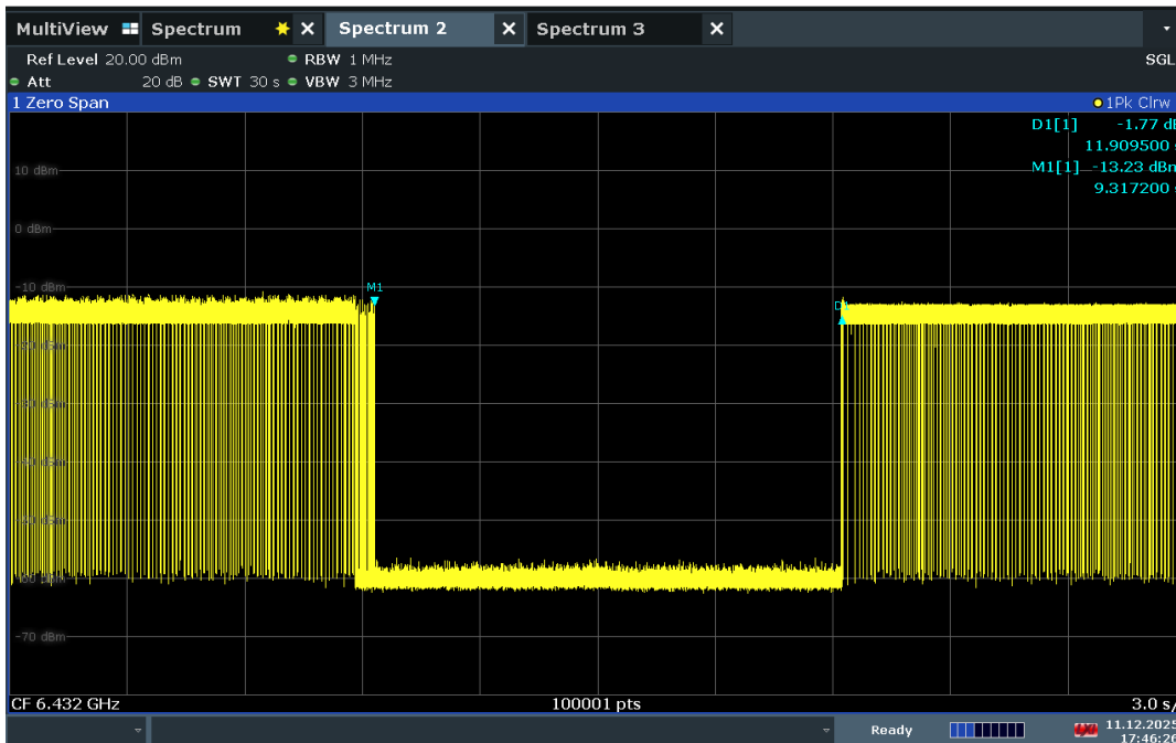
Plot 7-583. Contention Based Protocol Timing Plot – UNII 6 – 160MHz Channel 111 – Low
