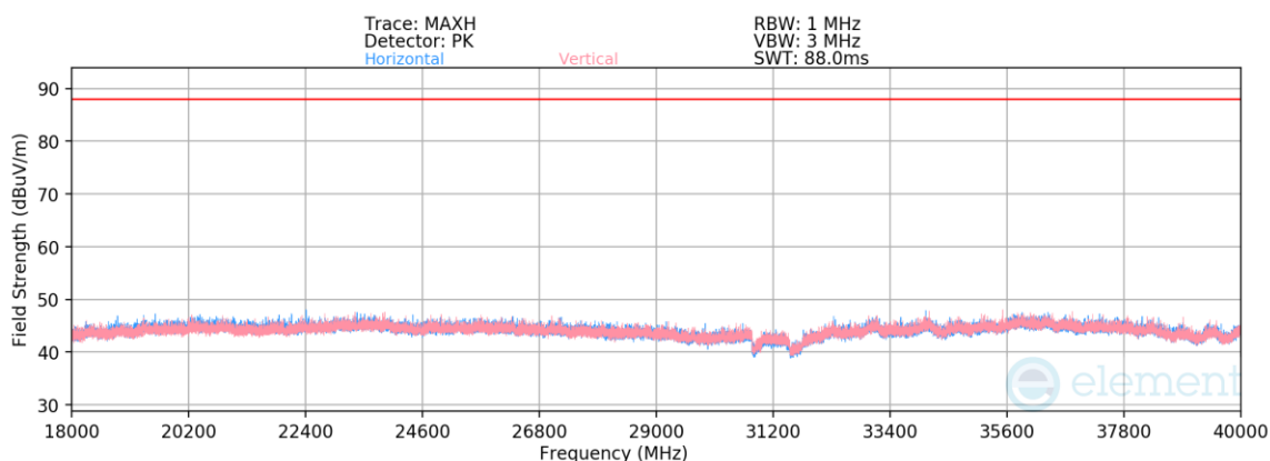
Plot 7-599. Radiated Spurious Emissions 18-40GHz SDM (802.11ax – Ch. 1 – RU26)
