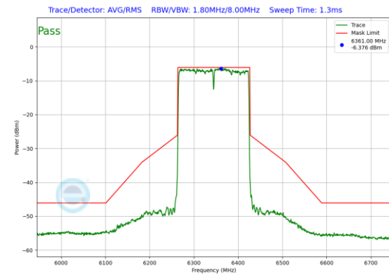
Plot 7-512. In-Band Emission Plot SDM Antenna 1 (160MHz 802.11ax RU996x2 (UNII Band 5) – Ch. 79)
