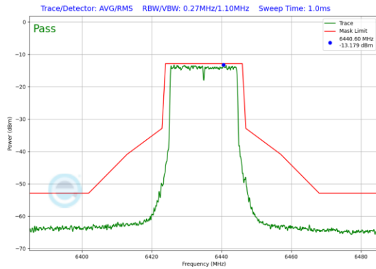
Plot 7-521. In-Band Emission Plot SDM Antenna 0 (20MHz 802.11ax RU242 (UNII Band 6) – Ch. 97)
