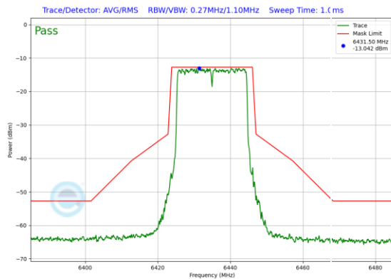
Plot 7-522. In-Band Emission Plot SDM Antenna 1 (20MHz 802.11ax RU242 (UNII Band 6) – Ch. 97)
