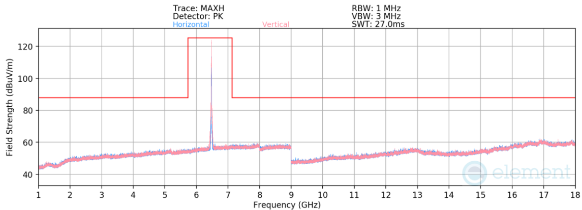
Plot 7-604. Radiated Spurious Emissions above 1GHz SDM (802.11ax – Ch. 105 – RU26)
