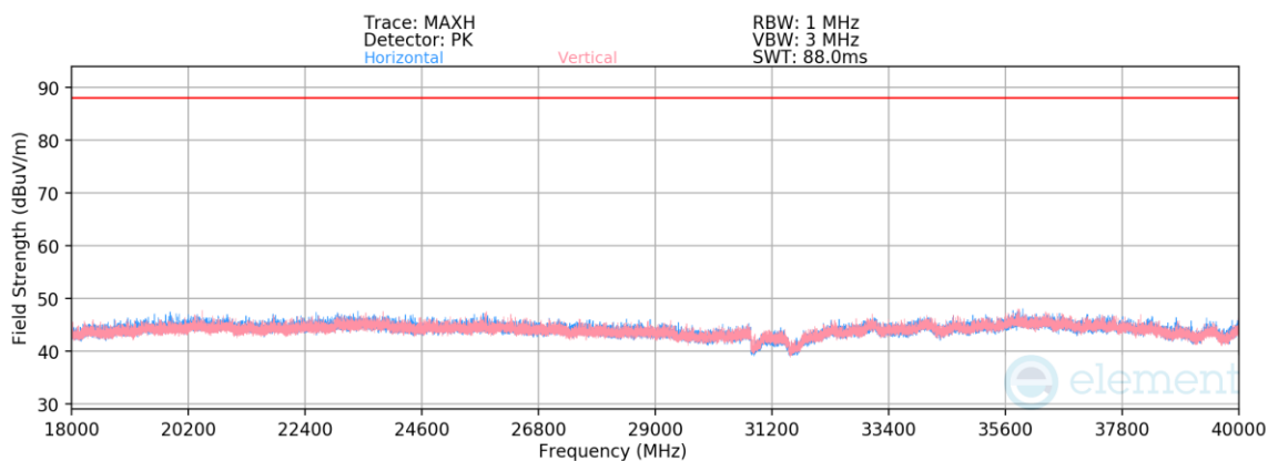
Plot 7-608. Radiated Spurious Emissions 18-40GHz SDM (802.11ax – Ch. 149 – RU26)
